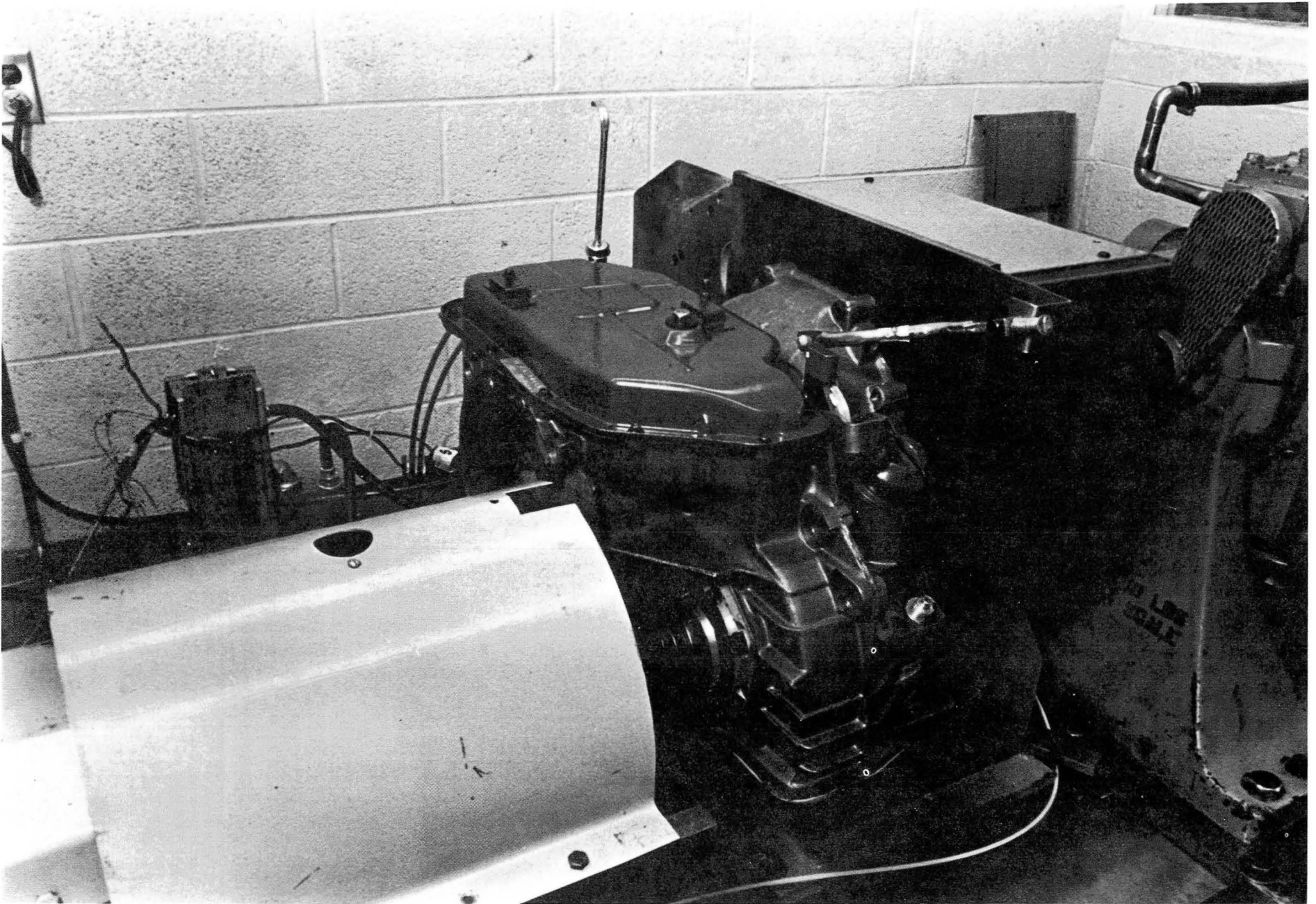
1981 Mercury Lynx Coast Performance Test Setup Side View
