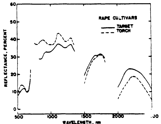
Fig. 1. Spectroradiometrically measured reflectance over the 500 to 2,500-nm wavelength for plants of the Target and Torch rape cultivars in soil-containing flats.
