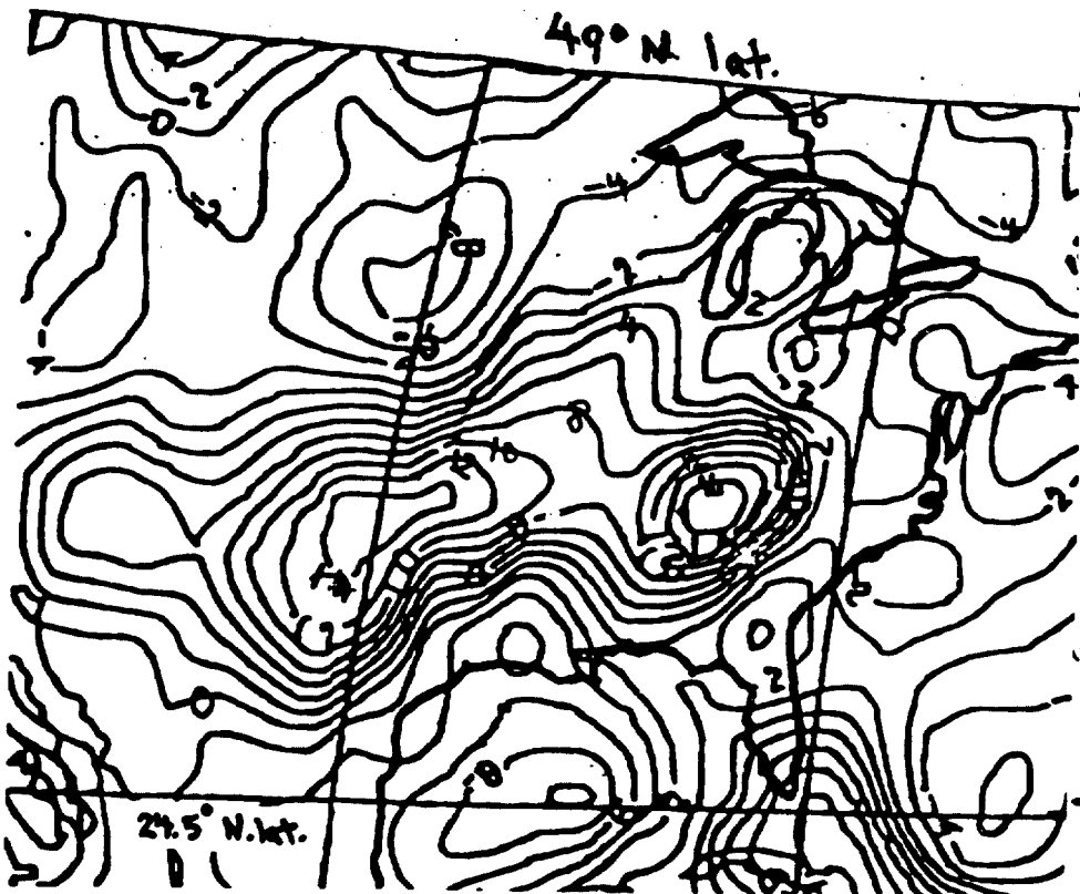
Contour Interval = 2 gammas
