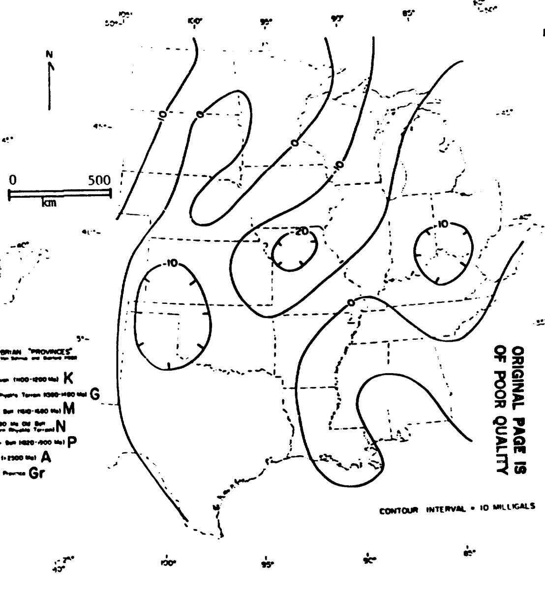
FIGURE 6. Wavelength-filtered, 1°x1° free-air gravity anomaly. (from Von Frese et al, 1980)
