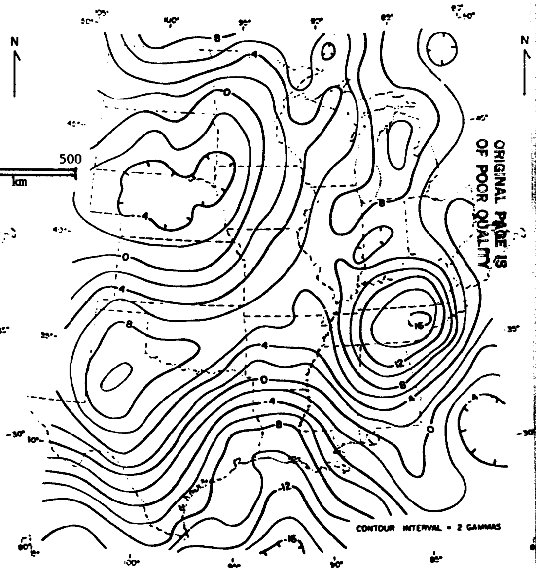
FIGURE 2. Low-cut (400 km) wavelength-filtered scalar data of Fig. 1
