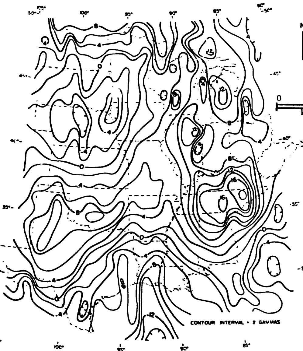
FIGURE 1. 1^{\circ} \times 1^{\circ} weighted-averaged Magsat scalar (magnitude) data, for the U.S. midcontinent. Albers equal-area projection. Plot by Black (1981).
