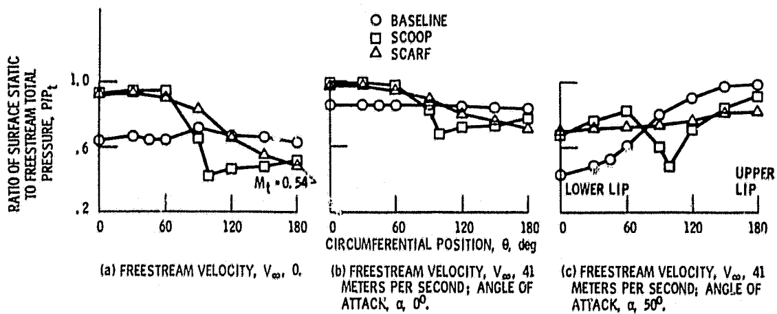
Figure 2. - Circumferential variation of measured surface static pressure at high/lift. Inlet throat Mach number, M_t = 0.63 except as indicated (ref. 5).
