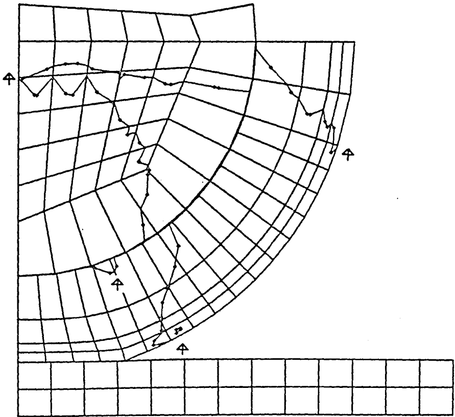
FIGURE H-13. CONTOURS OF HOOP STRESS AFTER 0.25 ms OF IMPACT (152 m/s IMPACT VELOCITY)
