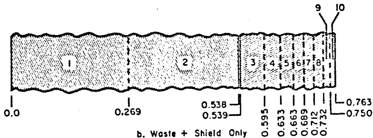
FIGURE 5-6. RING GEOMETRY FOR TWO MAJOR CONFIGURATIONS ANALYZED
