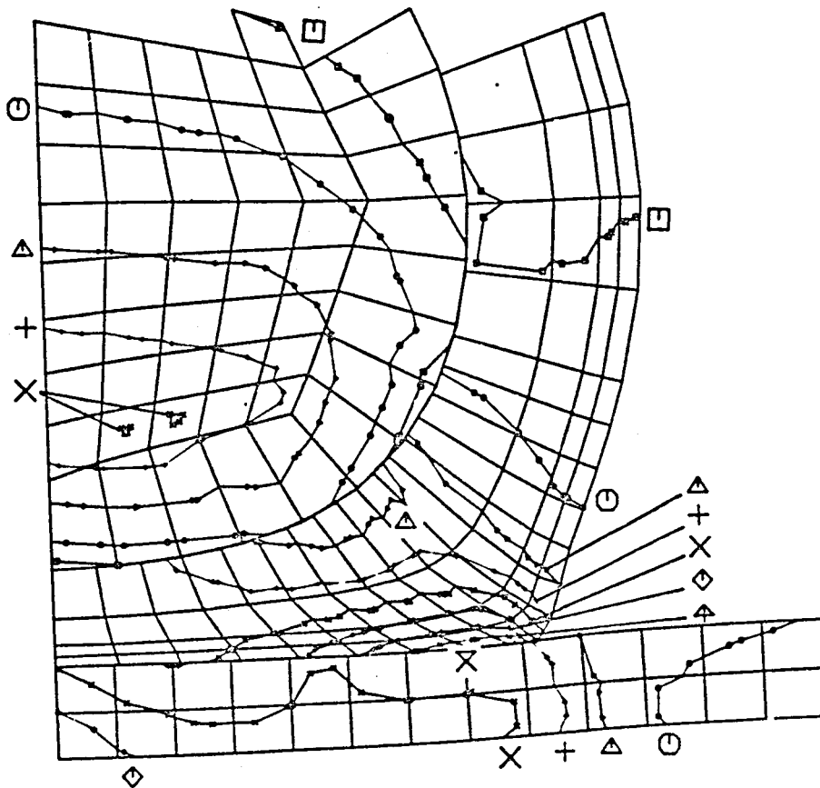
FIGURE H-2. CONTOURS OF VON MISES STRESS AFTER 0.50 ms OF IMPACT (442 m/s IMPACT VELOCITY)
