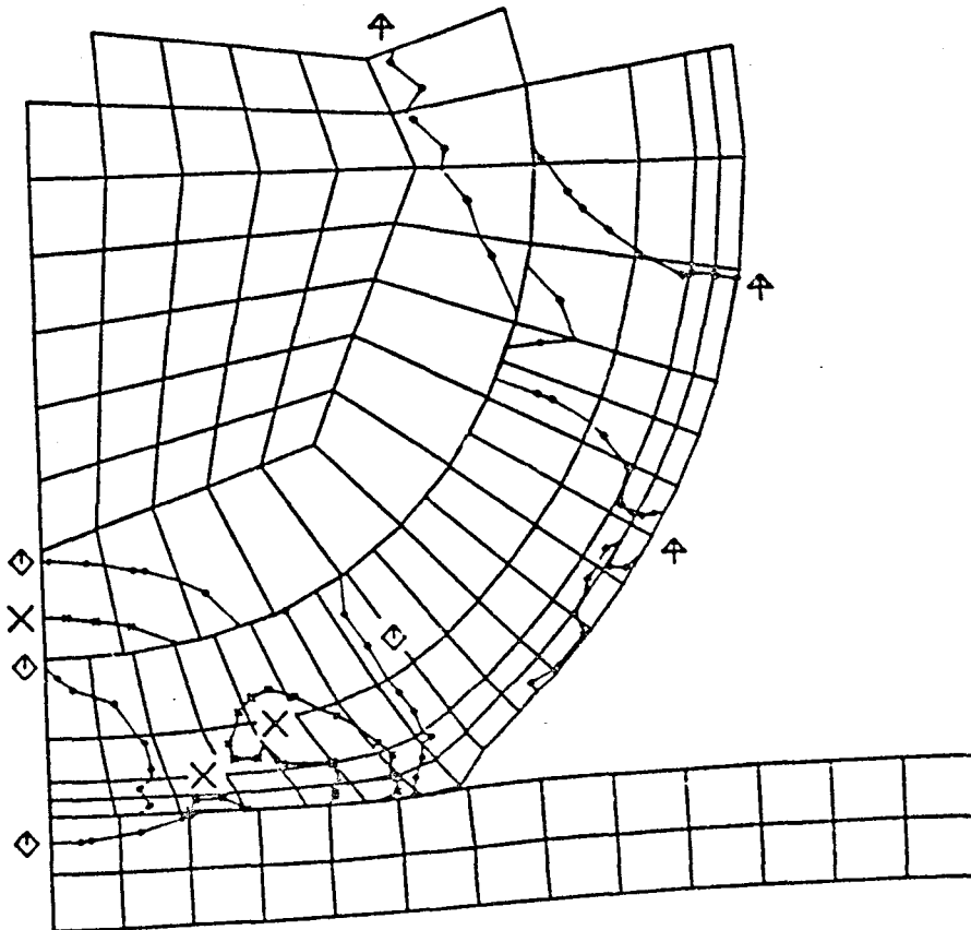
FIGURE H-5. CONTOURS OF HOOP STRESS AFTER 0.25 ms OF IMPACT (442 m/s IMPACT VELOCITY)
