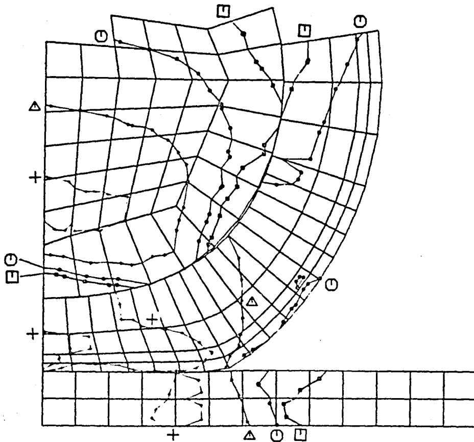
FIGURE H-11. CONTOURS OF VON MISES STRESS AFTER 0.75 ms OF IMPACT (152 m/s IMPACT VELOCITY)
