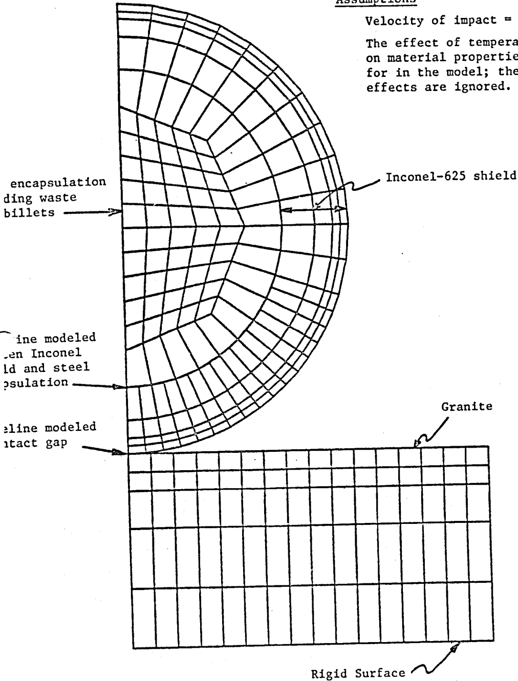
FIGURE 5-9. FINITE-ELEMENT MODEL FOR NUCLEAR WASTE PAYLOAD IMPACTING GRANITE
