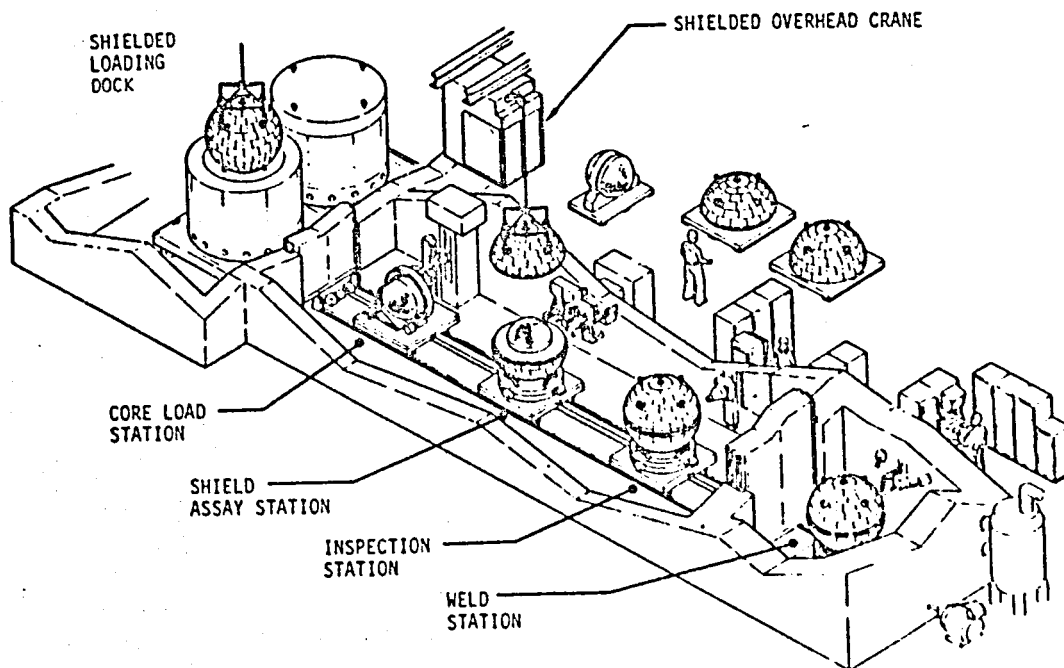
FIGURE 3-3. WASTE PAYLOAD ASSEMBLY FACILITY (FROM BOEING STUDY)
