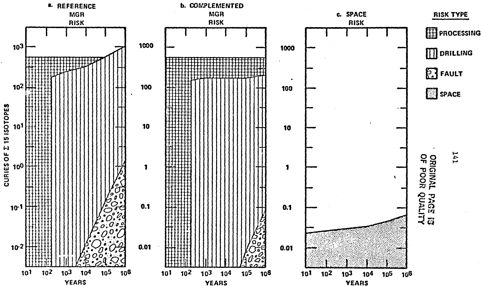
FIGURE 7-1. INTEGRATED EXPECTED CUMULATIVE RELEASE RISK COMPARISONS (IN CURIE SUM OF 15 EPA ISOTOPES) FOR HLW DISPOSAL IN SPACE
