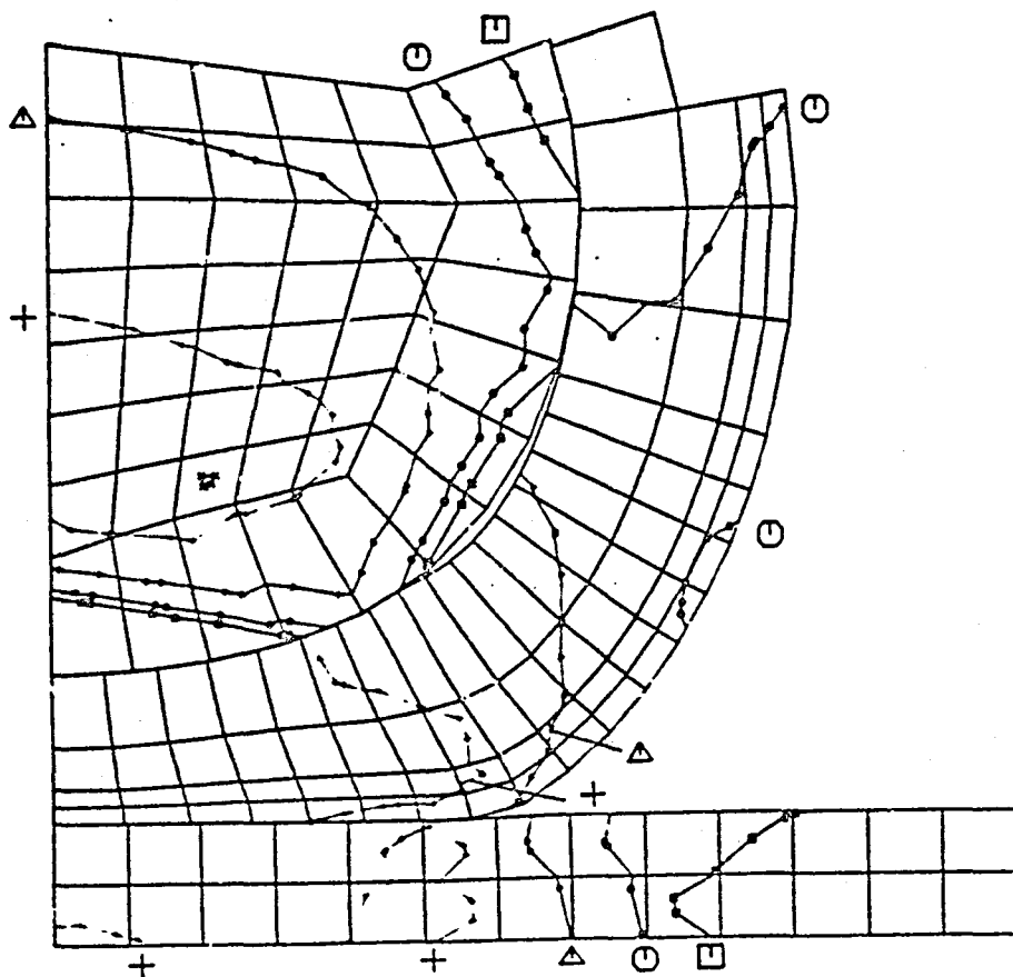
FIGURE 5-14. CONTOURS OF VON MISES STRESS AFTER 1 ms OF IMPACT (152 m/s INITIAL VELOCITY)
