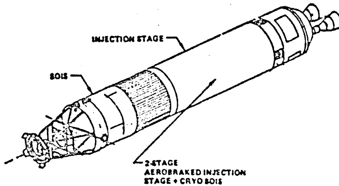
FIGURE 3-9. REFERENCE OTV/SOIS/WASTE PAYLOAD CONFIGURATION
