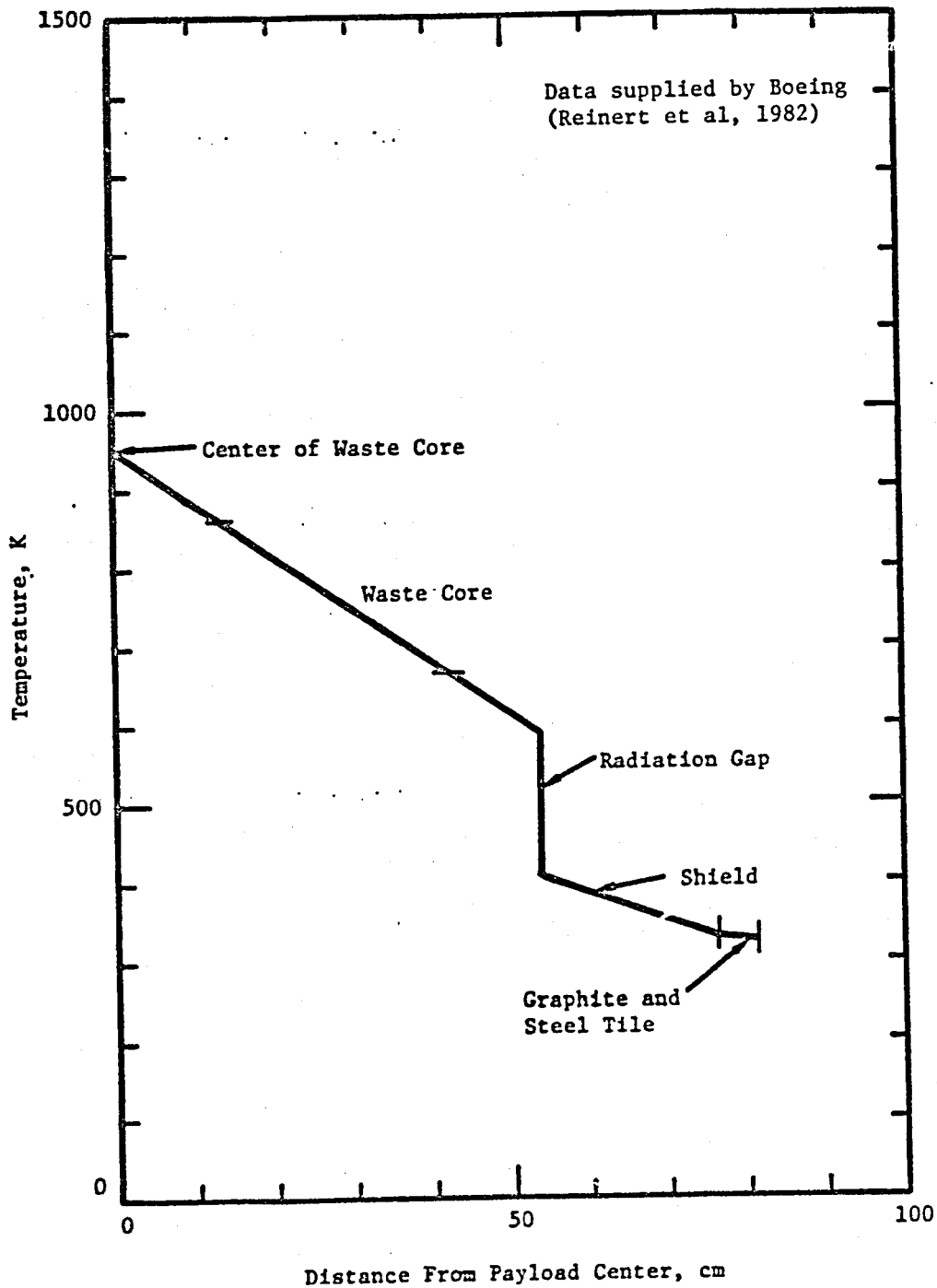
FIGURE 5-7. ON-ORBIT STEADY-STATE PRE-REENTRY TEMPERATURE CONDITION
