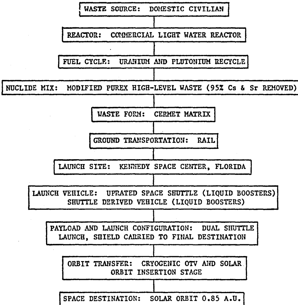
FIGURE 3-1. OVERVIEW OF REFERENCE CONCEPT FOR INITIAL NUCLEAR WASTE DISPOSAL IN SPACE
