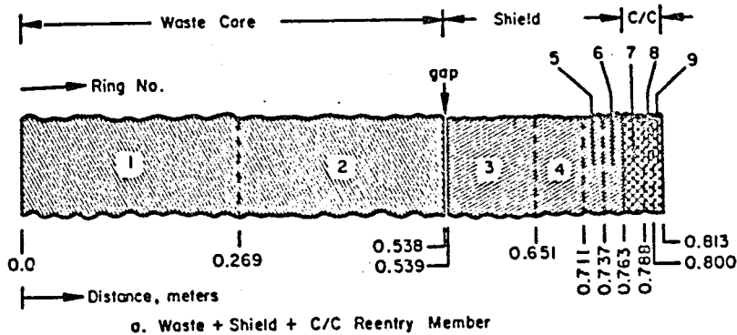
FIGURE 5-5. INTERNAL NODAL STRUCTURE USED TO MODEL THE TRANSIENT HEATING RESPONSE OF VARIOUS WASTE FORM MATERIAL CONFIGURATIONS
