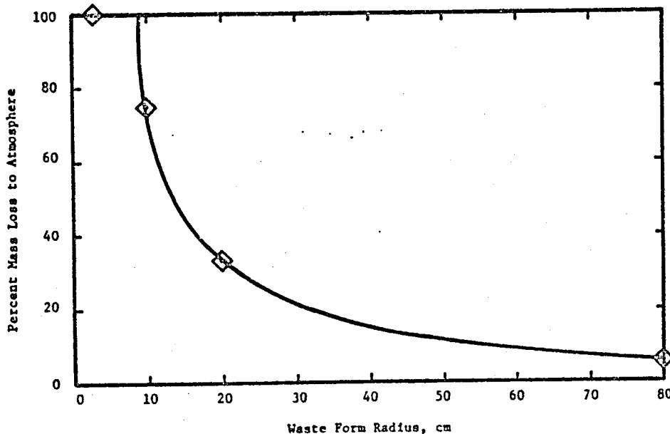
FIGURE 5-8. PERCENT WASTE FORM MASS LOSS FOR UNPROTECTED WASTE FORM AS A FUNCTION OF RADIUS
