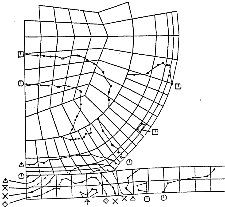
FIGURE H-1. CONTOURS OF VON MISES STRESS AFTER 0.25 ms OF IMPACT (442 m/s IMPACT VELOCITY)
