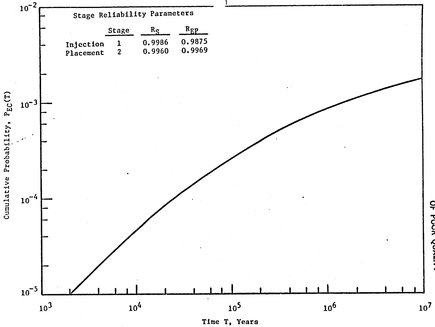
FIGURE 5-16. EARTH REENTRY PROBABILITY DISTRIBUTION FOR A SINGLE PAYLOAD LAUNCH WITHOUT RESCUE ( N=0 ); REDUCE SCALE BY 10^{-5} FOR RESCUE ( R_R=0.944 , N=4 )
