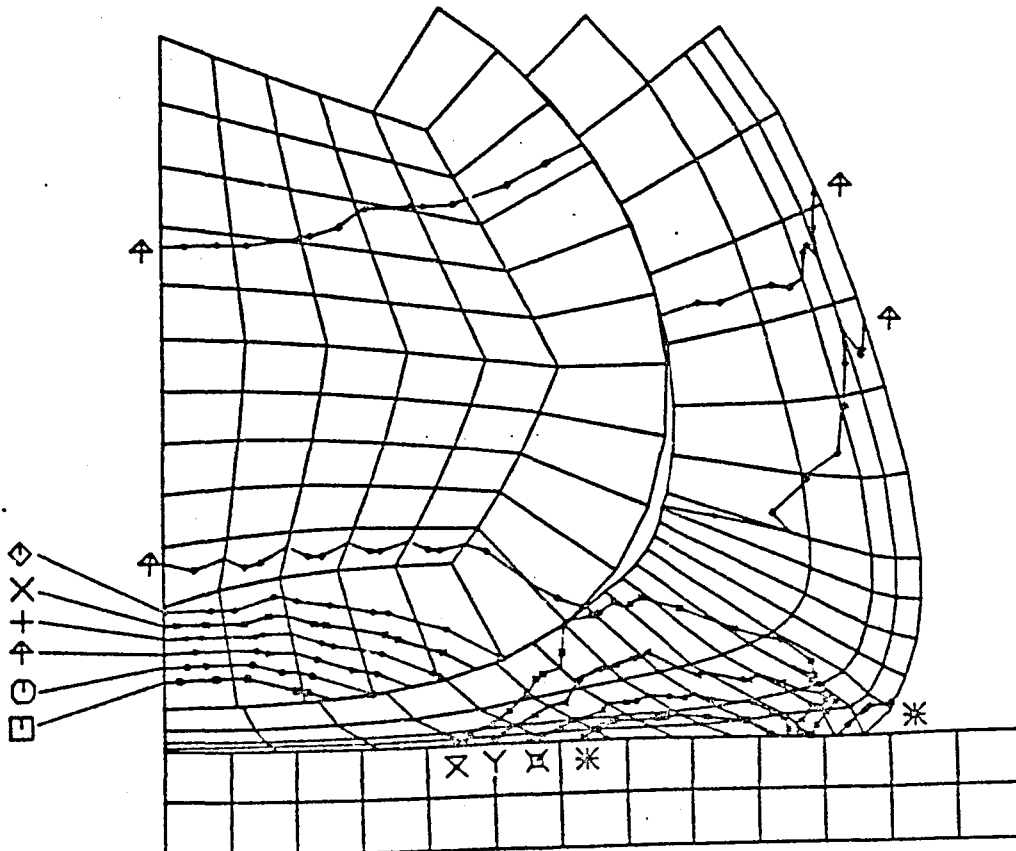
FIGURE 5-12. CONTOURS OF HOOP STRESS AFTER 1 ms OF IMPACT (442 m/s INITIAL VELOCITY FIGURE)
