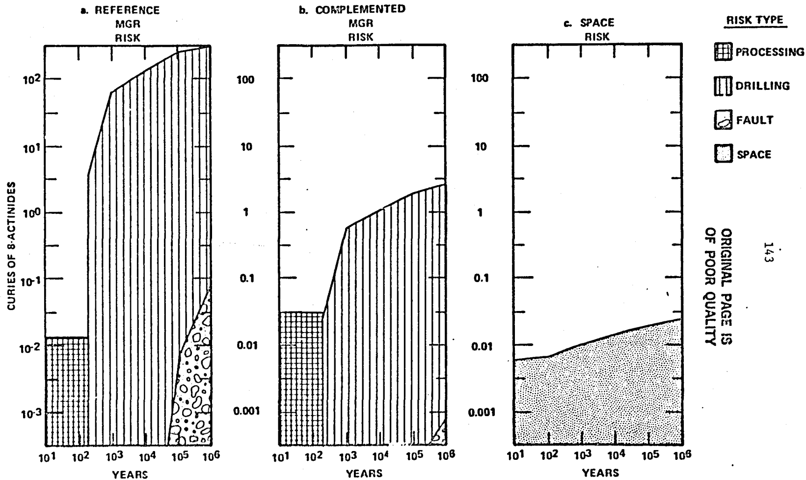
FIGURE 7-2. INTEGRATED EXPECTED CUMULATIVE RELEASE RISK COMPARISONS (IN CURIE SUM OF EIGHT EPA ACTINIDES) FOR HLW DISPOSAL IN SPACE
