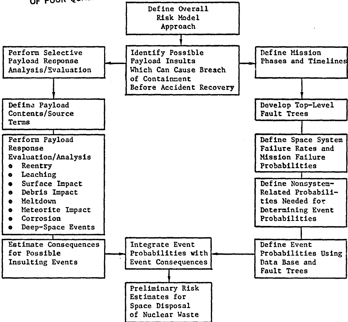
FIGURE 5-1. APPROACH FOR ESTIMATING SPACE DISPOSAL RISK
