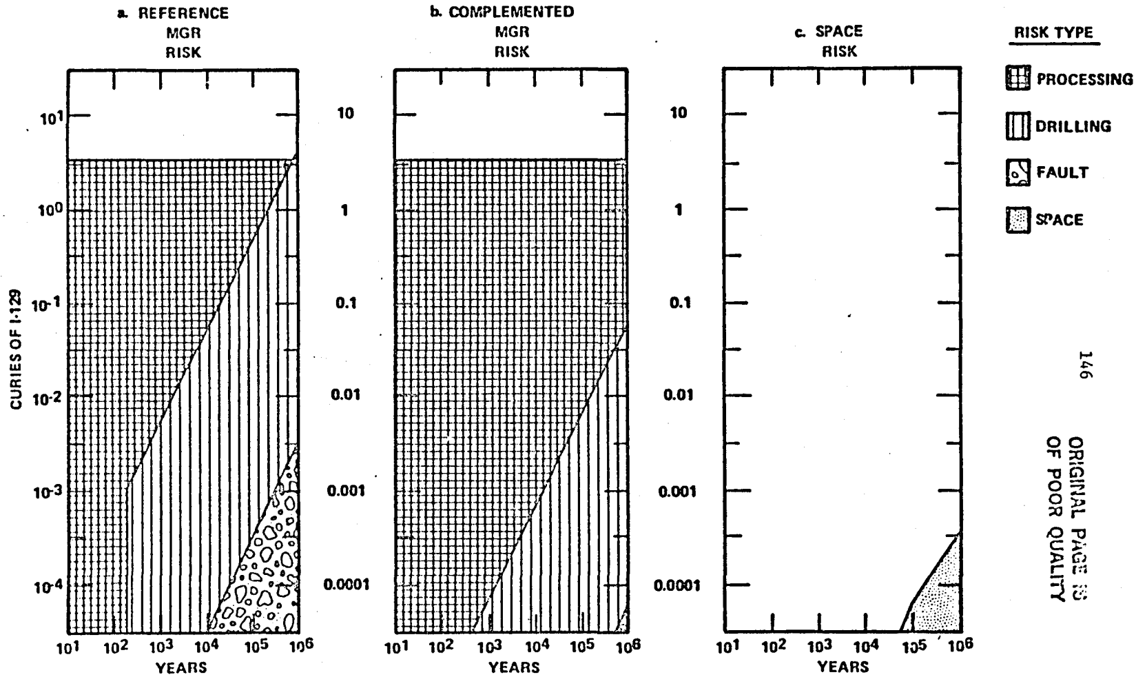
FIGURE 7-4. INTEGRATED EXPECTED CUMULATIVE RELEASE RISK COMPARISONS (IN CURIES OF I-129) FOR I-129 DISPOSAL IN SPACE
