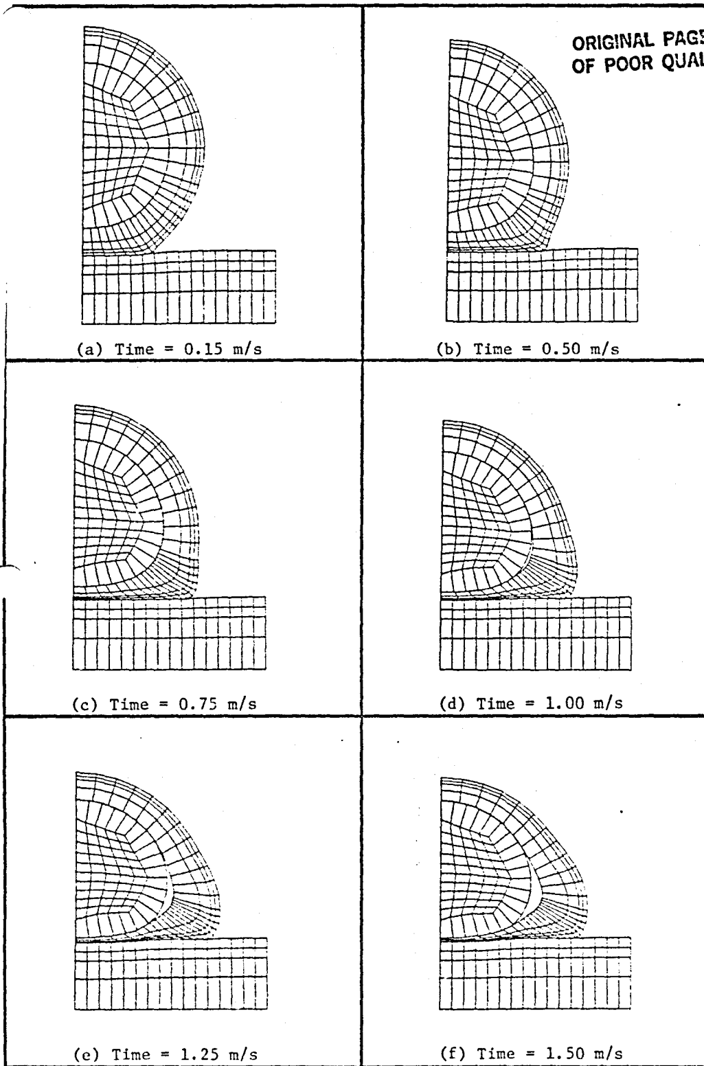
FIGURE 5-10. DEFORMED SHAPE OF THE SHIELDED WASTE PAYLOAD FOR VARIOUS TIMES DURING IMPACT (442 m/s INITIAL VELOCITY)
