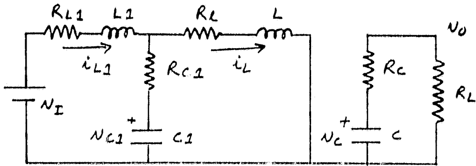
Fig. 5.12. Boost converter power stage model during T_{ON} .
