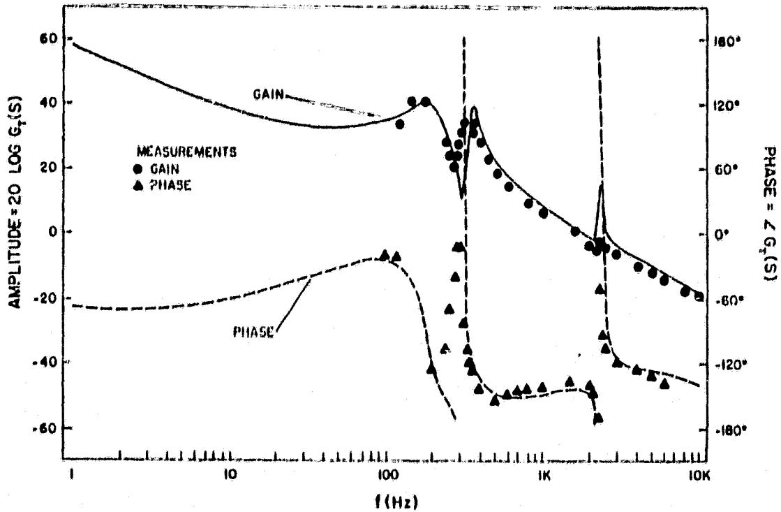
Fig. 2.7. Open loop gain and phase characteristics without the input filter damping resistance R_D .
