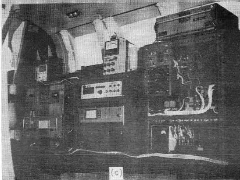
Figure 1.- (a) In situ aircraft; (b) nose probes; (c) instrumentation within main cargo area; and (d) forward compartment instrumentation.
