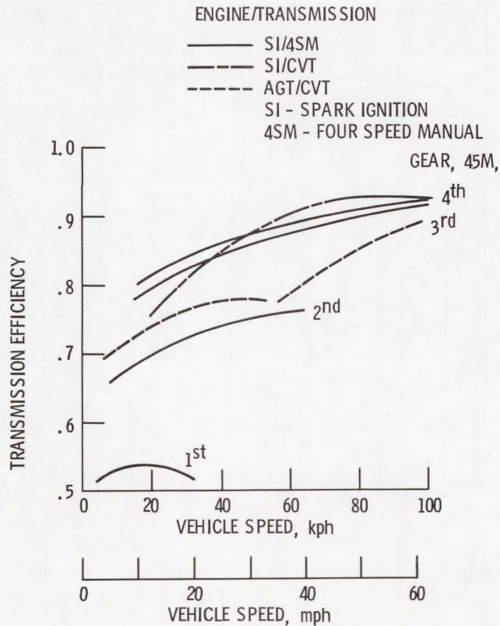
Figure 8. - Transmission efficiency comparisons: constant vehicle speed, Vehicle inertia mass, 964 kg (2125 lb); engine rated power, 37 kW (50 hp); vehicle C_D , 0.39.
