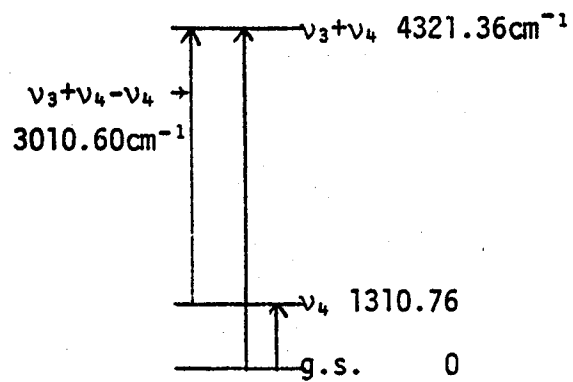
Figure 11. Hot bands like \nu_3 + \nu_4 - \nu_4 are transitions between two excited vibrational states, \nu_3 + \nu_4 and \nu_4 .
