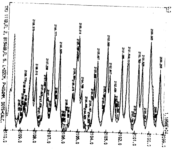
Figure 2. Comparisons of synthetic (broken line) and experimental (solid line) PH 3 spectra in the 2100 cm -1 region. See text for details.
