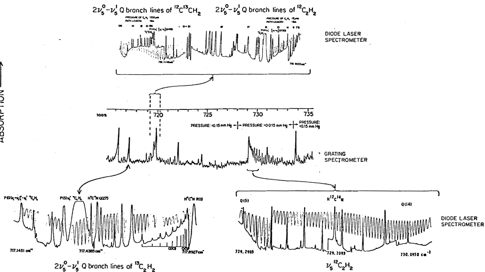
Figure 8. Diode laser spectra of acetylene near the center of the \nu_5 band (J. Mol. Spectrosc. 84, 313 (1980)).
