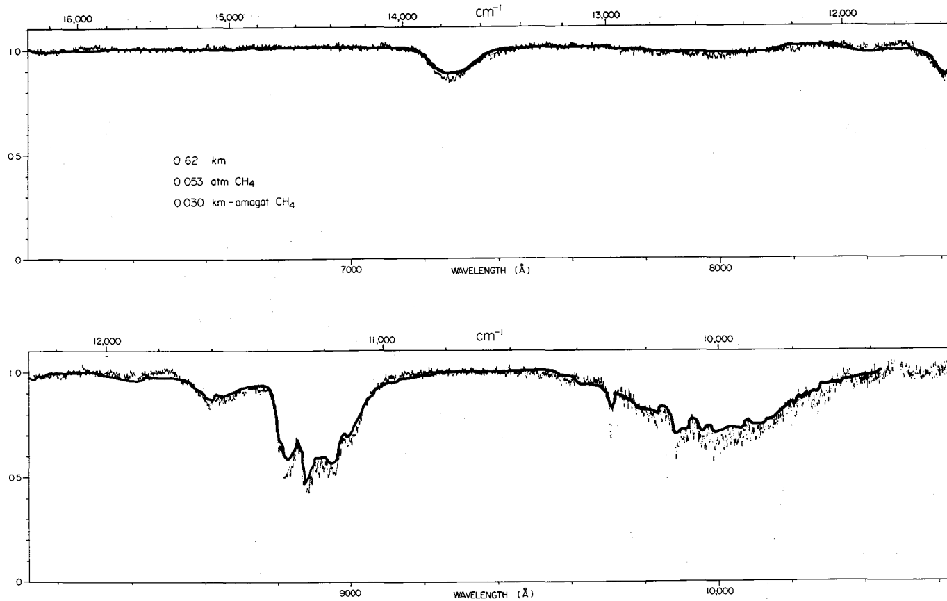
Figure 3. Comparison between experimental CH 4 absorption and fitted spectrum (heavy line) using the random-band model.
