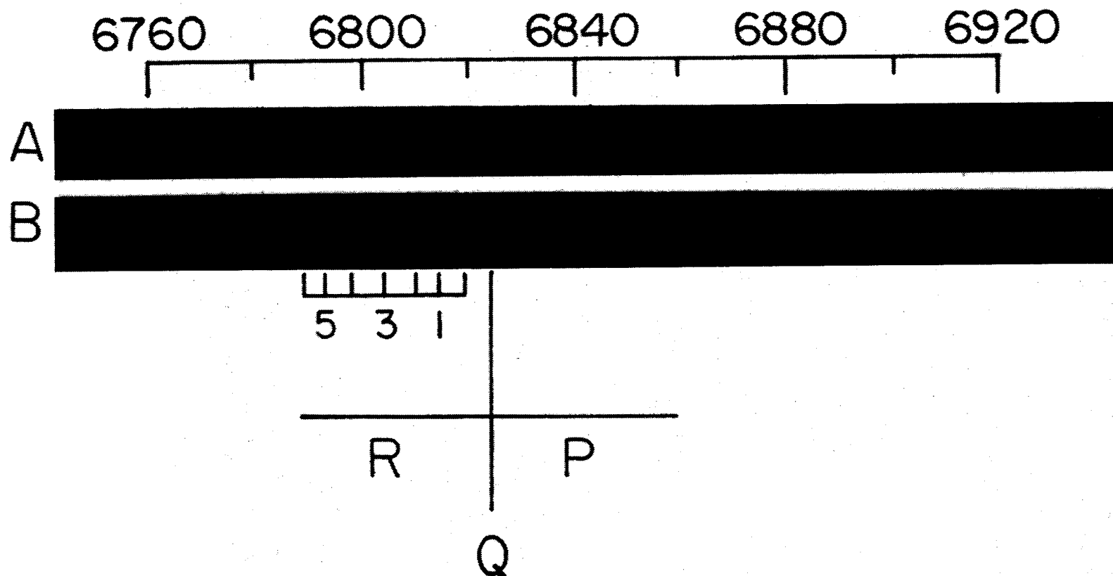
Figure 2. The spectrum of Jupiter (A) and Uranus (B) in the region of the 6825-A feature of methane. Taken from Owen (1966).
