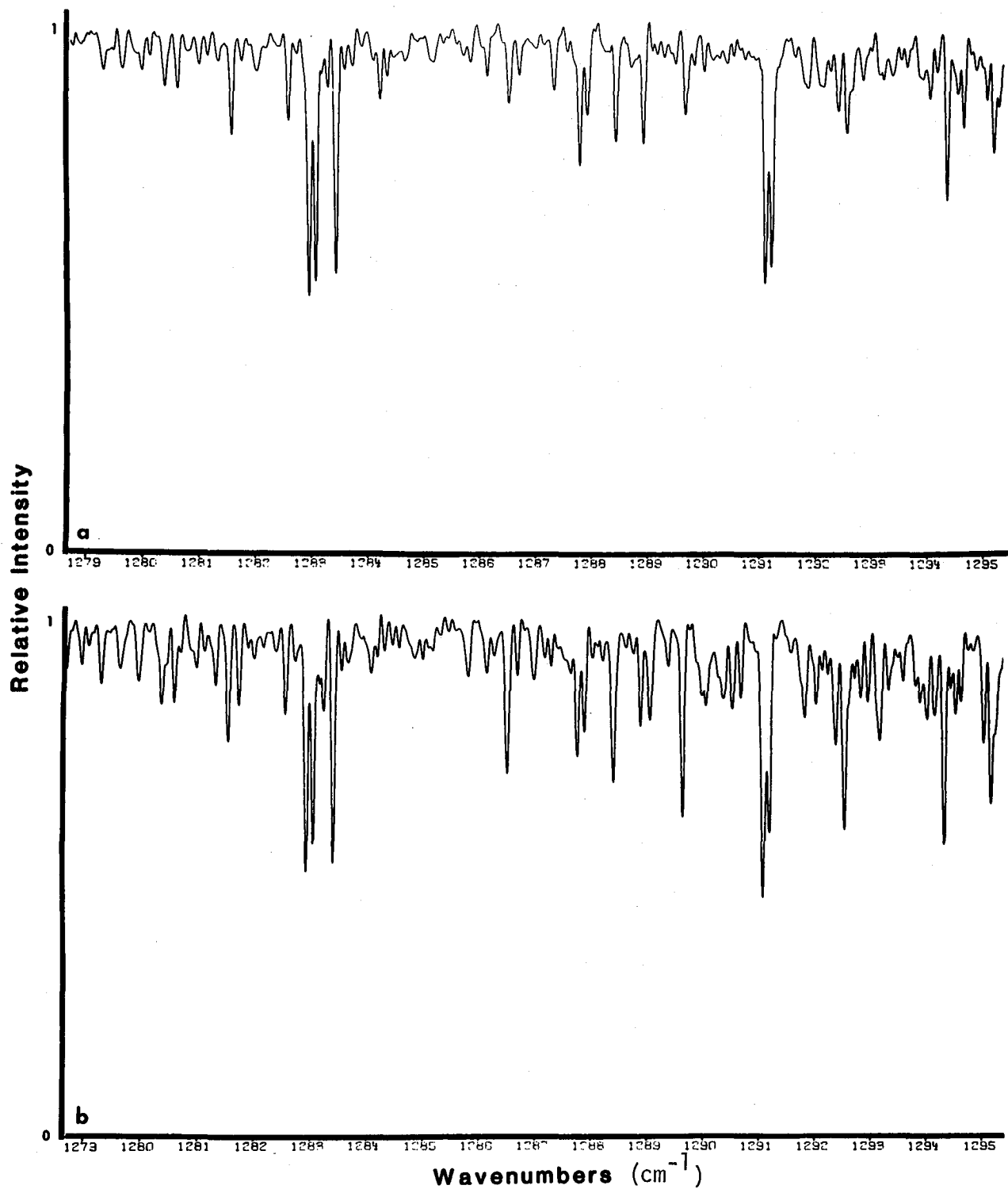
Figure 1. Spectrum of 3.4 cm-am of CH 3 D at (a) 206 K and (b) 295 K, obtained at NASA – Ames Research Center.
