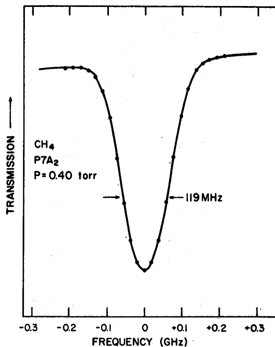
A sample spectrum of the P7A_2 line whose peak is at 1263.33 \text{ cm}^{-1} in the \nu_4 band of \text{CH}_4 . The experimental conditions were p = 0.40 \text{ Torr} , l = 10 \text{ cm} , and T = 296.9 \text{ K} . The Gaussian fit, indicated by black dots, yielded an experimental line width of 119 \text{ MHz} .
