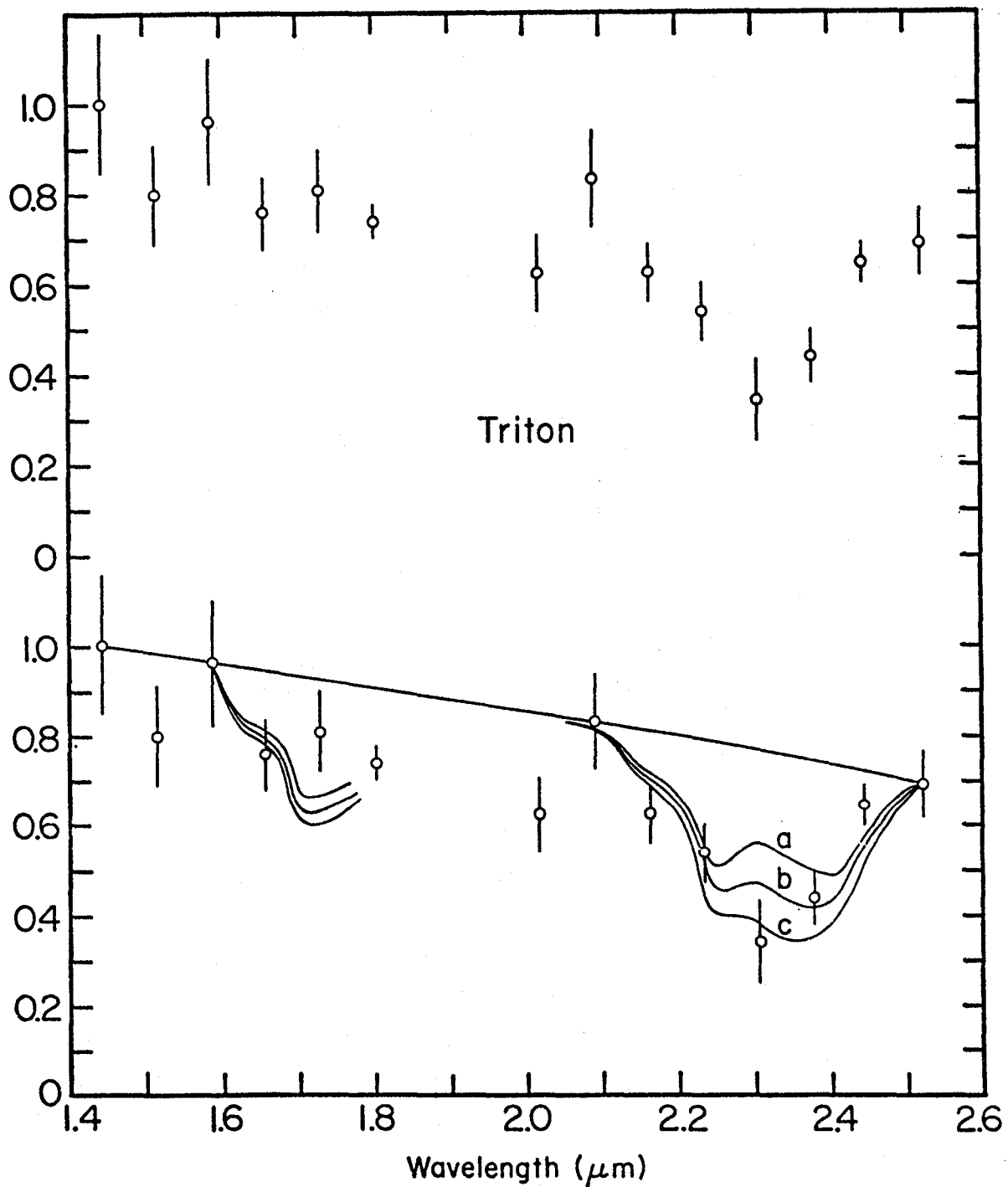
Figure 2. Infrared spectrophotometry of Triton (4). The data are shown twice. At the bottom, synthetic methane gas spectra are superimposed to show the quality of the fit in the 2.3 \mu\text{m} absorption band. Spectrum b represents the best fit to the measured width (EW) of the band in the spectrum of Triton, and spectra a and c have EW corresponding to the error bars on the EW of the Triton spectrum.
