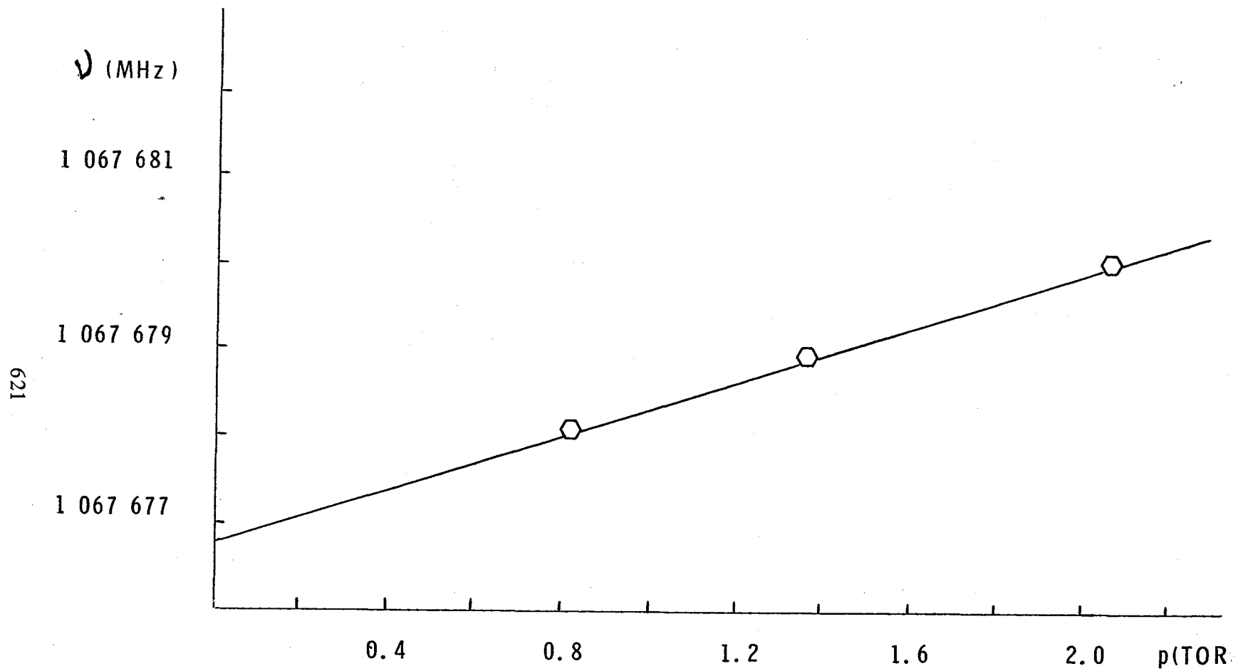
Figure 6. Dependence of the frequency of the (2,2) inversion transition of ^{14}\text{NH}_3 in the \nu_2 state on the pressure of ammonia gas (J. Mol. Spectrosc. 84, 291 (1980)).
