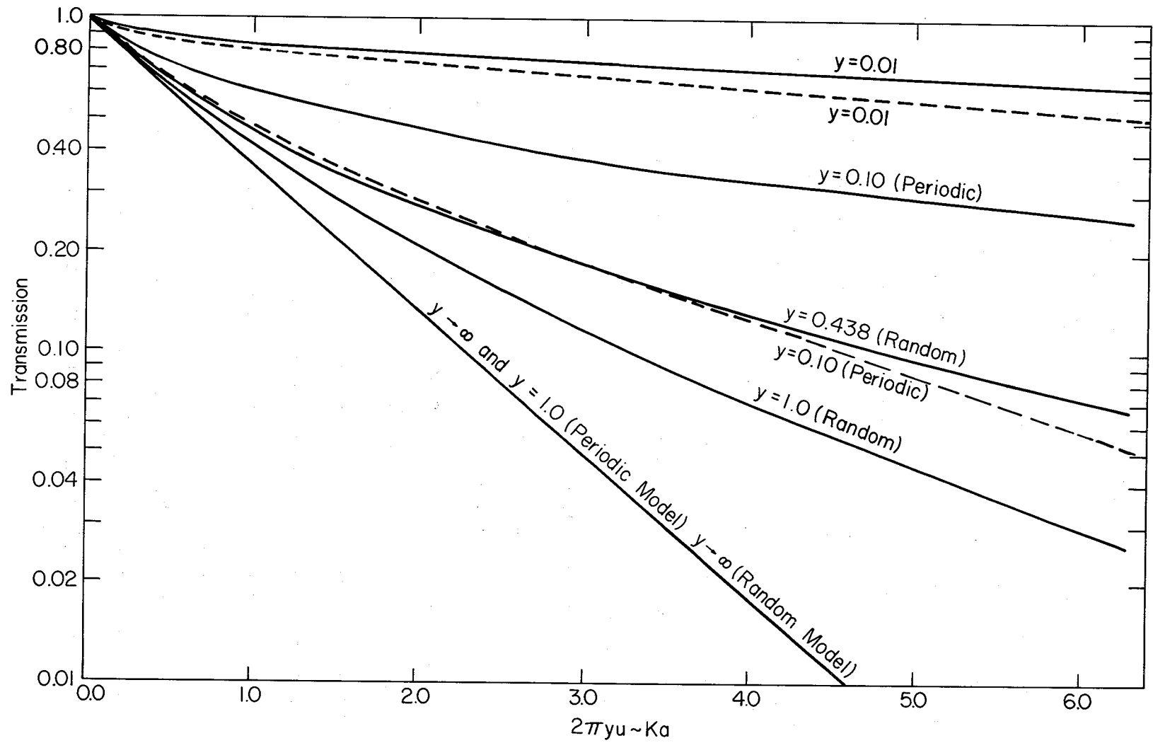
Figure 1. Behavior of the average transmission with K_p , Y_p , and a for the Elsasser (periodic) and Mayer-Goody (random) band models.
