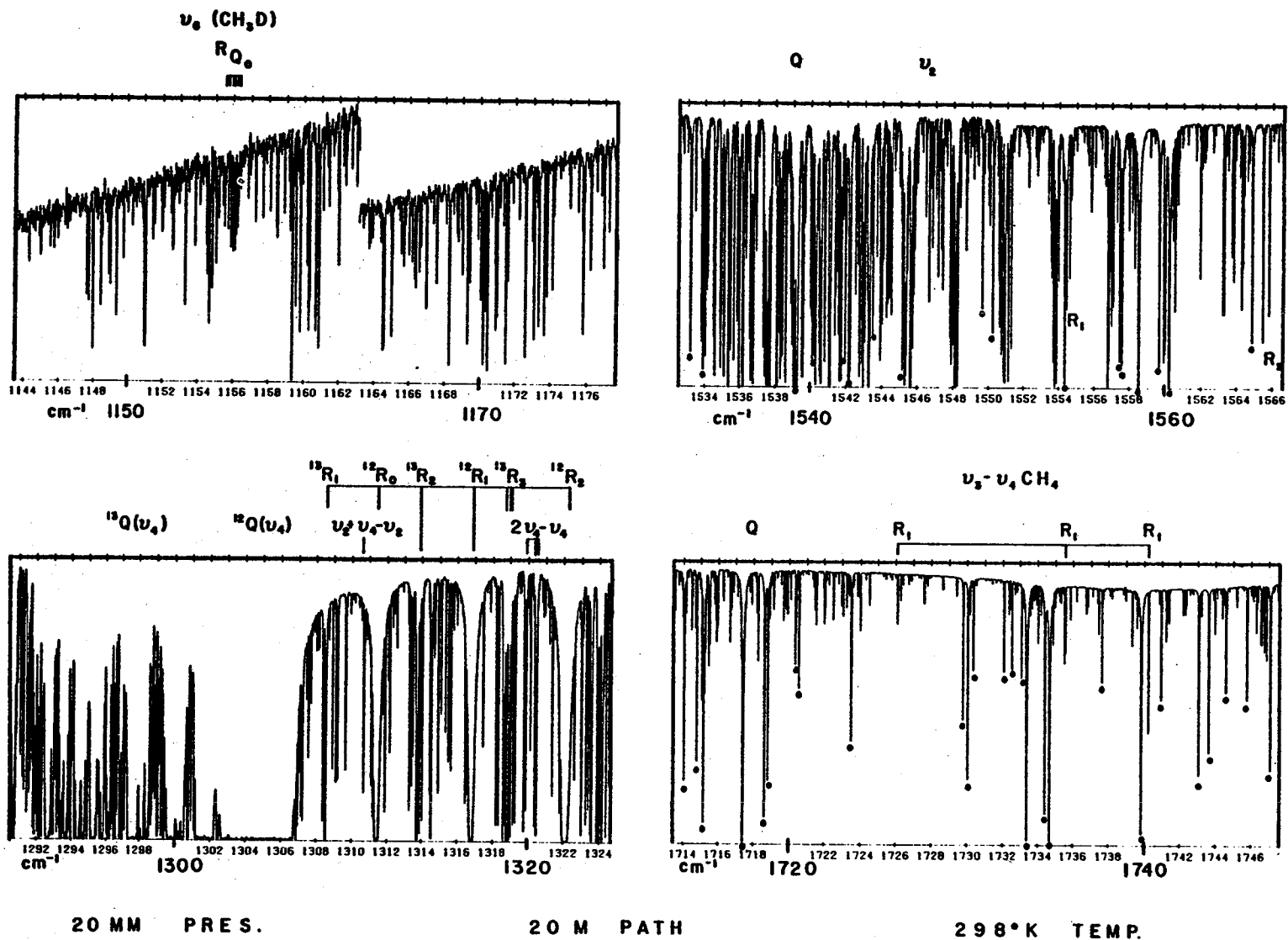
Figure 13. Portions of the methane FTS spectrum at high optical density in the 7\mu\text{m} region. The upper left panel indicates the strength of \text{CH}_3\text{D} absorptions observed in isotopic abundance. The remaining panels show the density of lines arising from \nu_4 , \nu_2 , \nu_2 + \nu_4 - \nu_2 , 2\nu_4 - \nu_4 , \nu_3 - \nu_4 and other hot bands of both ^{12}\text{CH}_4 and ^{13}\text{CH}_4 .
