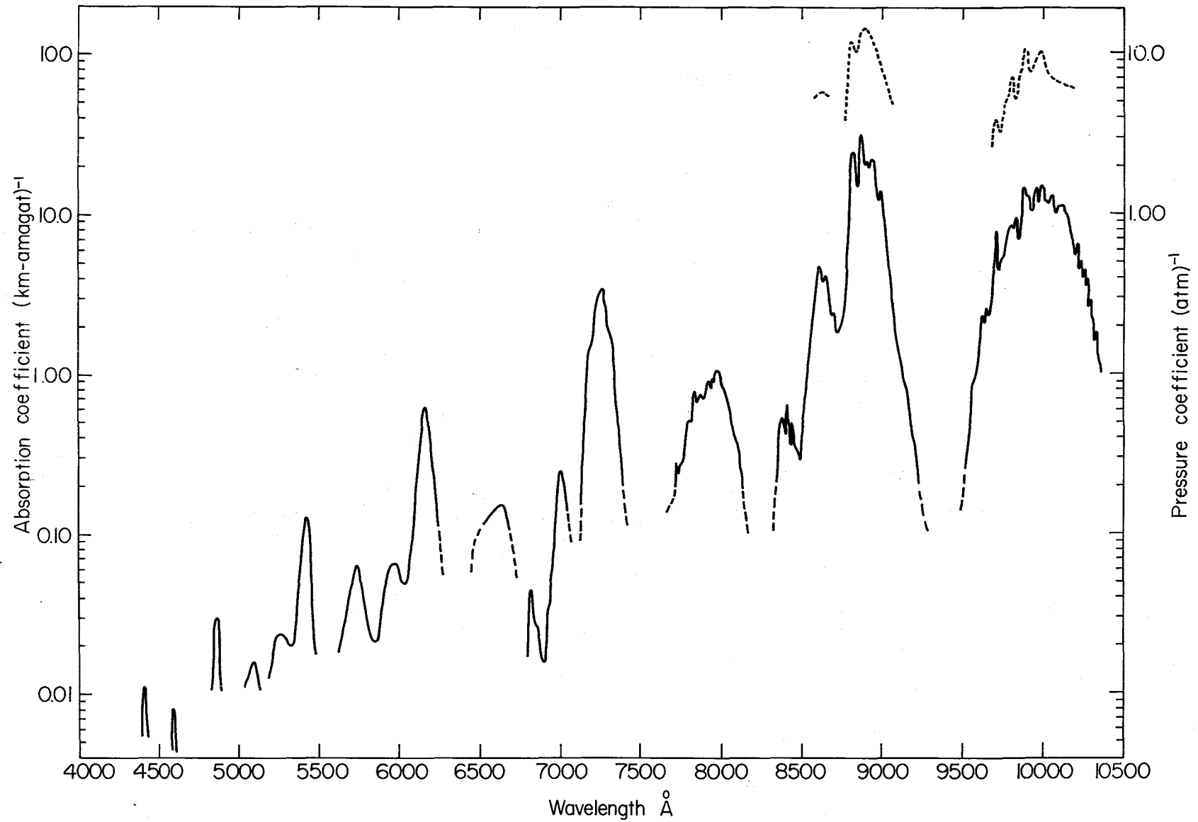
Figure 2. Absorption and pressure coefficients for CH 4 derived from the random band model and experimental results.
