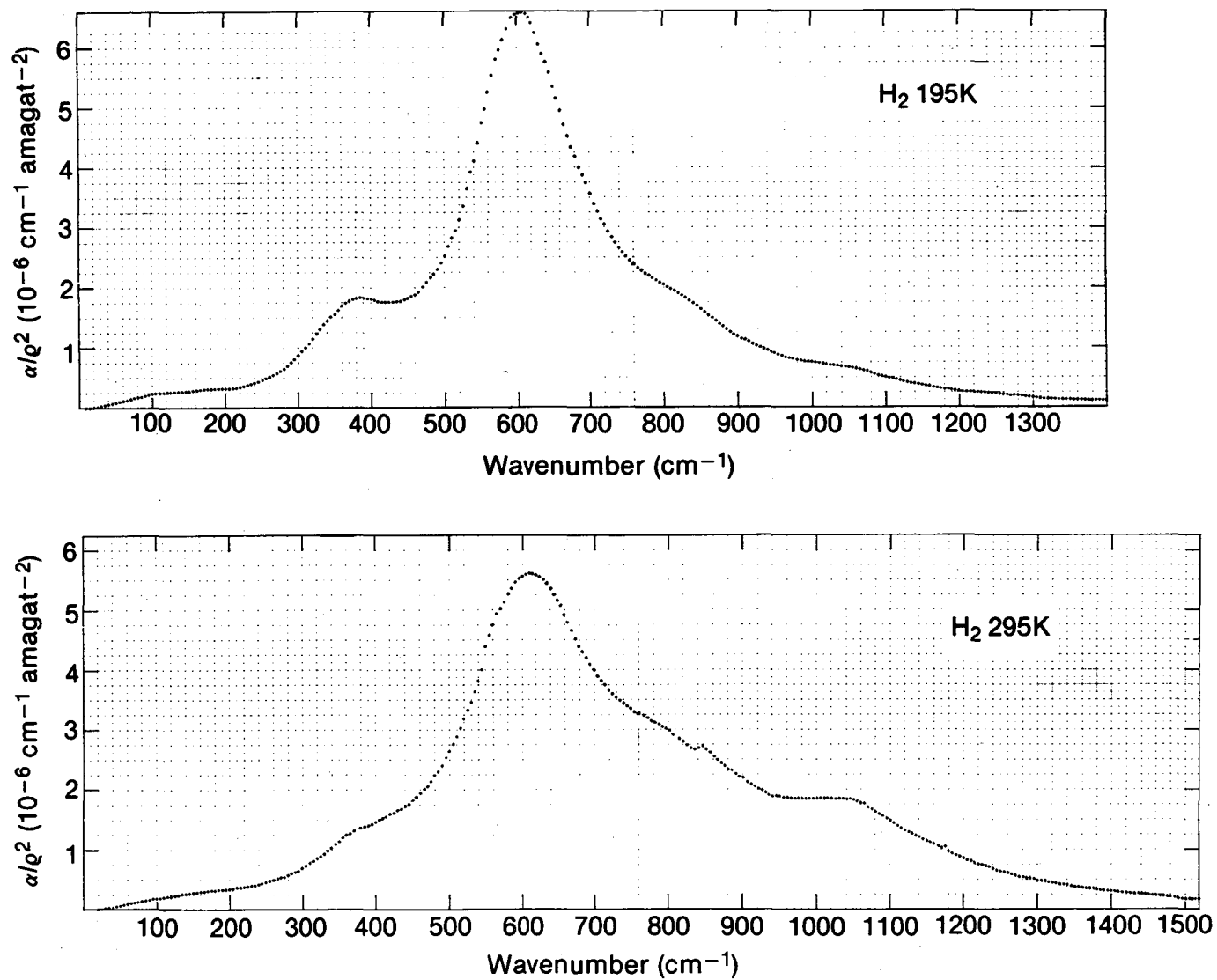
Figure 4. The translational-rotational spectrum of H 2 at 195 and 295K.
