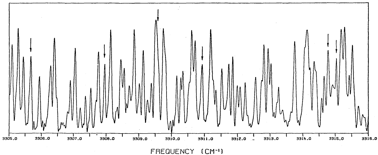
Figure 9. 0.04\text{ cm}^{-1} Fourier transform spectra of ^{14}\text{NH}_3 with a path length of about 300 m and ammonia pressure of a few microns. The arrows are forbidden transitions in the 2\nu_4 band of ^{14}\text{NH}_3 .
