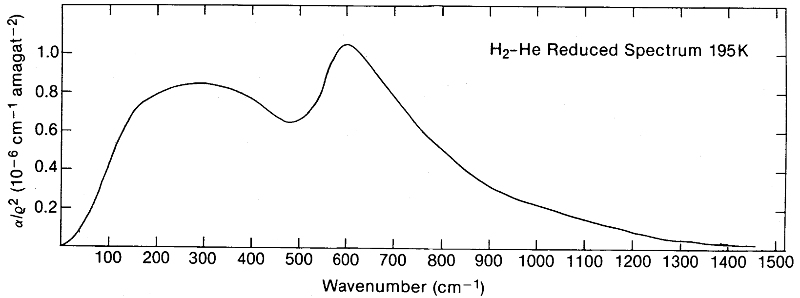
Figure 8. Translational-rotational spectrum due to H 2 -He collisions at 195K.
