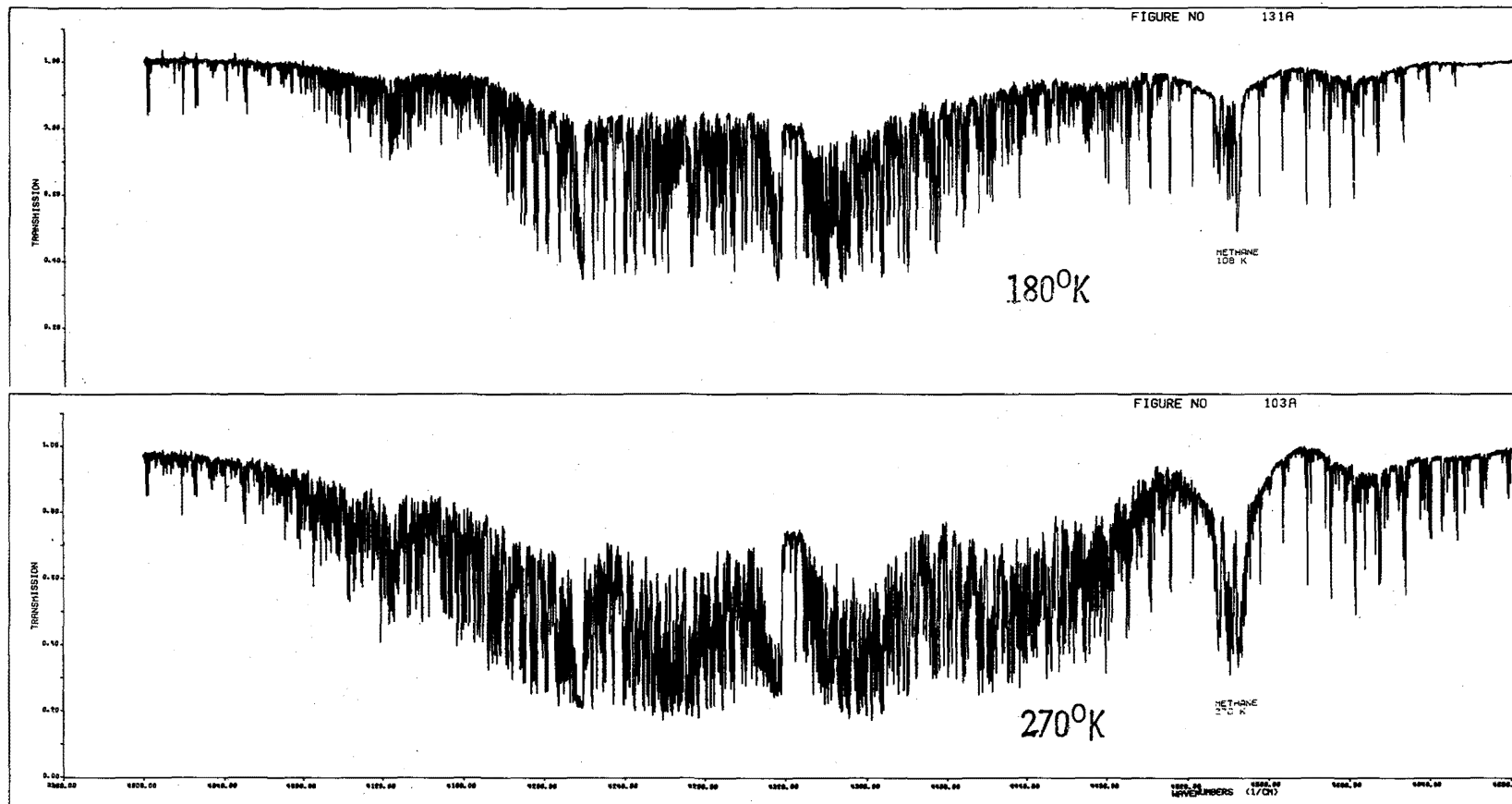
Figure 2. Methane spectra in the 4000 to 4600 \text{cm}^{-1} region.
