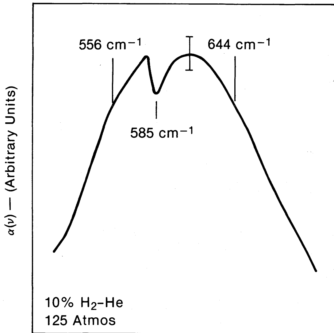
Figure 11. The S(1) line observed in a 10% H 2 -He mixture (125 atmos) at room temperature showing the intercollisional interference dip. Spectral resolution somewhat less than 10 \text{ cm}^{-1} . The data has been smoothed. The error bar indicated the fluctuation in the data.
