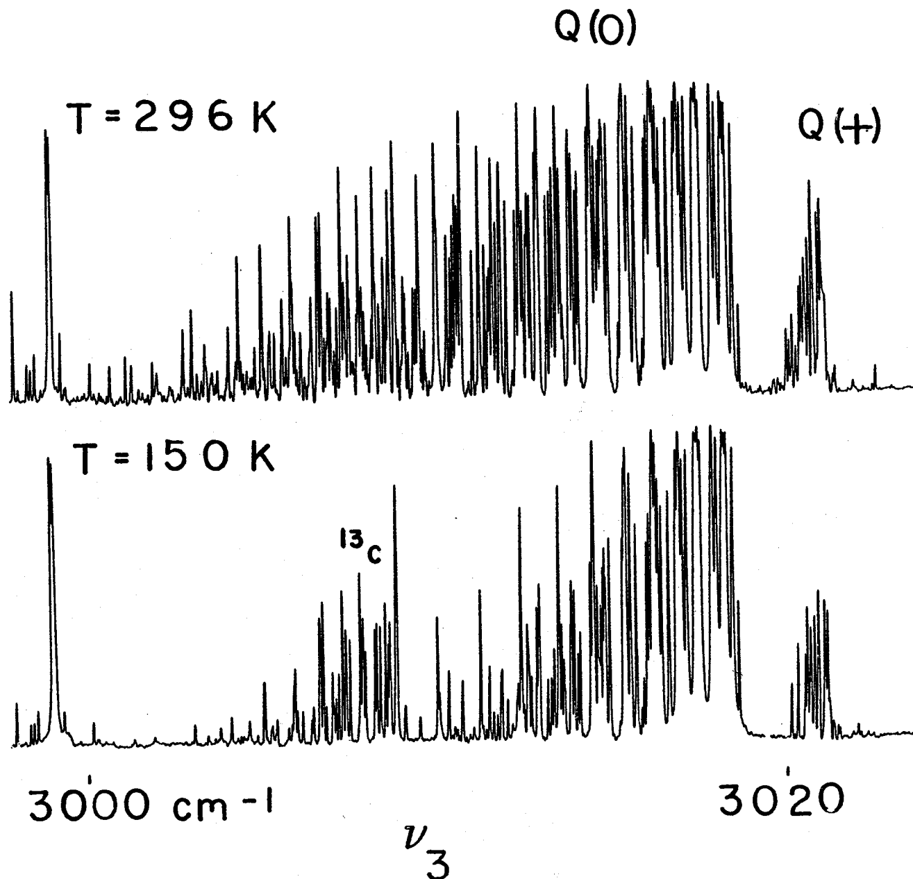
Figure 4. The spectrum of methane at 3000\text{ cm}^{-1} recorded at an intermediate optical density at 0.02\text{ cm}^{-1} resolution with the Florida State University grating spectrometer with the gas sample at 296\text{ K} and 150\text{ K} . The allowed Q(0) and forbidden Q(+) branches are indicated, as well as the ^{13}\text{CH}_4 Q branch, for the \nu_3 fundamental.
