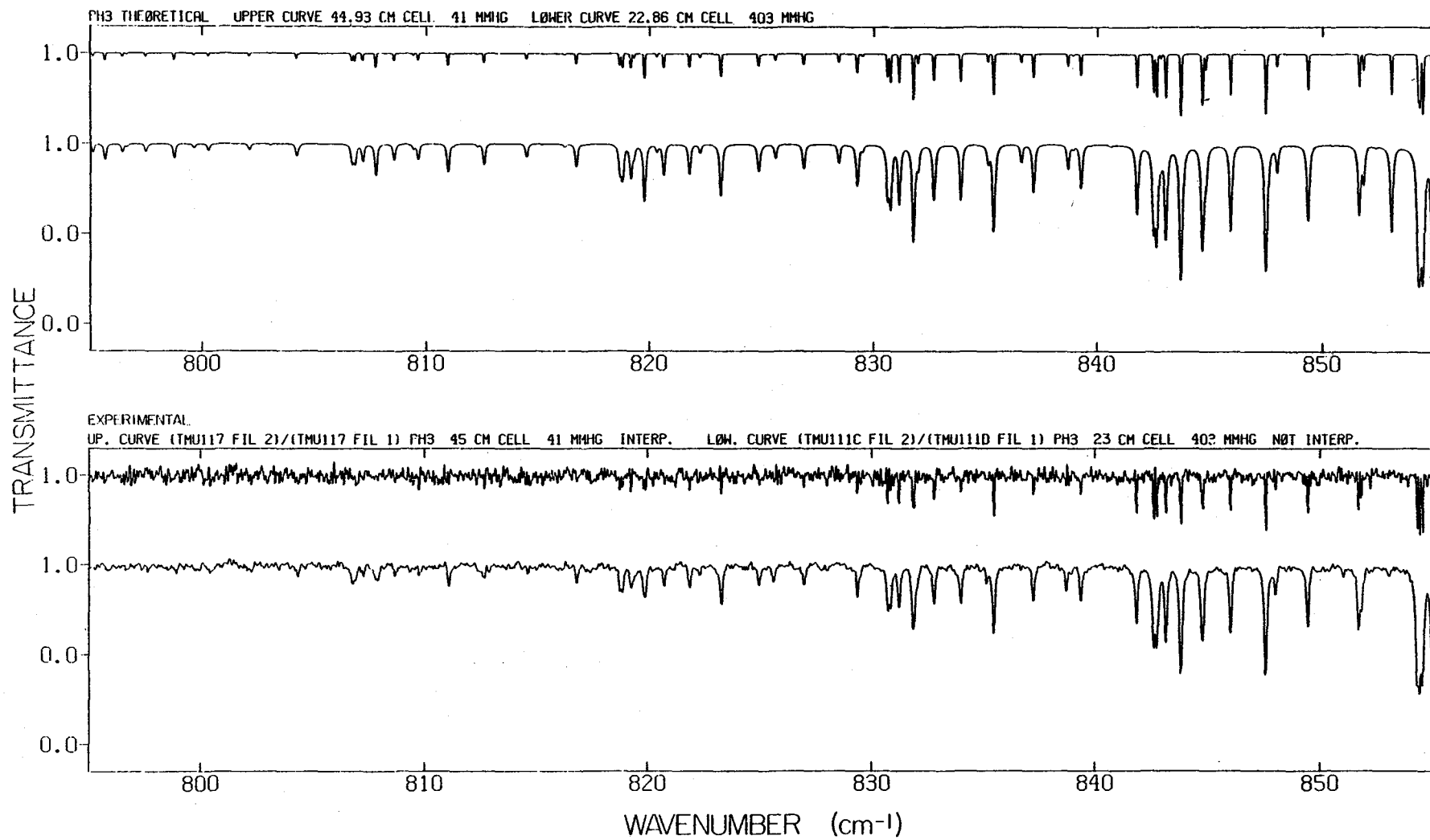
Figure 1. Calculated (upper 2 curves) and measured (lower 2 curves) transmittance of \text{PH}_3 at 25^\circ\text{C} . The zero lines and the 100% lines are shifted for clarity. See text for details.
