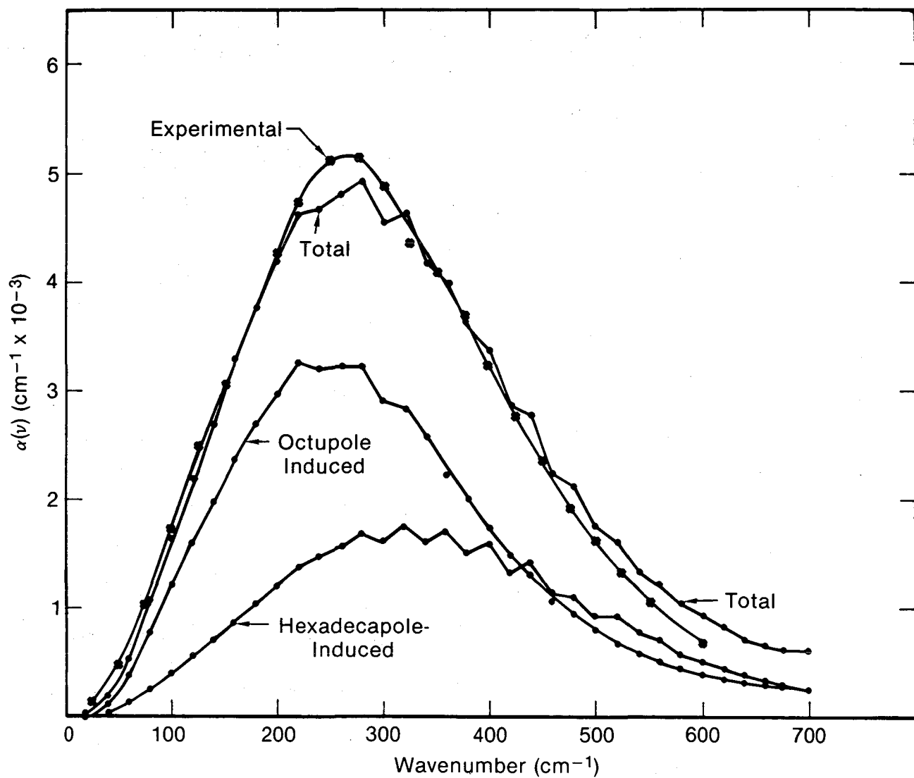
Figure 2. Comparison of experimental and theoretical (total) collision-induced spectrum of \text{CH}_4 at 296K, 24.1 amagats (from ref. 2). The separate octupole and hexadecapole induced contributions are shown.
