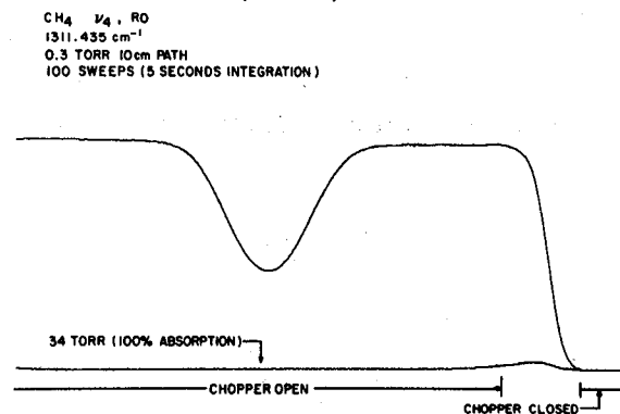
Line intensity data for R0 in \nu_4 of \text{CH}_4 . This spectrum was recorded in the sweep integration mode. The chopper reference generated a laser current modulation that was adjusted to sweep the absorption line during the open phase. A portion of the chopper-closed phase was also swept to provide a 0\% transmission reference. This reference was checked with a subsequent scan of the saturated line.
