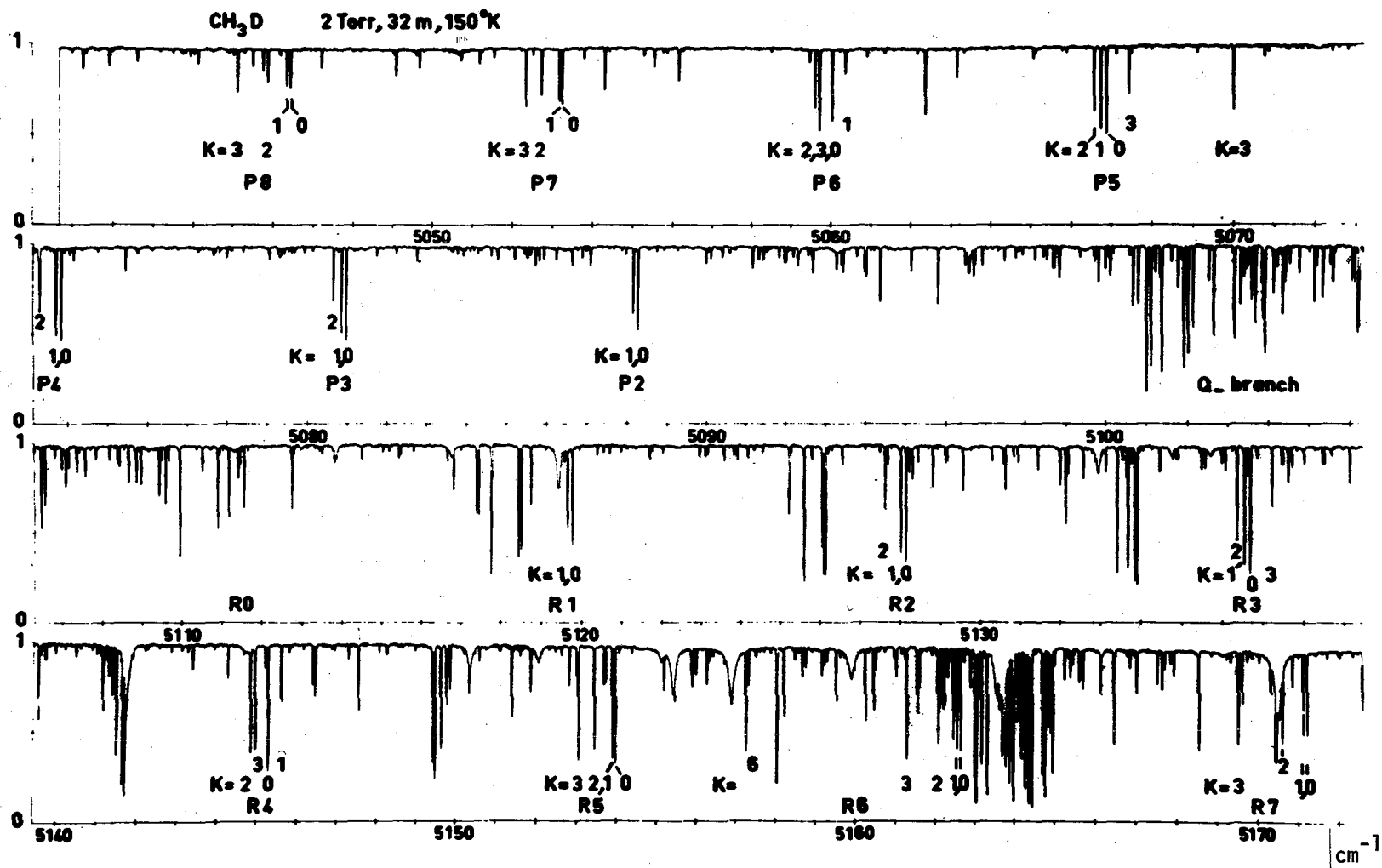
Figure 6. The 5105 cm -1 band of CH 3 D obtained at the Observatoire de Meudon.
