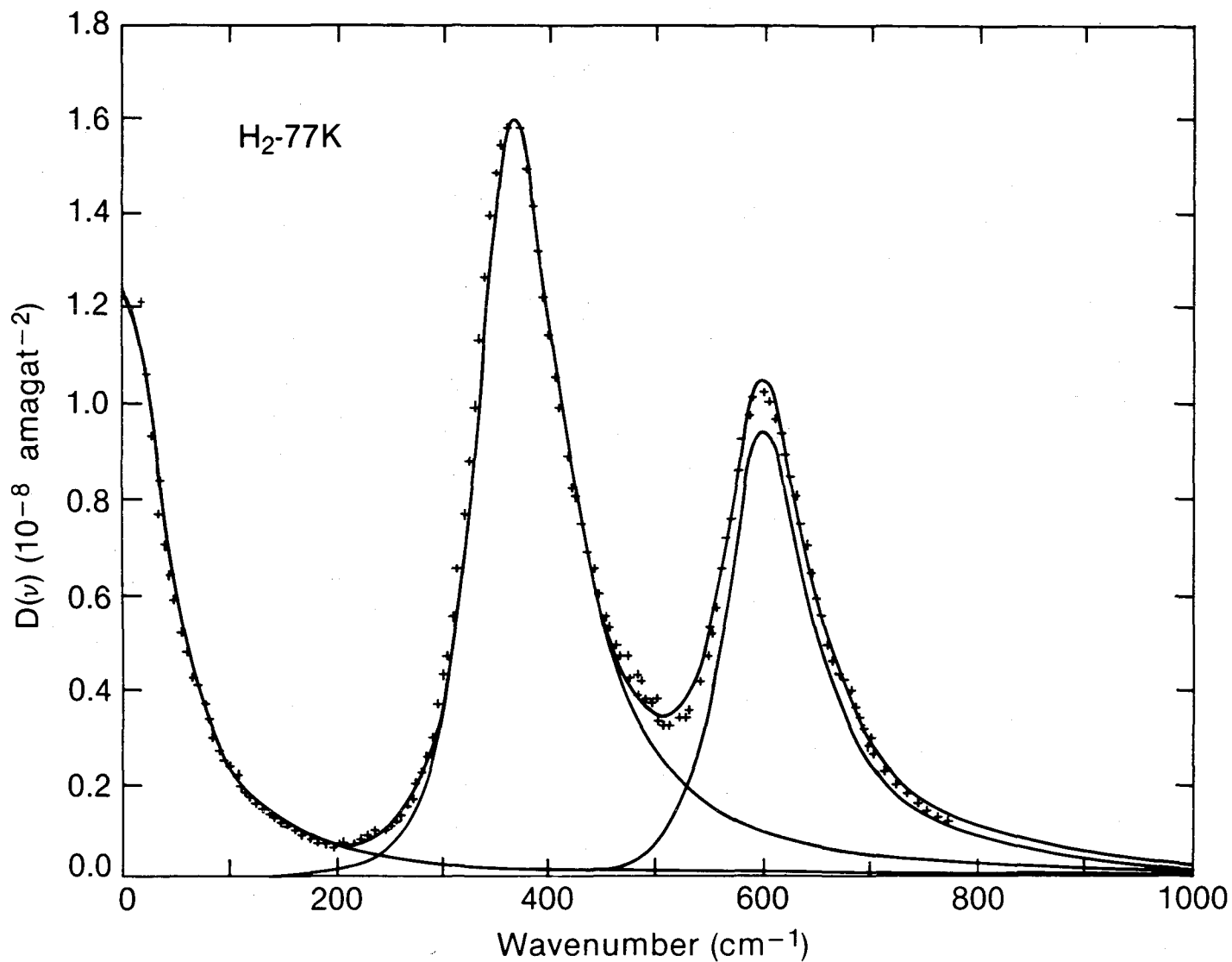
Figure 10. Three parameters fit obtained by adjusting an amplitude parameter and two time parameters (defined in ref. 5) to the spectrum of H 2 at 77K (ref. 4). The total spectrum as well as the translational and rotational components are shown.
