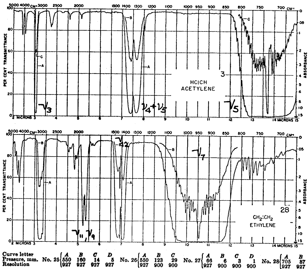
Figure 3. Laboratory infrared spectra of \text{C}_2\text{H}_2 and \text{C}_2\text{H}_4 . (From Pierson, 1956).
