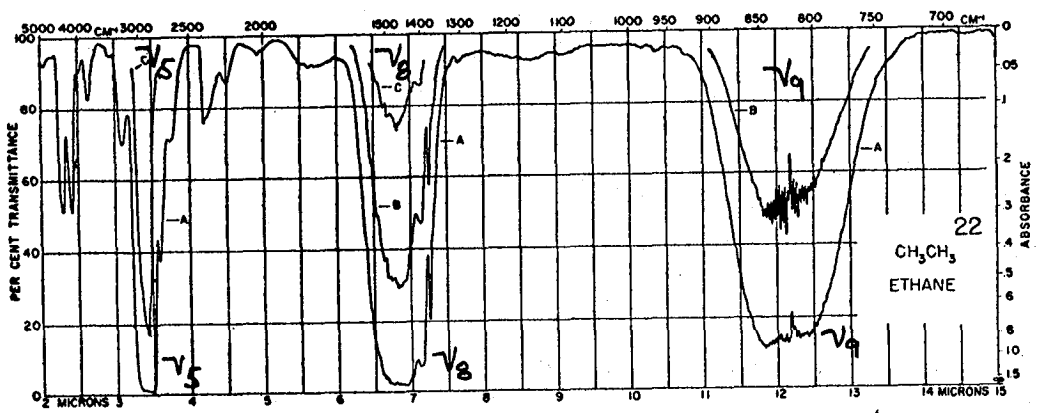
Figure 4. Laboratory infrared spectra of CH 4 and C 2 H 6 . (From Pierson, 1956).
