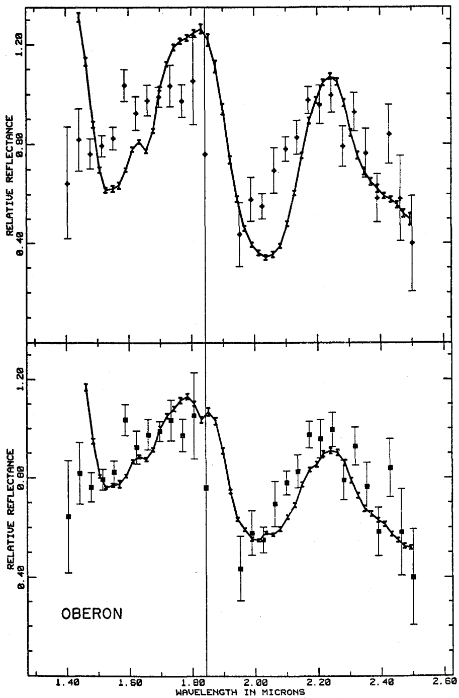
Figure 3. Infrared spectrophotometry of Oberon, showing the quality of data that can now be obtained for Triton and Pluto as well. The solid line in the top of the figure is the spectrum of Saturn's rings (known to consist of H_2O frost), and the solid line in the lower part is the spectrum of Ganymede (also known to contain H_2O frost). The Oberon data are normalized to each of the two comparison objects. The fit is best for the spectrum of Ganymede.
