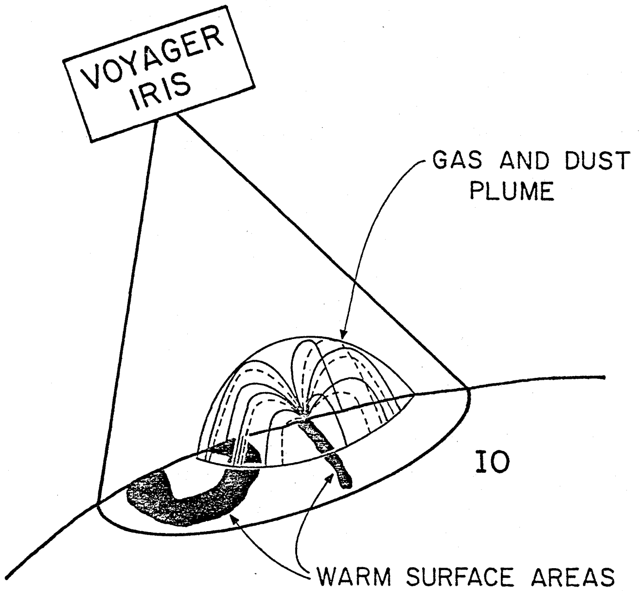
Figure 6. IRIS observations of LIKI hot spot (schematic).
