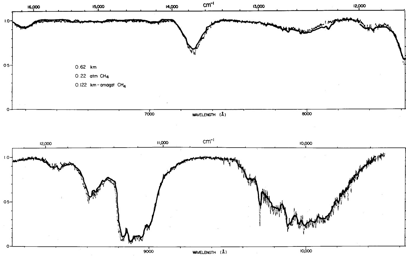
Figure 4. Similar comparison of experimental and modelled results, but with higher density of CH 4 .
