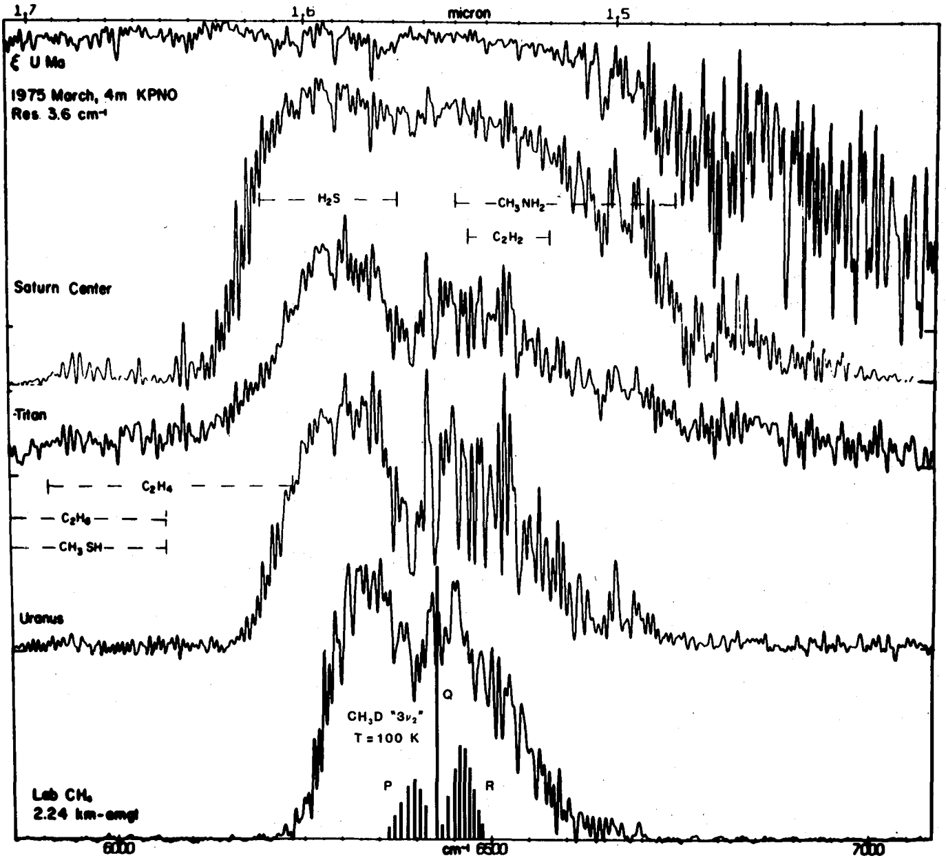
Figure 7. The 6425 \text{ cm}^{-1} band of \text{CH}_3\text{D} superimposed on the planetary spectra of Fink and Larson (1979). Relative intensities calculated for 100 K and smeared to match the planetary resolution.
