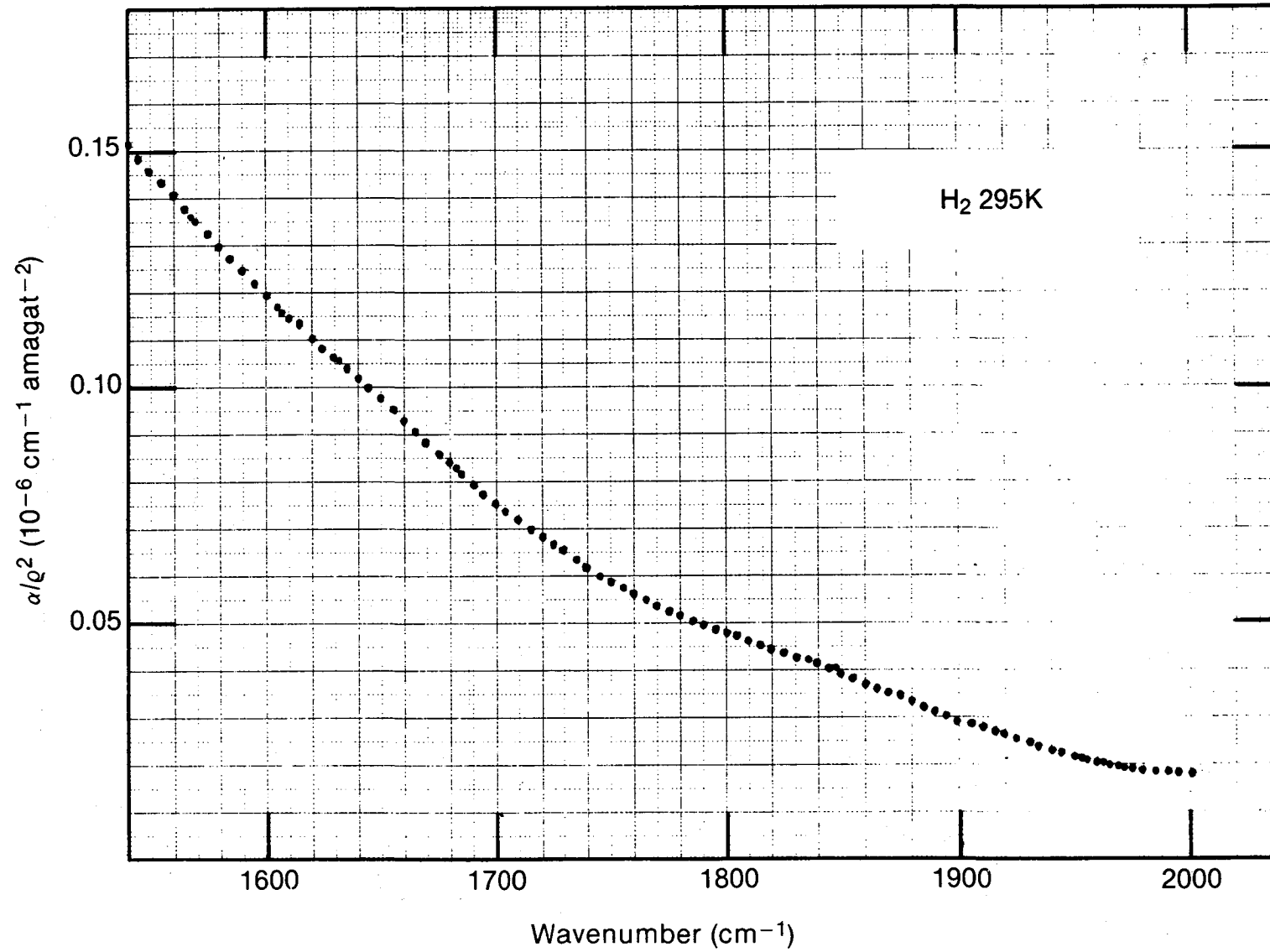
Figure 6. High frequency absorption in H 2 at 295K from 1540 to 2000 \text{cm}^{-1} .
