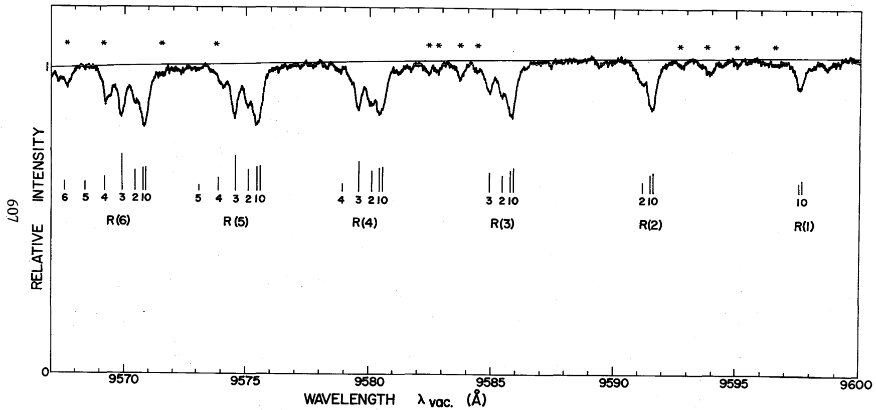
Figure 4. Intensity tracing of the 9613 Å band of CH 3 D obtained at NASA-Ames Research Center.
