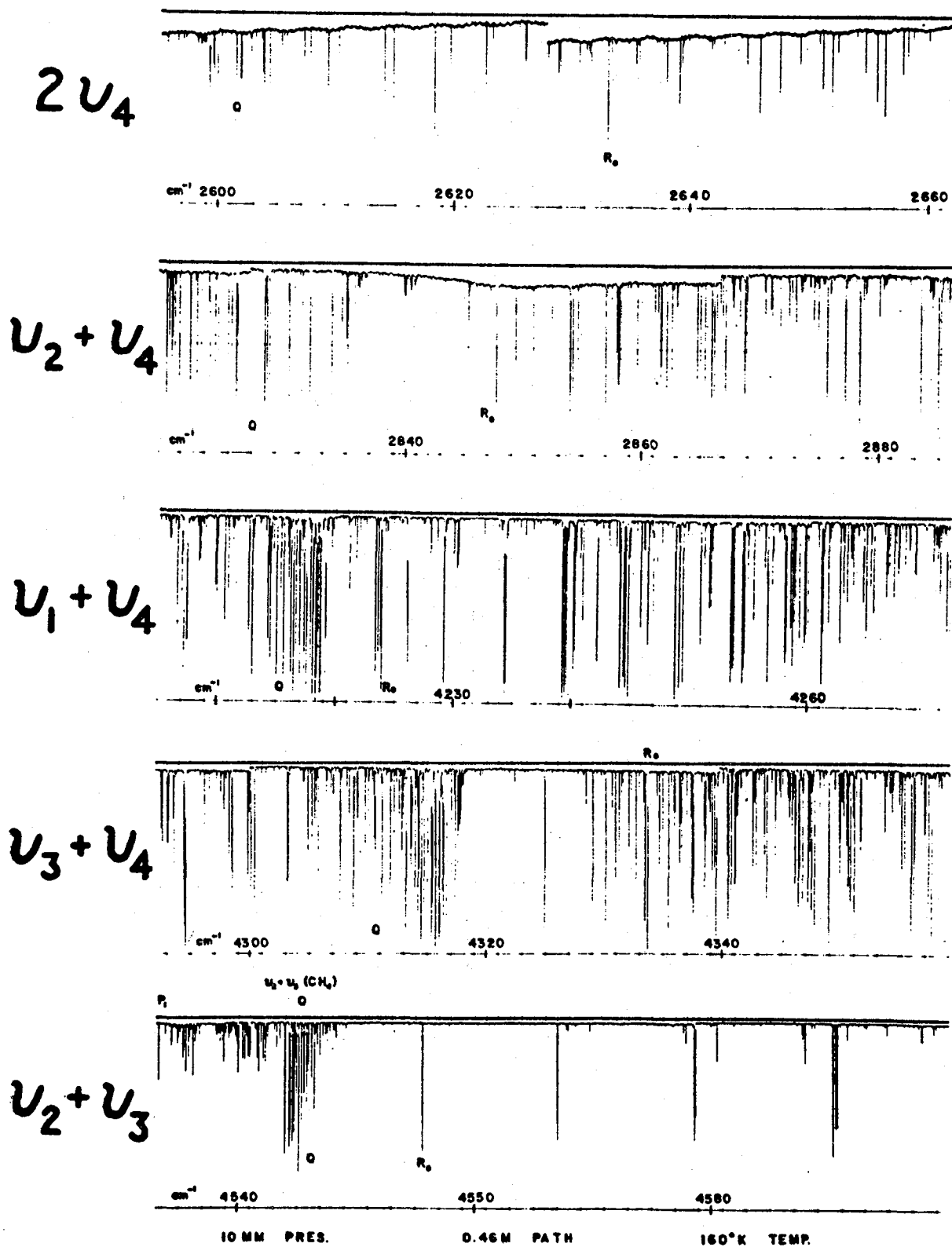
Figure 7. A spectrum of methane recorded with the FTS at an intermediate optical density at 160K showing portions of an overtone and 4 combination bands. Note that the spectral patterns vary greatly from band to band.
