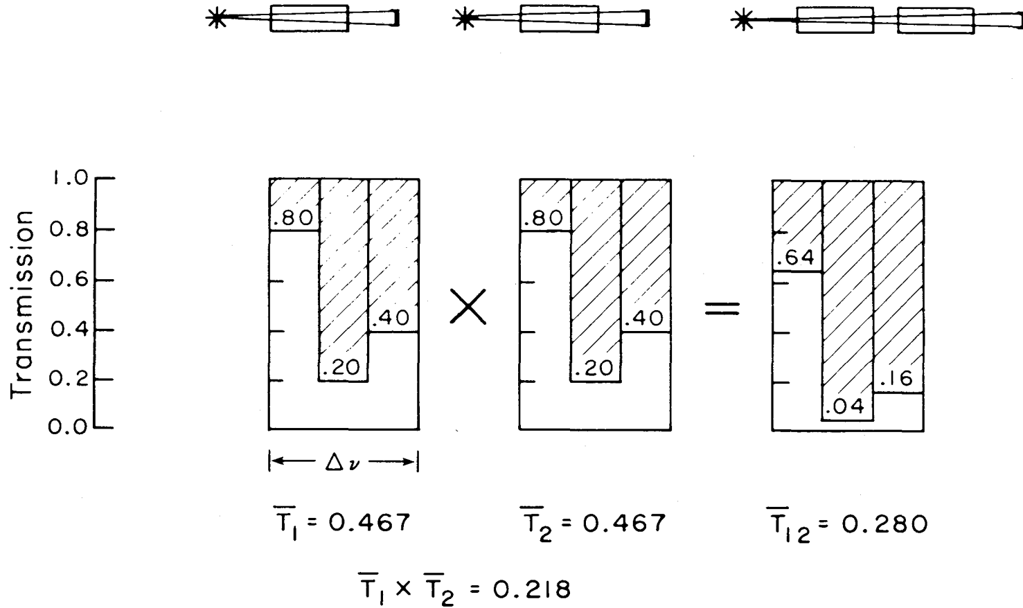
Figure 11. Limitations of band models as illustrated by failure of the multiplication property.
