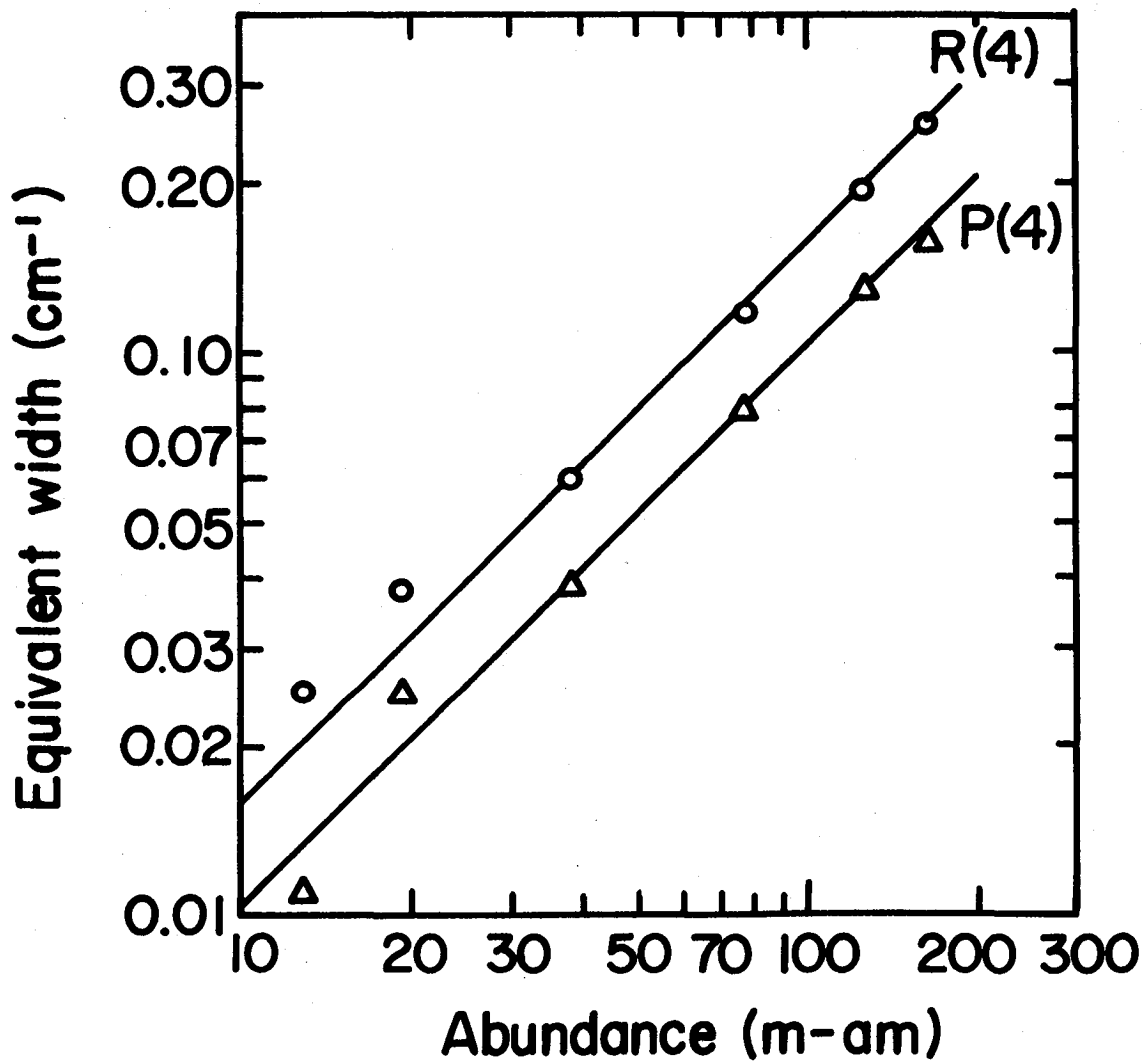
Figure 5. Curves of growth for the R(4) and P(4) lines of the 9613 Å band of CH 3 D.
