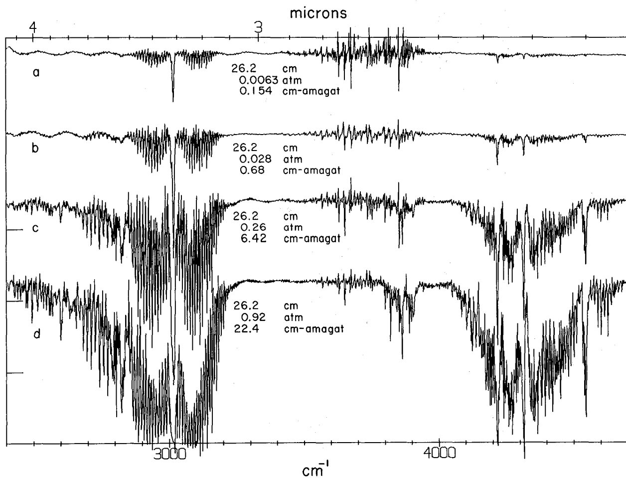
Figure 9. Low resolution spectra of \text{CH}_4 ( 2400\text{--}4700\text{ cm}^{-1} ) for various column densities.
