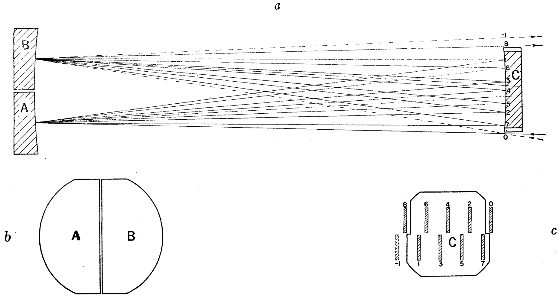
Figure 6. Schematic diagram of a typical multiple-pass absorption cell.
