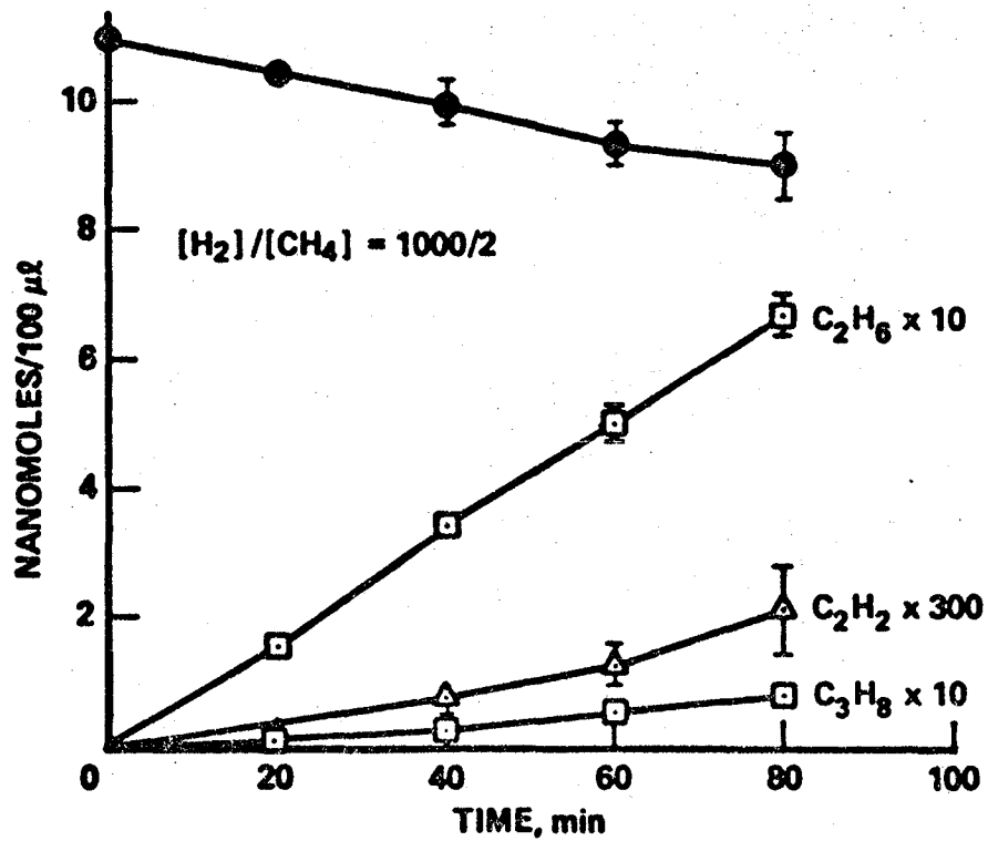
Figure 3. Variation of product concentrations with photolysis time.
