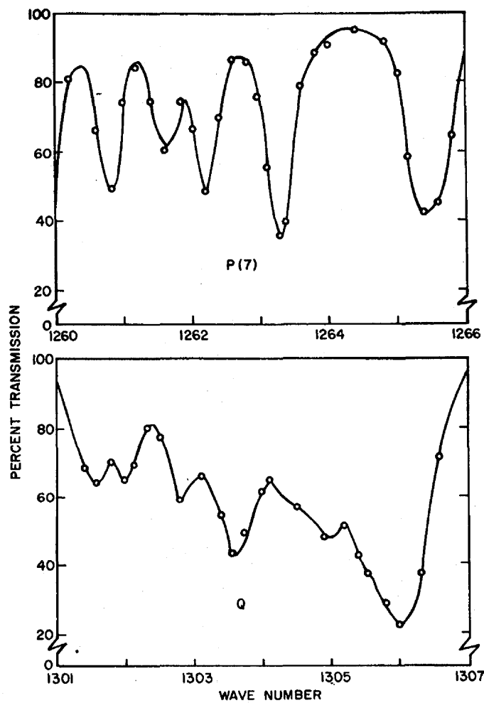
Percentage spectral transmission through rotational lines in the \nu_4 -fundamental of ^{12}\text{CH}_4 at 300°K. Spectral resolution = 0.2 \text{ cm}^{-1} ; 5.37% [for P(7) ], 1.1% (for Q -branch) methane in hydrogen; cell length = 6.1 cm; total pressure = 3 atm.
