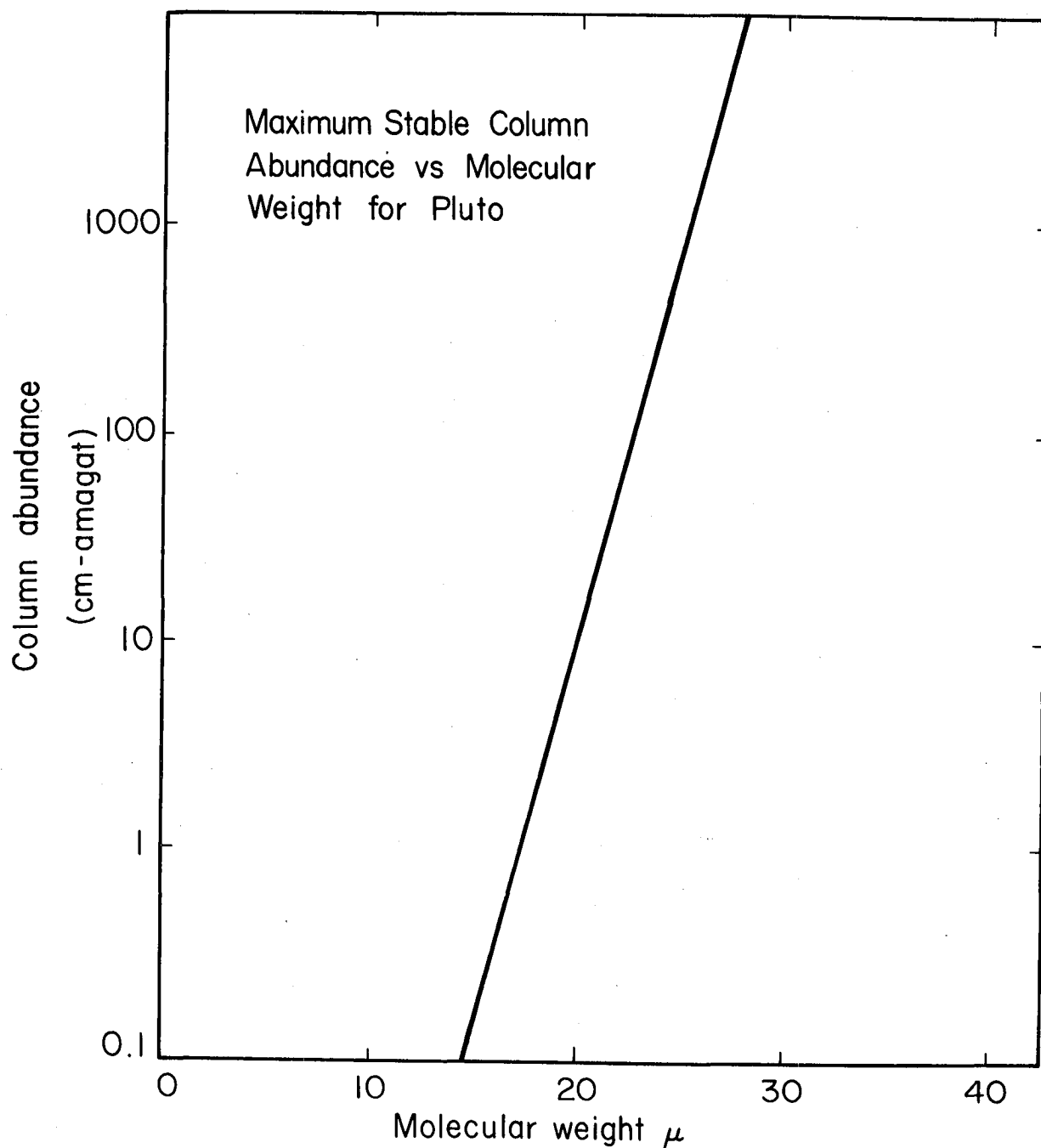
Figure 1. The maximum column abundance of gas stable on Pluto against blowoff vs. molecular weight. Values for the mass, radius, and temperature of 10^{25} g, 1500 km, and 55 K are assumed. See the appendix of Trafton (1980) for method of calculation.
