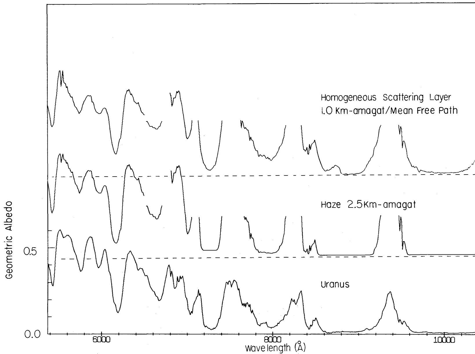
Figure 12. Comparison of observed albedo of Uranus (bottom trace) with two calculated models (after Benner and Fink, 1980).
