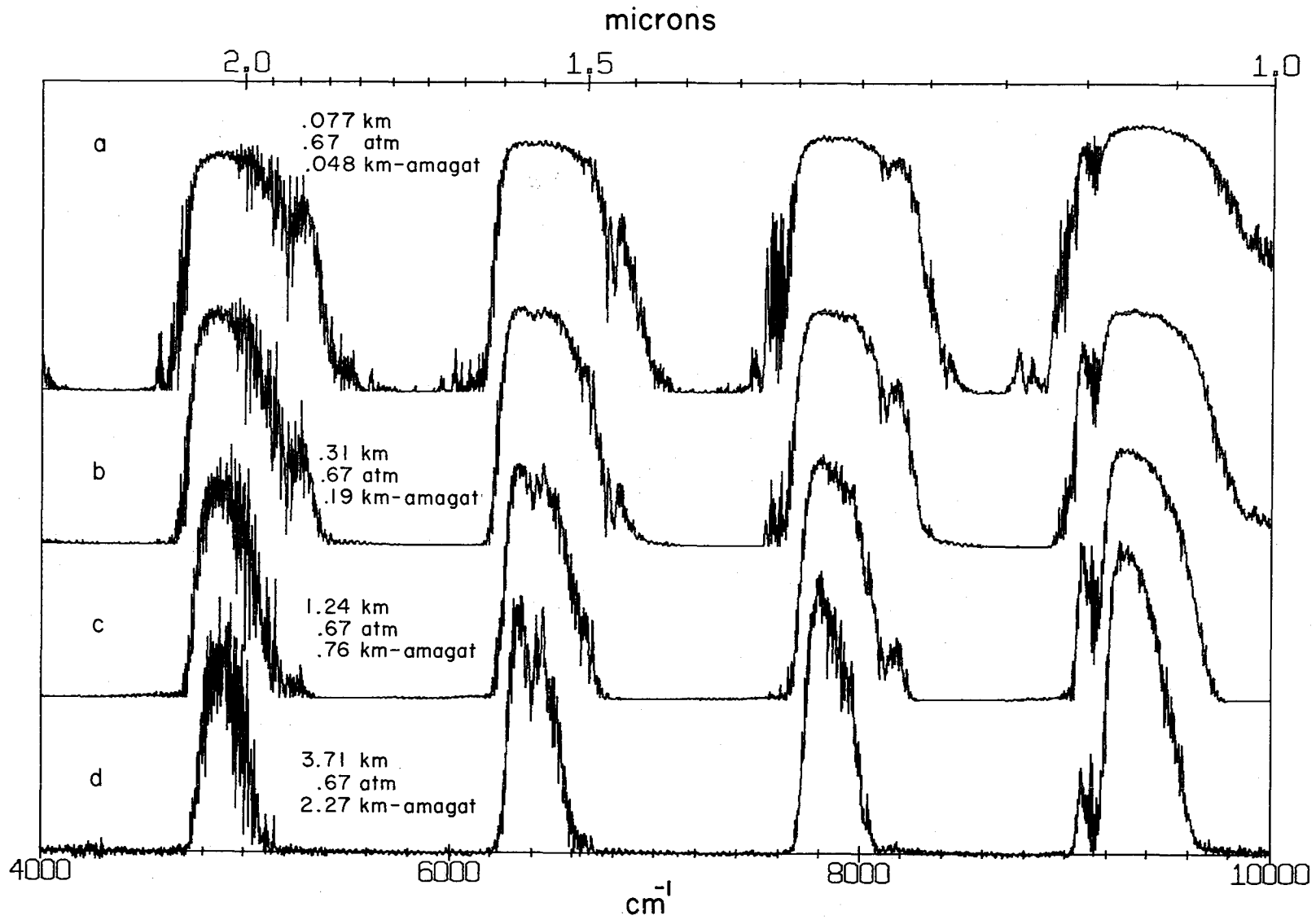
Figure 10. Low resolution spectra of \text{CH}_4 ( 4000\text{--}10,000\text{ cm}^{-1} ) at higher column densities than shown in Figure 8.
