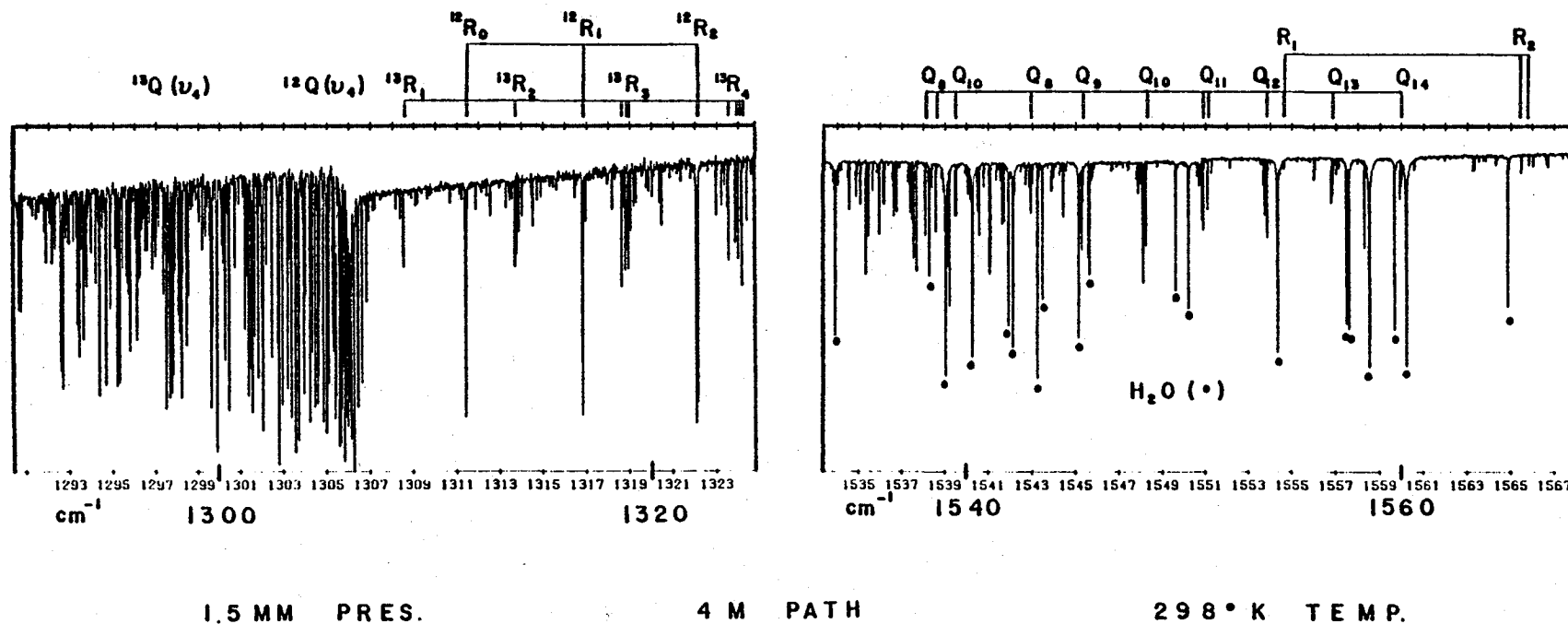
Figure 3. Spectrum of ^{12}\text{CH}_4 recorded at an intermediate optical density with the FTS at KITT Peak. In the left panel, transitions of the \nu_4 fundamental ^{12}\text{CH}_4 and ^{13}\text{CH}_4 are labelled. In the right panel, the \text{H}_2\text{O} lines are indicated, and the remaining lines of \nu_2 of ^{12}\text{CH}_4 have strengths similar to the ^{13}\text{CH}_4 \nu_4 lines observed in isotopic abundance.
