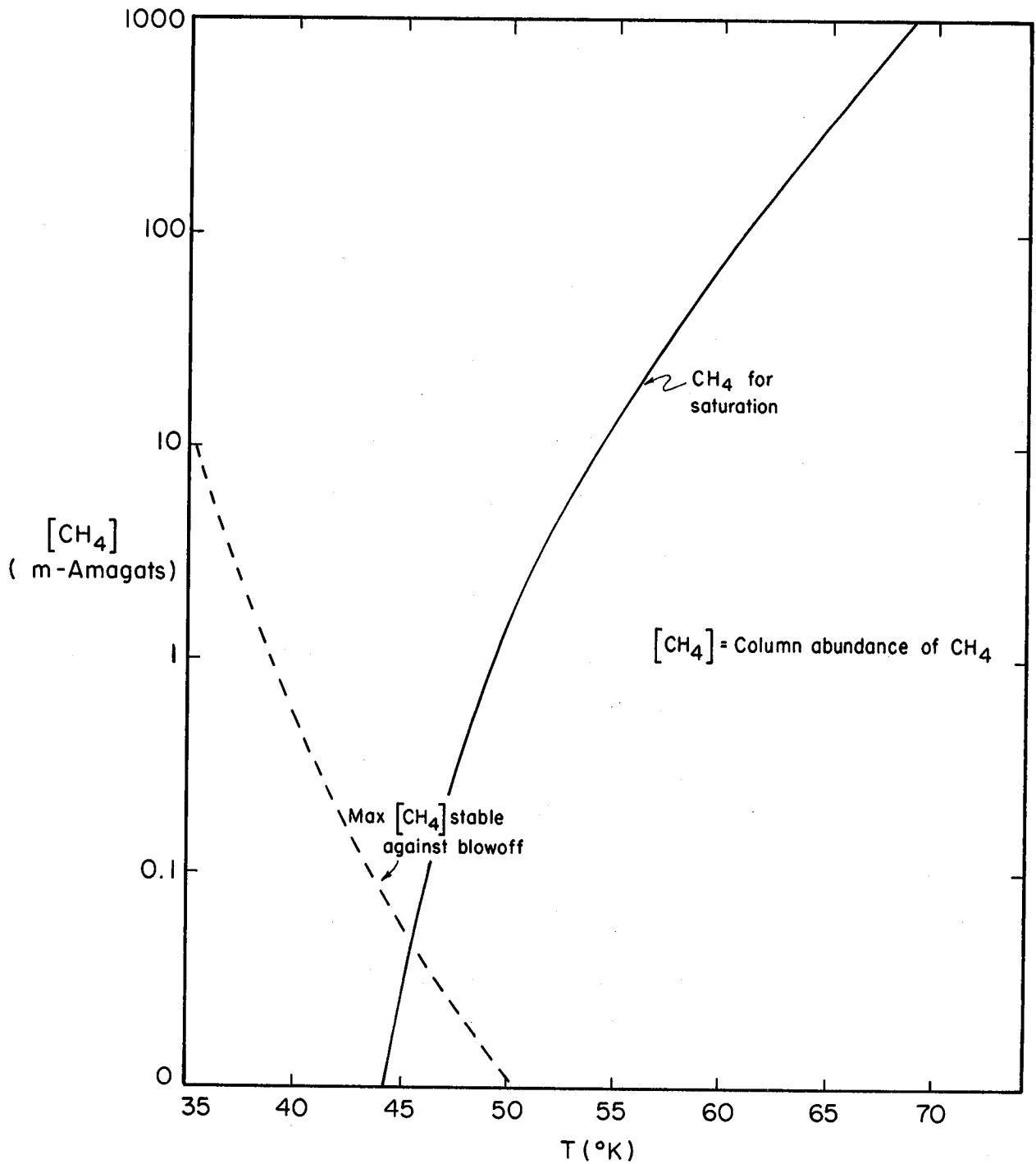
Figure 2. Maximum \text{CH}_4 column abundance stable on Pluto against blowoff and the column abundance of \text{CH}_4 corresponding to equilibrium between the gas and frost vs. temperature for an isothermal atmosphere. For T < 45 K, the atmosphere is stable against blowoff; for T > 45 K, sublimation drives blowoff (from Trafton, 1980).
