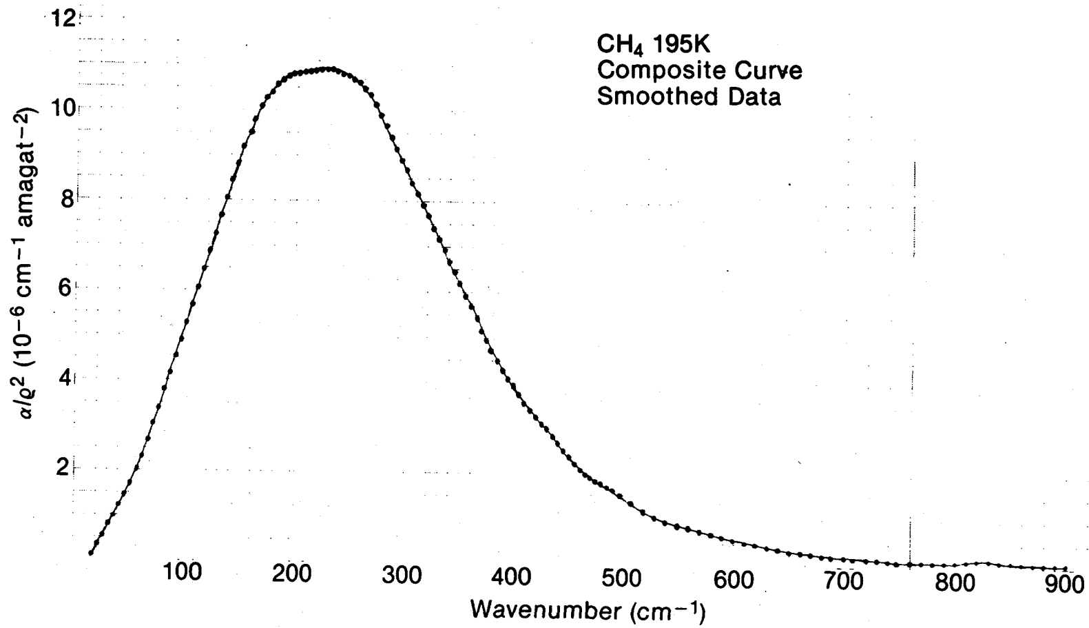
Figure 1. Spectrum of CH 4 at 195K.
