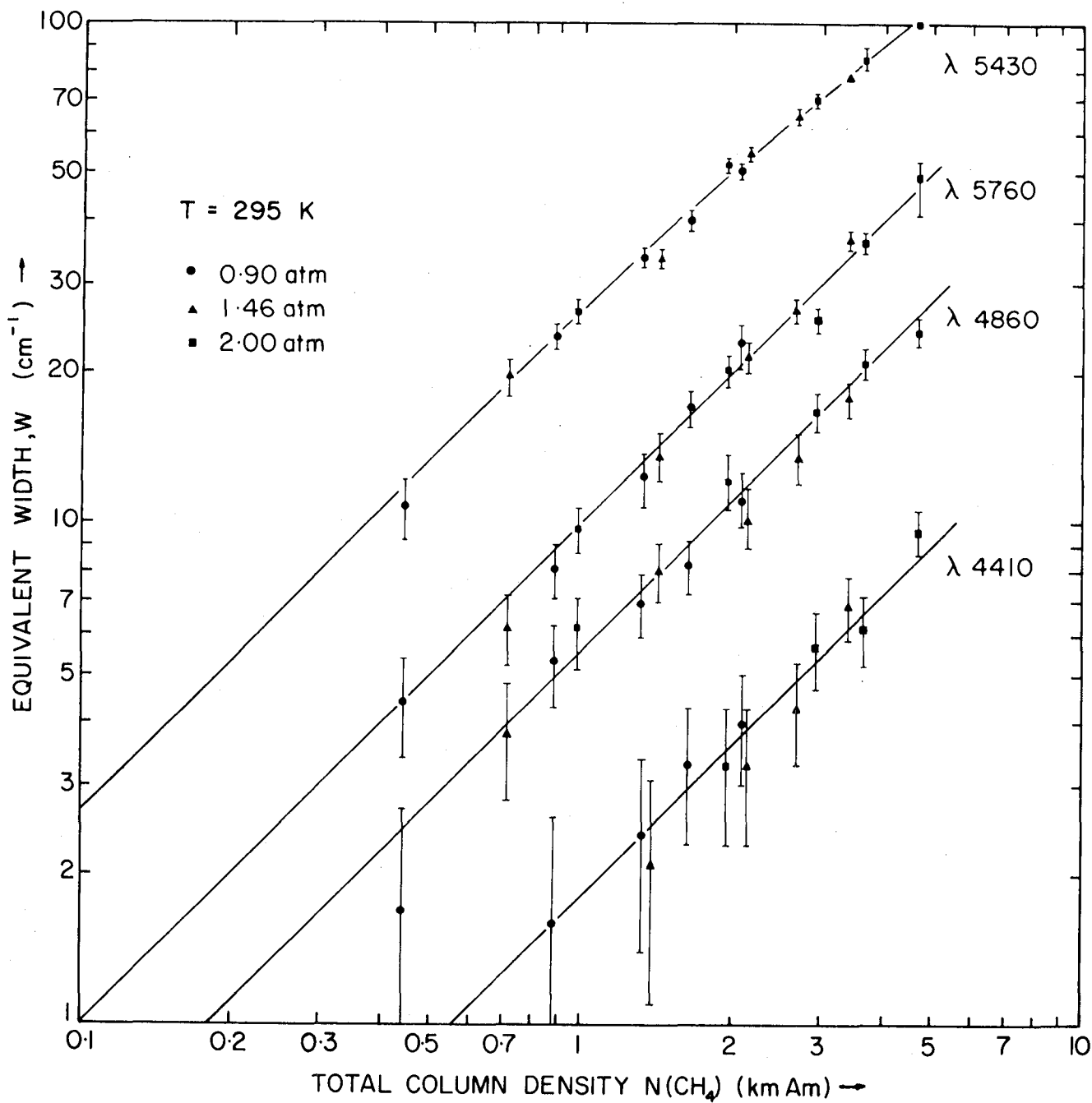
Figure 5. Equivalent width vs. column density for various CH 4 bands (after Lutz et al. 1976) illustrating the linear relationship with abundance.
