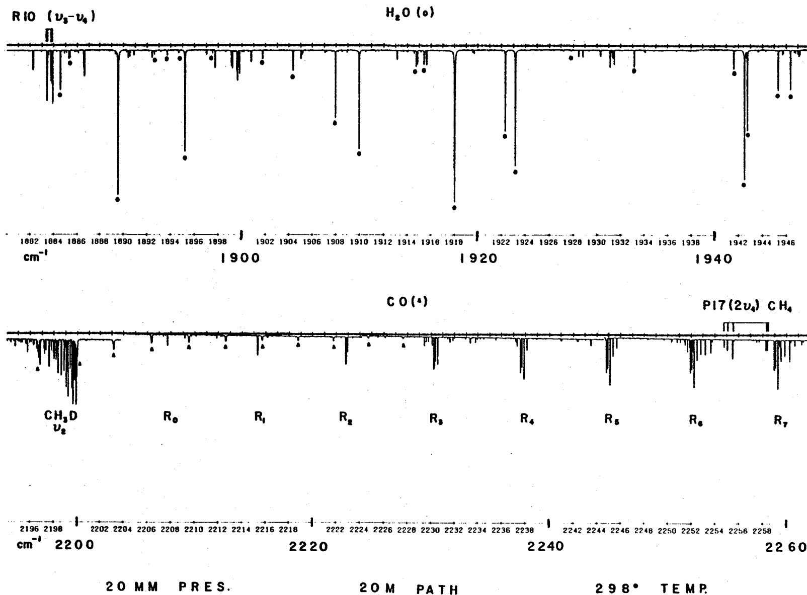
Figure 12. Portions of the methane FTS spectrum at high optical density near the 5\mu\text{m} window. Impurities of H 2 O and CO are indicated, and the remaining lines belong to \nu_3 - \nu_4 of 12 CH 4 , CH 3 D and 2\nu_4 of 12 CH 4 .
