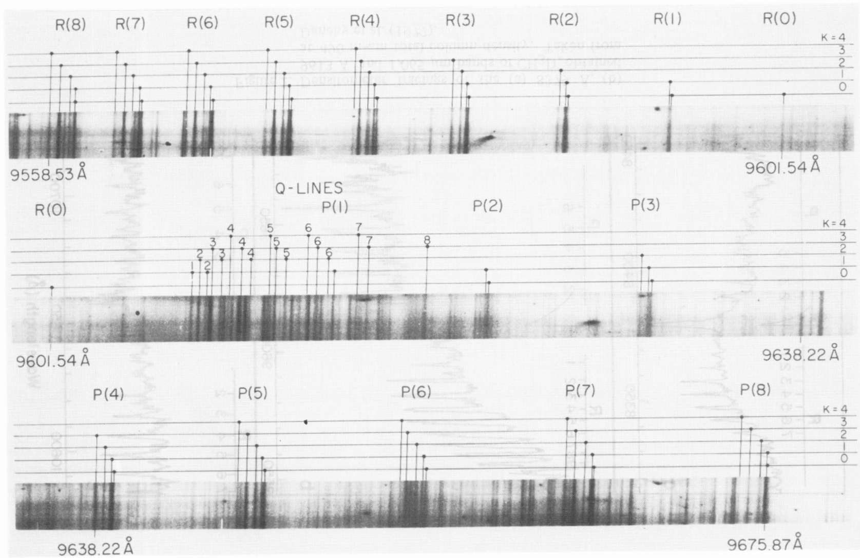
Figure 3. The 9614 Å band of CH 3 D photographed at 452 m-am total column density. Taken from Lutz, Danehy, and Ramsay (1978).
