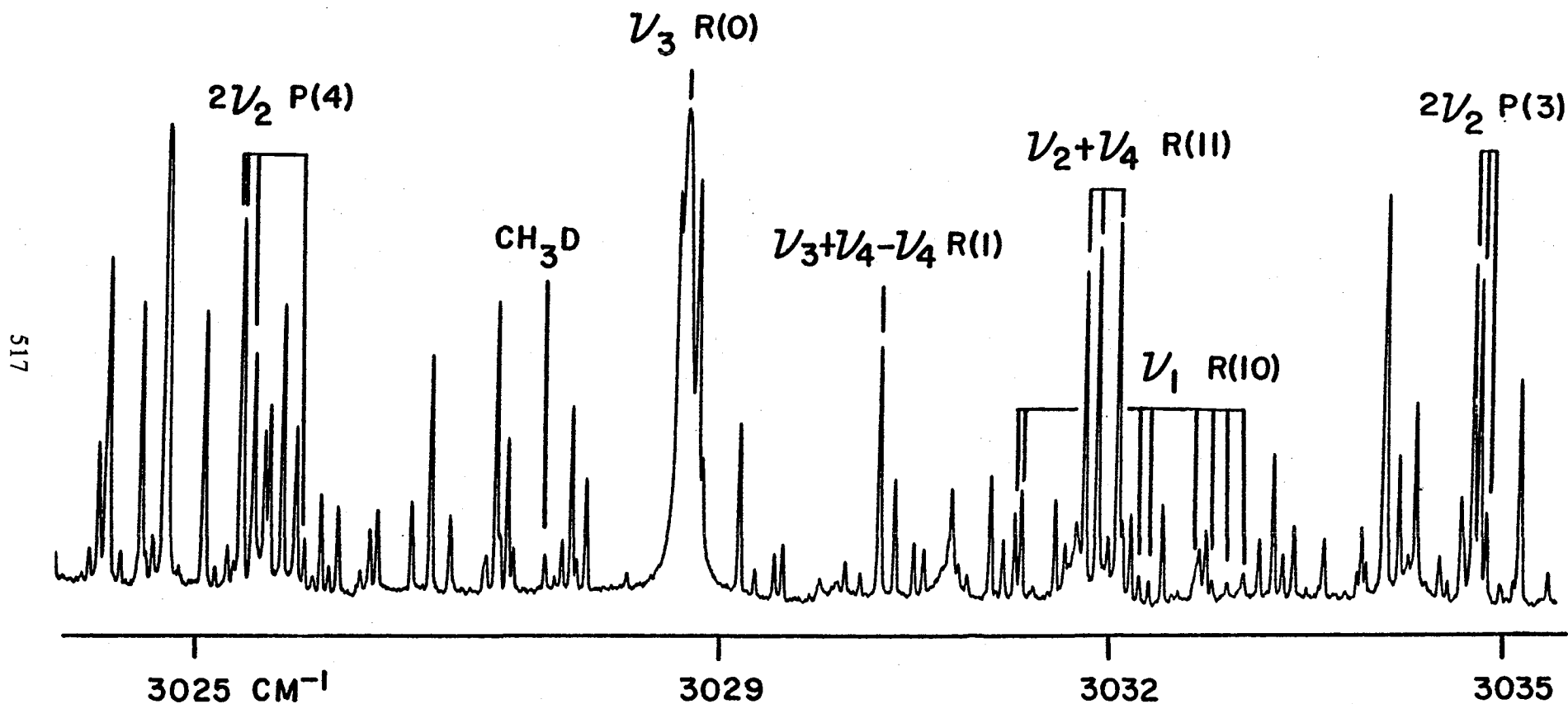
Figure 10. A methane spectrum recorded at 0.02 \text{ cm}^{-1} resolution with the Florida State grating spectrometer at high optical density. Transitions of 2\nu_2 , \nu_3 , \text{CH}_3\text{D} , \nu_3 + \nu_4 - \nu_4 , \nu_2 + \nu_4 and \nu_1 are indicated to show relative intensities of the bands.
