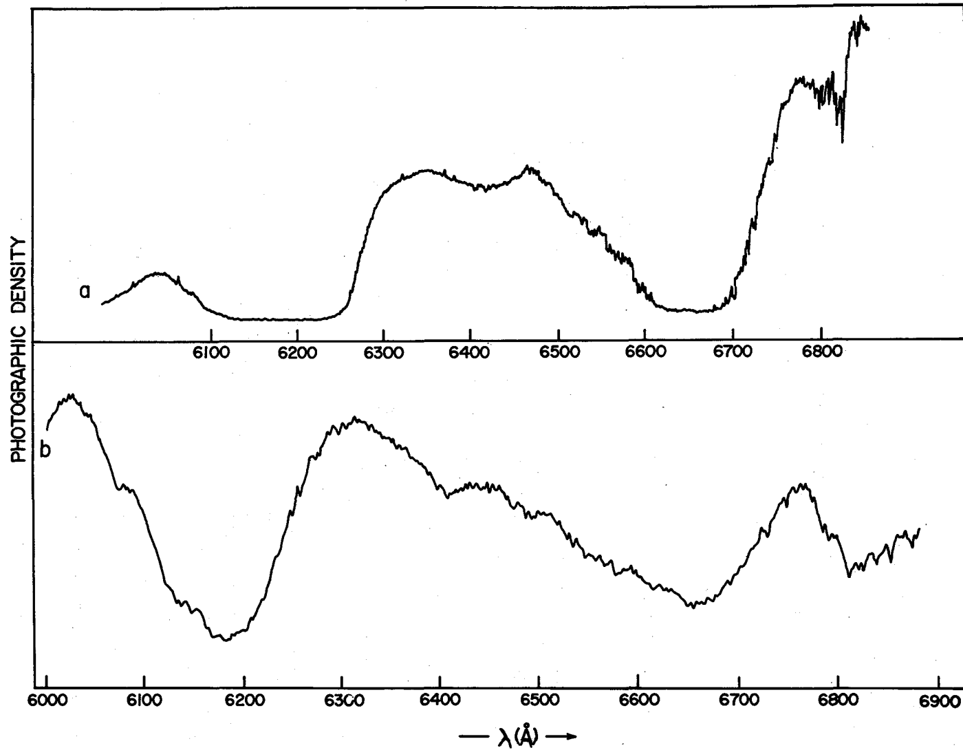
Figure 1. a) Density tracing of the 10.1 km-amagat spectrum of methane. b) Intensity spectrum of Uranus divided by the lunar spectrum. Taken from Owen et al. (1974).
