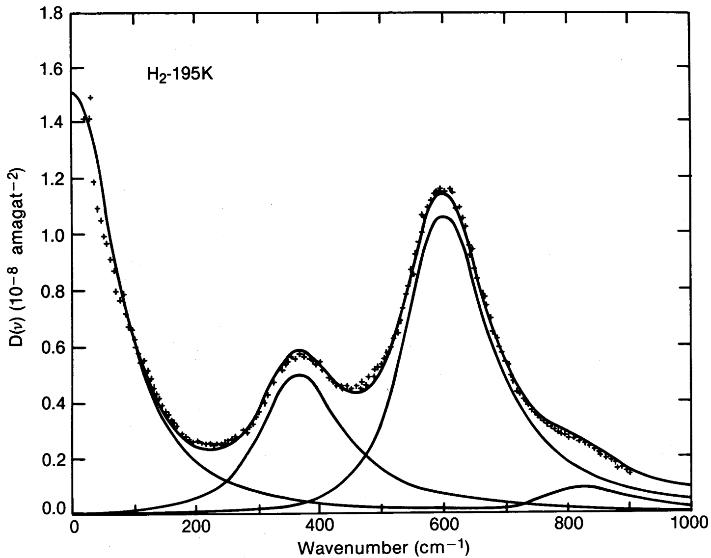
Figure 9. Three parameter fit obtained by adjusting an amplitude parameter and two time parameters (defined in ref. 5) to the spectrum of H 2 at 195K (ref. 4). The total spectrum as well as the translational and rotational components are shown.
