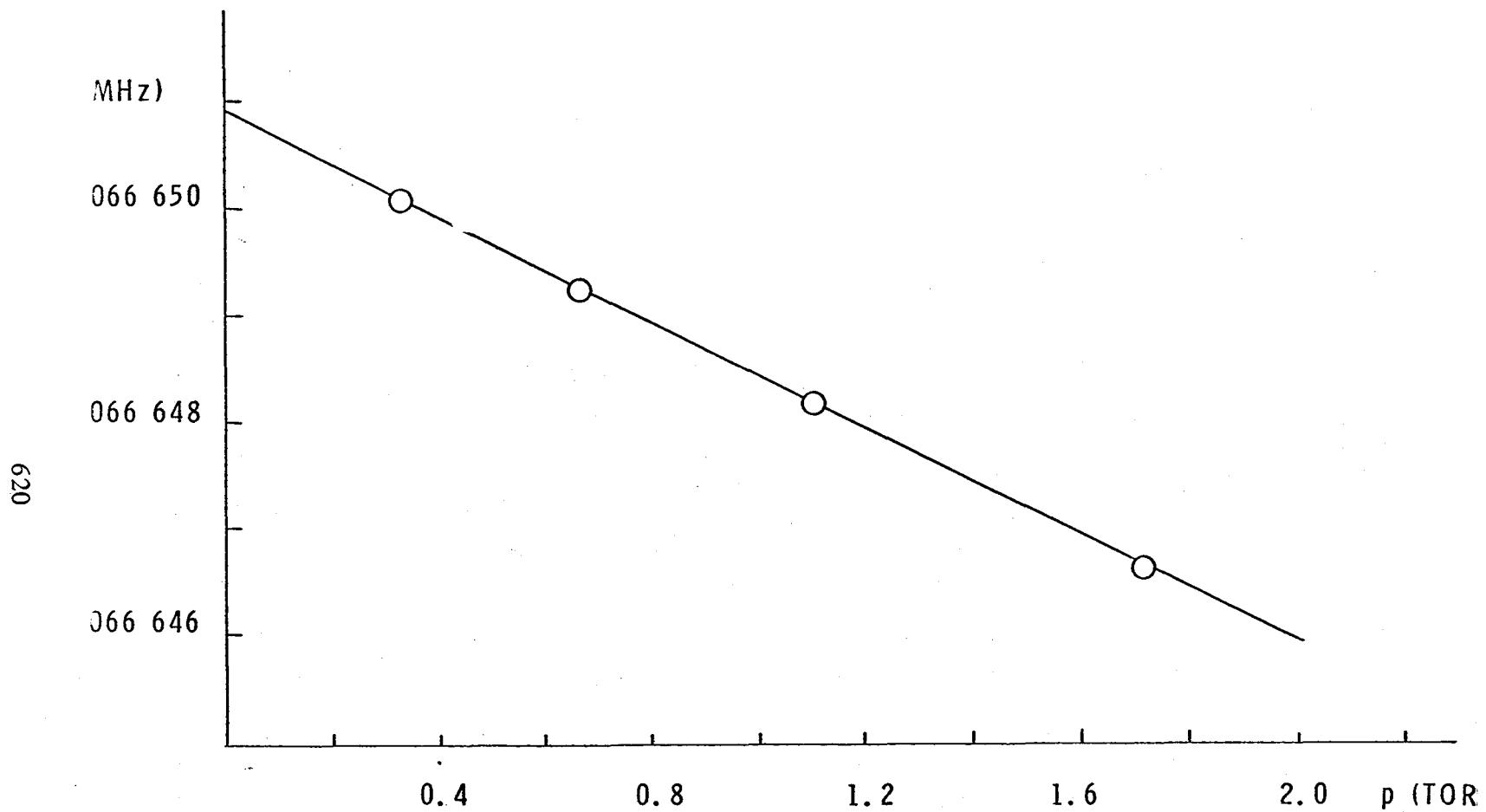
Figure 5. Dependence of the frequency of the (1,1) transition of ^{14}\text{NH}_3 in the \nu_2 state on the pressure of ammonia gas (J. Mol. Spectrosc. 84, 290 (1980)).
