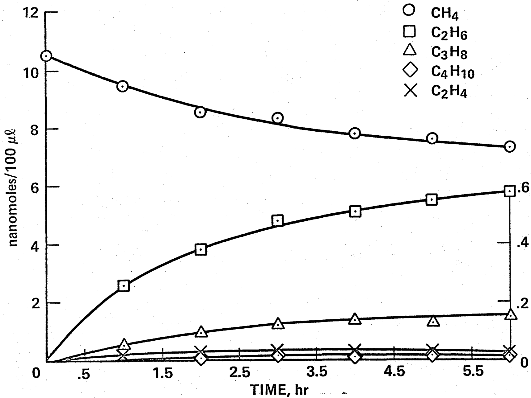
Figure 2. Concentrations of methane and products vs. photochemical exposure time.
