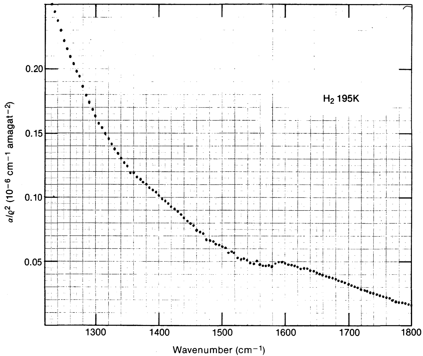
Figure 7. High frequency absorption in H 2 at 195K from 1220 to 1800 \text{cm}^{-1} .
