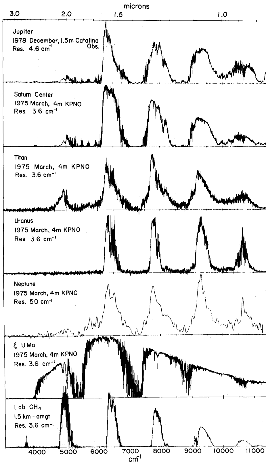
Figure 7. Spectra of the outer planets, a comparison star, and laboratory \text{CH}_4 illustrating the importance of \text{CH}_4 spectroscopy to the outer planets.
