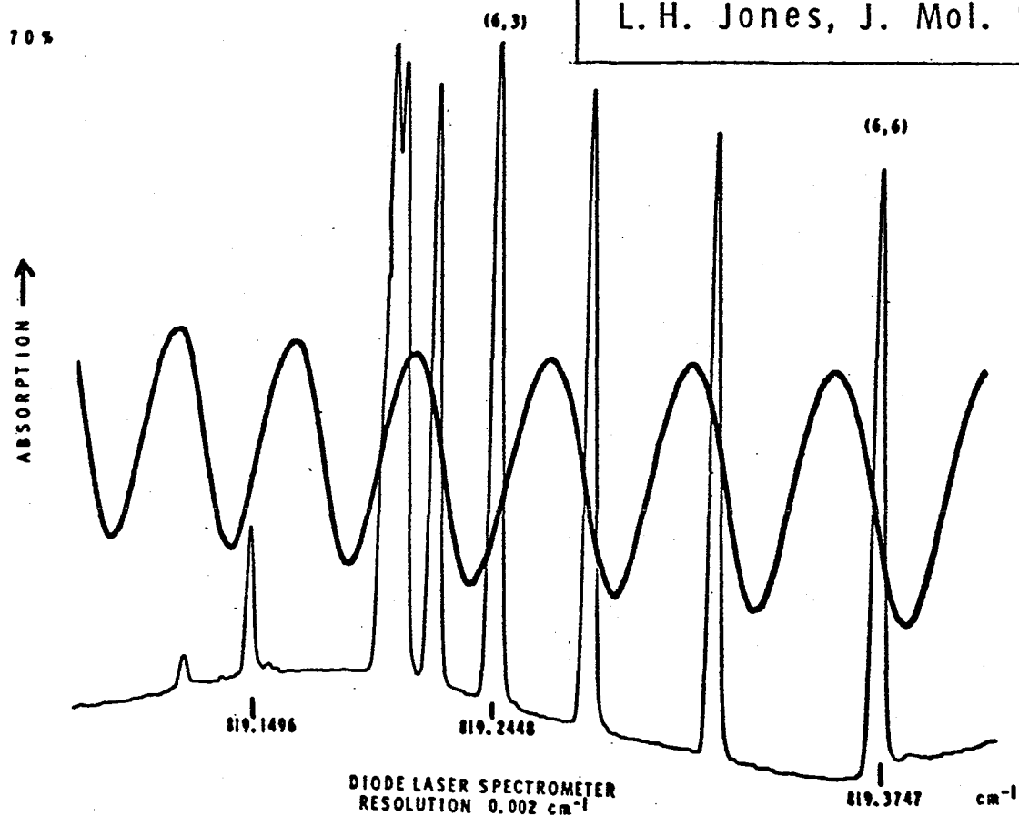
Figure 7. sR (6,K) multiplet in the \nu_2 band of ^{14}\text{ND}_3 .
