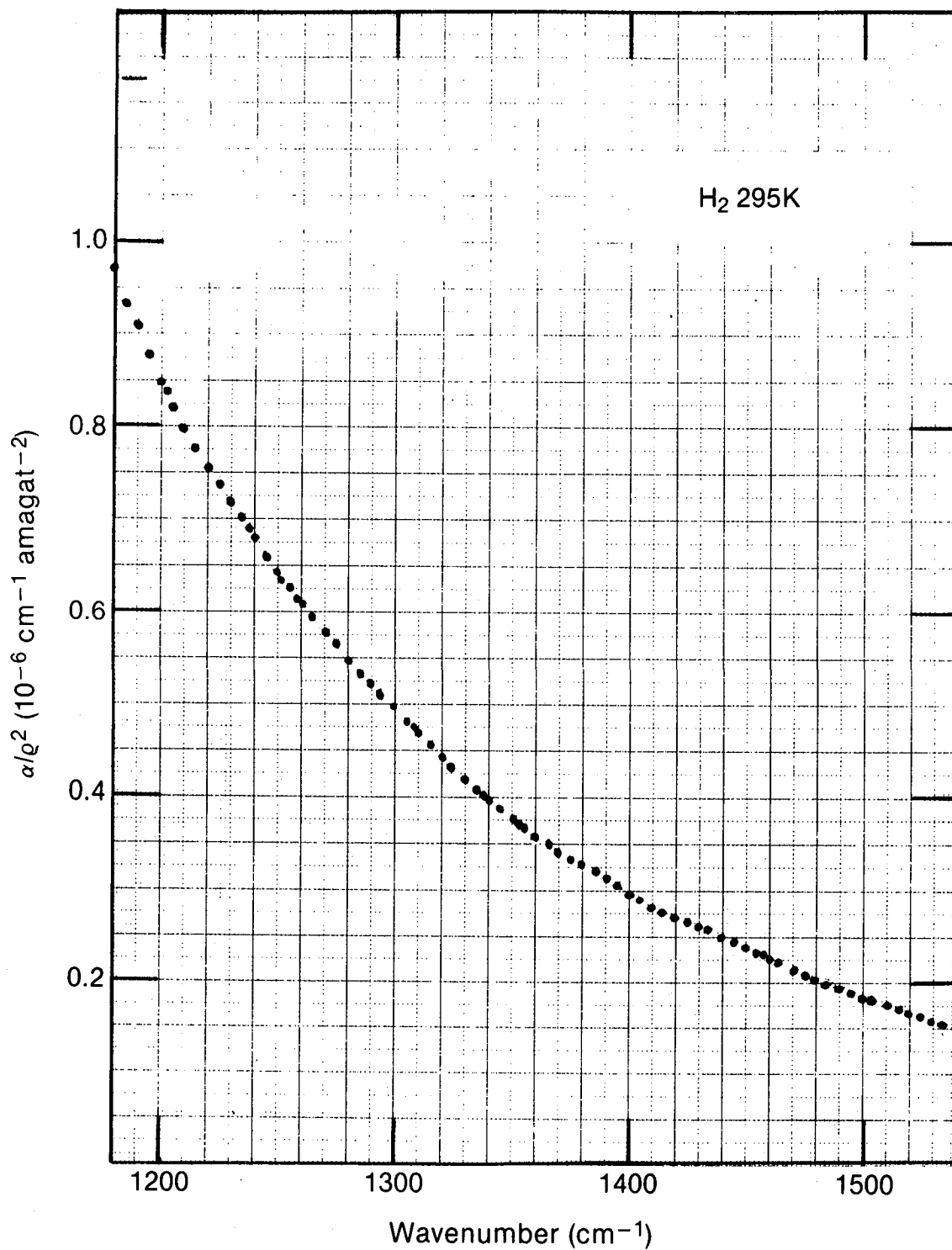
Figure 5. High frequency absorption in H 2 at 295K from 1180 to 1540 cm -1 .
