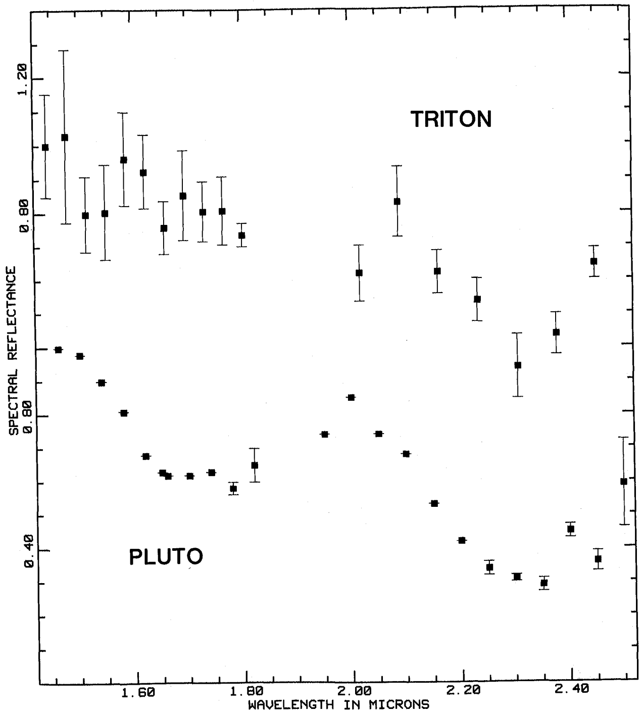
Figure 4. (Upper) Spectrum of Triton (4) with additional points omitted from Fig. 2, and (lower) the spectrum of Pluto (11) showing strong absorption of CH 4 frost.
