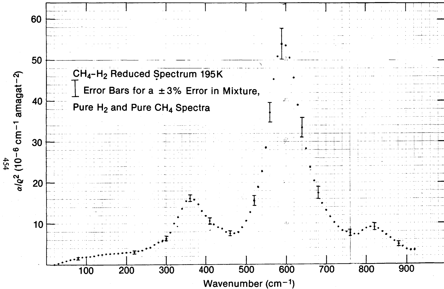
Figure 3. Spectrum due to H 2 -CH 4 collisions at 195K. The error bars are estimated on the assumption that the error in measuring the absorption in H 2 , CH 4 and the H 2 -CH 4 mixture is \pm 3\% .
