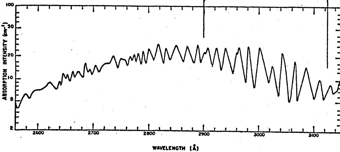
FIG. 2. Absorption intensities of \text{SO}_2 at 2560–3150 Å.
