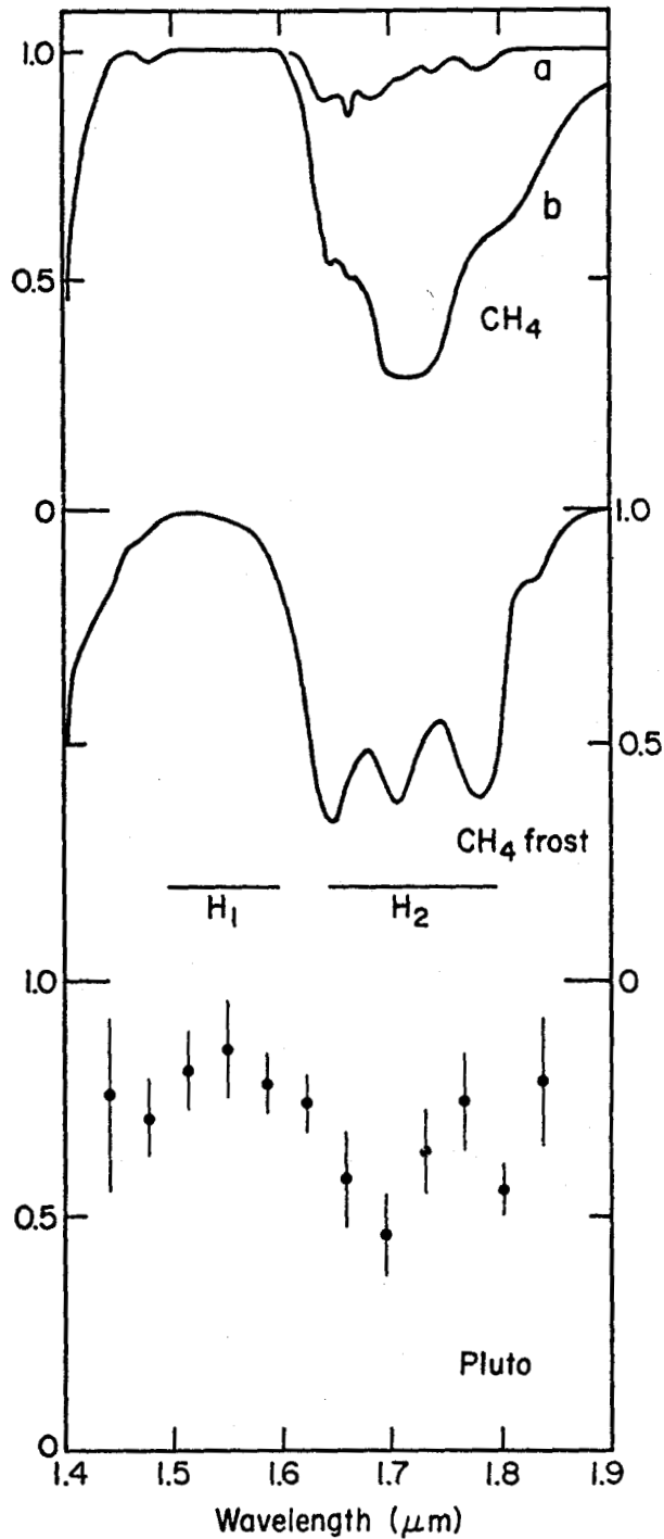
Figure 1. Infrared spectrophotometry of Pluto (data points at bottom). In the schematic CH 4 gas spectra shown at the top, a represents a few cm-atm of CH 4 observed in the laboratory and b represents several m-atm. The frost spectrum is after Kieffer (private communication). H 1 and H 2 show the wavelengths of the two filters used in Ref. 2.
