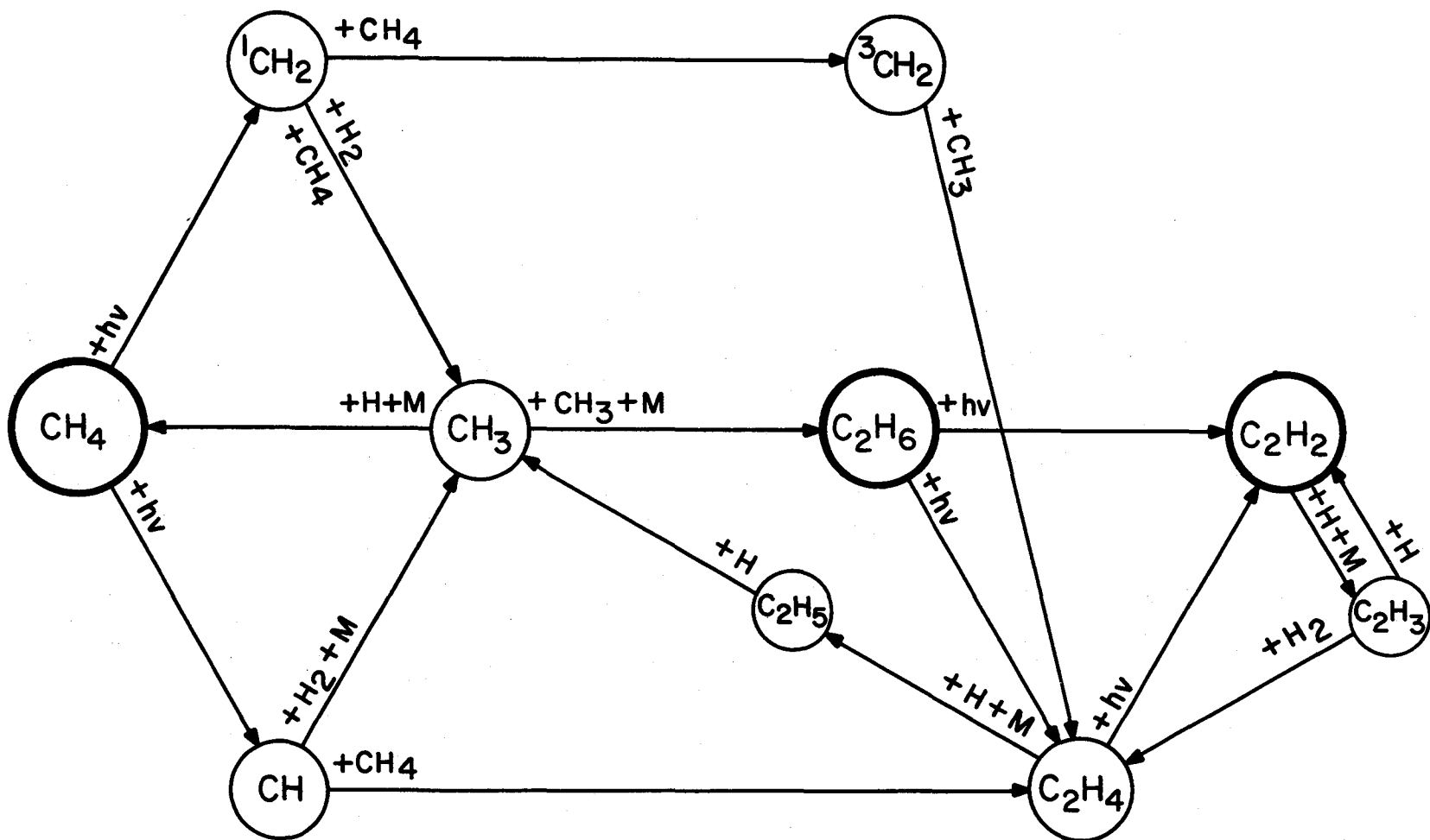
Figure 1. Principal photochemical pathways postulated for synthesis of acetylene, ethylene and ethane from methane in outer planetary atmospheres. (From Strobel, 1973).
