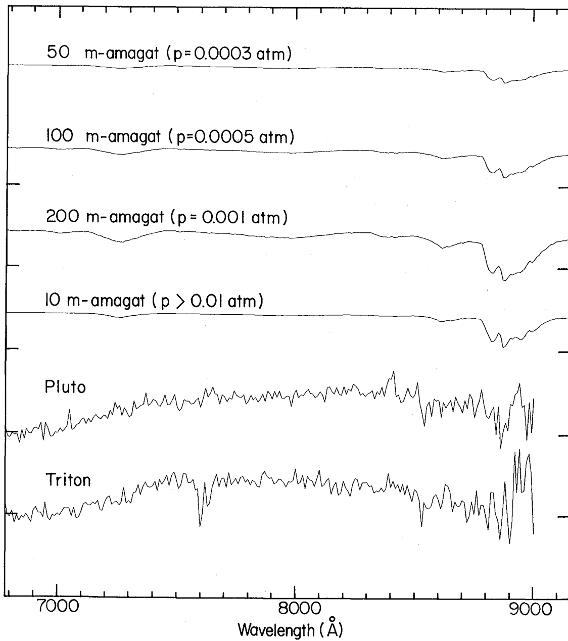
Figure 13. Comparison of observed spectra of Pluto and Triton (Benner et al. 1978) with various random band models.
