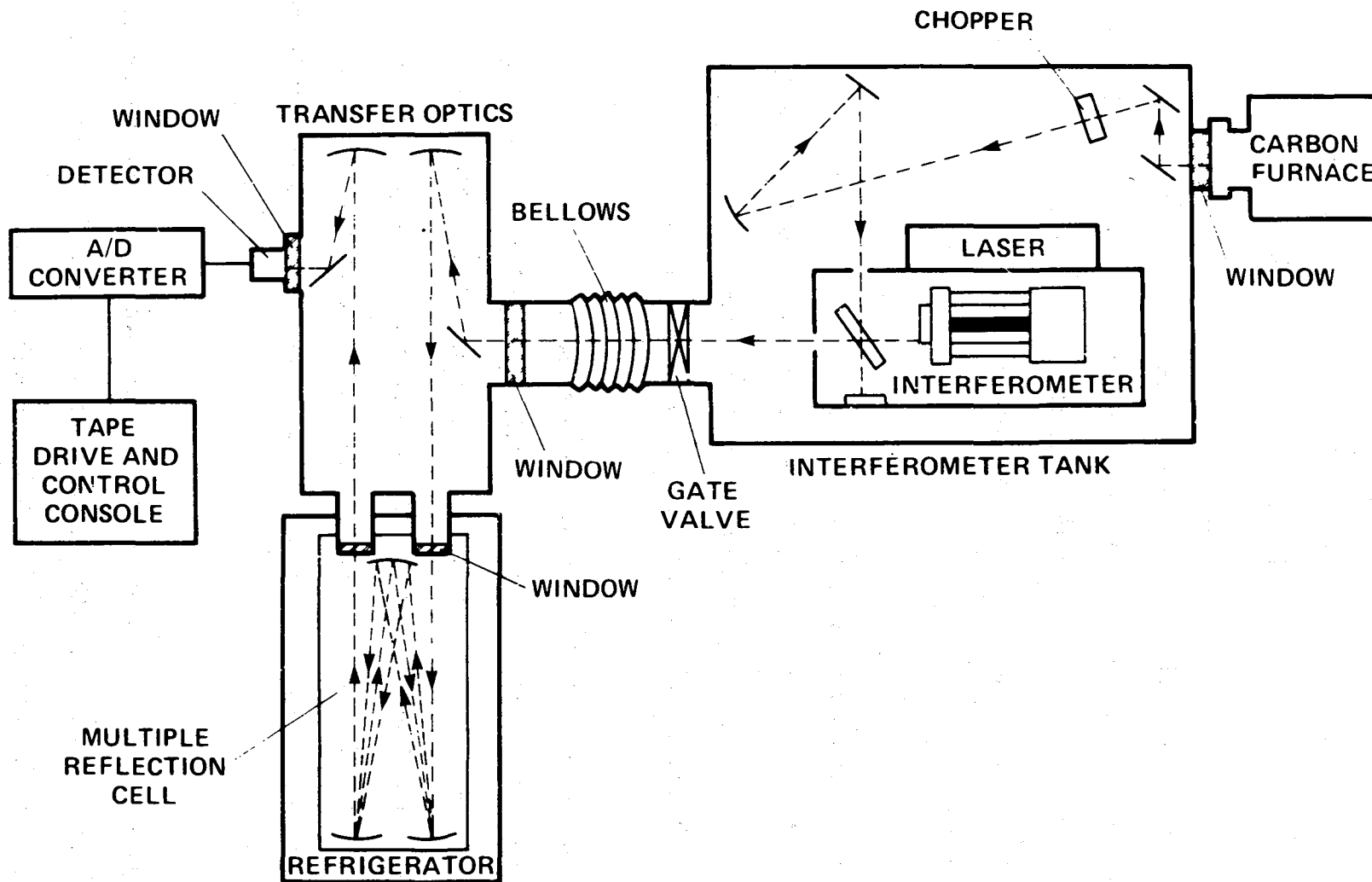
Figure 1. Schematic of apparatus.
