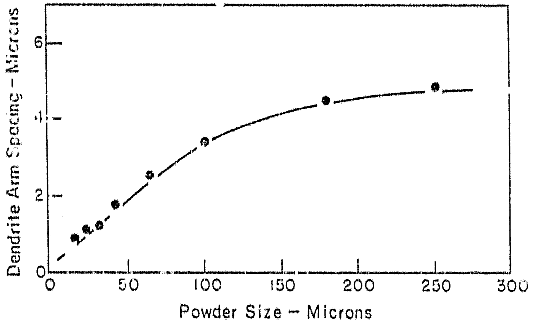
Figure 5. Variability of dendrite arm spacing with powder size for 2024 + Ti 0.3% aluminum alloy.
