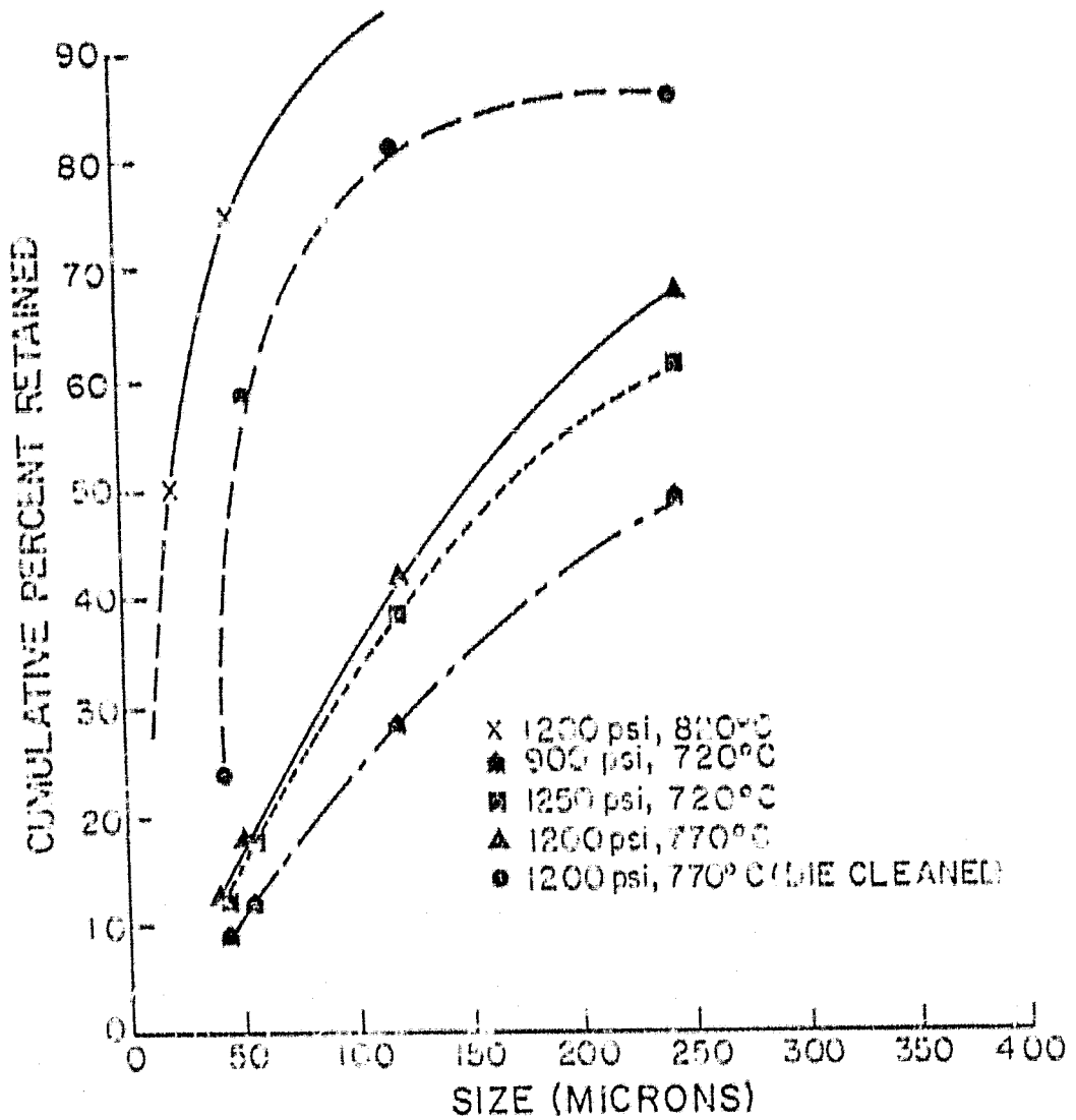
Figure 9. Breaker size ranges for BMA (broken) as a function of steam temperature and gas pressure (velocity).
