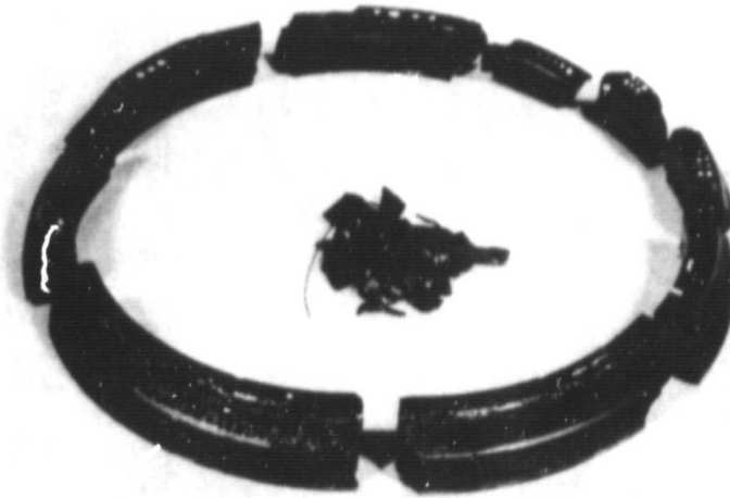
Figure 11. - Fractured bearing inner race initiated by a rolling-element fatigue spall. (From ref. 34.)
