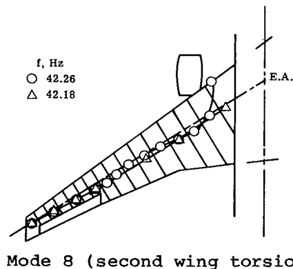
Figure 3.- Node lines and frequencies for first eight structural modes.
