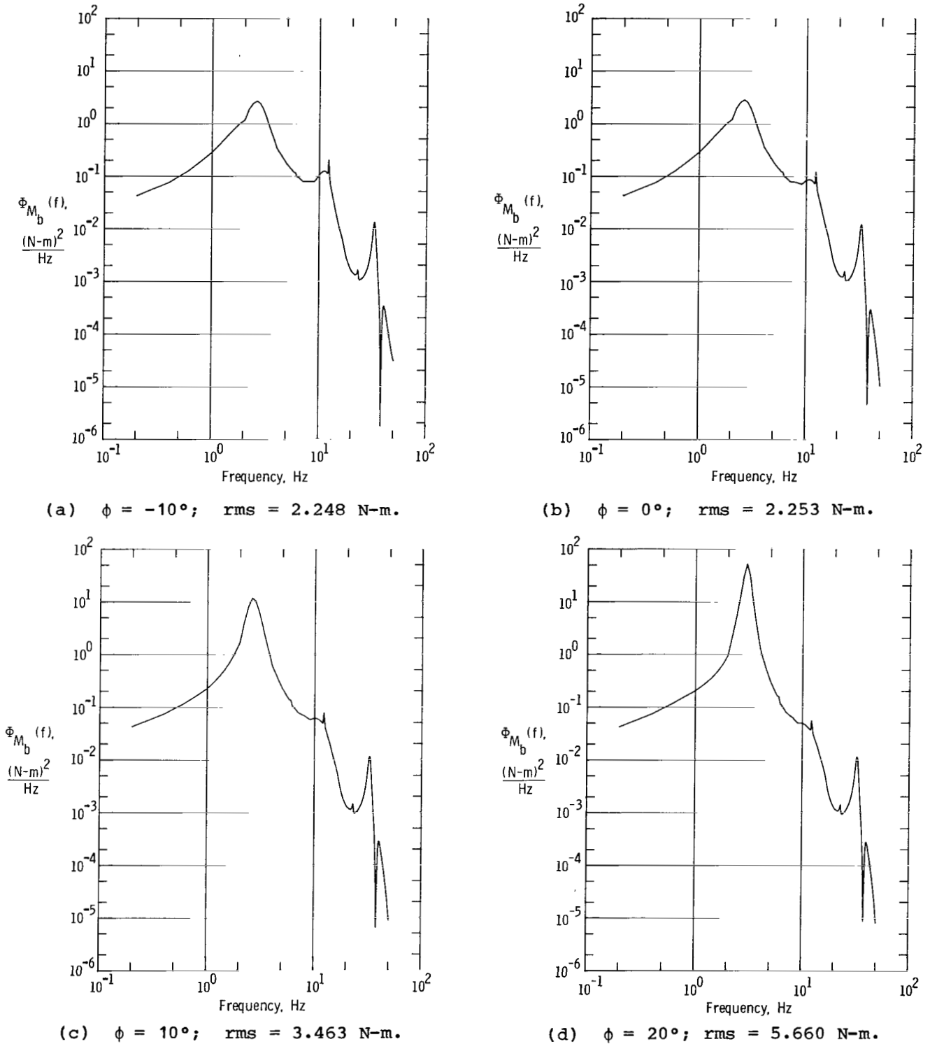
Figure 26.- Bending-moment psd as function of phase angle for control law 1 at V = 30.9 m/sec. 48-percent semispan station.
