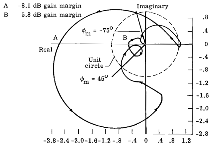
Figure 9.- Nyquist diagram for control law 1 at V = 56.32 m/sec. (Arrows indicate increasing frequency.)
