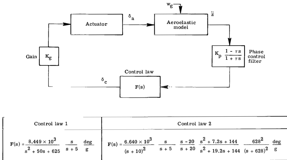
Figure 14.- Block diagram of active control system.
