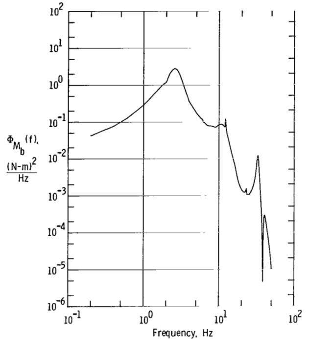
(b) Control law 1; rms = 2.253 N-m.
