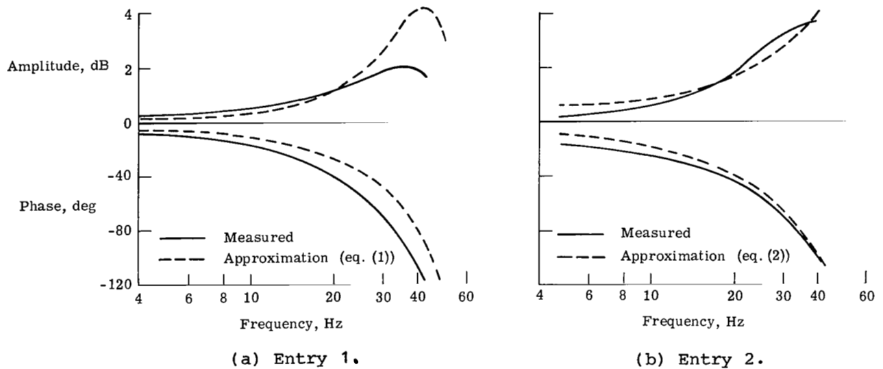
Figure 4.- Measured and approximated frequency responses of actuator.
