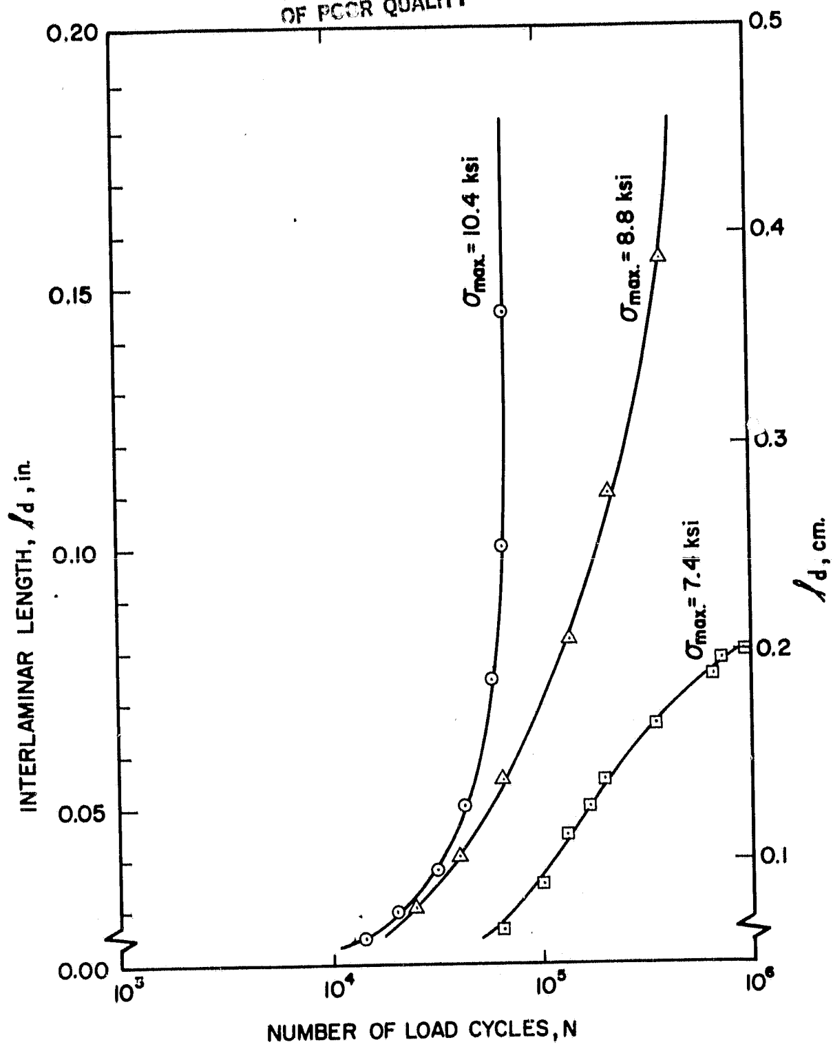
FIG. 6 INTERLAMINAR CRACK GROWTH DURING FATIGUE IN (45°-45°//45°-45°-45°/45°-45°/45°) GLASS/EPOXY
