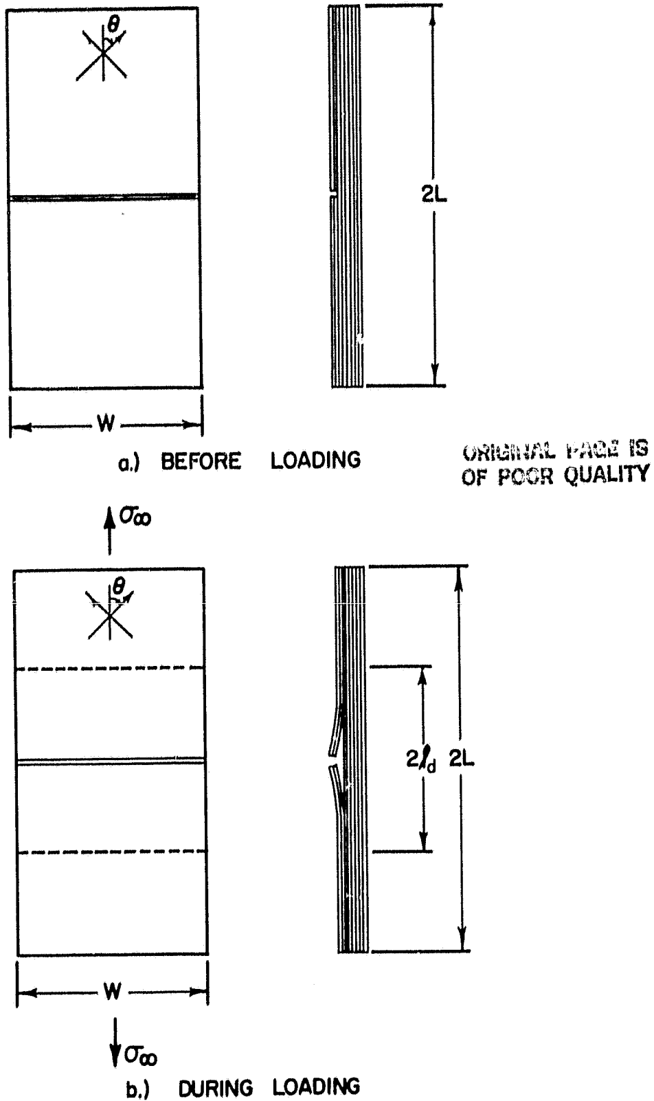
FIG. 2 FATIGUE TEST SPECIMEN FOR INTERLAMINAR CRACK GROWTH STUDY ( 2L = 6.0 in.; W = 1.0 in.)
