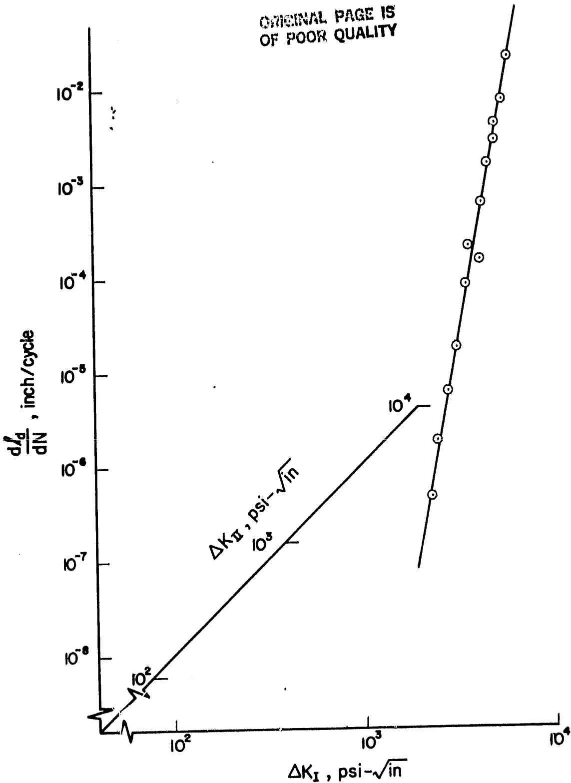
FIG.12 INTERLAMINAR CRACK GROWTH RATE d/d/dN AS A FUNCTION OF RANGES OF MIXED-MODE STRESS INTENSITY FACTORS, \Delta K_I & \Delta K_{II} FOR (45°-45°/45°-45°-45°/45°-45°/45°) GLASS/EPOXY
