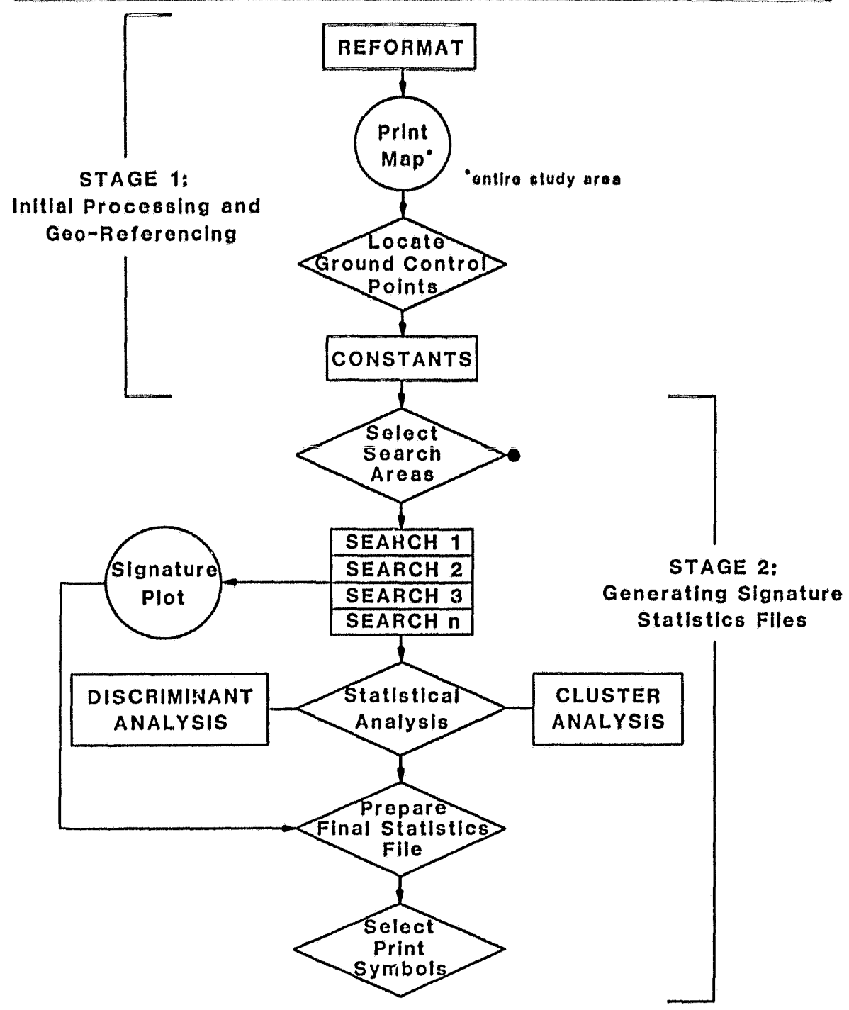
Figure 1. Summary of steps in Landsat digital data analysis: Stages 1 and 2.
