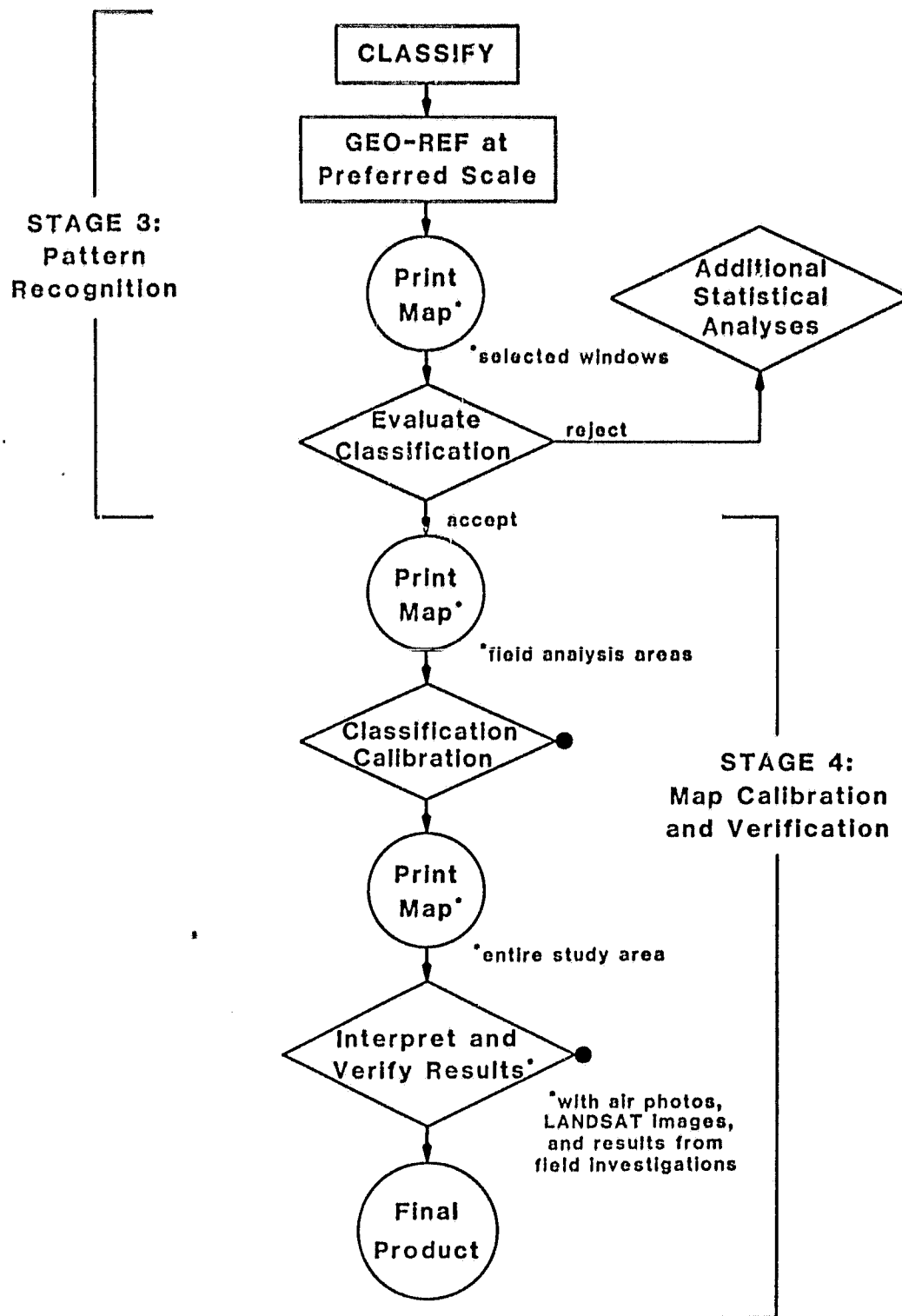
Figure 2. Summary of steps in Landsat digital data analysis: Stages 3 and 4.
