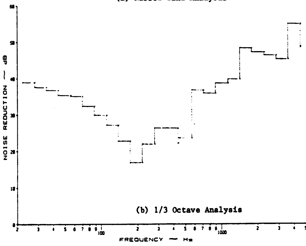
Figure B.93: Noise Reduction Characteristics of a Curved, Stiffened Panel at 0 psi Pressure Differential with Y-370 Damping Tape and 7.345 lb/ft 3 Insulation under White Noise
