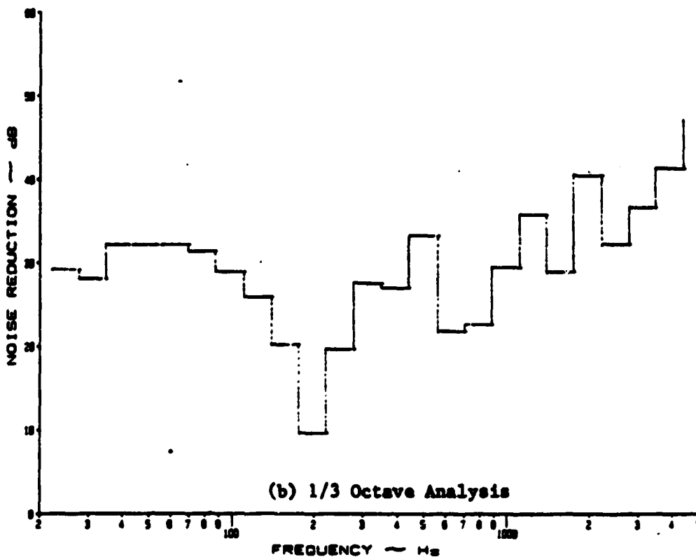
Figure A.6: Noise Reduction Characteristics of a Flat, Stiffened Panel at 1 psi Pressure Differential with No Treatment under White Noise
