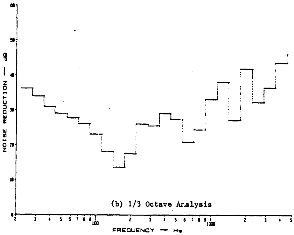
Figure A.37: Noise Reduction Characteristics of a Flat, Stiffened Panel at 0 psi Pressure Differential with Y-434 Damping Tape under White Noise
