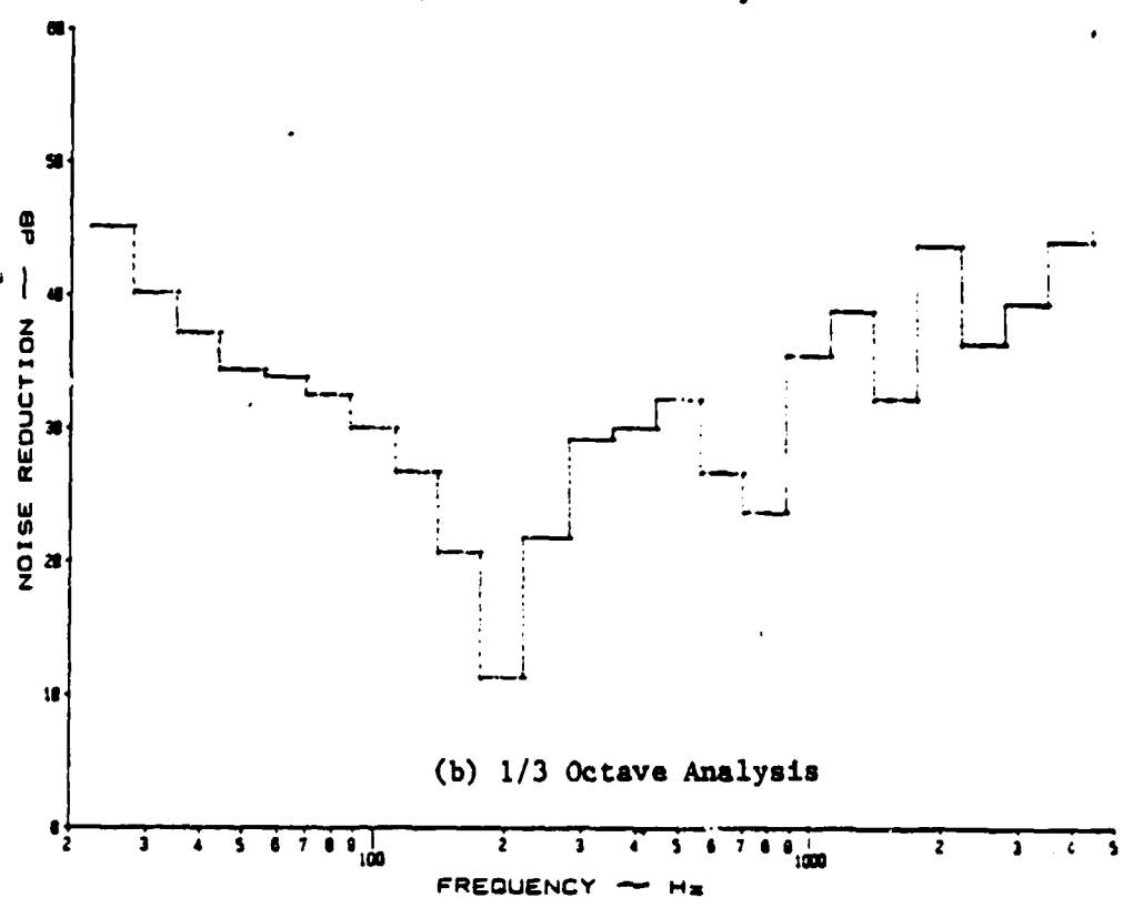
Figure A.75: Noise Reduction Characteristics of a Flat, Stiffened Panel at 2 psi Pressure Differential with Y-436 Damping Tape under a Discrete Noise Source
