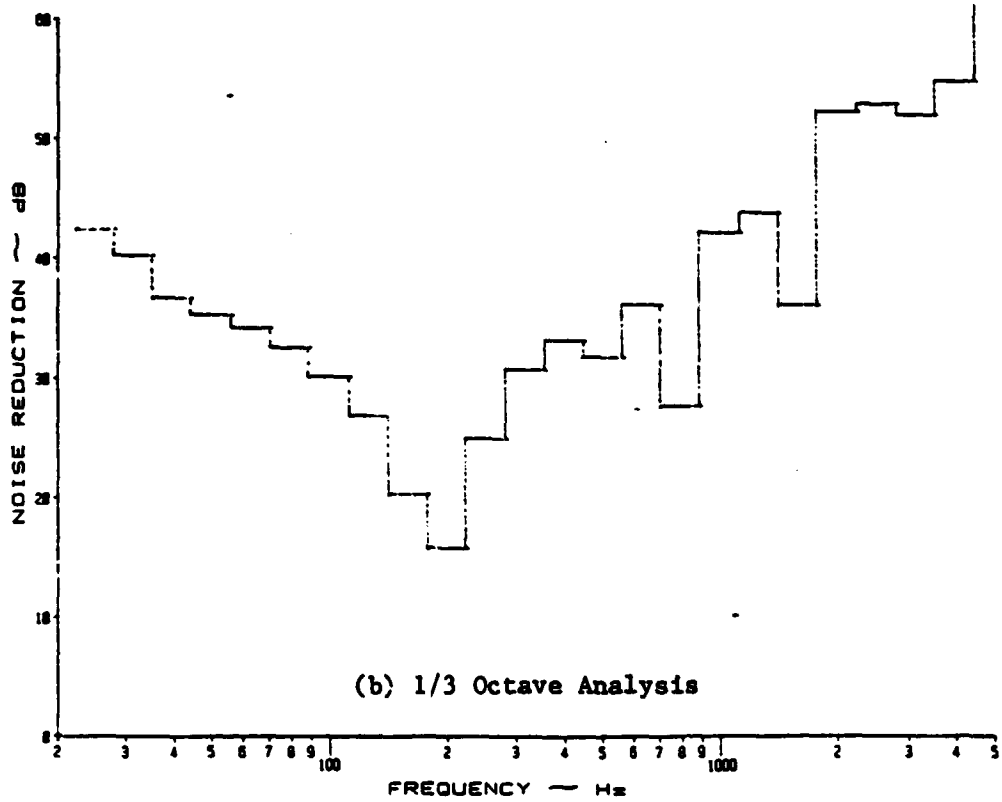
Figure A.92: Noise Reduction Characteristics of a Flat, Stiffened Panel at 3 psi Pressure Differential with Y-378 Damping Tape and 7.345 lb/ft 3 Insulation under a Discrete Noise Source
