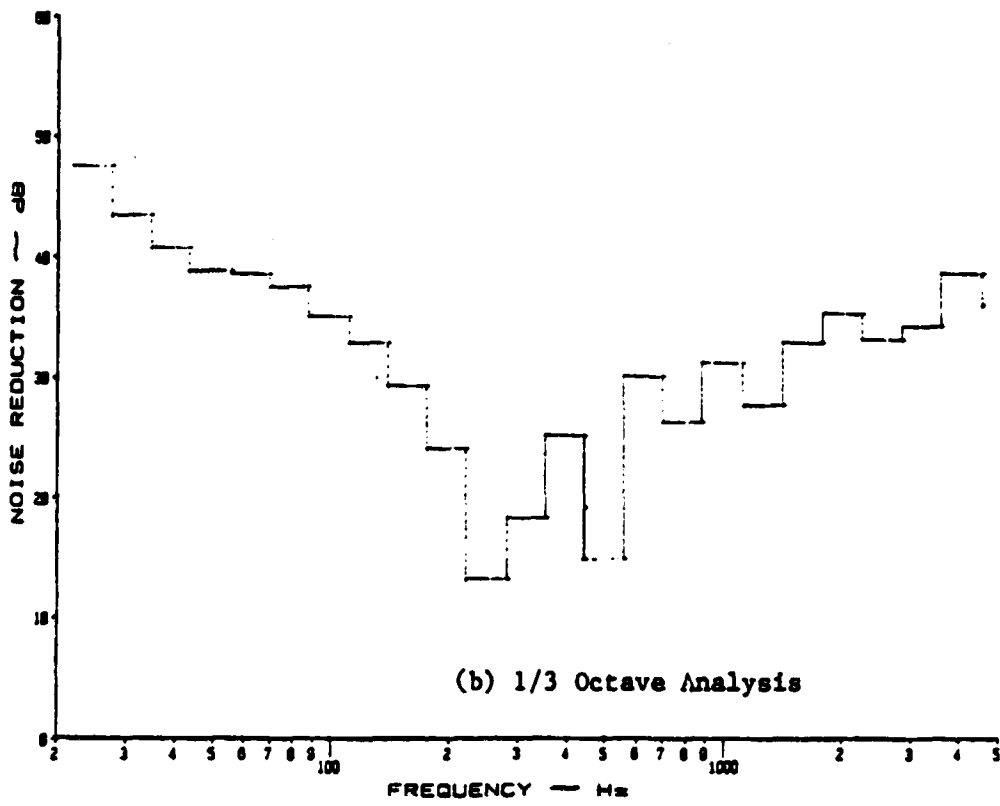
Figure B.34: Noise Reduction Characteristics of a Curved, Stiffened Panel at 1 psi Pressure Differential with Y-434 Damping Tape under a Discrete Noise Source
