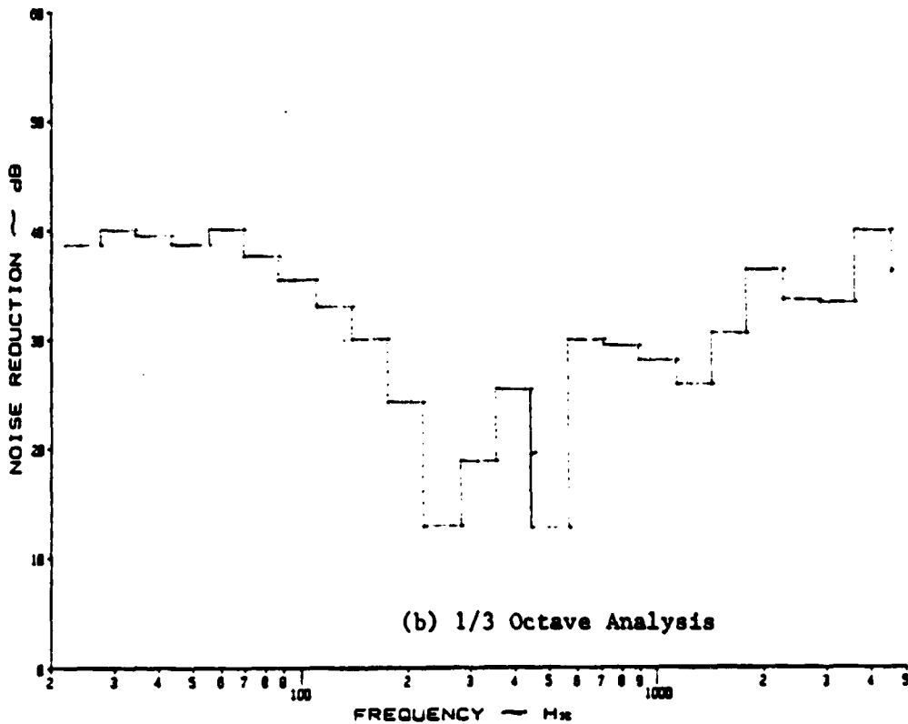
Figure B.47: Noise Reduction Characteristics of a Curved, Stiffened Panel at 2 Psi Pressure Differential with Y-434 Damping Tape under White Noise
