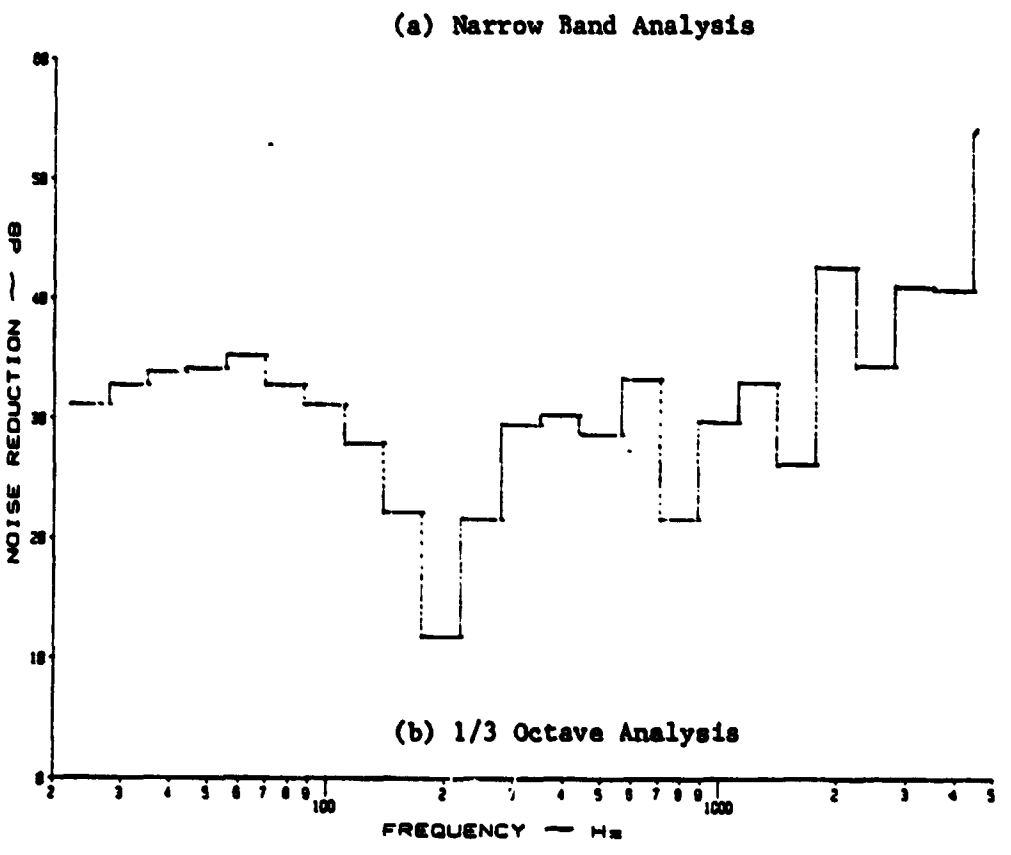
Figure A.16: Noise Reduction Characteristics of a Flat, Stiffened Panel at 3 psi Pressure Differential with Y-370 Damping Tape under White Noise
