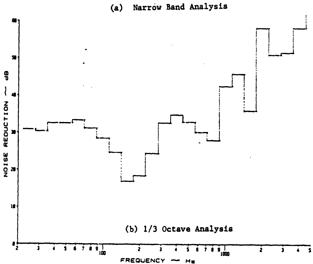
Figure A.94: Noise Reduction Characteristics of a Flat, Stiffened Panel at 1 psi Pressure Differential with Y-370 Damping Tape and 7.345 lb/ft 3 Insulation under White Noise
