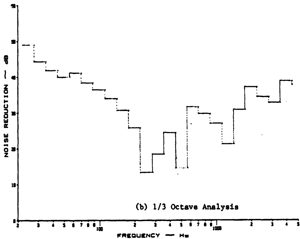
Figure B.59: Noise Reduction Characteristics of a Curved, Stiffened Panel at 2 psi Pressure Differential with Y-436 Damping Tape under a discrete noise source
