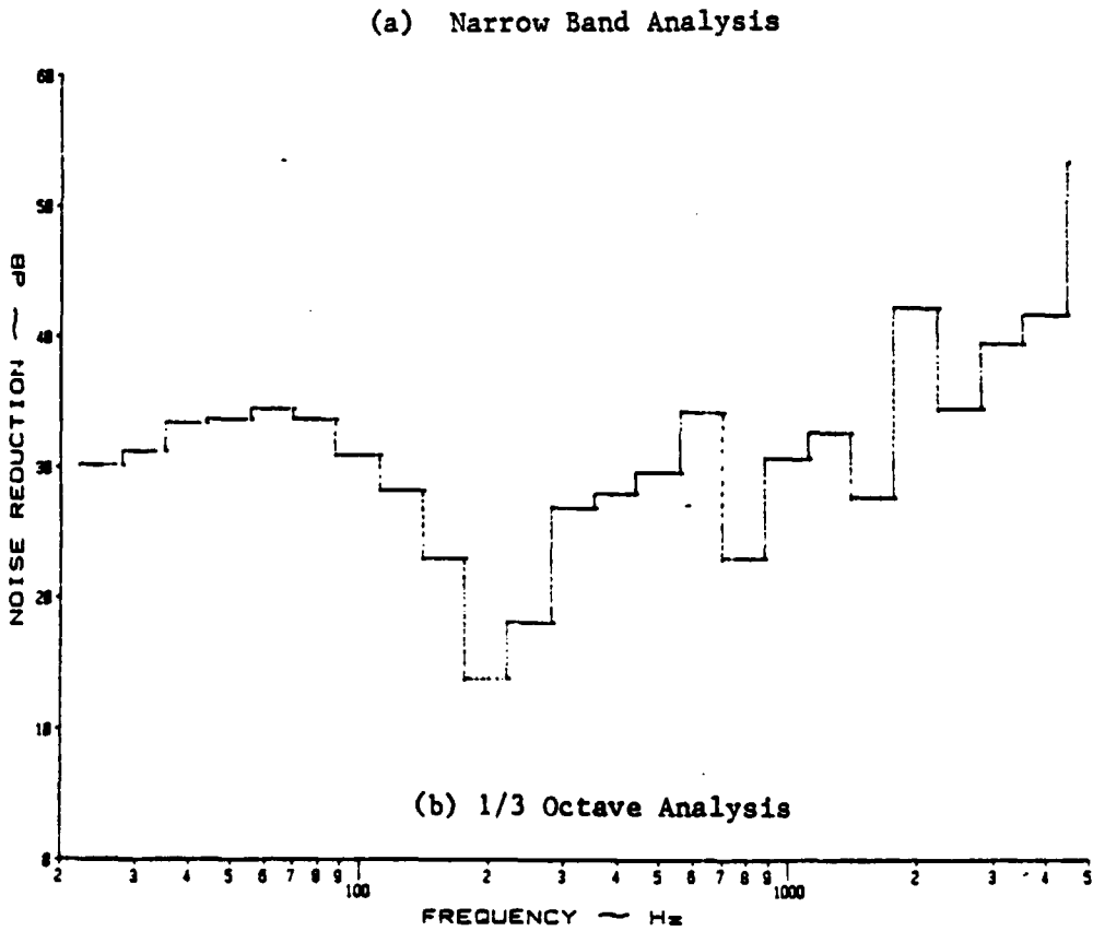
Figure A.40: Noise Reduction Characteristics of a Flat, Stiffened Panel at 3 psi Pressure Differential with Y-434 Damping Tape under White Noise
