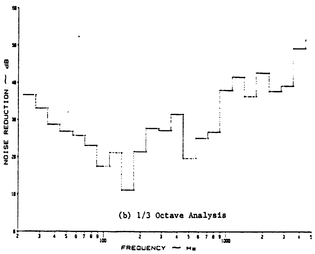
Figure A.73: Noise Reduction Characteristics of a Flat, Stiffened Panel at 0 psi Pressure Differential with Y-436 Damping Tape under a Discrete Noise Source
