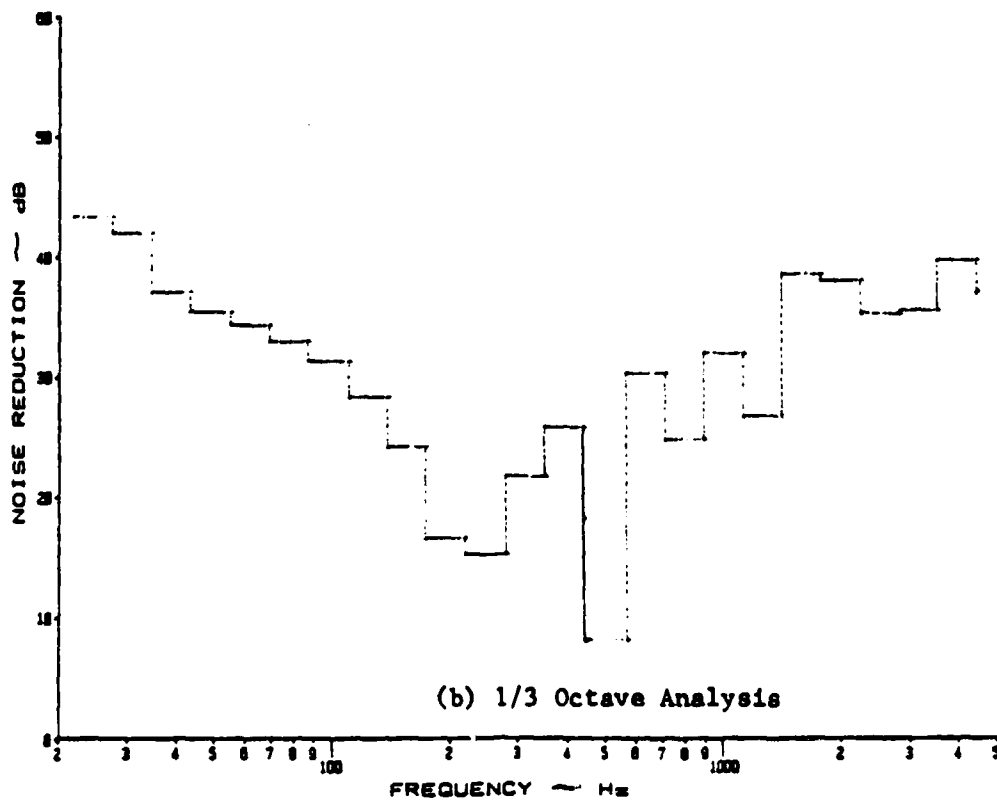
Figure B.33: Noise Reduction Characteristics of a Curved, Stiffened Panel at 0 psi Pressure Differential with Y-434 Damping Tape under a Discrete Noise Source
