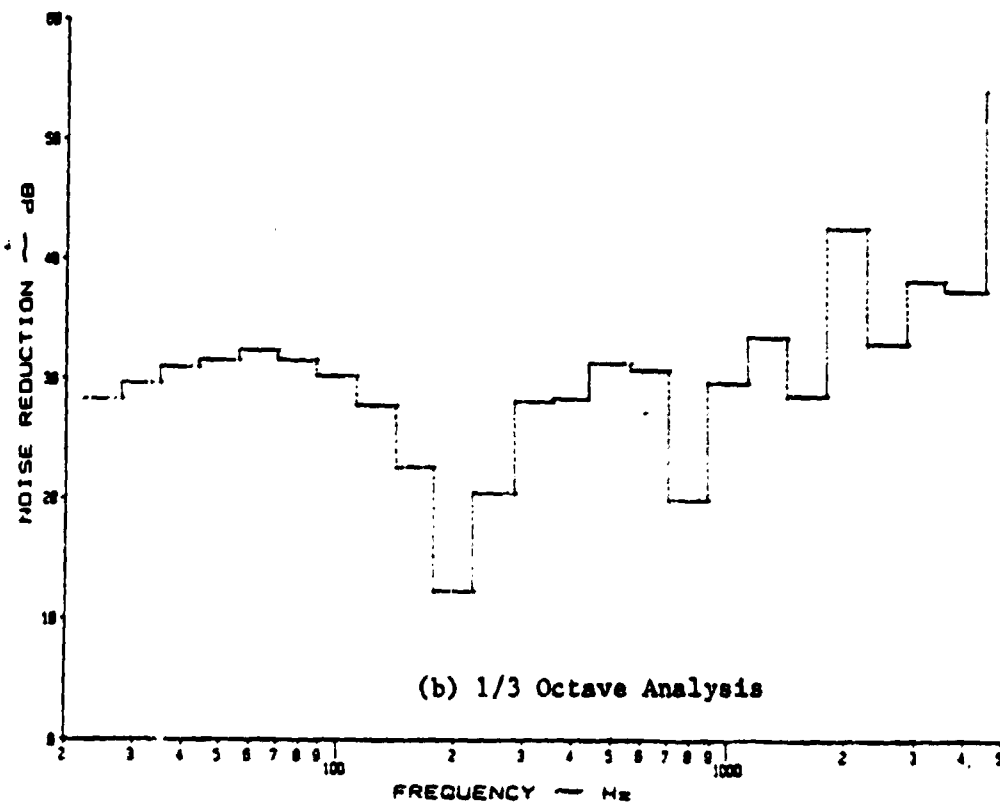
Figure A.64: Noise Reduction Characteristics of a Flat, Stiffened Panel at 3 psi Pressure Differential with Y-436 Damping Tape under White Noise
