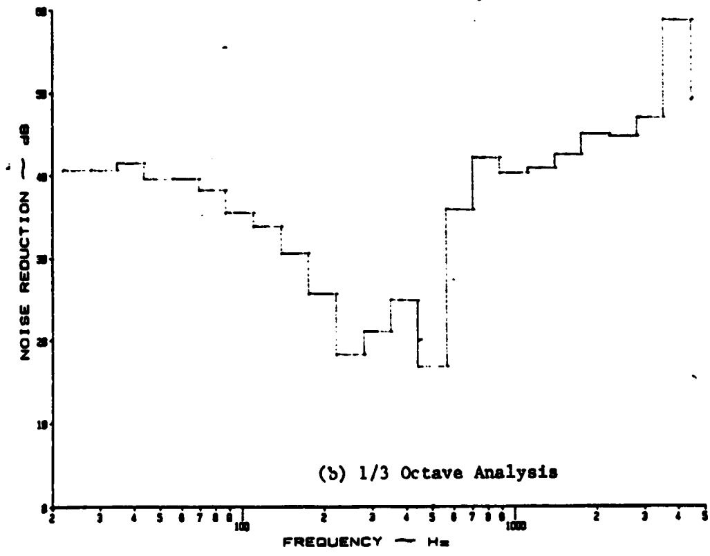
Figure B.96: Noise Reduction Characteristics of a Curved, Stiffened Panel at 3 psi Pressure Differential with Y-370 Damping Tape and 7.345 lb/ft 3 Insulation under White Noise
