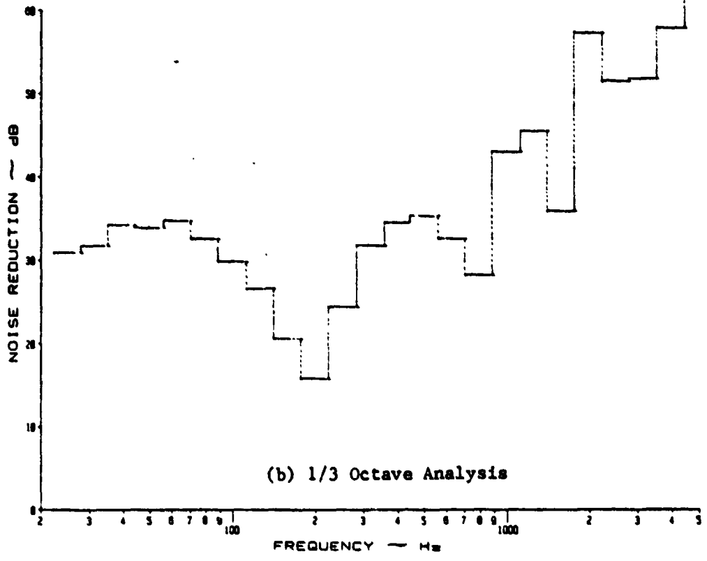
Figure A.96: Noise Reduction Characteristics of a Flat, Stiffened Panel at 3 psi Pressure Differential with Y-370 Damping Tape and 7.345 lb/ft 3 Insulation under White Noise
