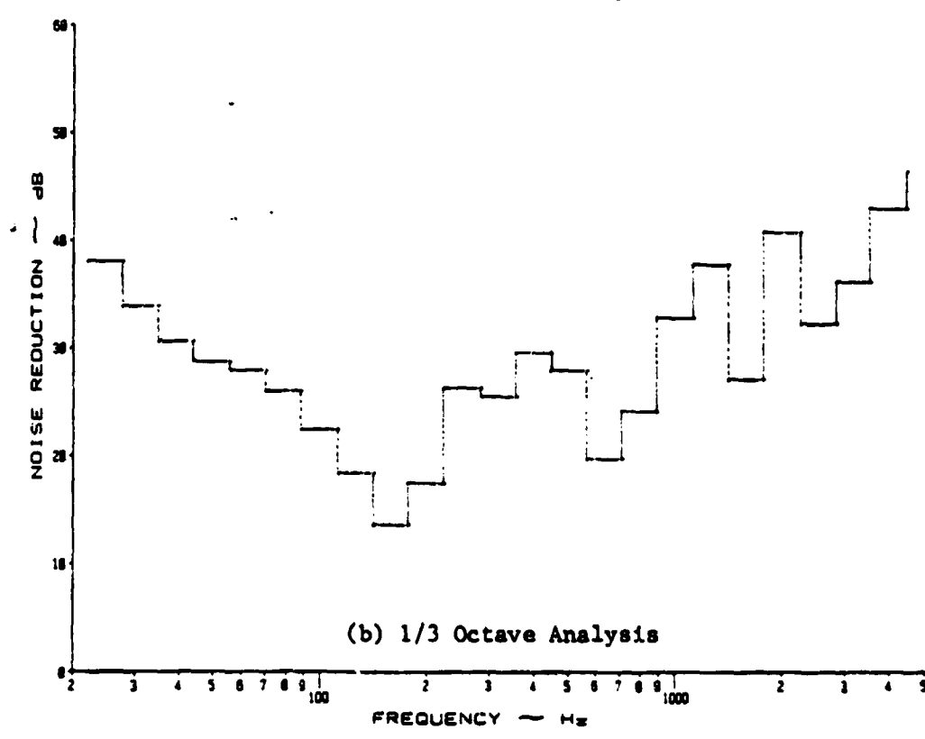
Figure A.33: Noise Reduction Characteristics of a Flat, Stiffened Panel at 0 psi Pressure Differential with Y-434 Damping Tape under a Discrete Noise Source
