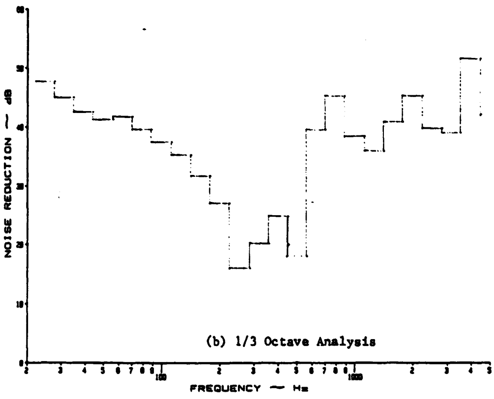
Figure B.84: Noise Reduction Characteristics of a Curved, Stiffened Panel at 3 psi Pressure Differential with Y-370 Damping Tape and 0.817 lb/ft 3 Insulation under a Discrete Noise Source
