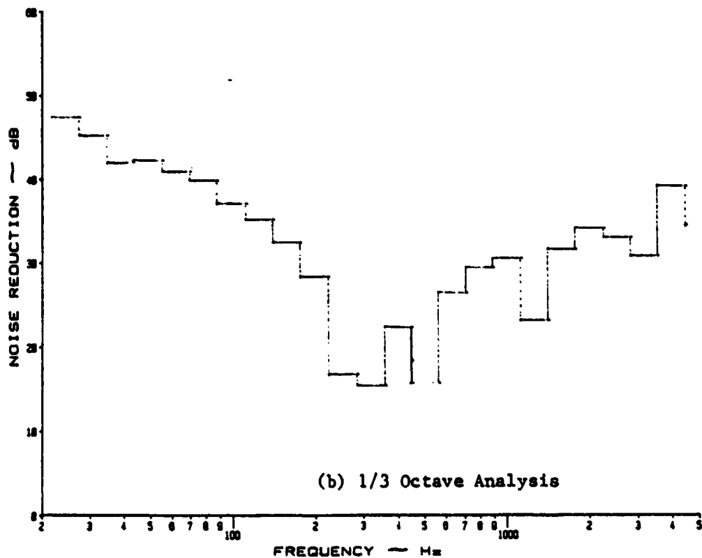
Figure B.12: Noise Reduction Characteristics of a Curved, Stiffened Panel at 3 psi Pressure Differential with Y-370 Damping Tape under a Discrete Noise Source
