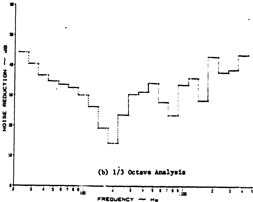
Figure A.19: Noise Reduction Characteristics of a Flat, Stiffened Panel at 2 psi Pressure Differential with Y-370 Damping Tape under a Discrete Noise Source
