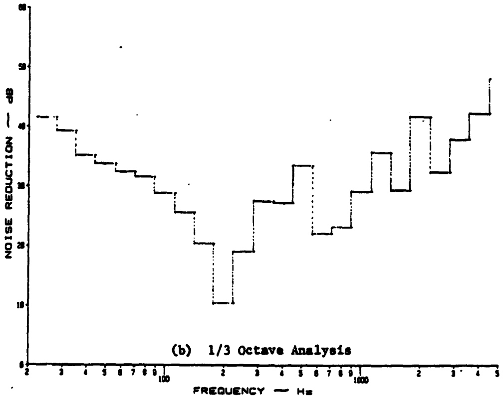
Figure A.2: Noise Reduction Characteristics of a Flat, Stiffened Panel at 1 psi Pressure Differential with No Treatment under a Discrete Noise Source
