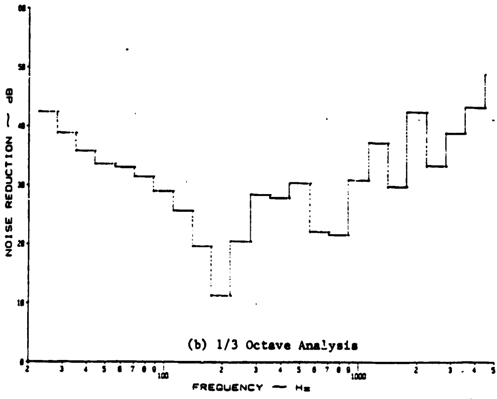
Figure A.34: Noise Reduction Characteristics of a Flat, Stiffened Panel at 1 psi Pressure Differential with Y-434 Damping Tape under a Discrete Noise Source
