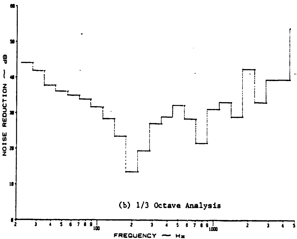
Figure A.44: Noise Reduction Characteristics of a Flat, Stiffened Panel at 3 psi Pressure Differential with Y-434 Damping Tape under a Discrete Noise Source
