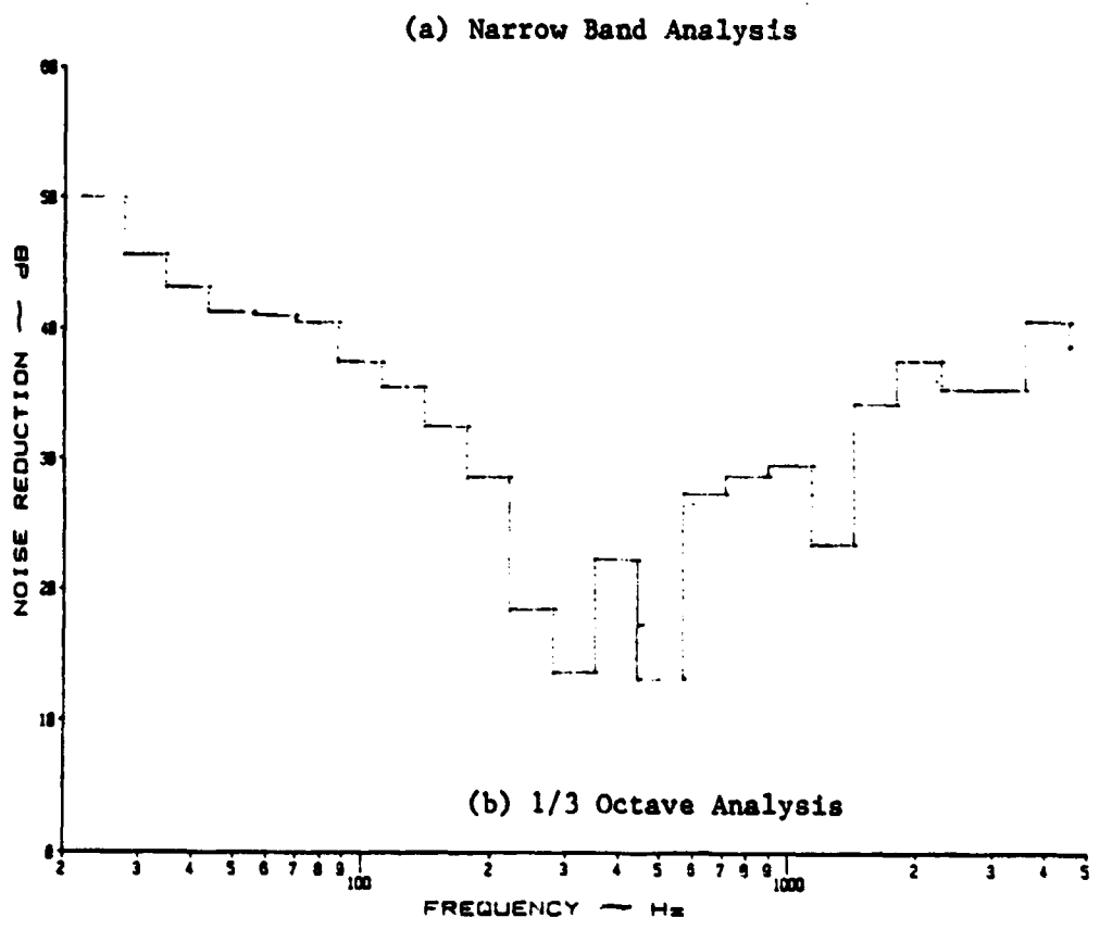
Figure B.52: Noise Reduction Characteristics of a Curved, Stiffened Panel at 3 psi Pressure Differential with Y-434 Damping Tape under a Discrete Noise Source
