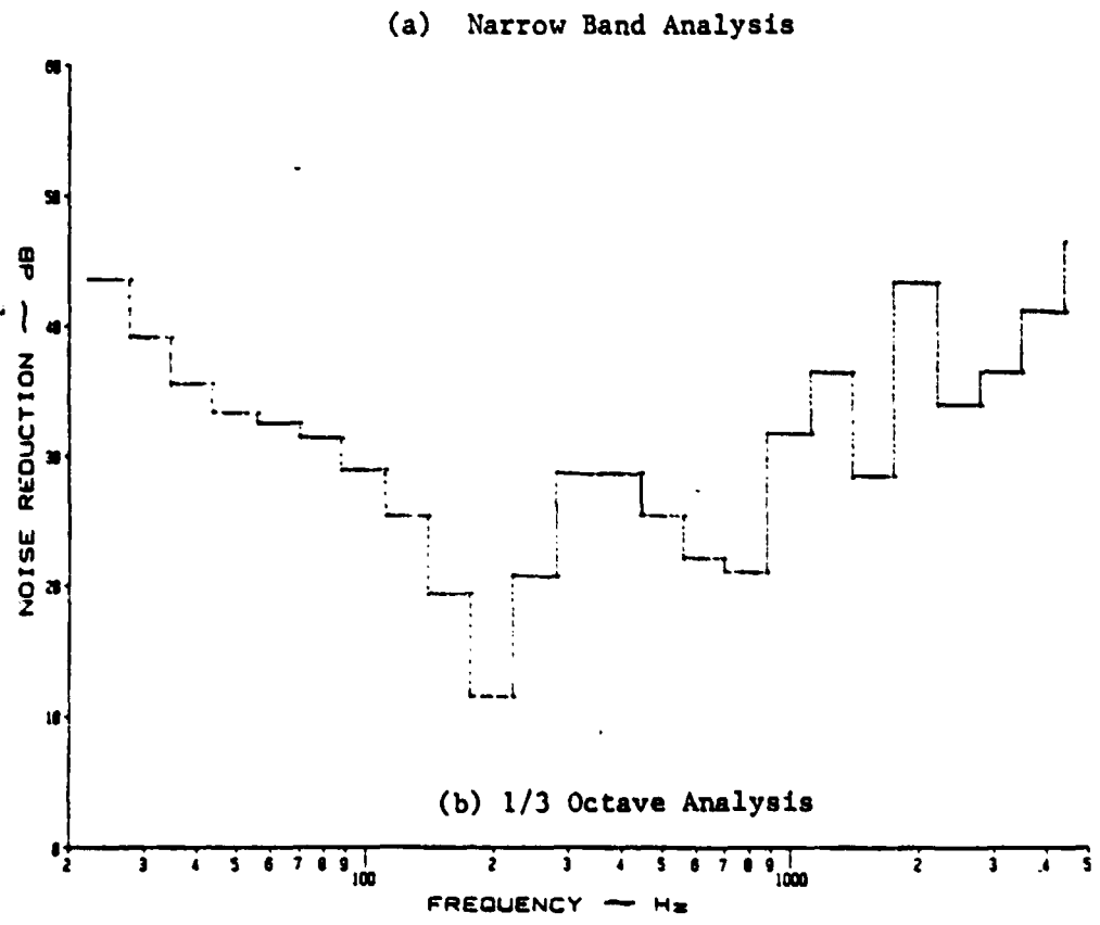
Figure A.42: Noise Reduction Characteristics of a Flat, Stiffened Panel at 1 psi Pressure Differential with Y-434 Damping Tape under a Discrete Noise Source
