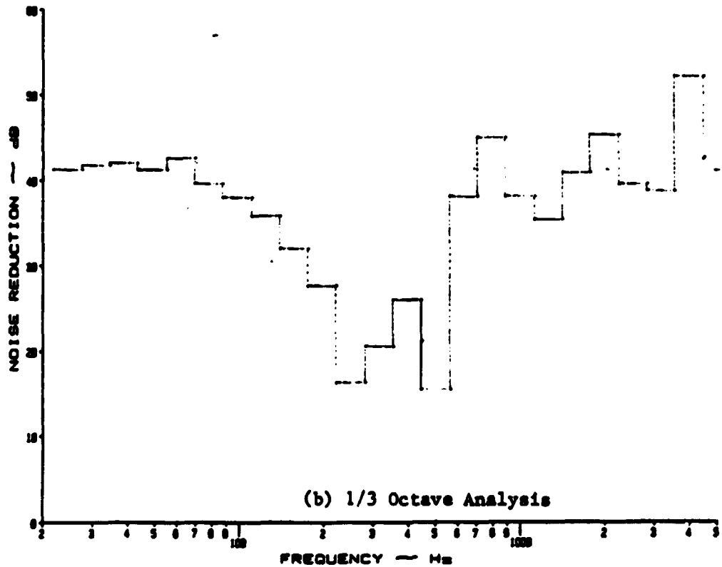
Figure B.88: Noise Reduction Characteristics of a Curved, Stiffened Panel at 3 psi Pressure Differential with Y-370 Damping Tape and 0.817 lb/ft 3 Insulation under White Noise
