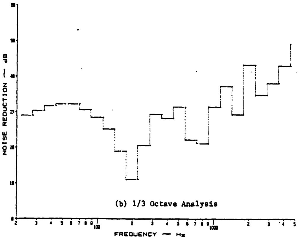
Figure A.46: Noise Reduction Characteristics of a Flat, Stiffened Panel at 1 psi Pressure Differential with Y-434 Damping Tape under White Noise
