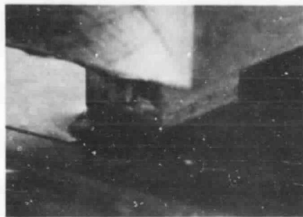
(b) Nucleate boiling off tool trailing edge, Trichloroethane at 600 MPa.
