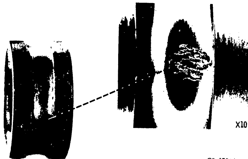
Figure 1. - Typical fatigue spall in bearing race.
