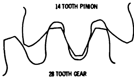
Figure 3. - Unequal addenda mesh geometry.
