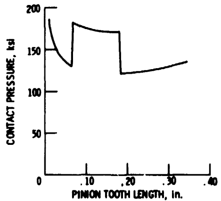
Figure 6. - Optimal design Hertzian contact pressure.
