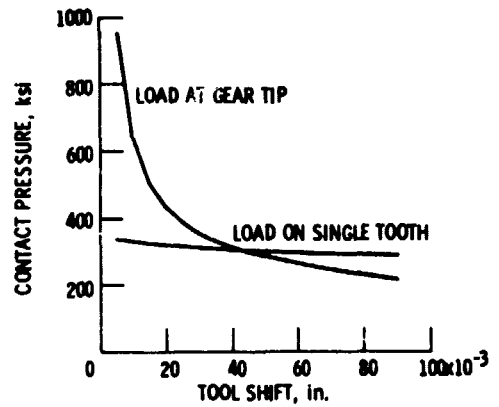
Figure 5. - Hertzian contact pressure comparison.
