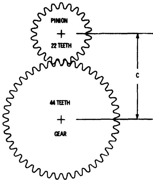
Figure 1. - Standard gear mesh.
