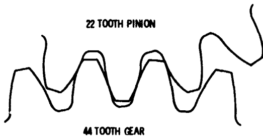
Figure 2. - Standard involute mesh geometry.
