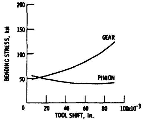
Figure 4. - Tooth bending stress comparison.
