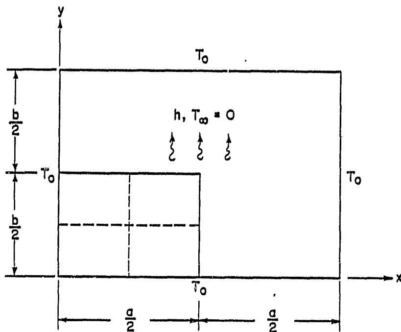
(a) PLATE COOLED BY SURFACE CONVECTION
