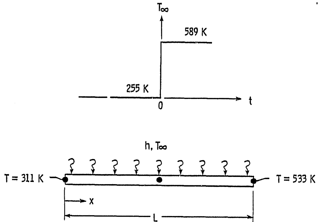
(a) Rod heated by surface convection.
