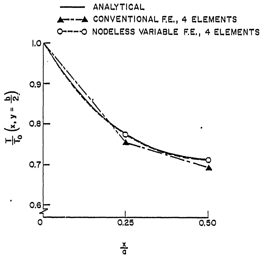
(c) COMPARATIVE TEMPERATURE DISTRIBUTIONS ALONG y = \frac{b}{2} .
