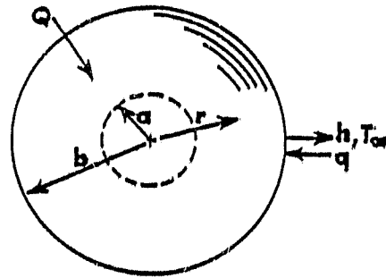
Case 4, HOLLOW SPHERE,
