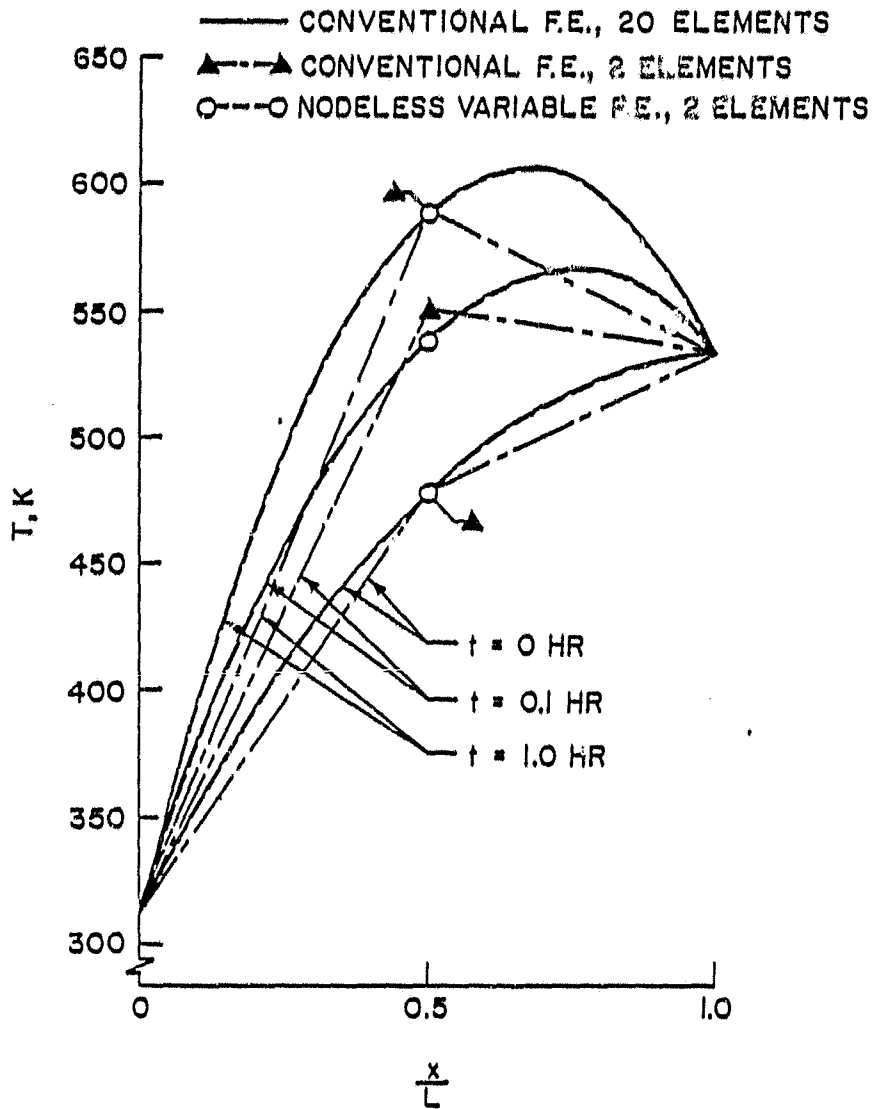
(b) COMPARATIVE TEMPERATURE DISTRIBUTIONS
