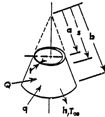
Case 6, CONICAL SHELL
