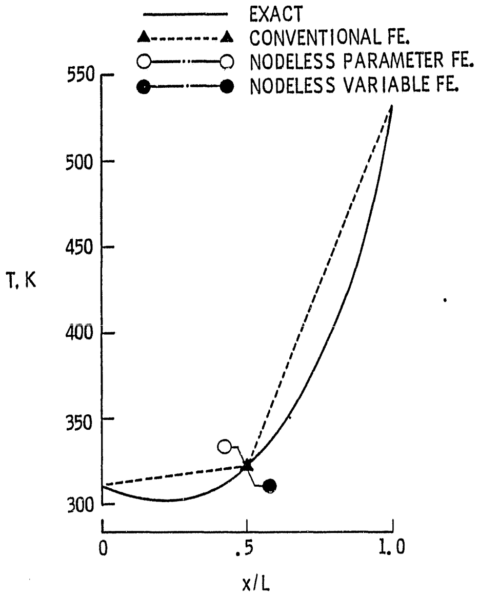
(b) Comparative temperature distributions at t = 0 s.
