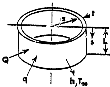
Case 5, CYLINDRICAL SHELL
