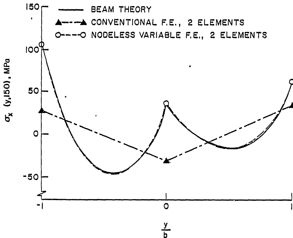
(c) COMPARATIVE THERMAL STRESS DISTRIBUTIONS ALONG CHORDWISE DIRECTION, t = 150 s.
