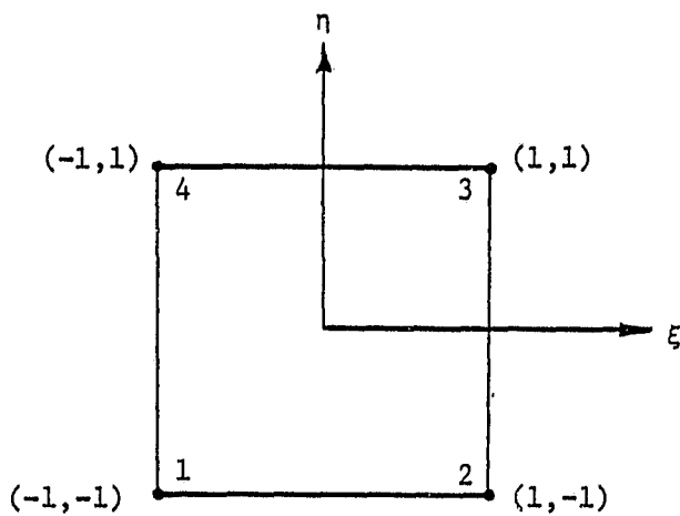
(b) Natural coordinates
