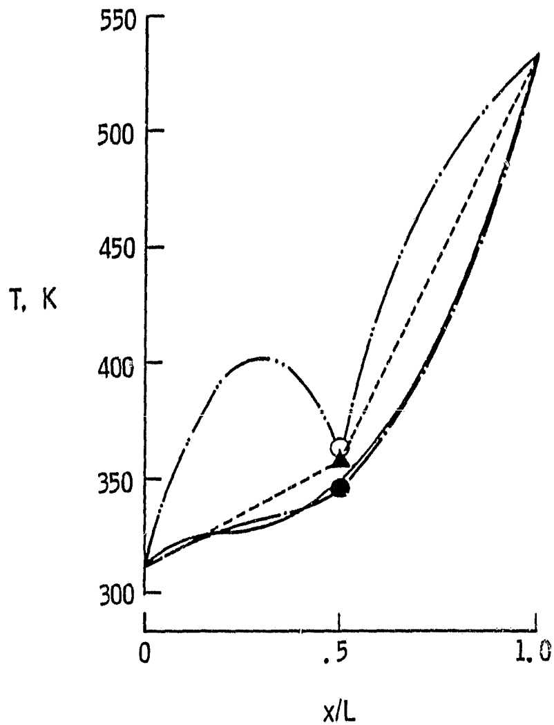
(c) Comparative temperature distributions at t = .01 s.
