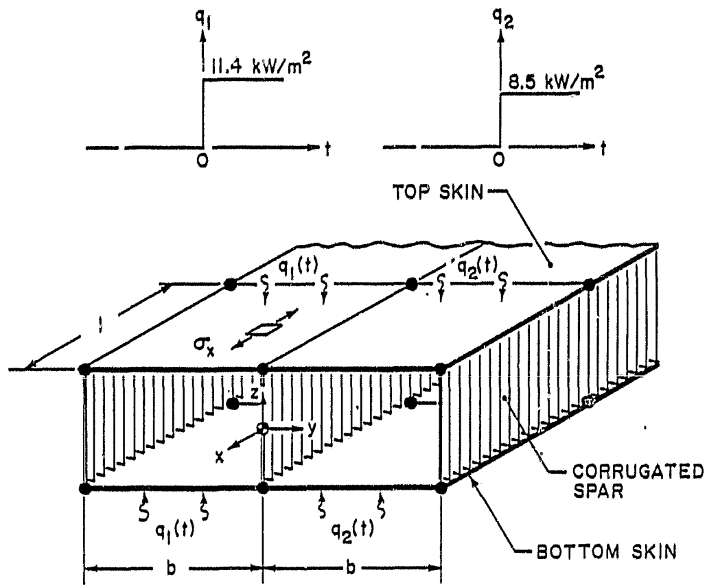
(a) SIMPLIFIED WING SECTION WITH AERODYNAMIC HEATING
