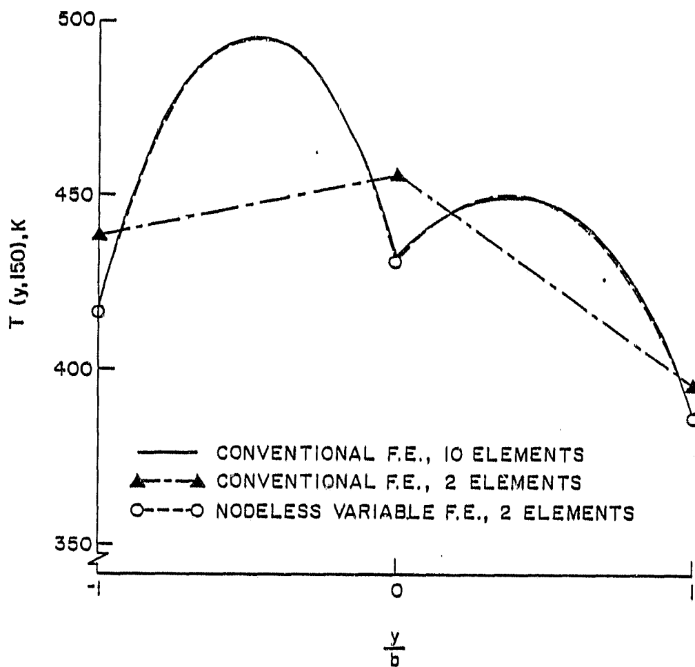
(b) COMPARATIVE TEMPERATURE DISTRIBUTIONS ALONG CHORDWISE DIRECTION, t = 150 s.
