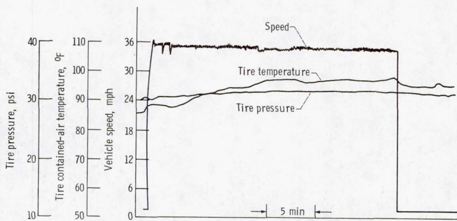
Figure 4. - Sample test record taken during 56-km/h (35-mph) constant-speed tests. (Temperature trace was copied from another record.)
