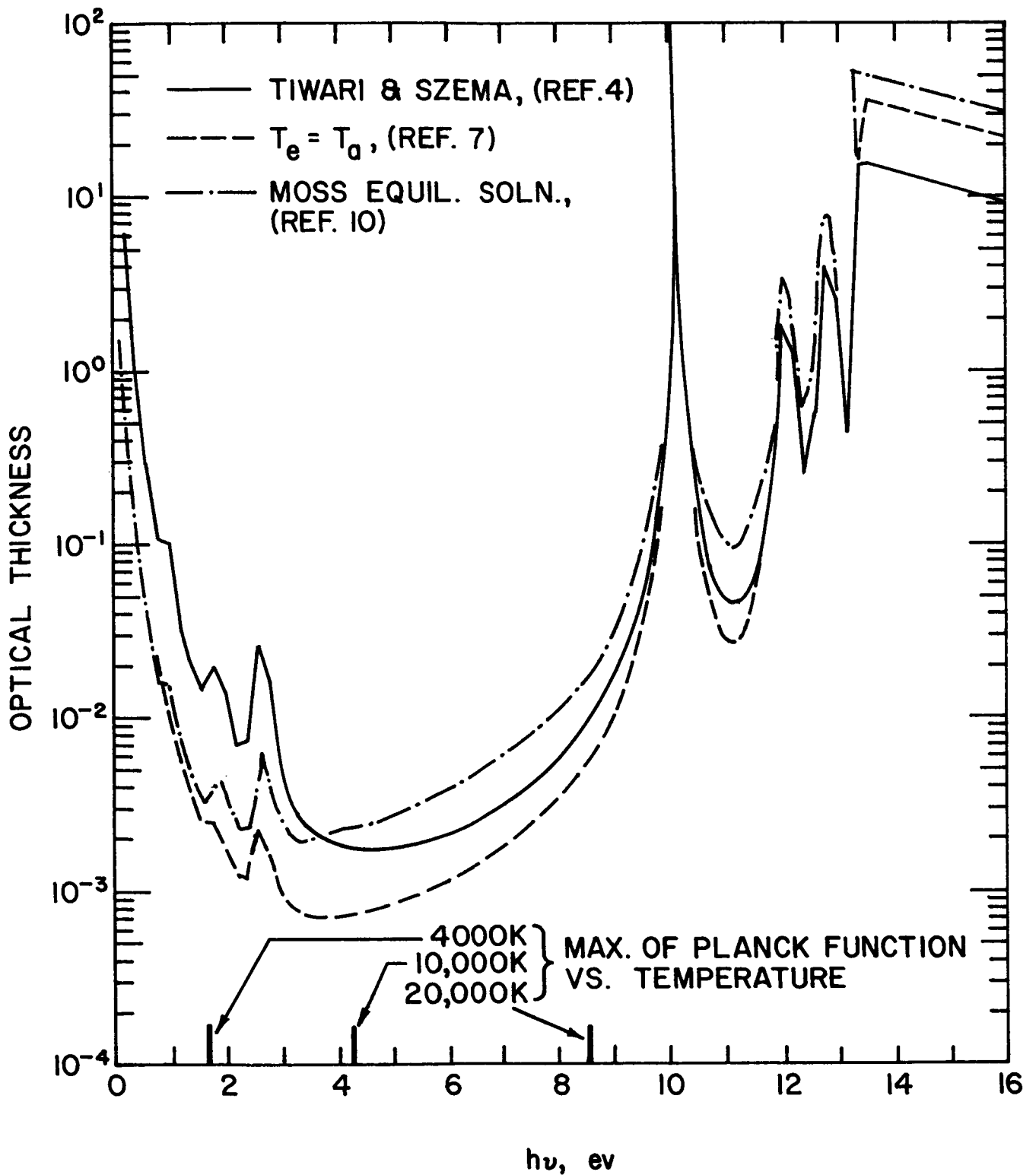
Figure 6. Optical Thickness of the Stagnation Shock Layer as a Function of Radiation Energy.
