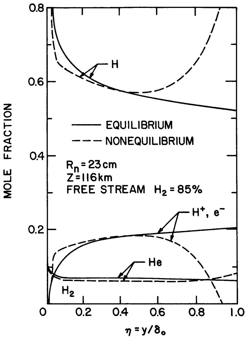
Figure 5. Species Mole Fraction Variation as a Function of Nondimensional Position across the Stagnation Shock Layer. (From Ref. 4)
