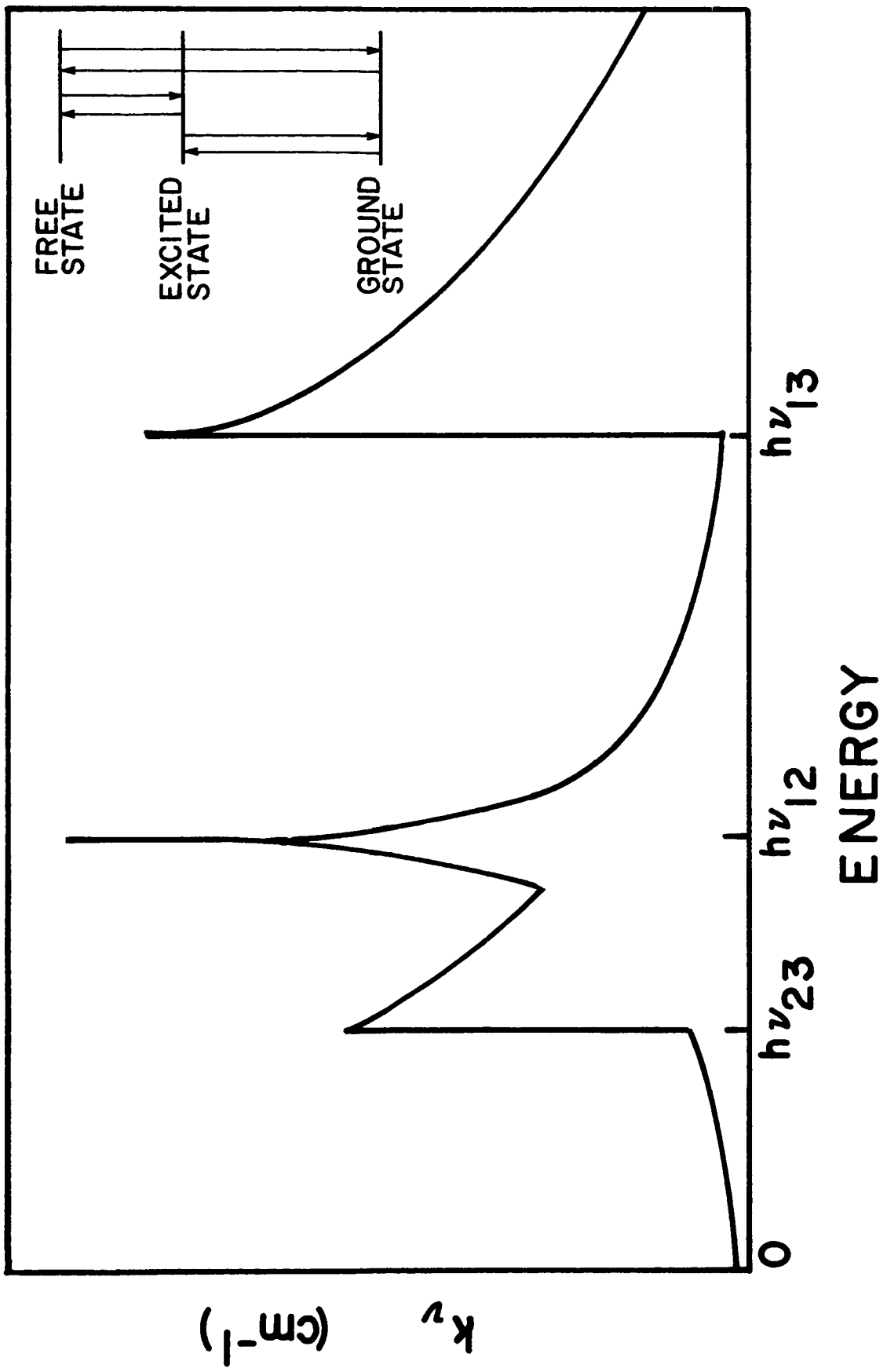
Figure 2. Schematic of the Radiation Absorption Coefficient for a Two-Level Atomic Gas.
