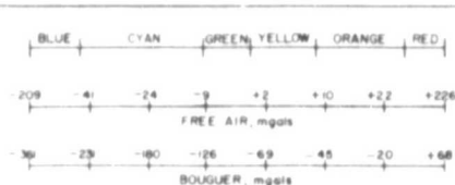
Fig. 4 This diagram shows the approximate color-coding scheme used to produce the color contours for the gravity anomaly maps shown on the cover of this issue of Eos . Histograms showing the fractional area occupied by each anomaly value were used to assign colors in such a manner that each color value occupies an area comparable to any other color value. About 45 discrete color values (i.e., discrete hue and saturation values) were used in each anomaly map. On the other hand, the shaded relief map versions of the anomalies each contain 256 shades of gray.
