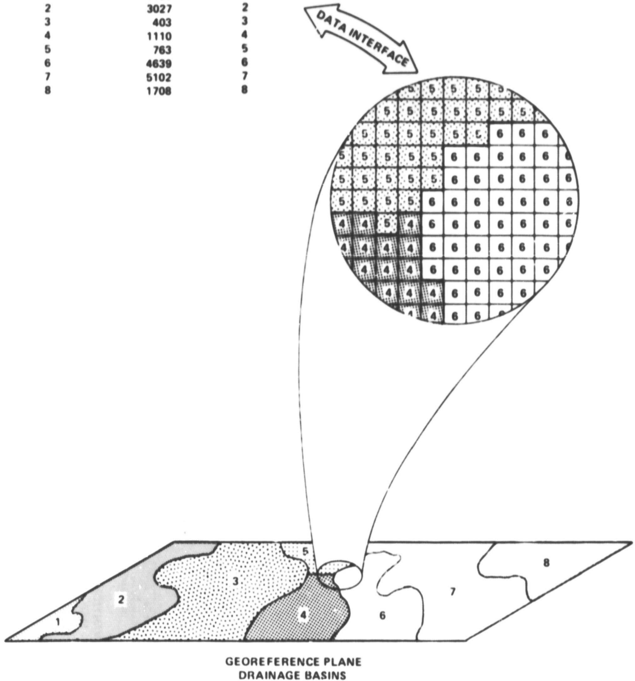
Figure II-20. Conceptual drawing of the georeference plane and tabular interface file
