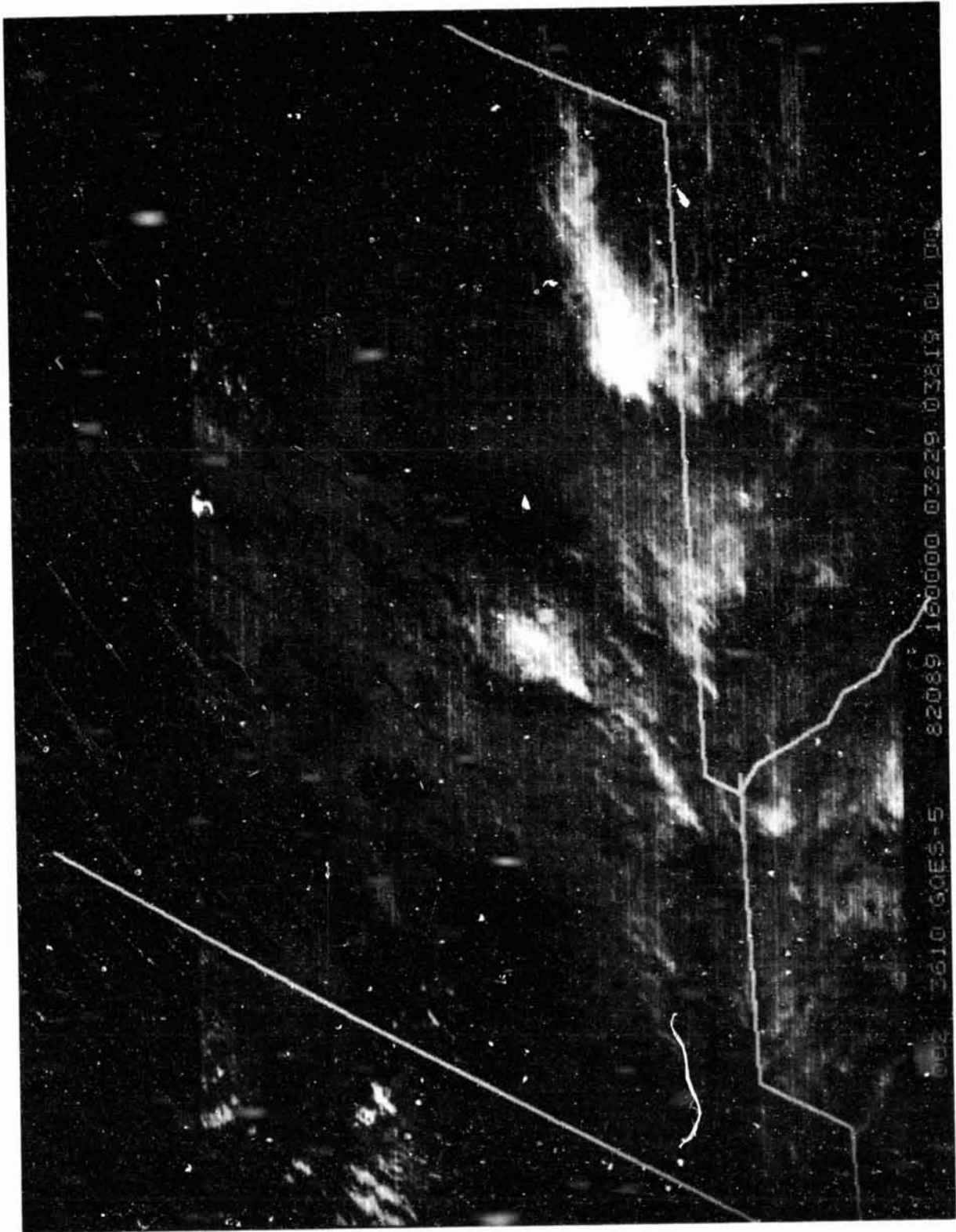
Figure 9. Visible GOES-W satellite image at 1600 GMT March 30, 1982 over southern New Mexico.
