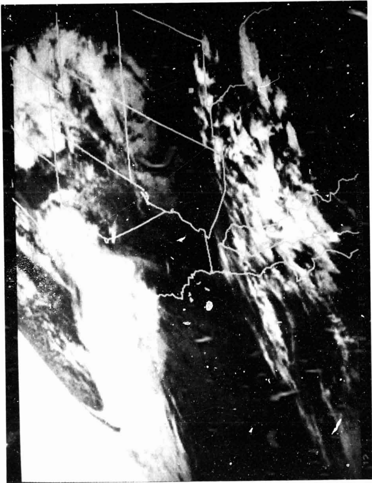
Figure 3. GOES-W infrared satellite image at 1600 GMT March 30, 1982.
