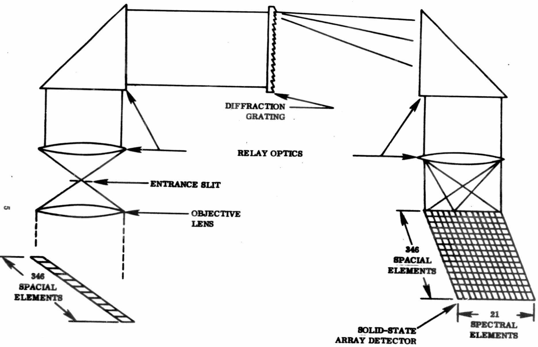
Figure 2. Solid-state Array Spectroradiometer Optics Concept.
