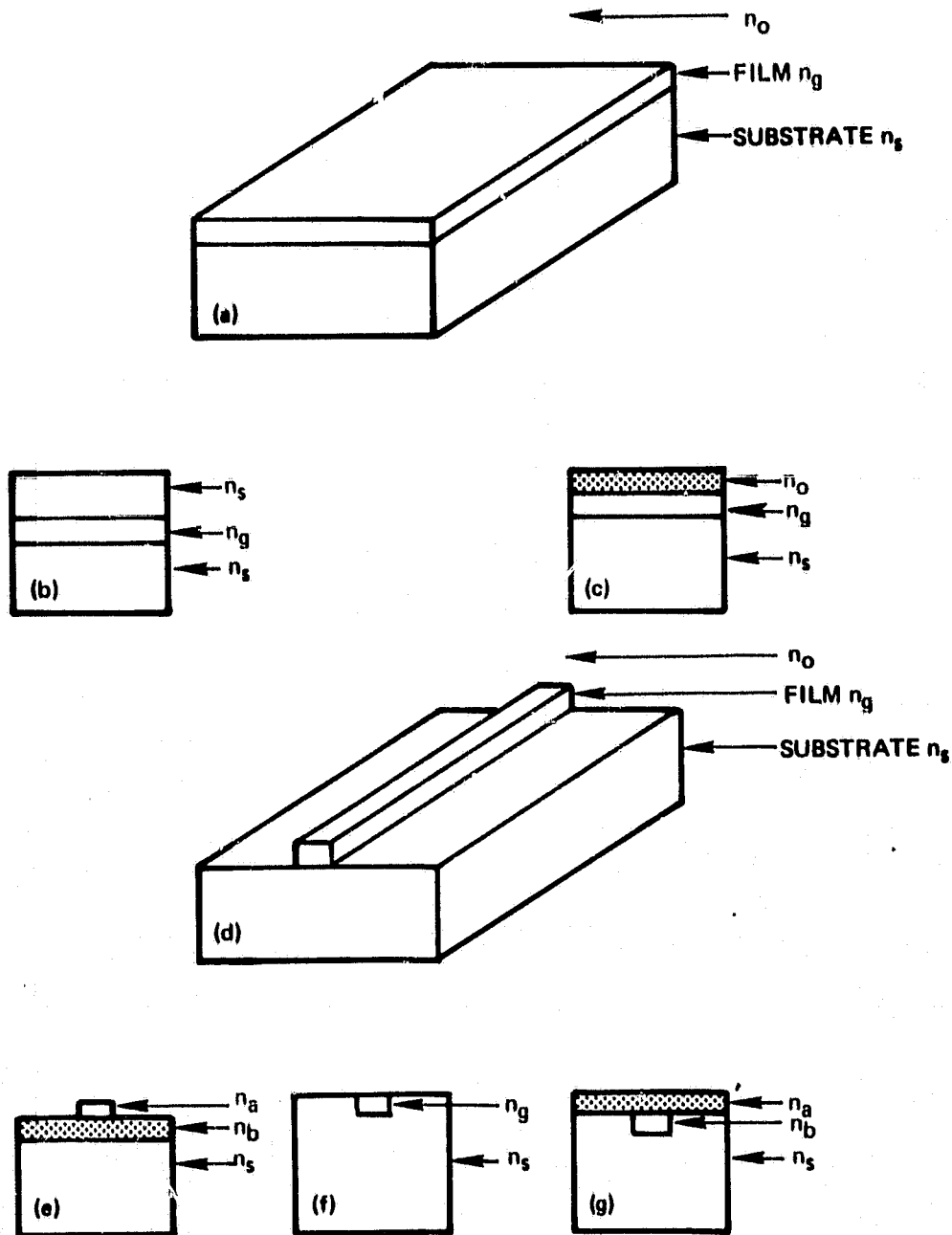
Figure 3-1. Various Waveguide Structures
