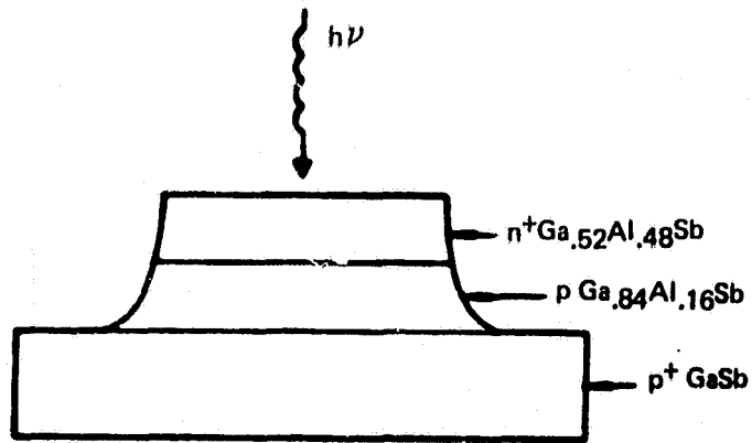
Figure 9-3. (a) Structure of the GaAlSb diode for electron injection; (b) structure of the GaAlSb diode for hole injection.
