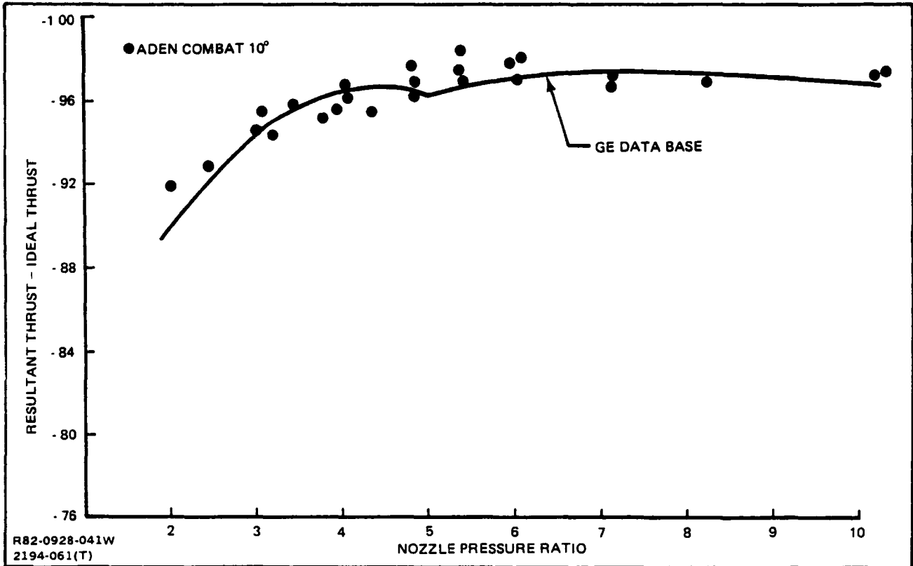
Fig. 6-14 Nozzle Balance Resultant Thrust Comparison with GE Data Base
