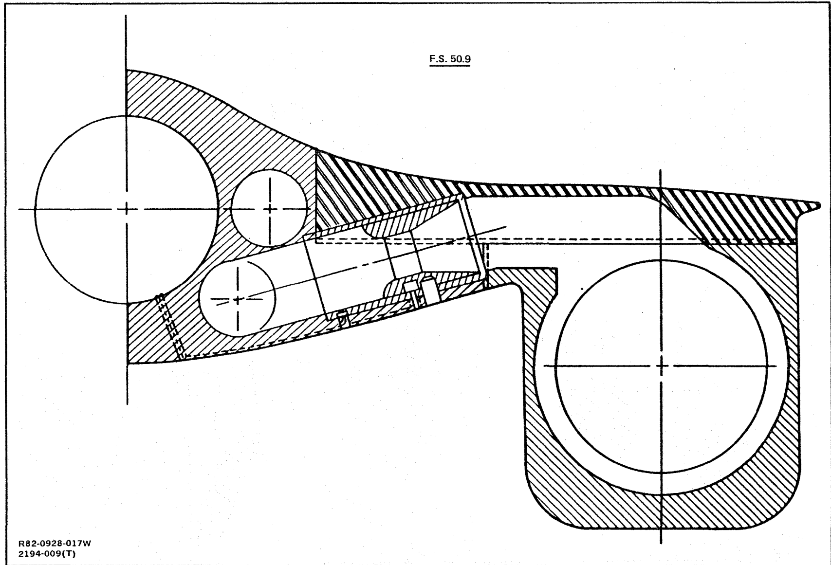
Fig. 2-6 Model Venturi Installation
