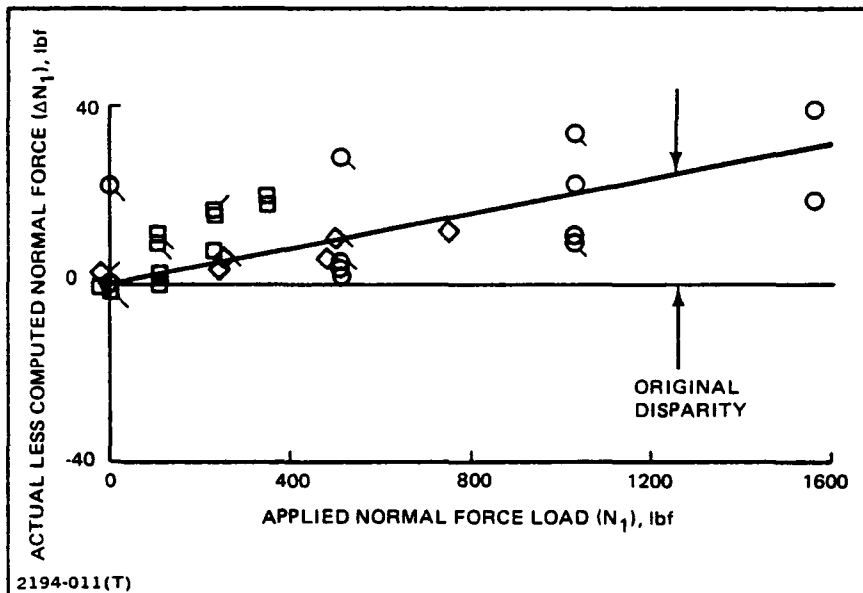
Fig. 4-2 Installed Main Balance Check Loading
