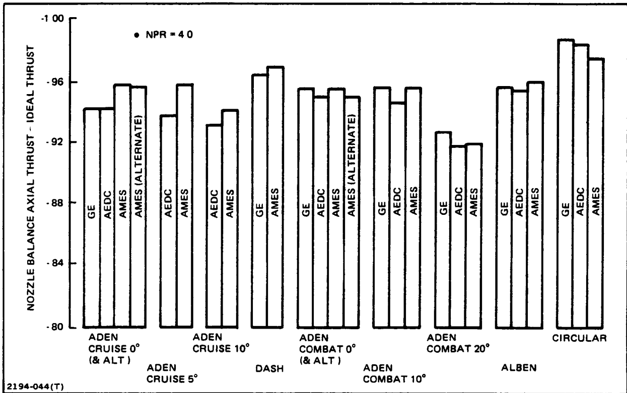
Fig. 6-6 Nozzle Balance Thrust Comparison at NPR = 4.0
