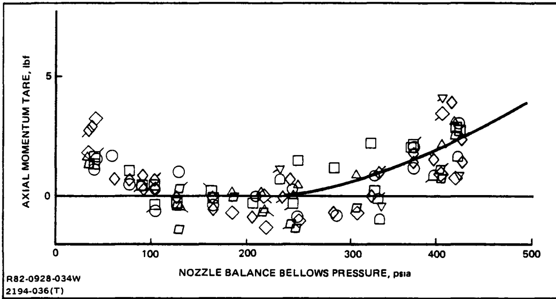
Fig. 5-13 Nozzle Balance Axial Momentum Tare Calibration
