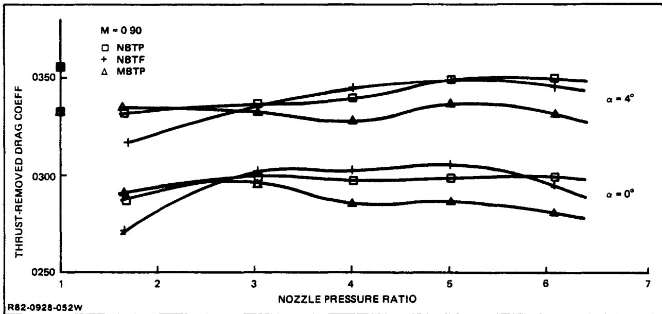
Fig. 6-31 ADEN Cruise 0° Drag Comparison
