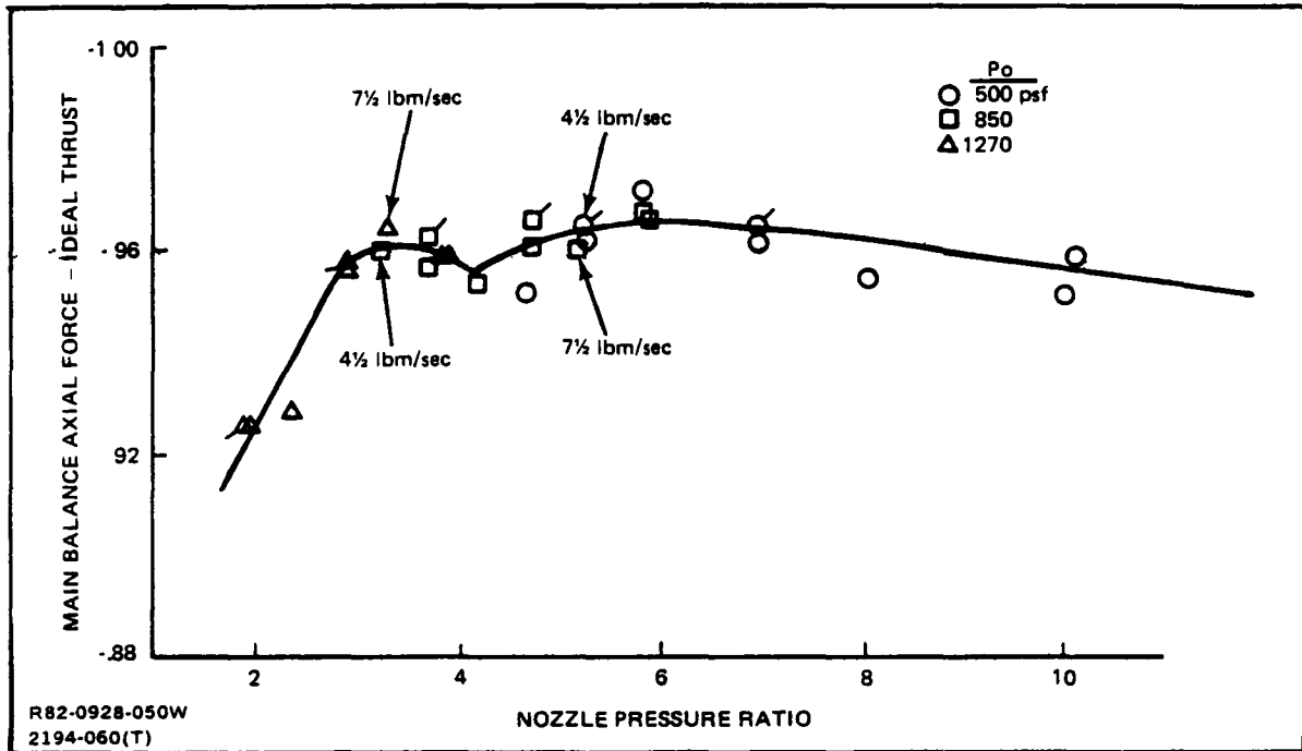
Fig. 6-23 Momentum Tare Diagnostic For Main Balance Shift
