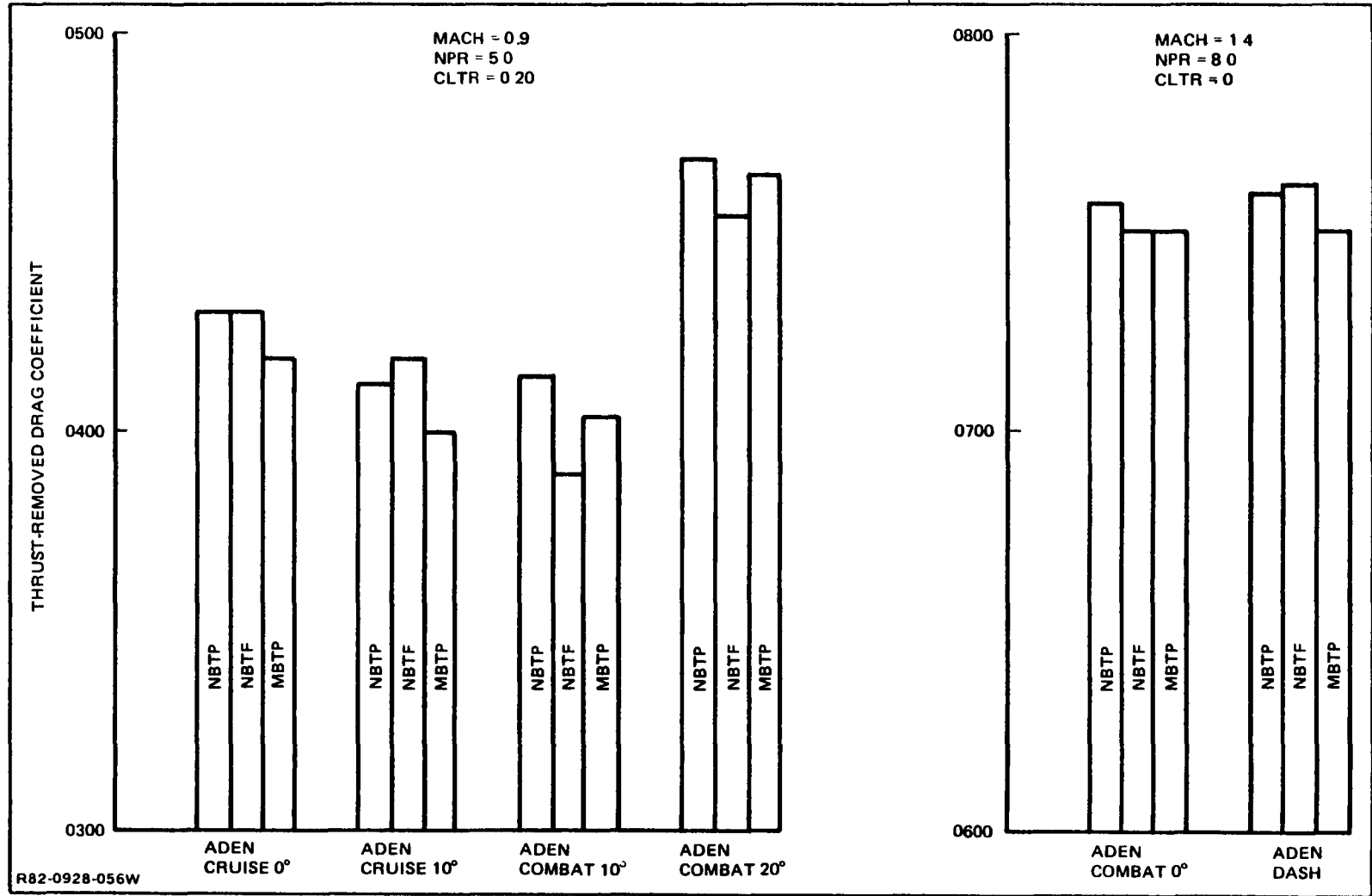
Fig. 6-35 Comparison of Data Reduction Methods
