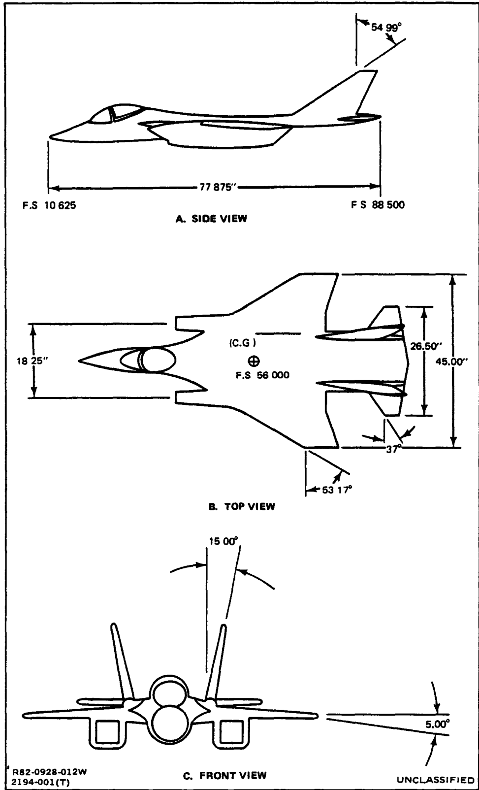
Fig. 2-1 Navy V/STOL High-Speed Model 623-20048
