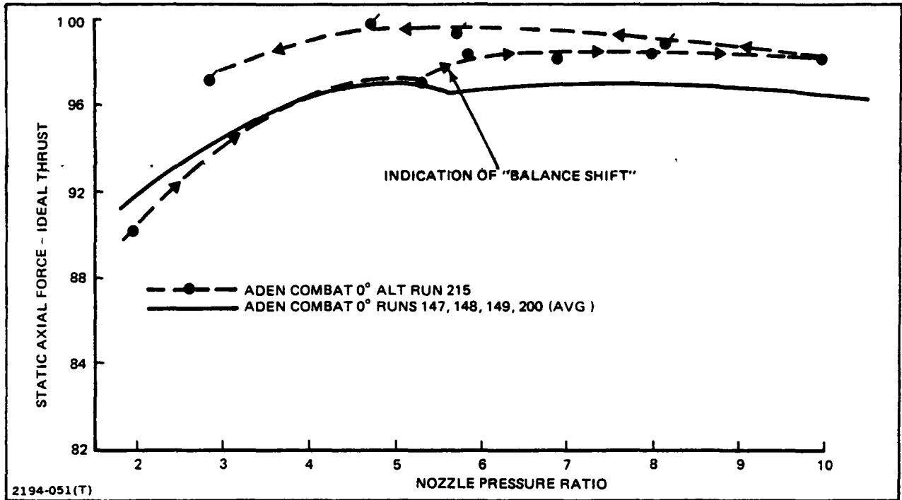
Fig. 6-13 Inception of Main Balance Shift
