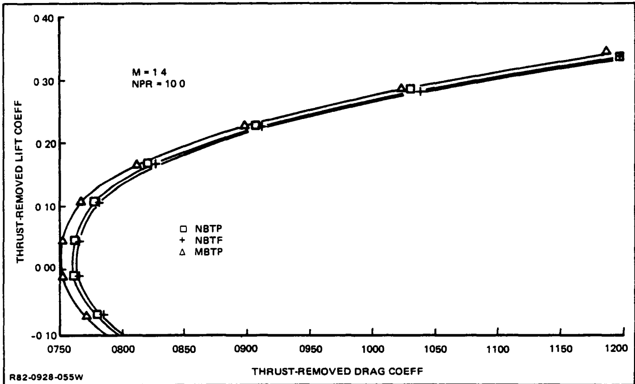
Fig. 6-34 ADEN Dash Polar Comparison
