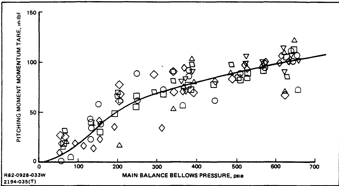
Fig. 5-12 Main Balance Pitching Moment Momentum Tare Calibration
