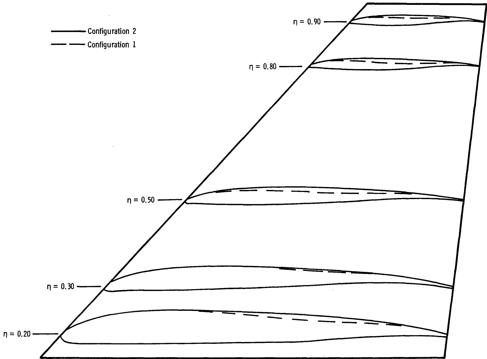
Figure 5.- Comparison of wing airfoils for configurations 1 and 2.
