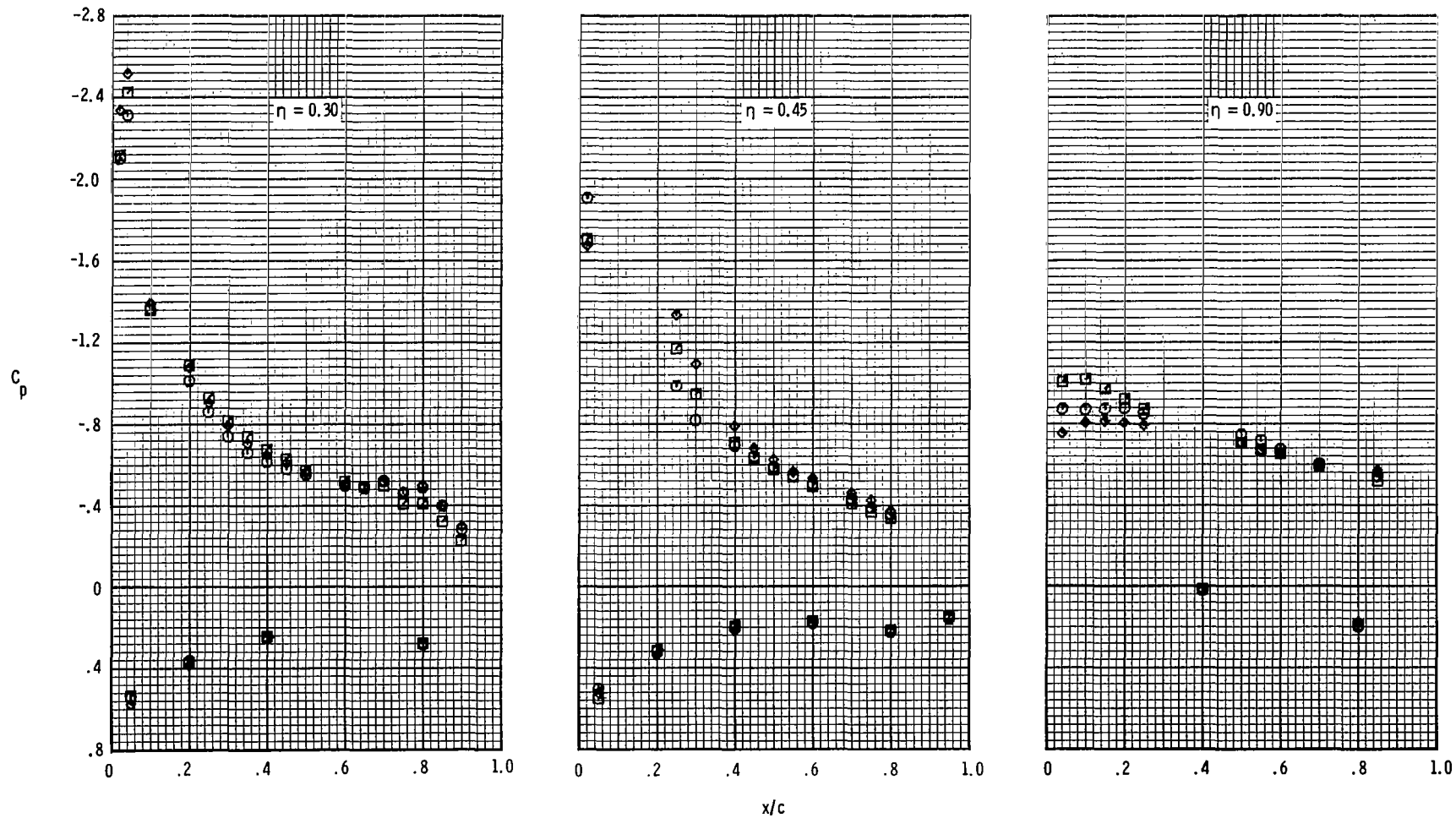
(a) M = 0.60 ; \alpha \approx 16^\circ .
