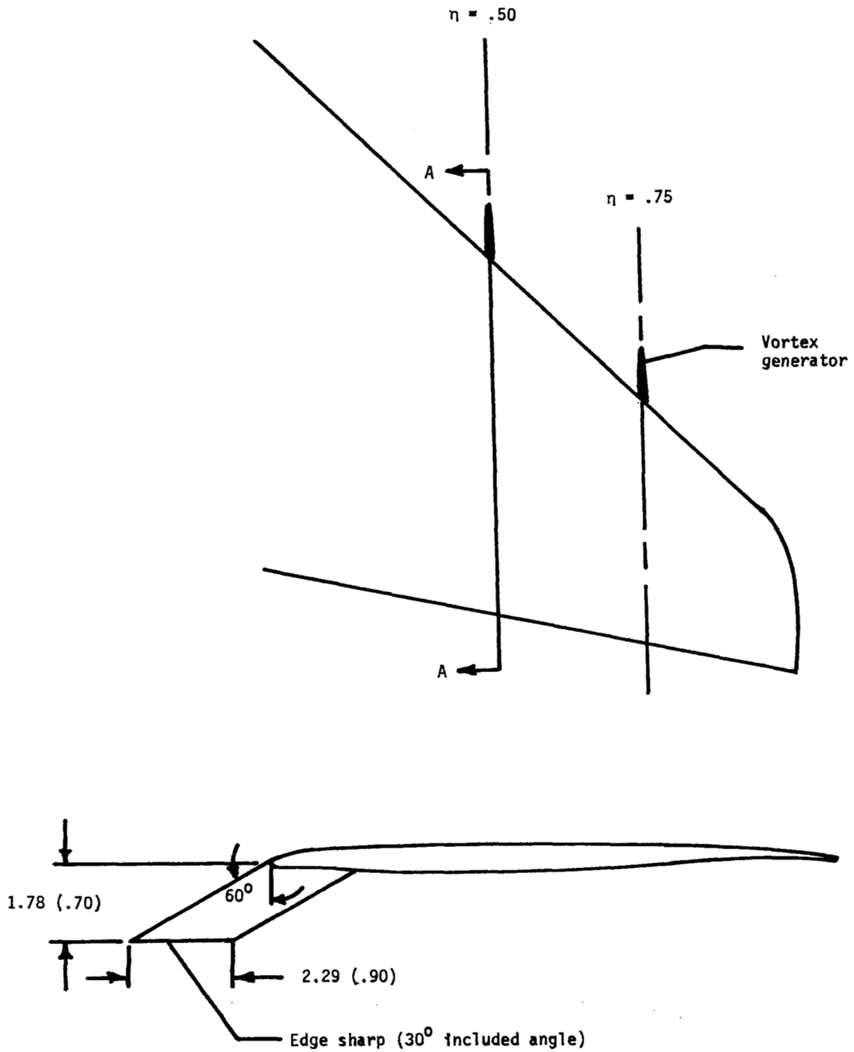
Details of vortex generator (section A-A)
