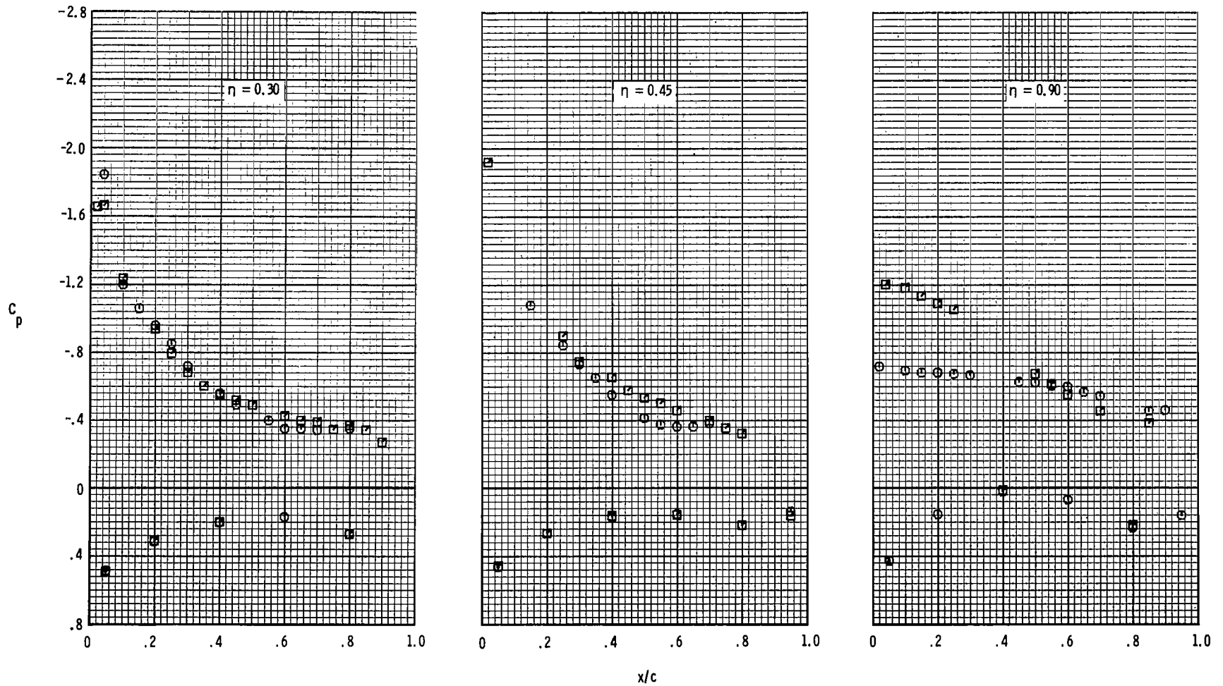
(a) M = 0.60 ; \alpha \approx 14^\circ .
