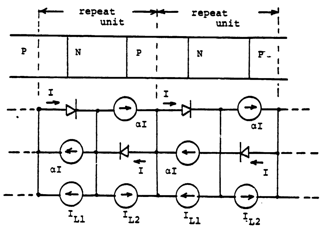
Fig. 8. Circuit model for repeated p-n-p structure.
