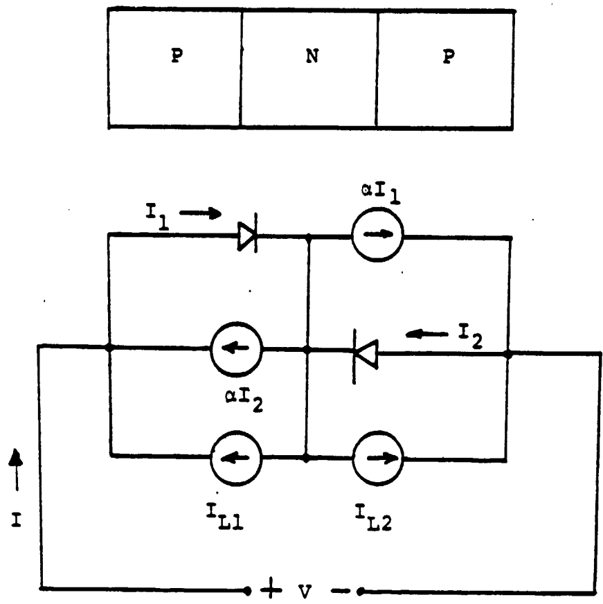
Fig. 7. Ebers-Moll model for illuminated p-n-p structure.
