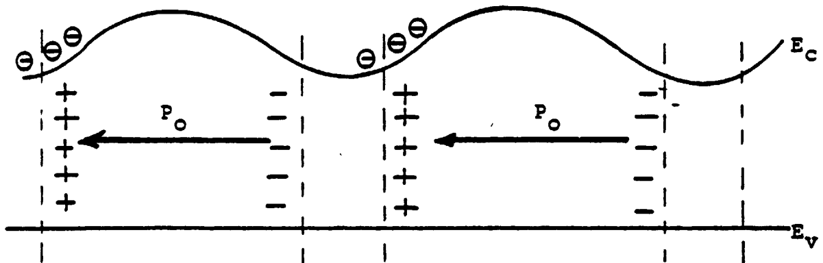
Fig. 14. The fundamental Fourier components of n'(x) and dE_C/dx are in phase; \cos \theta = +1 .
