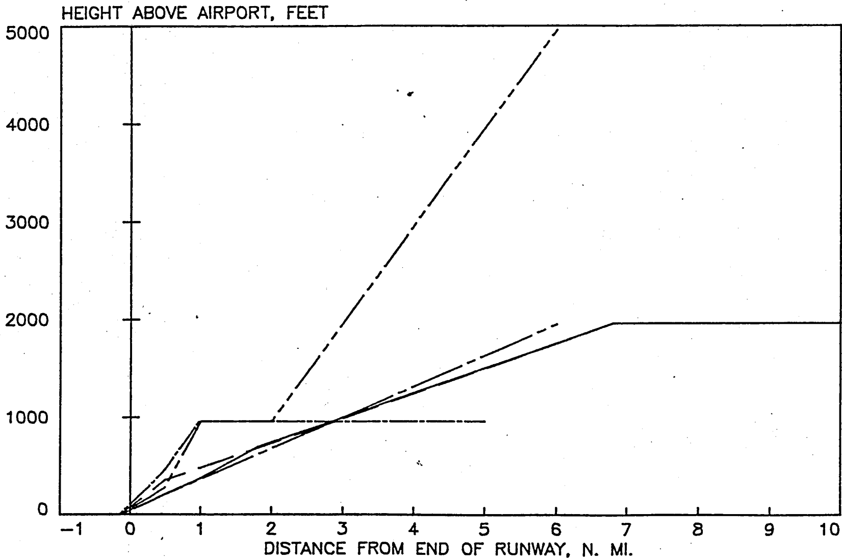
Figure 3(c).- New approach profiles in 2005, assuming a runway-change alternative is selected.
