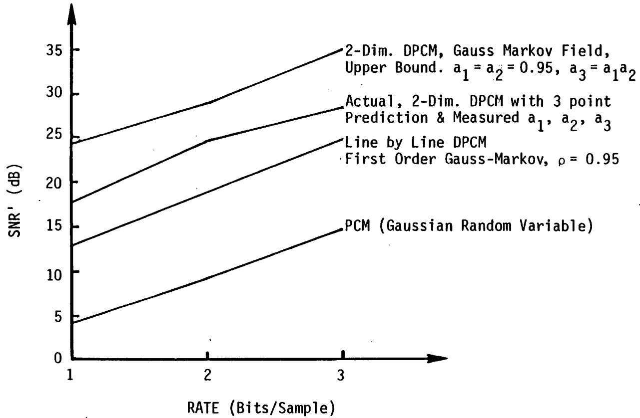
Figure 4-4. SNR versus rate of DPCM of two-dimensional, separable covariance causal model images and its comparison with line-by-line DPCM and with PCM. [5]
