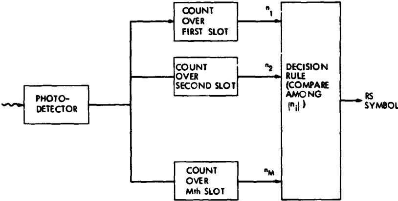
Fig. 2. Demodulator structure
