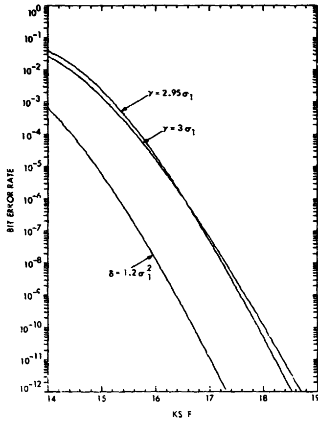
Fig. 11. Bit error rate vs K_p/F for K_p/F = 5 for RS (265, 223)
