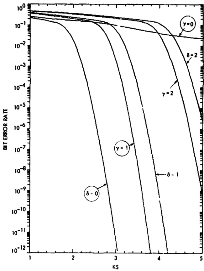
Fig. 5. Bit error rate vs K_s for K_b = 10^{-3} for RS (255, 191)
