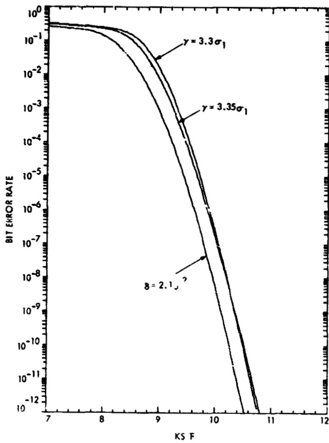
Fig. 9. Bit error rate vs K_p/F for K_p/F = \infty for RS (255, 127)
