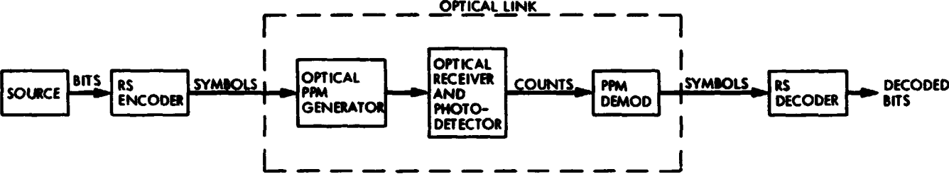
Fig. 1. PPM communication system, block diagram
