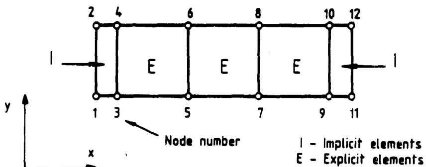
FINITE ELEMENT MESH - 2 EQUATIONS PER NODE
