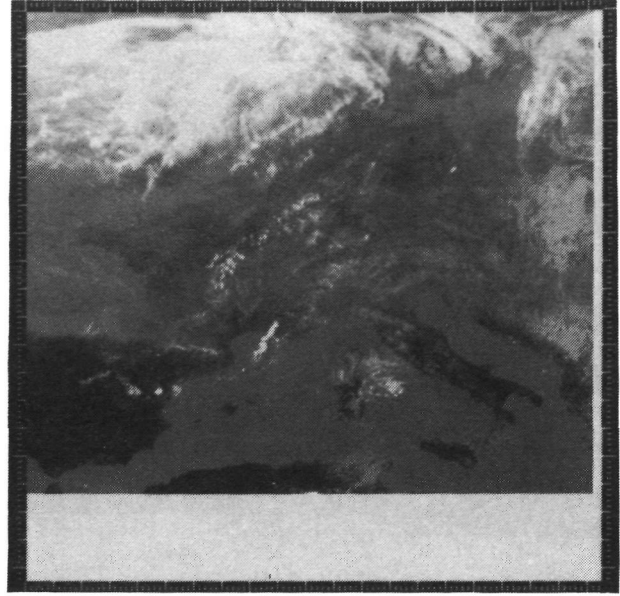
(b) Infrared.
