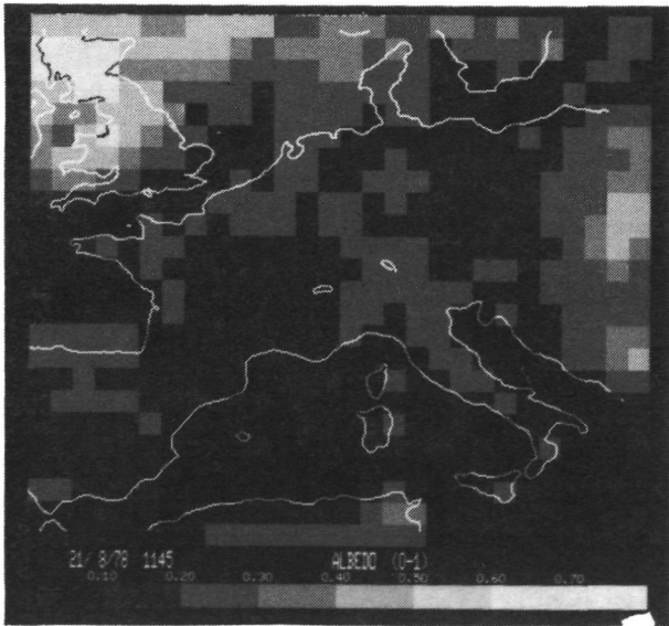
(c) Albedo.
