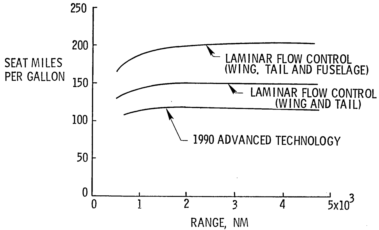
FIGURE 12 - LAMINAR FLOW CONTROL FUEL CONSERVATION POTENTIAL
