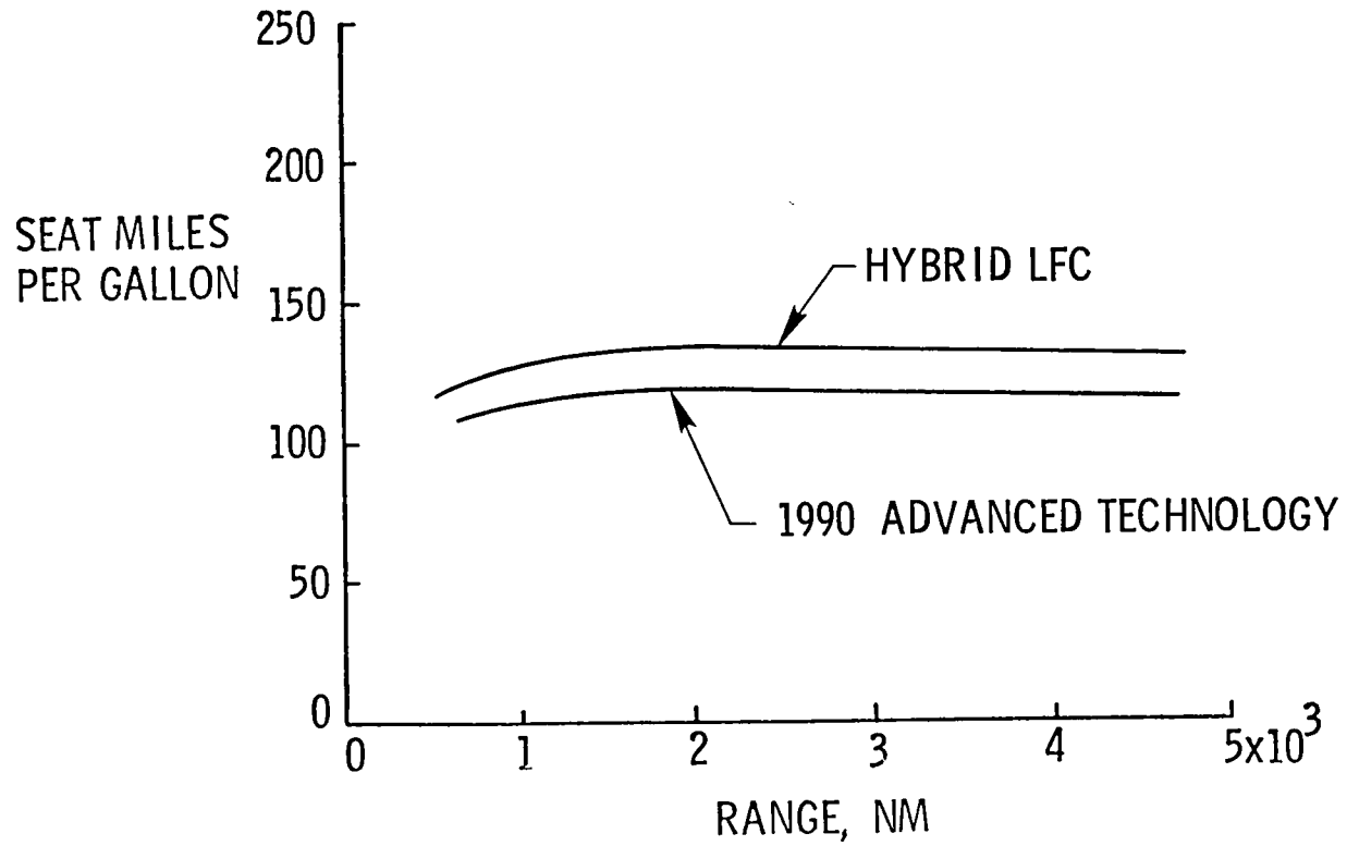
FIGURE 14 - HYBRID LAMINAR FLOW CONTROL FUEL CONSERVATION POTENTIAL
