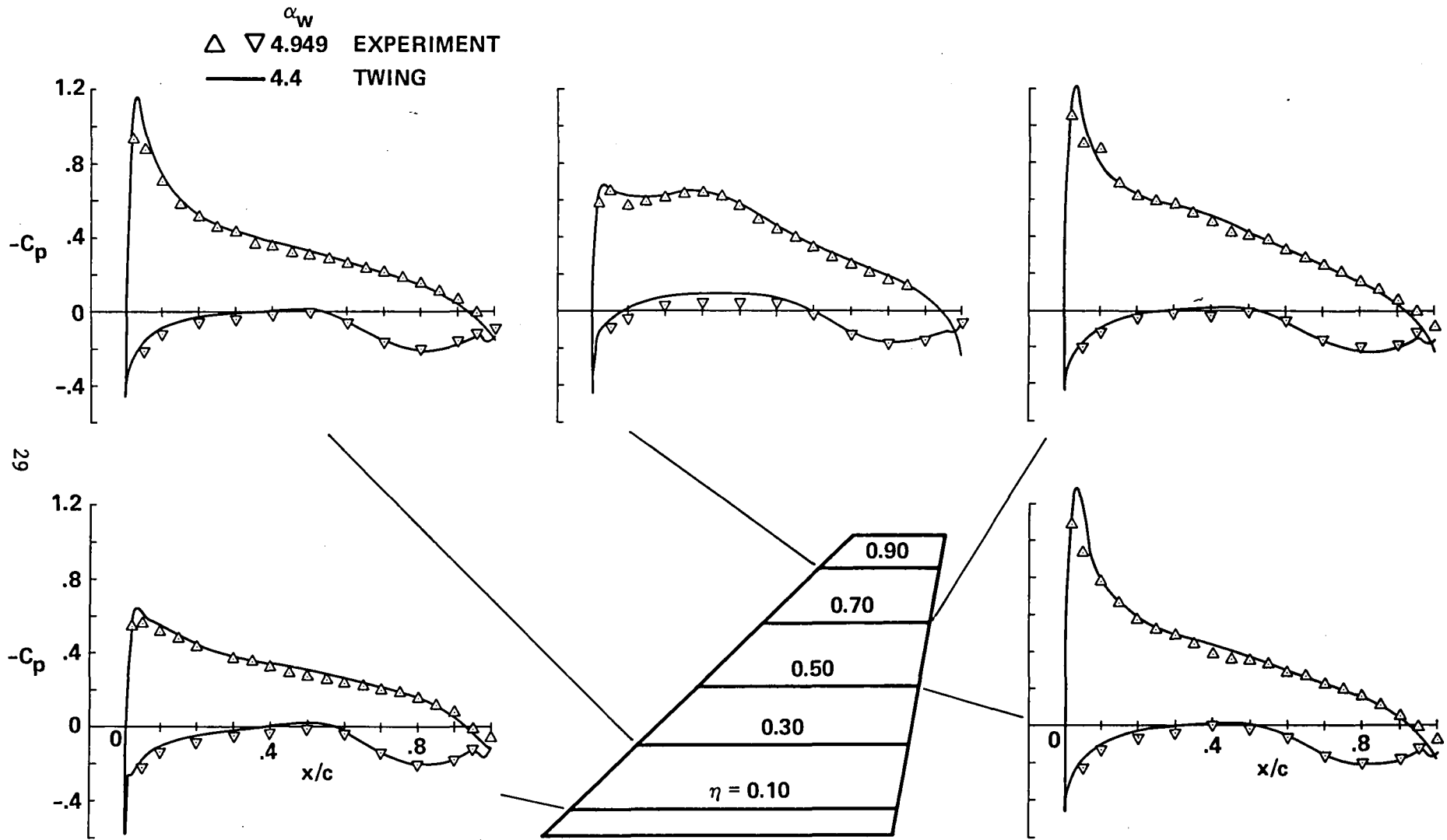
Figure 14.- Comparison of pressure coefficient distributions, experiment taken from Hinson and Burdges (ref. 29), configuration 4, \Lambda_{LE} = 45^\circ , TR = 0.3, R = 2.6 , M_\infty = 0.7 .
