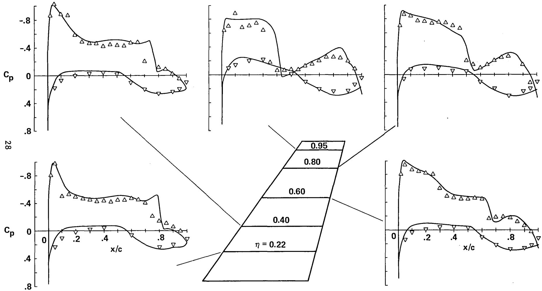
Figure 13.- Comparison of pressure coefficient distributions, experiment taken from Hinson and Burdges (ref. 29), configuration 3, \Lambda_{LE} = 35^\circ , TR = 0.4, R = 3.8 .
