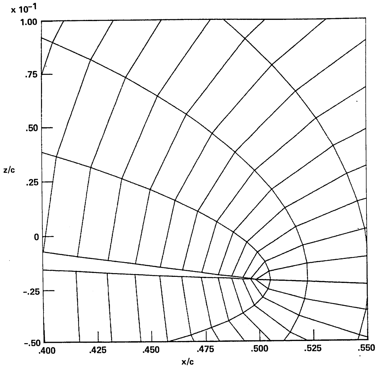
Figure 6.- Root station trailing edge close up about configuration 4 (ref. 29).
