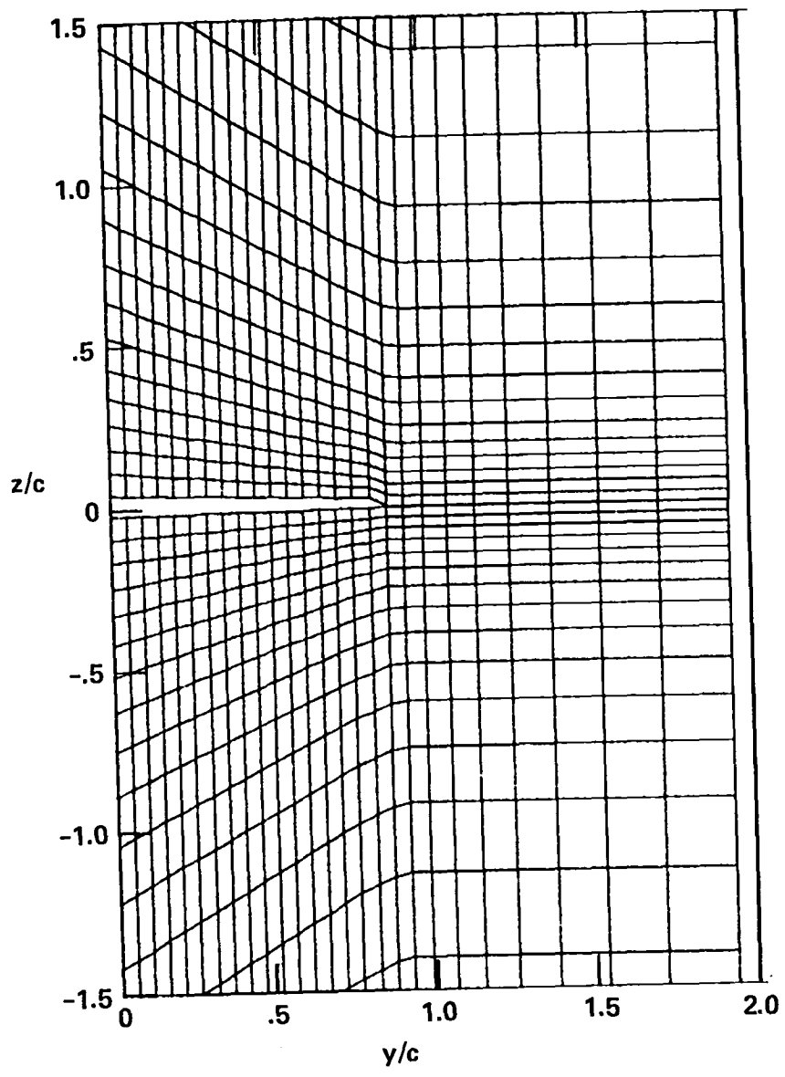
Figure 8.- Three-dimensional grid about configuration 4 (ref. 29), half chord view, 27x20 grid points.
