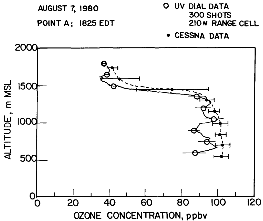
Figure 3. - Ozone profile obtained by the UV-DIAL system and compared with in situ measurements. Point A is located at 39°59'N latitude and 75°27'W longitude.
