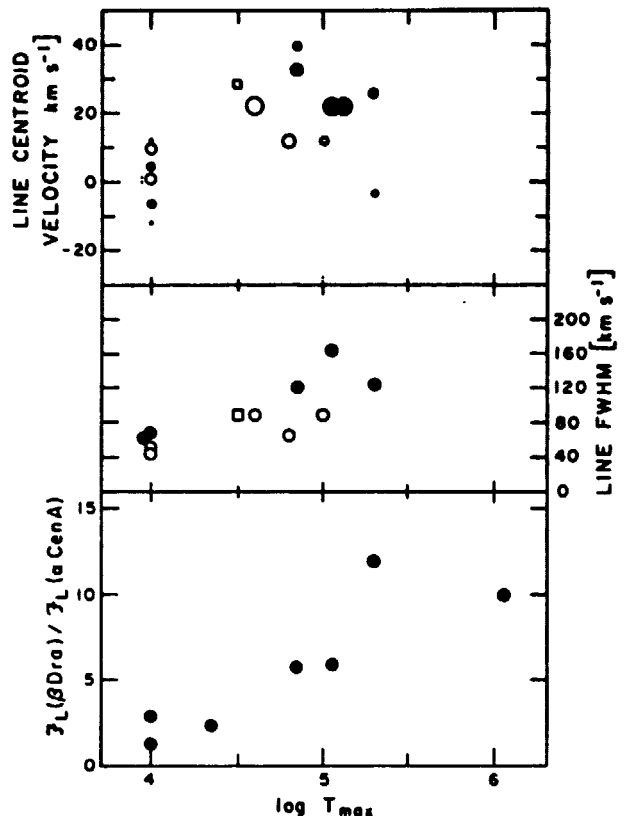
Fig. 6. Plots of the line centroid velocities, line widths, and relative surface fluxes as a function of line formation temperature for \beta Dra (G2 Ib) (Ref. 83). In the top two panels resonance lines are indicated by filled circles and intersystem lines by open circles. In the top panel the size of the symbol indicates the relative line flux and thus its weight in determining the mean velocity for the low and high excitation lines.
