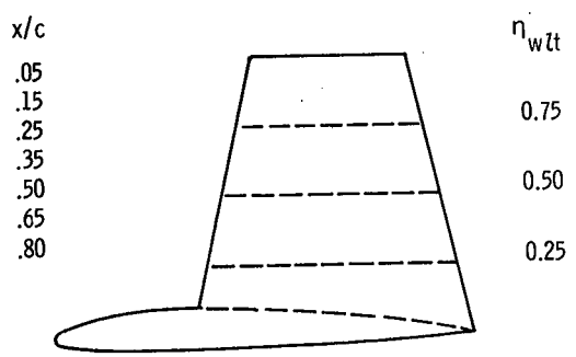
Figure 7. Winglet pressure orifice locations.
