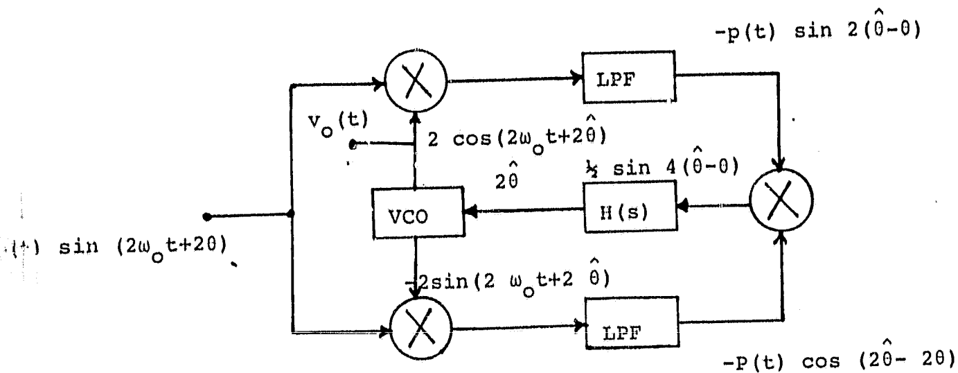
Fig. 5 Block Diagram of a Costas Loop set at 2f_0 .
