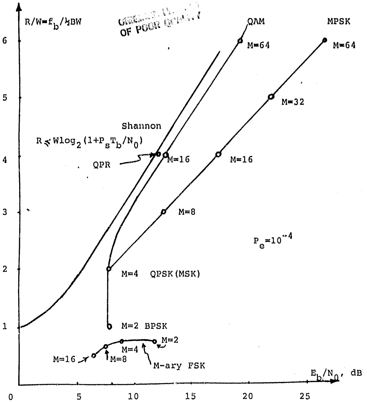
Fig. 27 Comparison of Modulation Techniques
