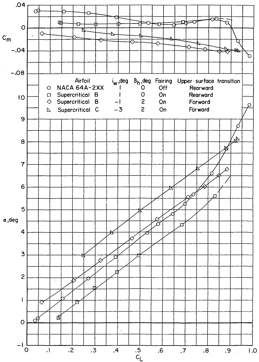
(c) M = 0.75 .
