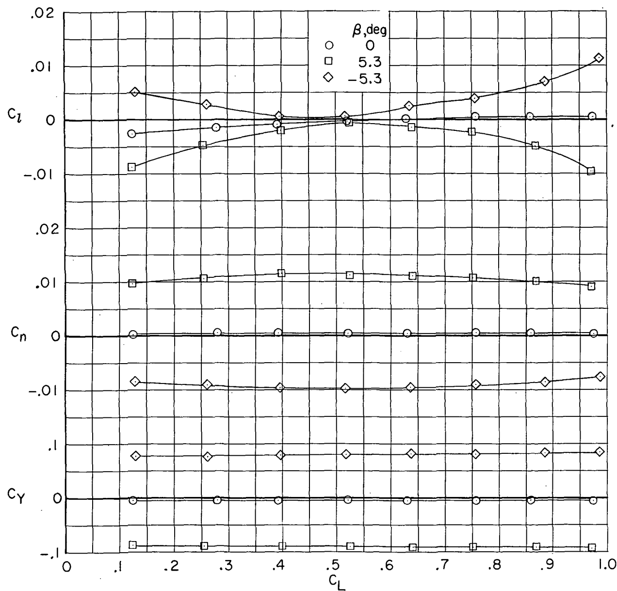
(b) M = 0.91 .
