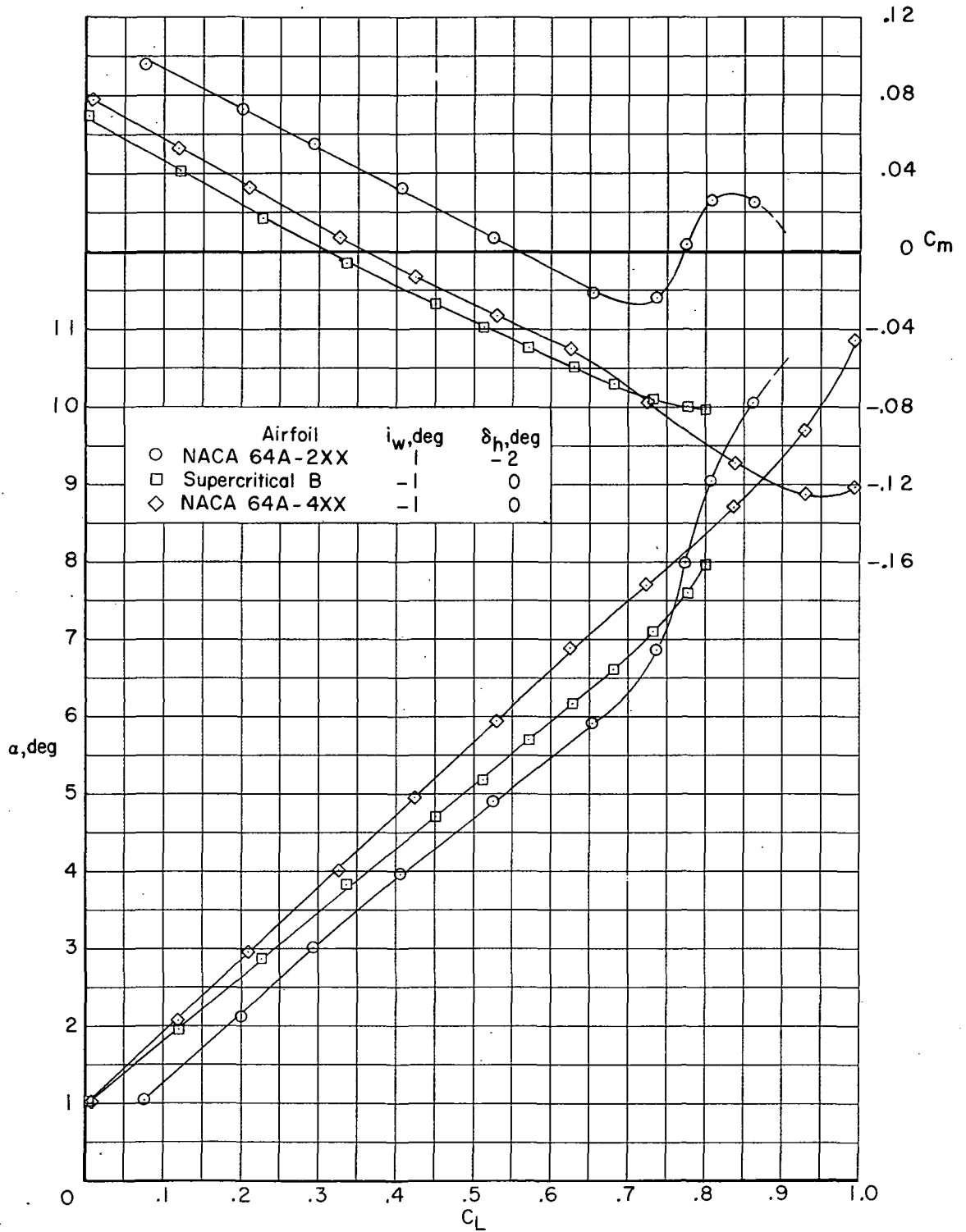
(a) M = 0.80 .
