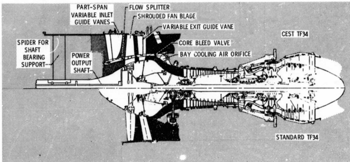
Figure 2. - CEST TF34 compared to standard TF34 engine.
