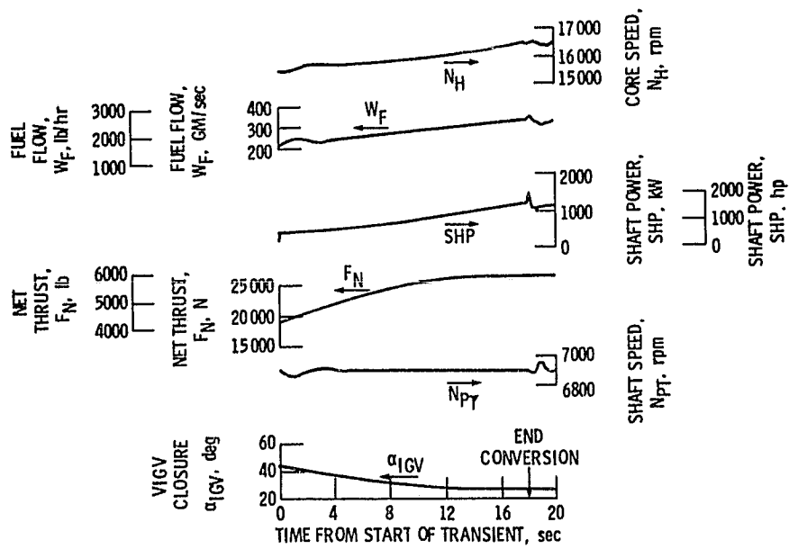
Figure 18. - Engine response to simulated X-wing rotor-start conversion.
