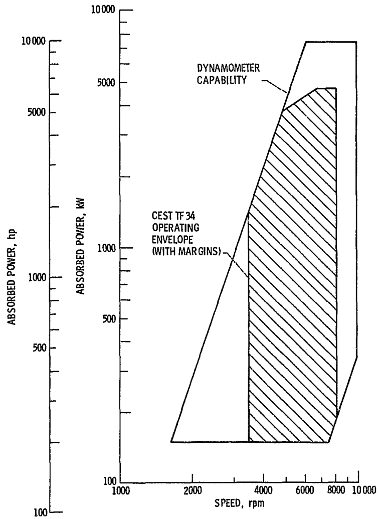
Figure 5. - Waterbrake dynamometer capability.
