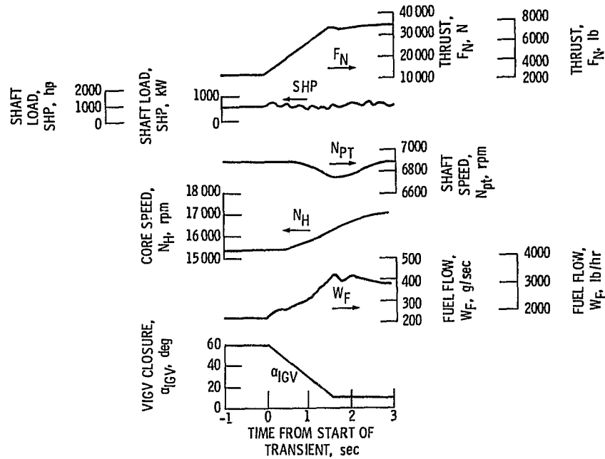
Figure 12. - Engine response to rotorcraft thrust transient.
