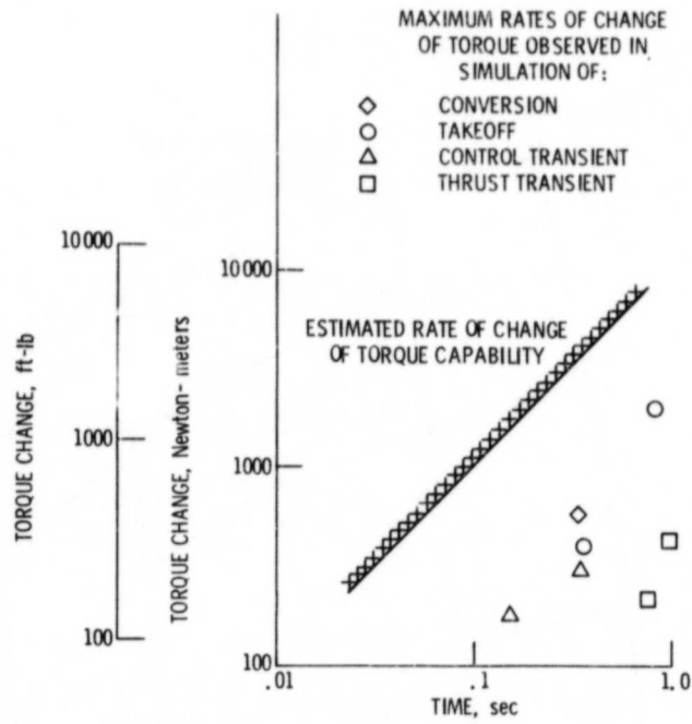
Figure 8. - Dynamic capability of power absorber system.
