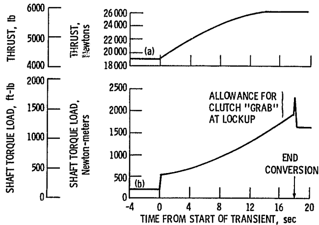
Figure 17. - Thrust and torque command programs for test stand simulation of X-wing rotor-start conversion.
