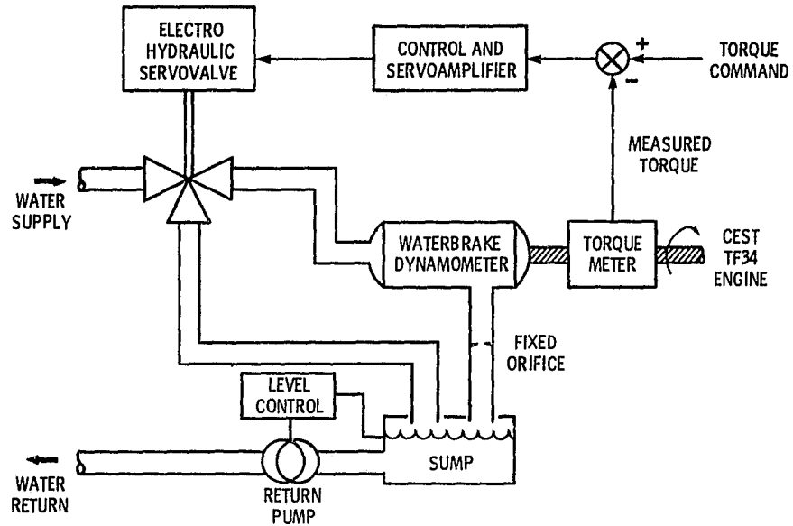
Figure 6. - Power absorber system.
