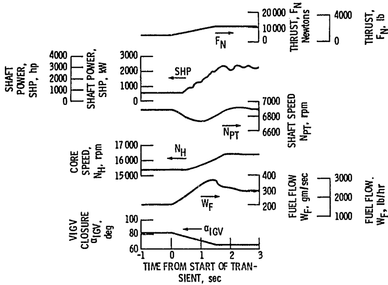
Figure 14. - Engine response to rotorcraft take-off transient.
