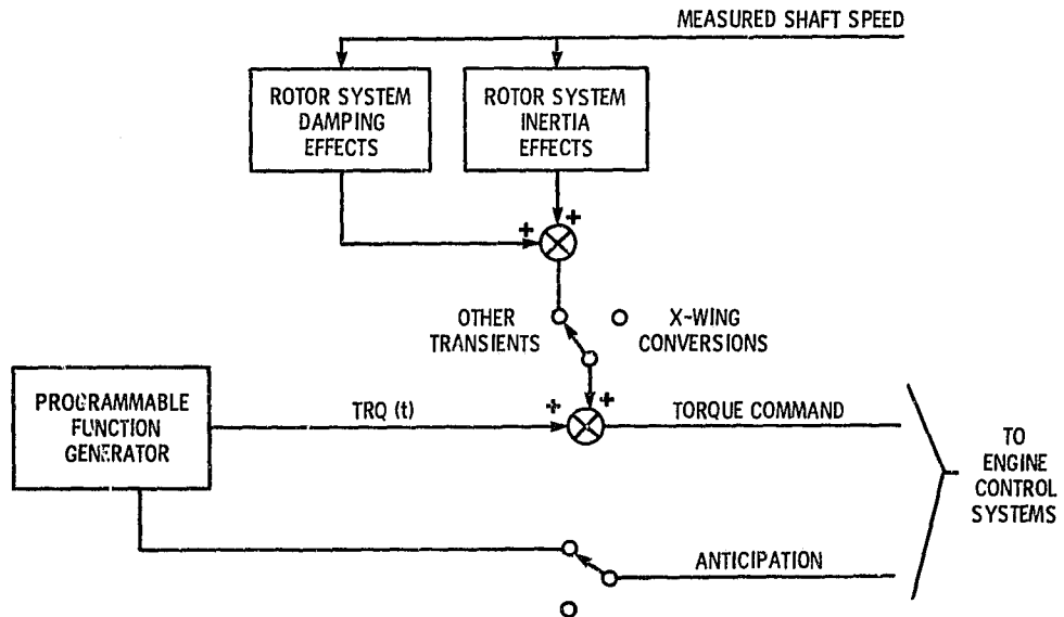
Figure 7. - Simplified block diagram of torque command system.
