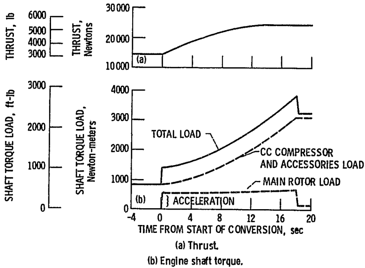
Figure 15. - X-wing rotorcraft total demand during rotor-start conversion. 13 600-kg (30 000-lb) craft; 15.2-m (50 ft) diameter rotor; 1500-m (5000 ft) altitude; 250 kn airspeed.
