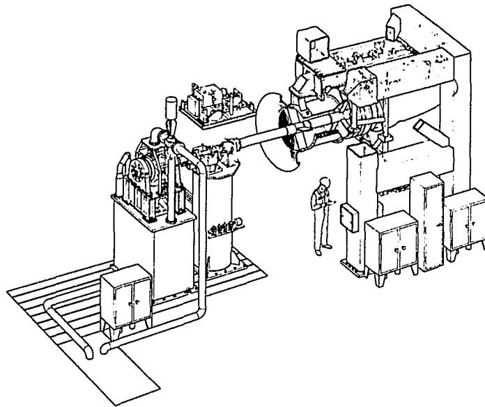
Figure 4. - CEST TF 34 on test stand at NASA Lewis Research Center.
