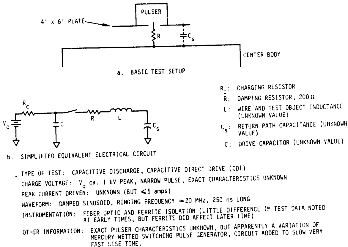
Figure 4. Center body excitation test of STARSAT
