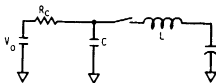
(b) EQUIVALENT ELECTRICAL CIRCUIT
