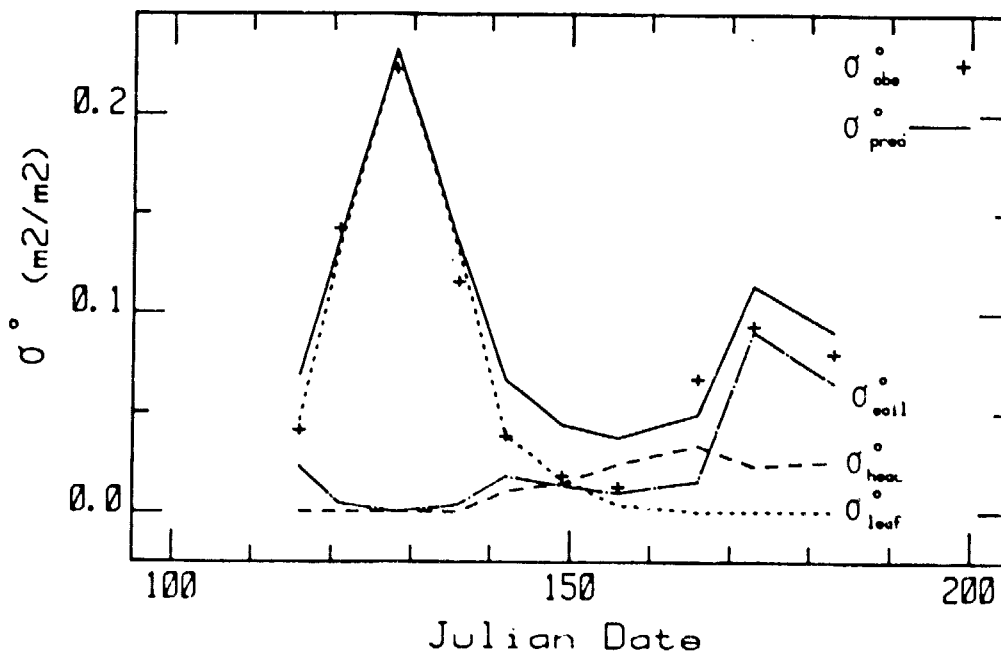
Figure 4.1b. Comparison of predicted and observed \sigma^{\circ} vs date for 13.0 GHz, VV, 1979 wheat W-41.
