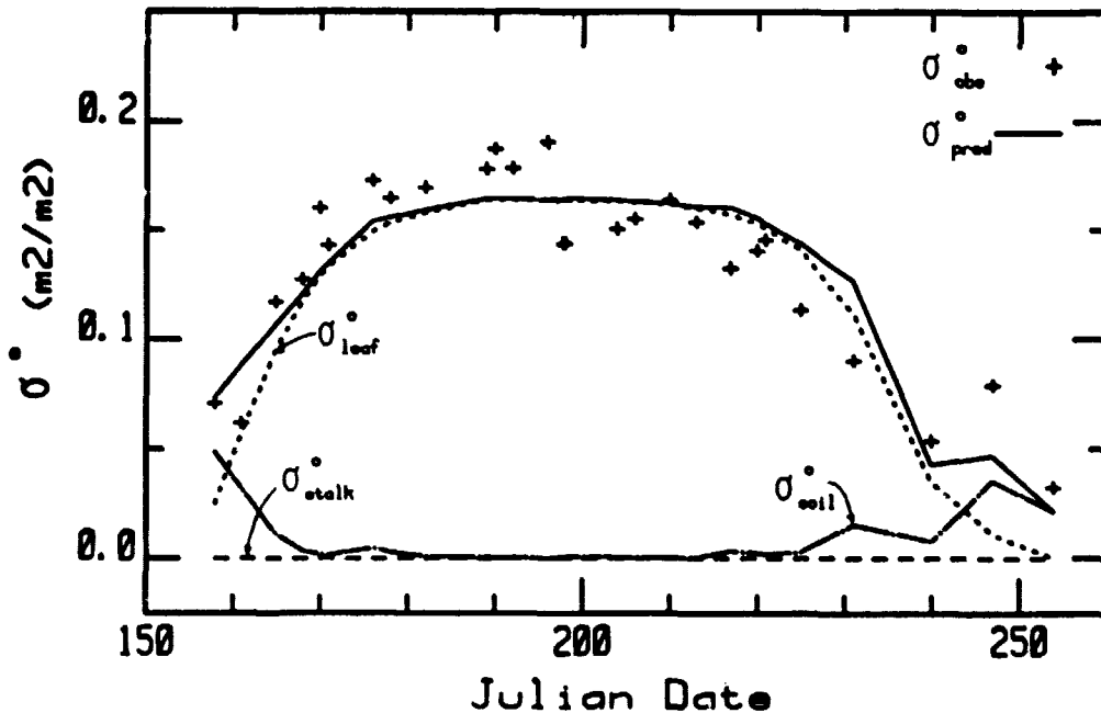
Figure 4.4b. Comparison of predicted and observed \sigma^{\circ} vs date for 13.0 GHz, VV, 1980 corn C-13.
