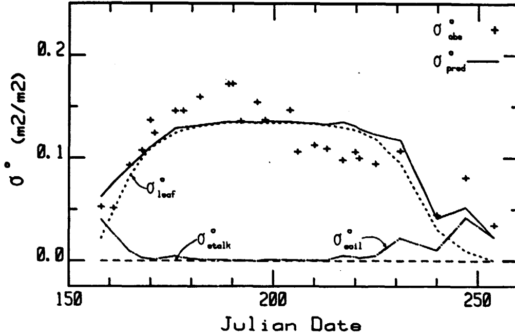
Figure 4.4a. Comparison of predicted and observed \sigma^{\circ} vs date for 8.6 GHz, VV, 1980 corn C-13.
