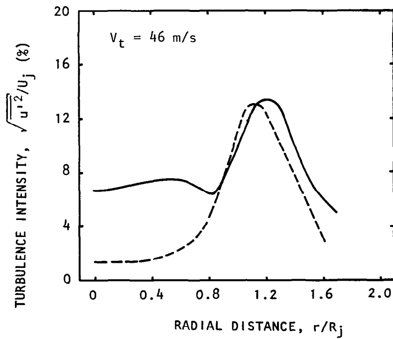
Figure 5.38 Turbulence-intensity profiles at X/D_j = 3 under flight simulation. M_j = 0.58 , U_j = 195 \text{ m/s} , Unheated, S_e = 0.5 , L_e = 141 \text{ dB} . - - - , Unexcited, ——— Excited
