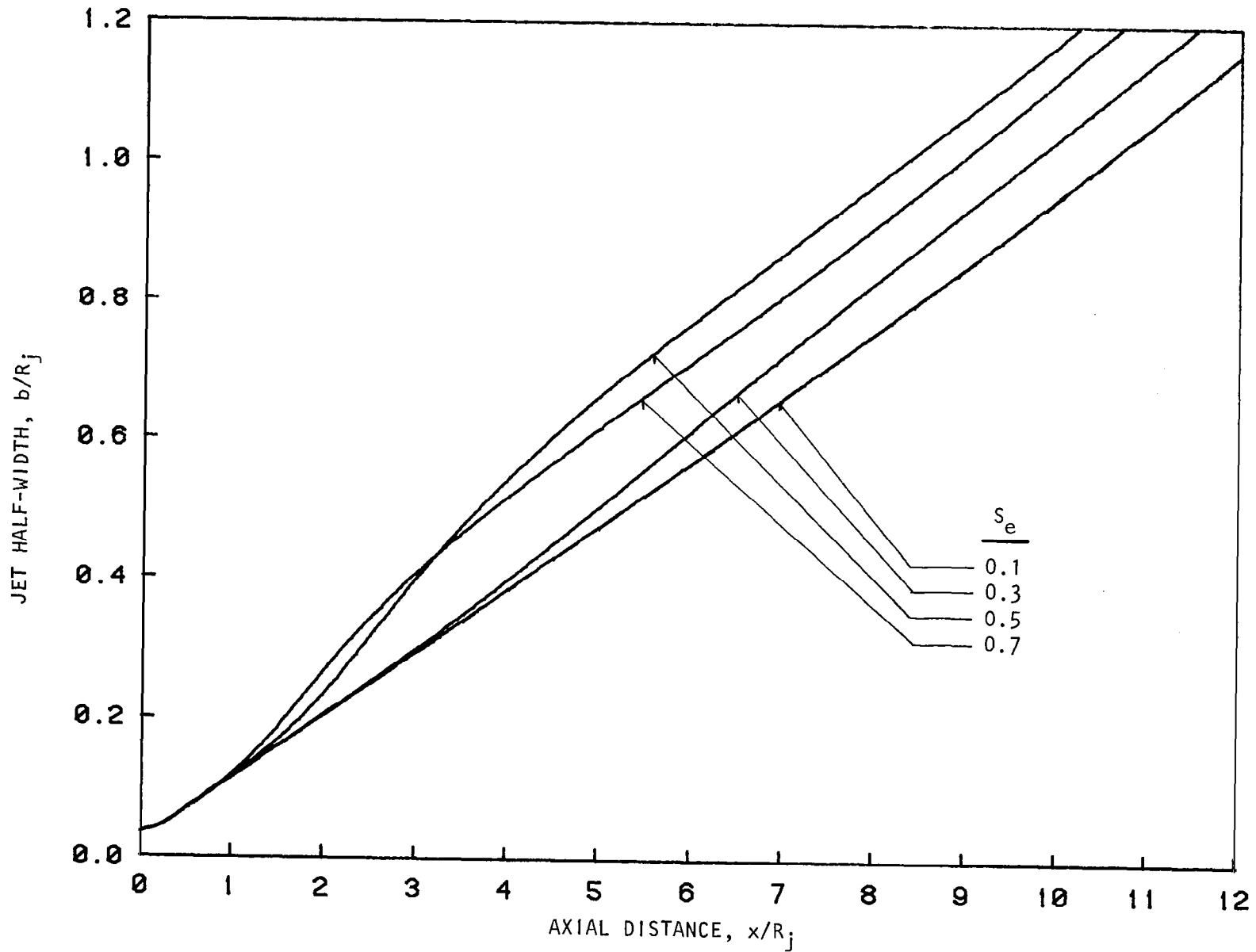
Figure 7.11 Predicted axial variation of jet half-width with excitation Strouhal number \xi = 1.25 , t_r/t_p = 1.0 (unheated), (0,0) Mode, L_e = 141 dB.
