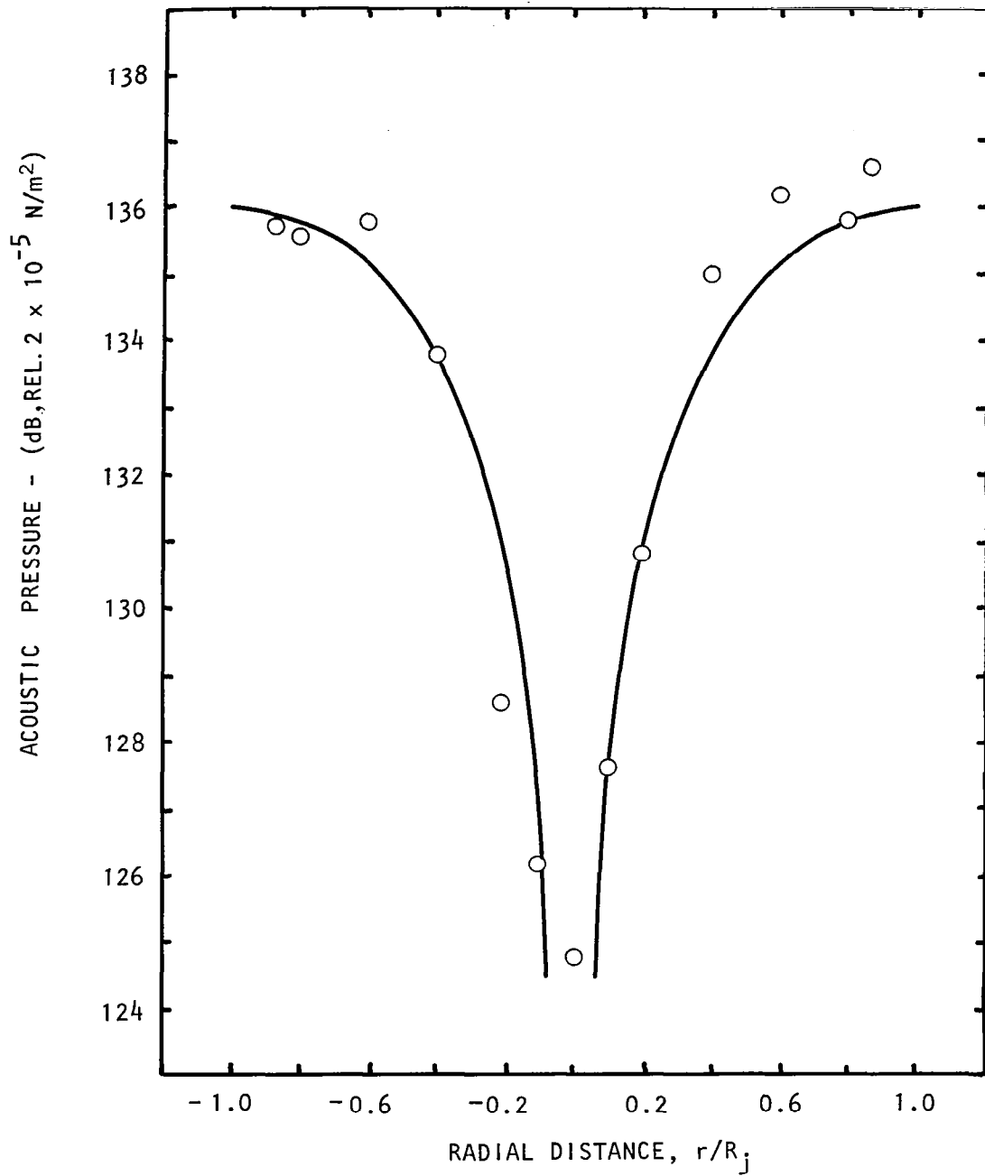
Figure 5.24 Comparison between measured ( \circ ) and predicted ( \text{—} ) acoustic pressures at the nozzle exit for the (1,0) mode. M_j = 0.58 , U_j = 195 \text{ m/s} , Unheated, Static, S_e = 1.0 , L_e = 136 \text{ dB} .
