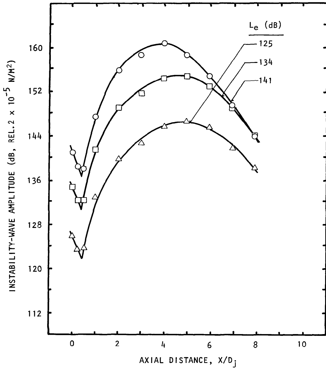
Figure 5.3 Centerline variation of instability-wave pressure amplitude at various excitation levels. M_j = 0.78 , U_j = 255 m/s, Unheated, Static, S_e = 0.5 , (0,0) Mode.
