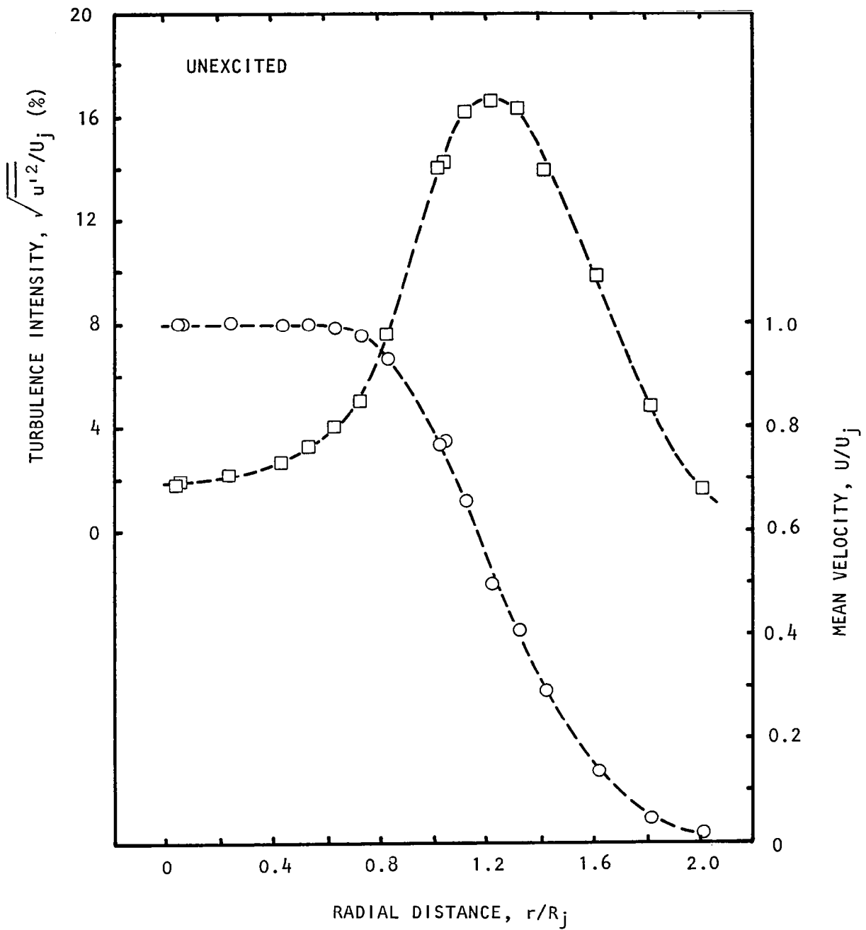
Figure D.2(a) Excitation effects on radial distribution of axial components of mean velocity (O) and turbulence intensity (□) at x/D = 3 . M_j = 0.58 , U_j = 195 m/s. Unheated, Static. (Also see figure 5.14)
