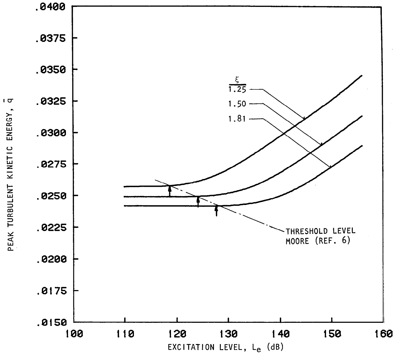
Figure 7.15 Effect of excitation level and Mach number on the peak turbulent kinetic energy. S_e = 0.5 , t_r/t_0 = 1.0 (Unheated), (0,0) Mode.
