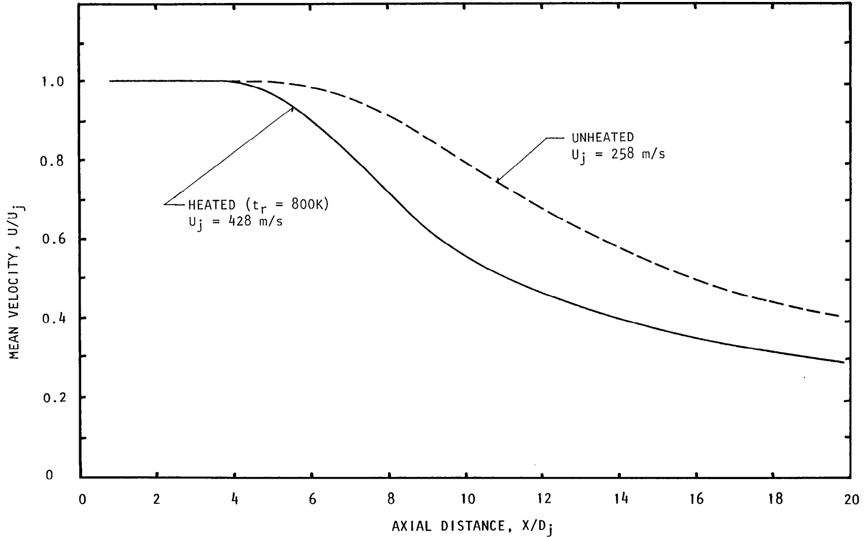
Figure 5.39(b) Reservoir-temperature effects on centerline distribution of mean velocity. M_j = 0.78 , Static, Unexcited.
