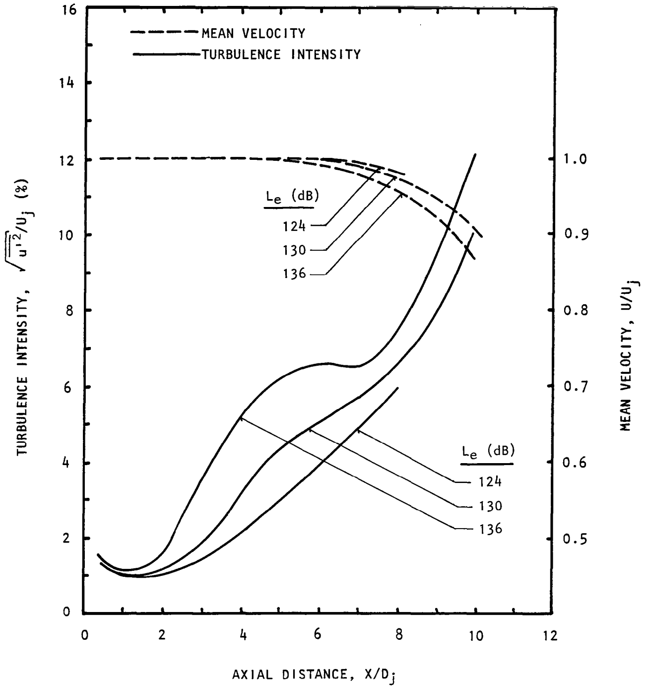
Figure 5.37 Excitation-level effects on centerline distributions of jet under flight simulation. M_j = 0.78 , U_j = 255 m/s, Unheated V_t = 57 m/s, S_e = 0.5 , (0,0) Mode .
