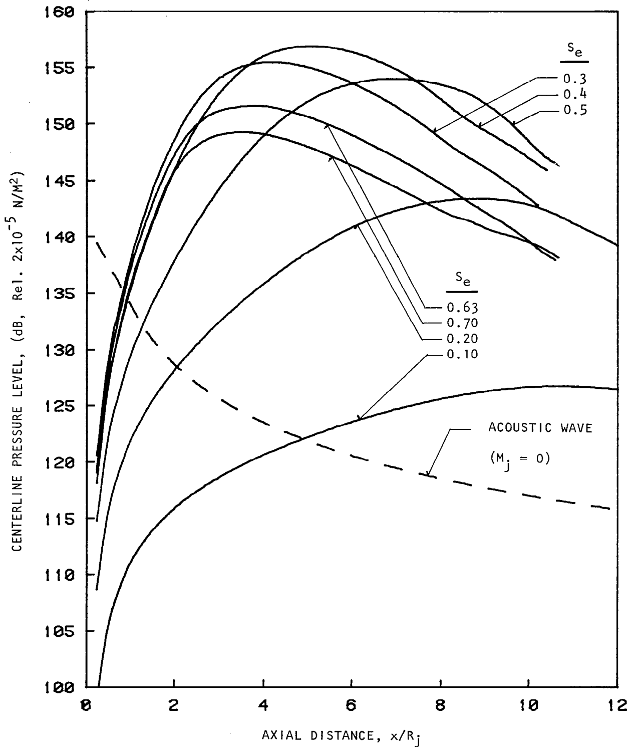
Figure 7.10 Predicted axial variation of centerline pressure level with excitation Strouhal number. \xi = 1.25 , t_r/t_o = 1.0 (unheated) (0,0) Mode, L_e = 141 \text{ dB} \cdot
