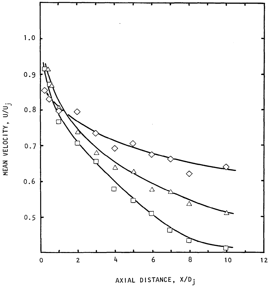
Figure D.7 Flight-velocity effects on lip-line distribution of mean velocities.
