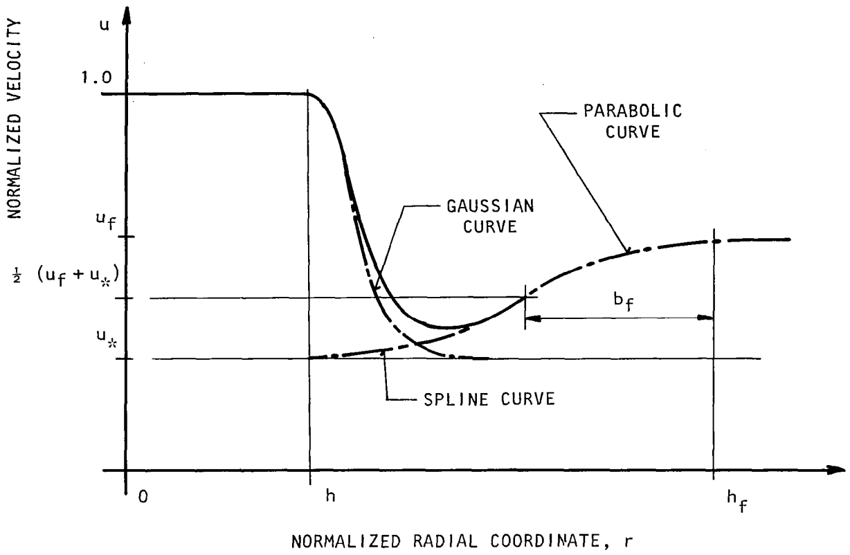
Figure 7.21 Schematic diagram of equation(7-44)indicated by the solid curve.
