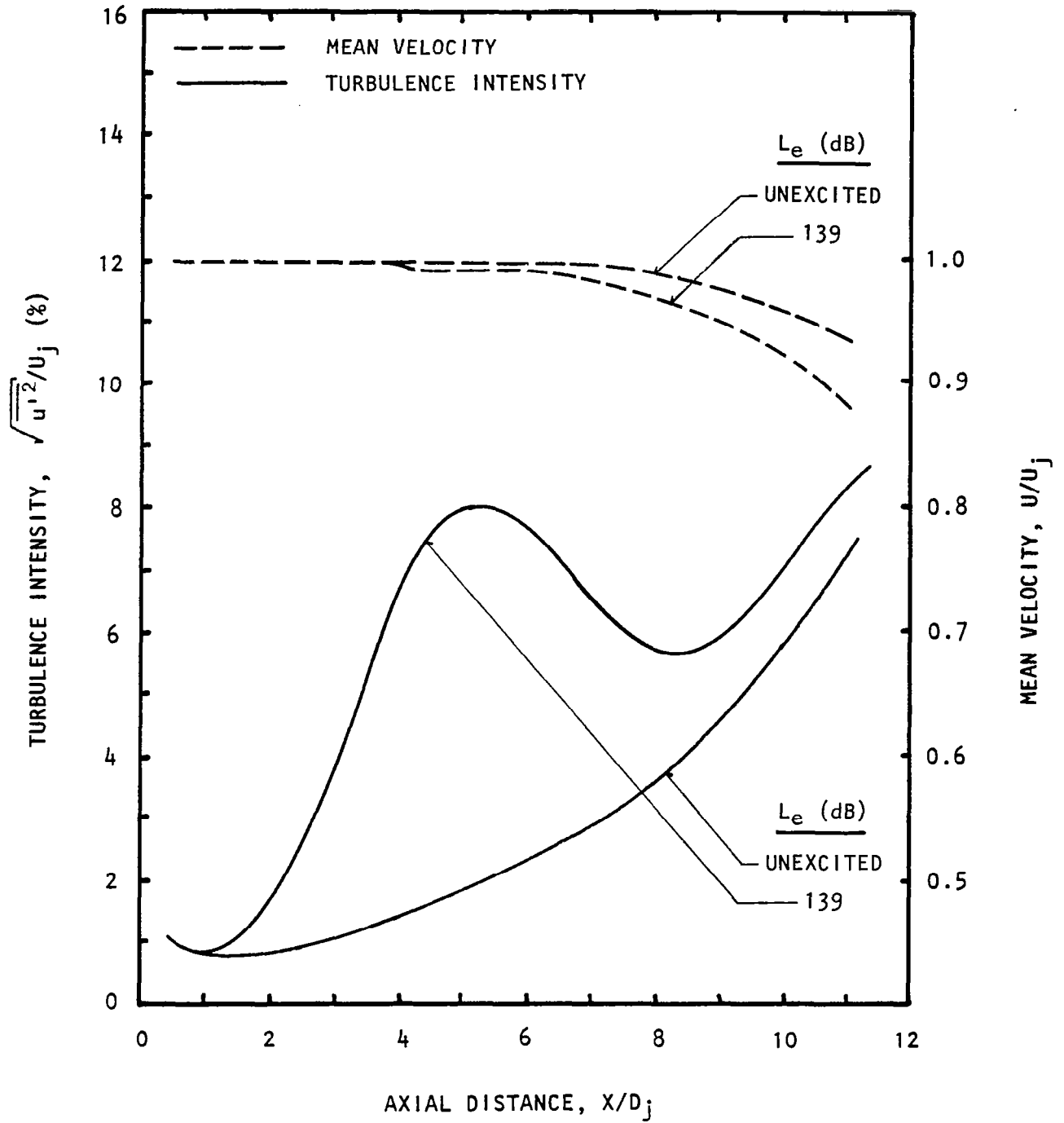
Figure 5.35 Excitation-level effects on centerline distributions of jet under flight simulation. M_j = 0.58 , U_j = 195 m/s, Unheated, V_t = 84 m/s, S_e = 0.5 , (0,0) Mode.
