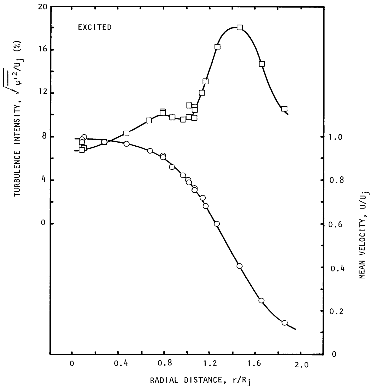
Figure D.2(b) Excitation effects on radial distribution of axial components of mean velocity (O) and turbulence intensity ( \square ) at x/D_j = 3 . M_j = 0.58 , U_j = 195 m/s, Unheated, Static, L_e = 141 dB, S_e = 0.5 . (Also see figure 5.14.)
