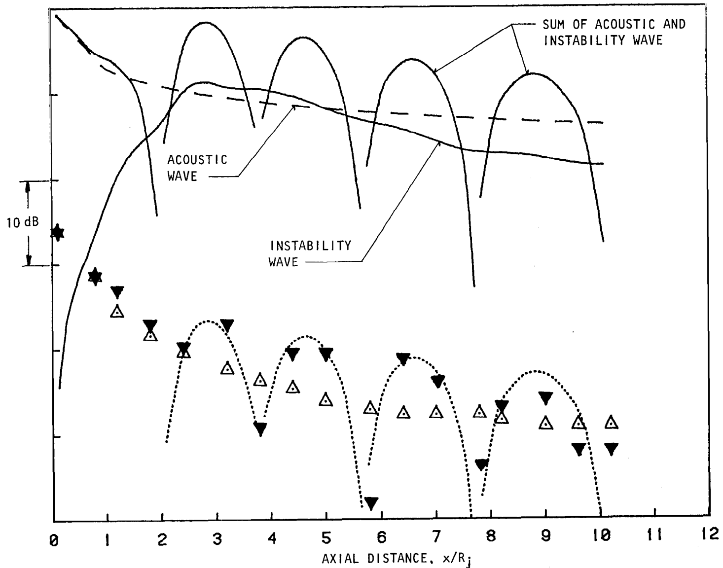
Figure 7.20 Prediction (---, —) of centerline pressure fluctuation as sum of acoustic wave and excited instability wave and comparison with measurements ( \Delta , \nabla ) by Moore (ref. 6). \Delta , No flow; \nabla , u_j = 0.15 a_0 , S_e = 0.98 ; ..... , prediction: U_j = 0.15 a_0 ; St = 1.0 .
