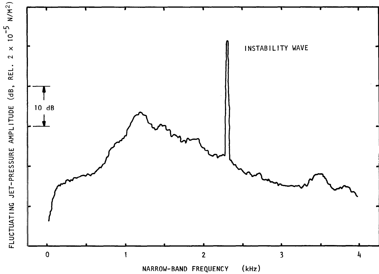
Figure 5.1 Typical spectrum of the jet-centerline pressure at x/D_j = 3.0 . M_j = 0.58 , Unheated, Static, f_e = 2330 Hz, S_e = 0.6 , L_e = 136 dB, analysis bandwidth \Delta f = 10 Hz.
