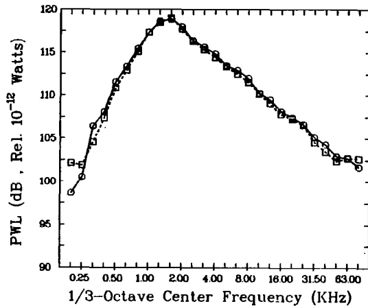
Figure 6.29 Effect of upstream excitation on a heated jet. M_j = 0.58 , U_j = 321 m/s, t_r = 800 K, Static, S_e = 0.5 , (0.0) mode. L_e : \circ , Unexcited; \square , 142 dB.
