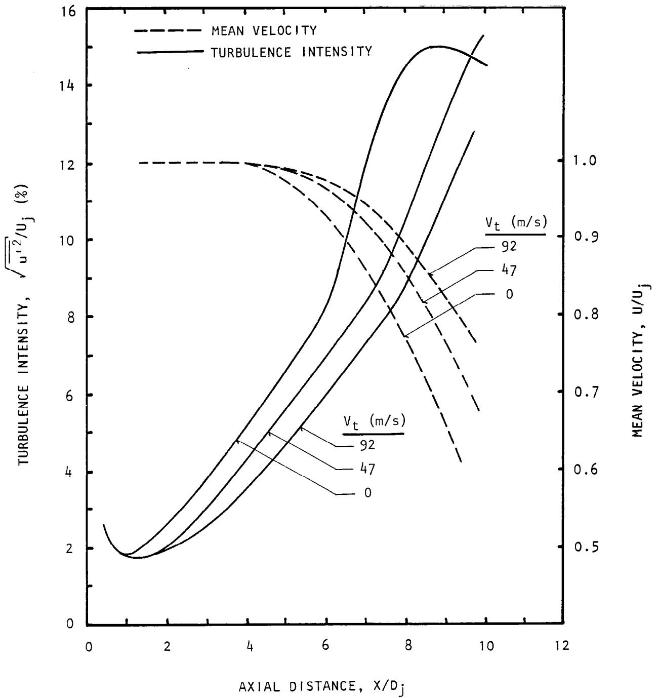
Figure 5.41 Flight-velocity effects on centerline distributions of the heated jet. M_j = 0.78 , U_j = 428 m/s, t_r = 800 K, S_e = 0.5 , L_e = 141 dB, (0,0) Mode .
