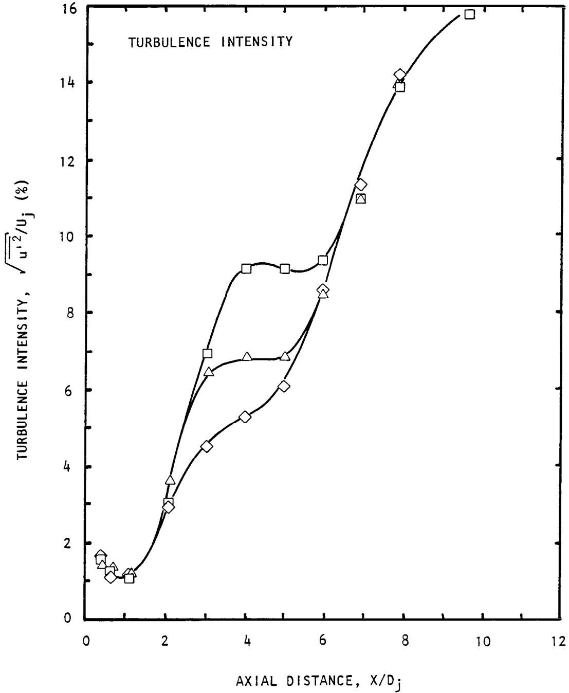
Figure D.4(b) Strouhal-number effects on centerline distributions. M_j = 0.58 , U_j = 195 m/s, Unheated, Static, L_e = 136 dB, (0,0) Mode. S_e : \square , 0.4; \triangle , 0.5; \diamond , 0.6. (Also see figure 5.19)
