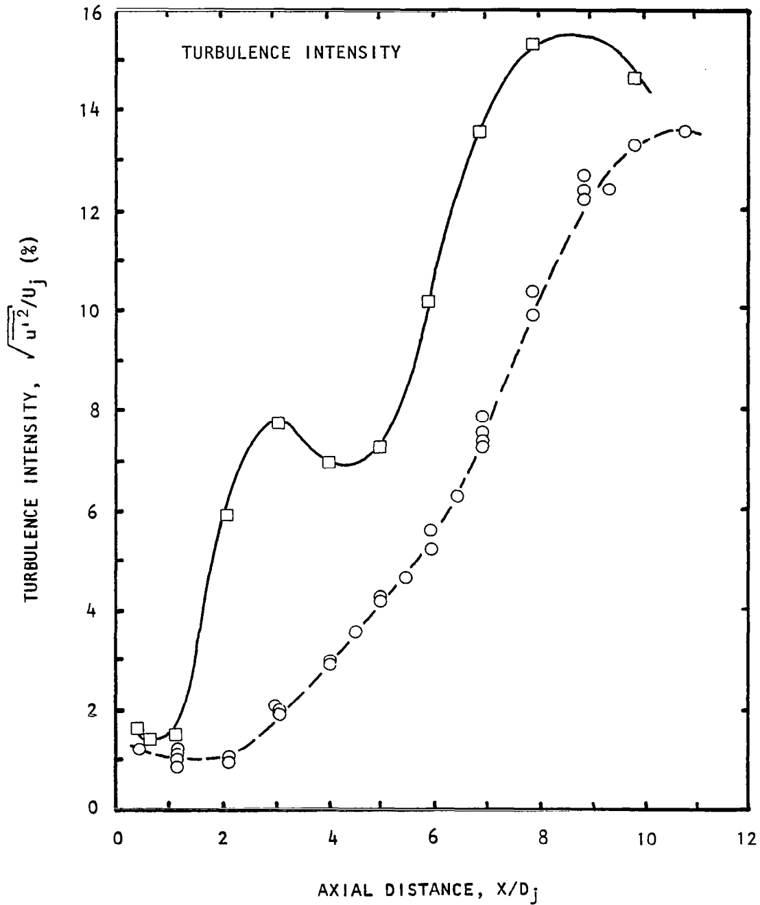
Figure D.1(b) Excitation-level effects on centerline distributions. M_j = 0.58 , U_j = 195 m/s, Unheated, Static, S_e = 0.5 , (0,0) Mode. L_e : ○ , Unexcited; □ , 141 dB. (Also see figure 5.8)
