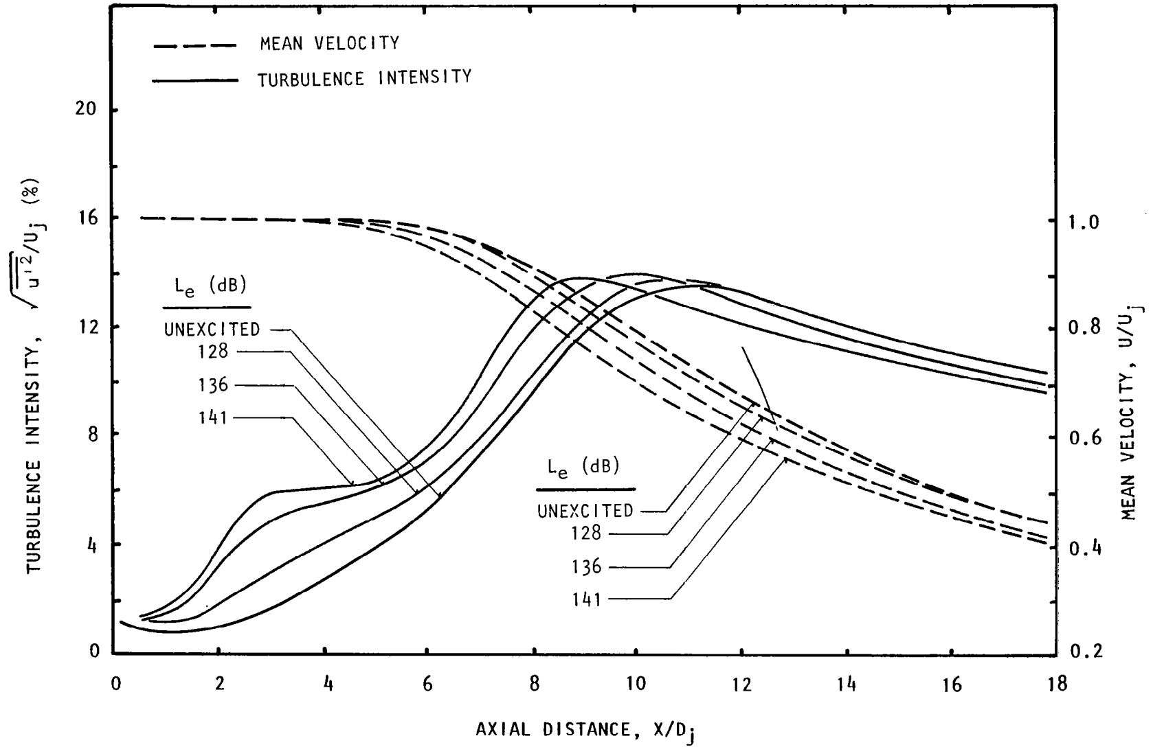
Figure 5.10 Excitation-level effects on centerline distributions. M_j = 0.78 , U_j = 255 m/s, Unheated, Static; S_e = 0.5 , (0,0) Mode
