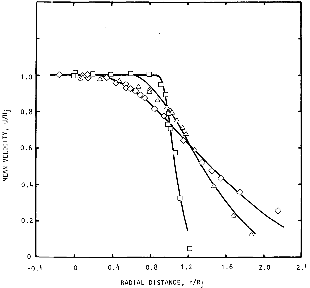
Figure 7.2 Comparison of mean-velocity profile of excited jet and Gaussian profile. M_j = 0.575 , S_e = 0.5 , L_e = 141 dB, t_r/t_0 = 1.0 . —, fitted Gaussian profile; Measured data: \square , x/D_j = 1.0 ; \triangle , x/D_j = 3.0 ; \diamond , x/D_j = 5.0 .
