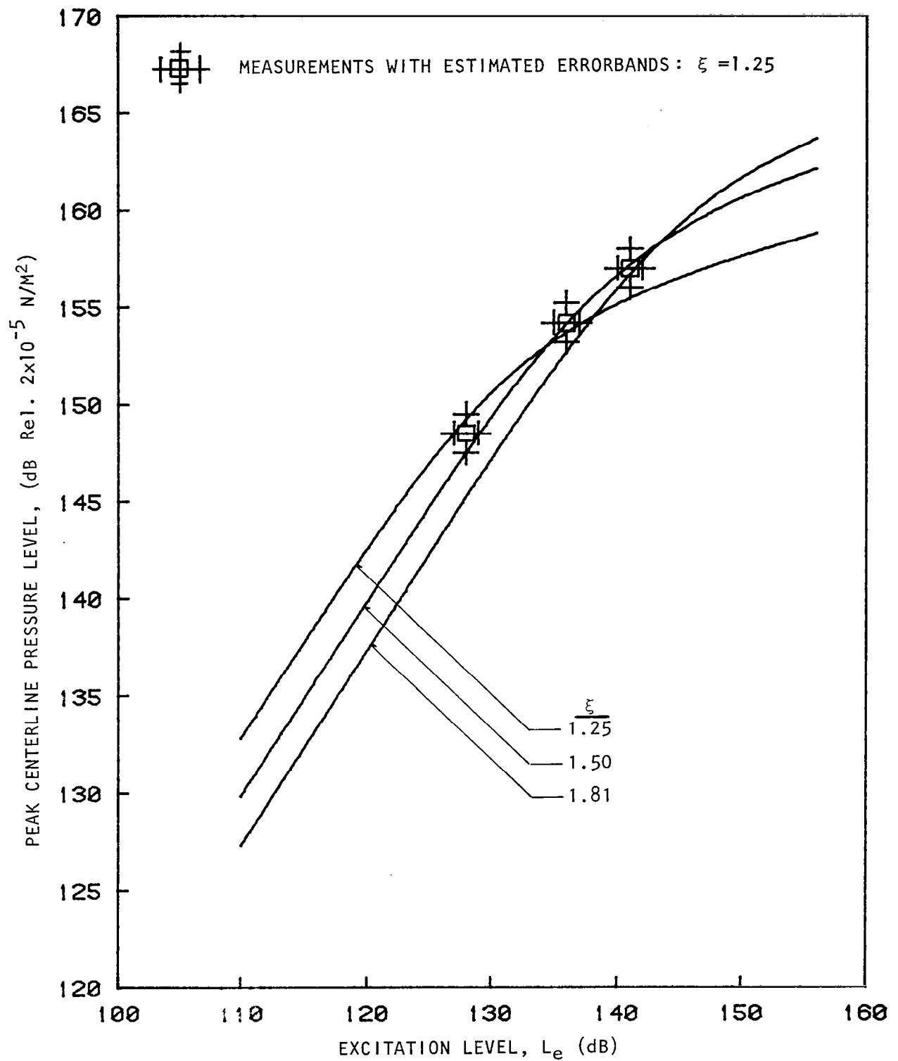
Figure 7.14 Effect of excitation level and Mach number on the peak centerline pressure level. S_e = 0.5 , t_r/t_0 = 1.0 (Unheated), (0,0) Mode.
