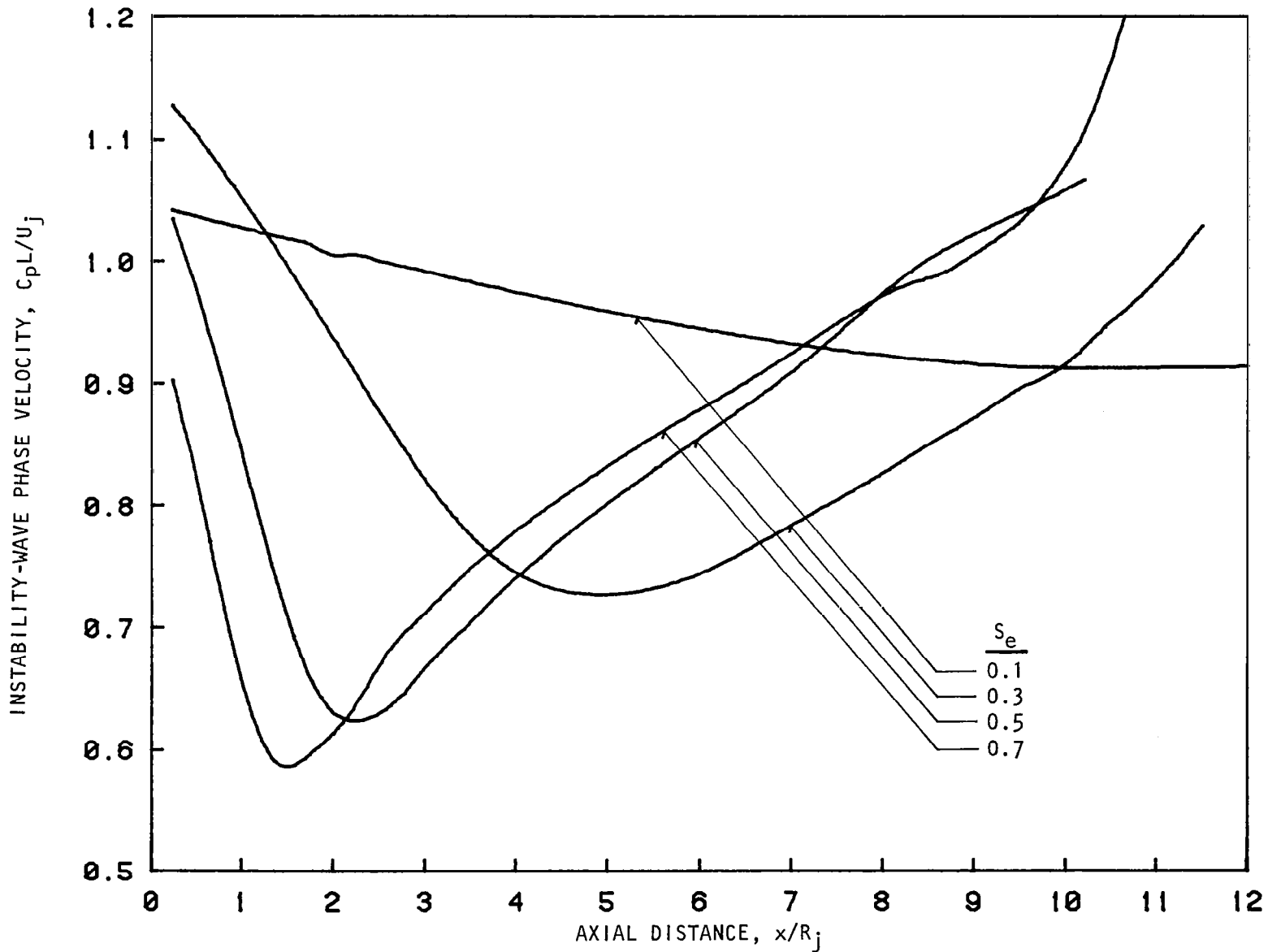
Figure 7.13 Axial variation of instability wave phase velocity with excitation Strouhal number. \xi = 1.25 , t_r/t_o = 1.0 (Unheated), (0,0) Mode, L_e = 141 dB.
