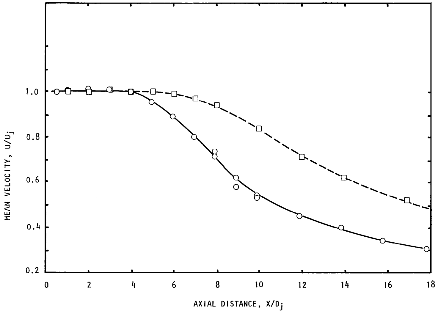
Figure D.8(b) Reservoir-temperature effects on centerline distribution of mean velocity. M_j = 0.78 , Static, Unexcited. ○ , Heated ( t_r = 800k ), U_j = 428 m/s □ , Unheated, U_j = 258 m/s (Also see figure 5.39(b))
