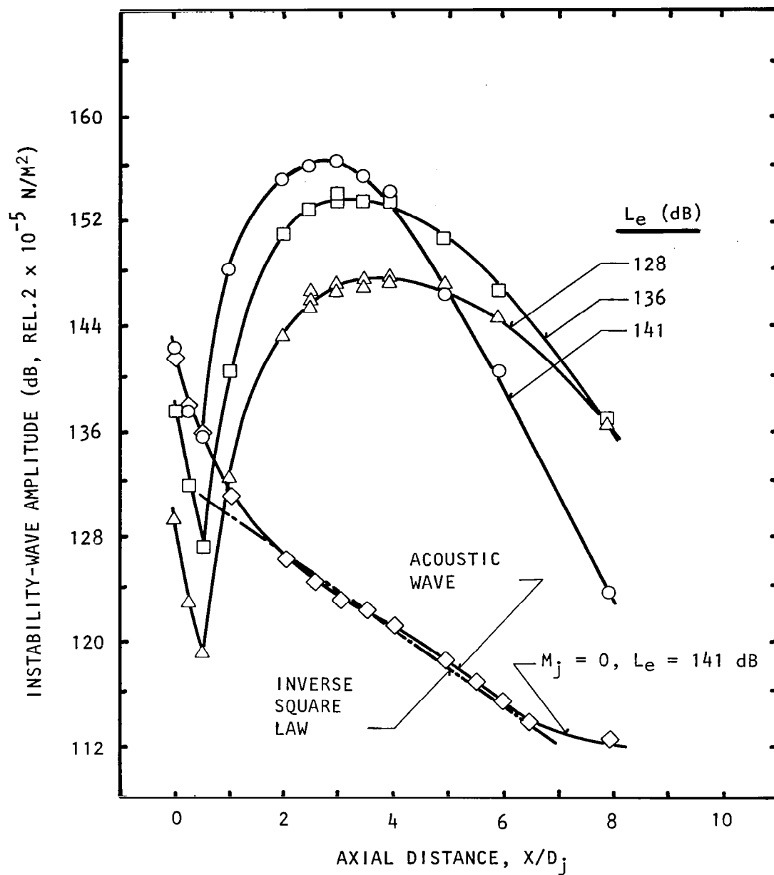
Figure 5.2 Centerline variation of instability-wave pressure amplitude at various excitation levels. M_j = 0.58 , U_j = 195 m/s, Unheated, Static, S_e = 0.5 , (0,0) Mode.
