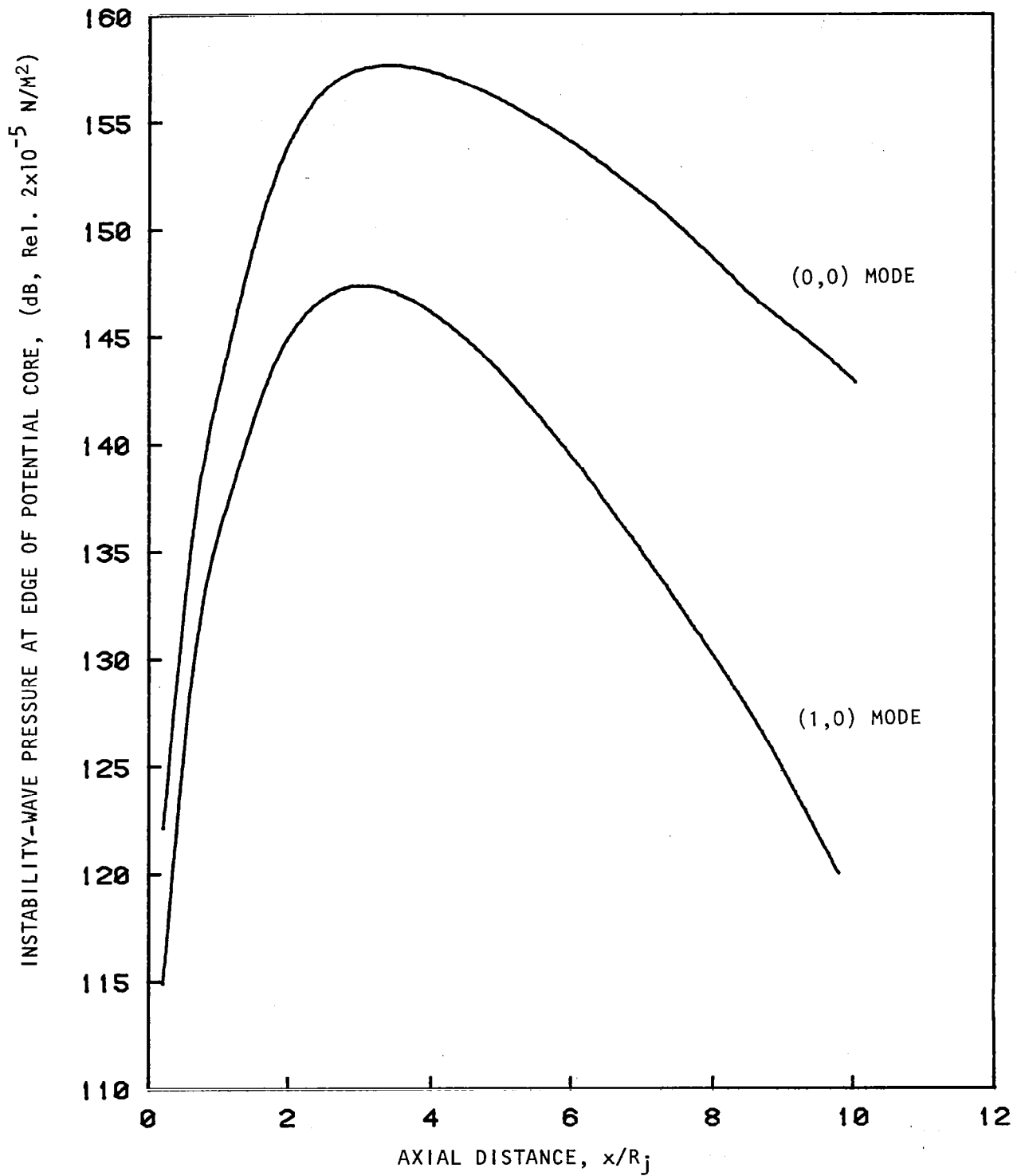
Figure 7.19 Predicted effect of the excitation mode number on the axial variation of the excited instability wave. \xi = 1.25 , t_r/t_0 = 1.0 , L_e = 141 dB, S_e = 0.5 .
