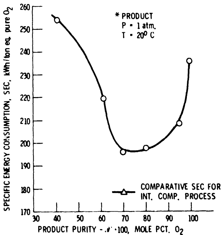
Figure 2. - Air separation process study results (Contract DEN 3-165).
