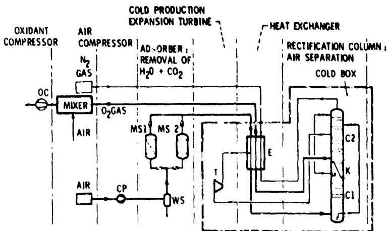
Figure 1. - Basic air separation plant delivering product O 2 at atmospheric pressure.
