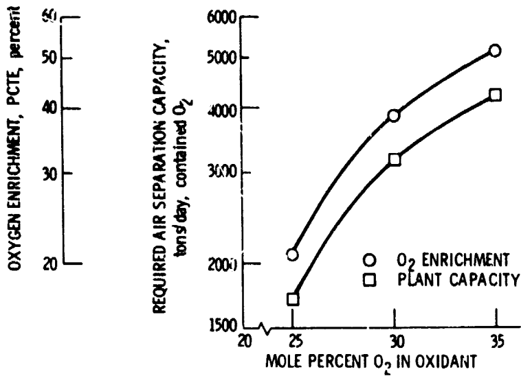
Figure 5. - Air separation plant size variation for 500 MW e MHD/steam plant. Product O 2 concentration is 70 mole percent.
