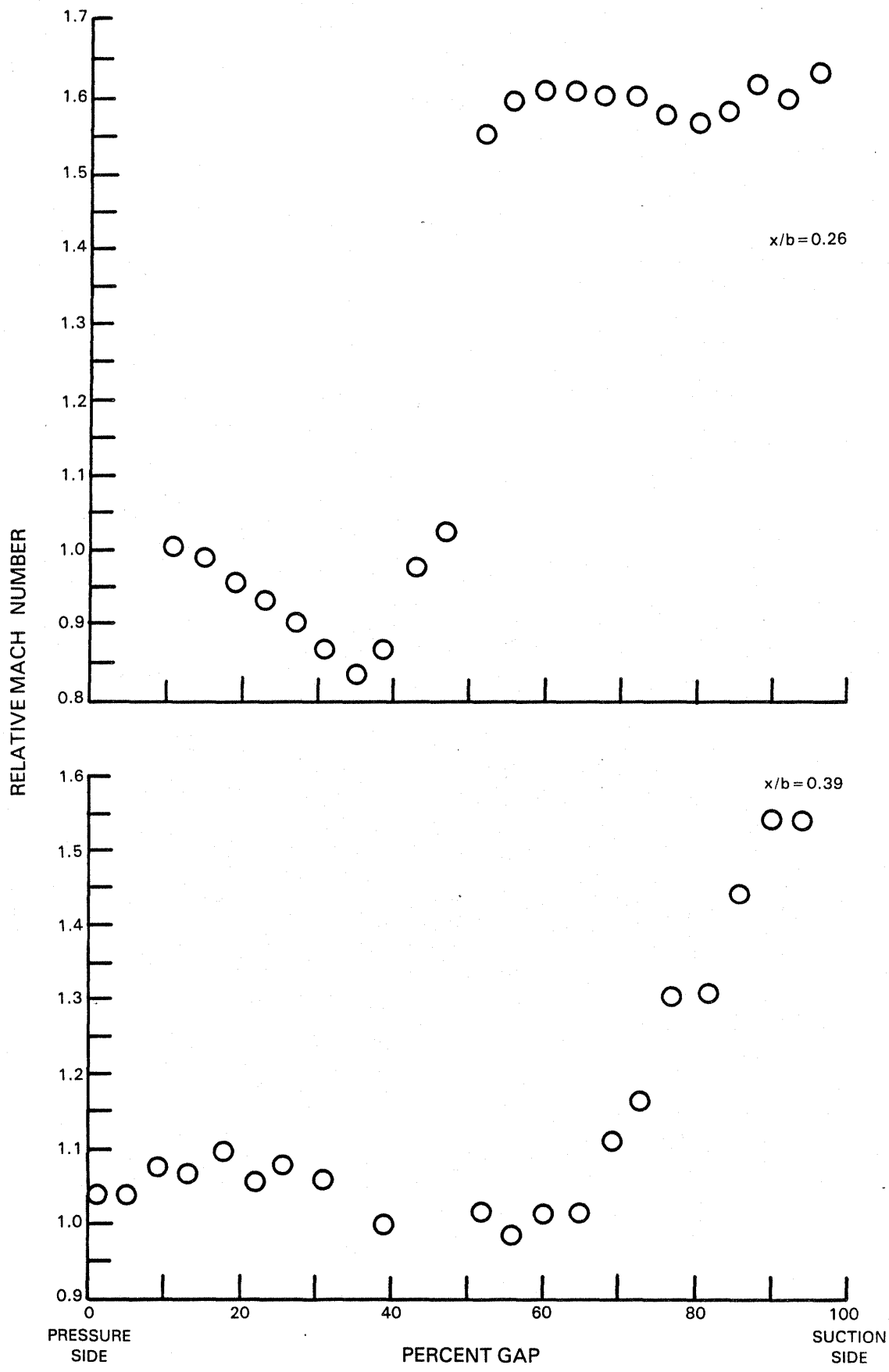
Figure 24b Mach Number Profiles at 85 Percent Span, 100 Percent Design Speed, Near Surge - Passage No. 1
