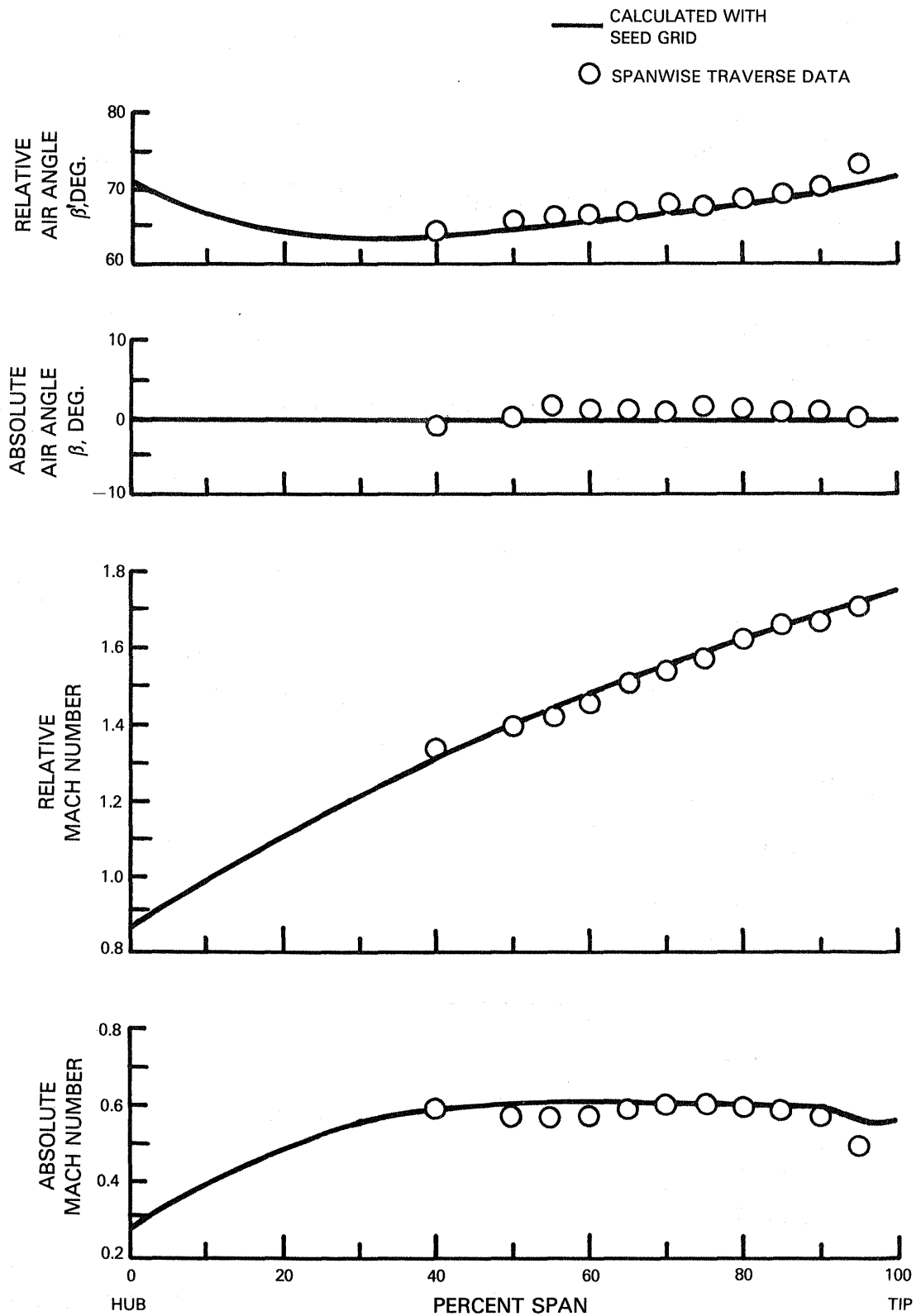
Figure 52 Laser Doppler Velocimeter Traverse at Leading Edge Plane (Station 13) - 100 Percent Design Speed, Peak Efficiency
