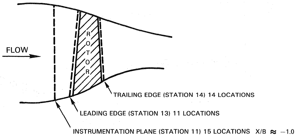
Figure 15 Laser Doppler Velocimeter Data Stations
