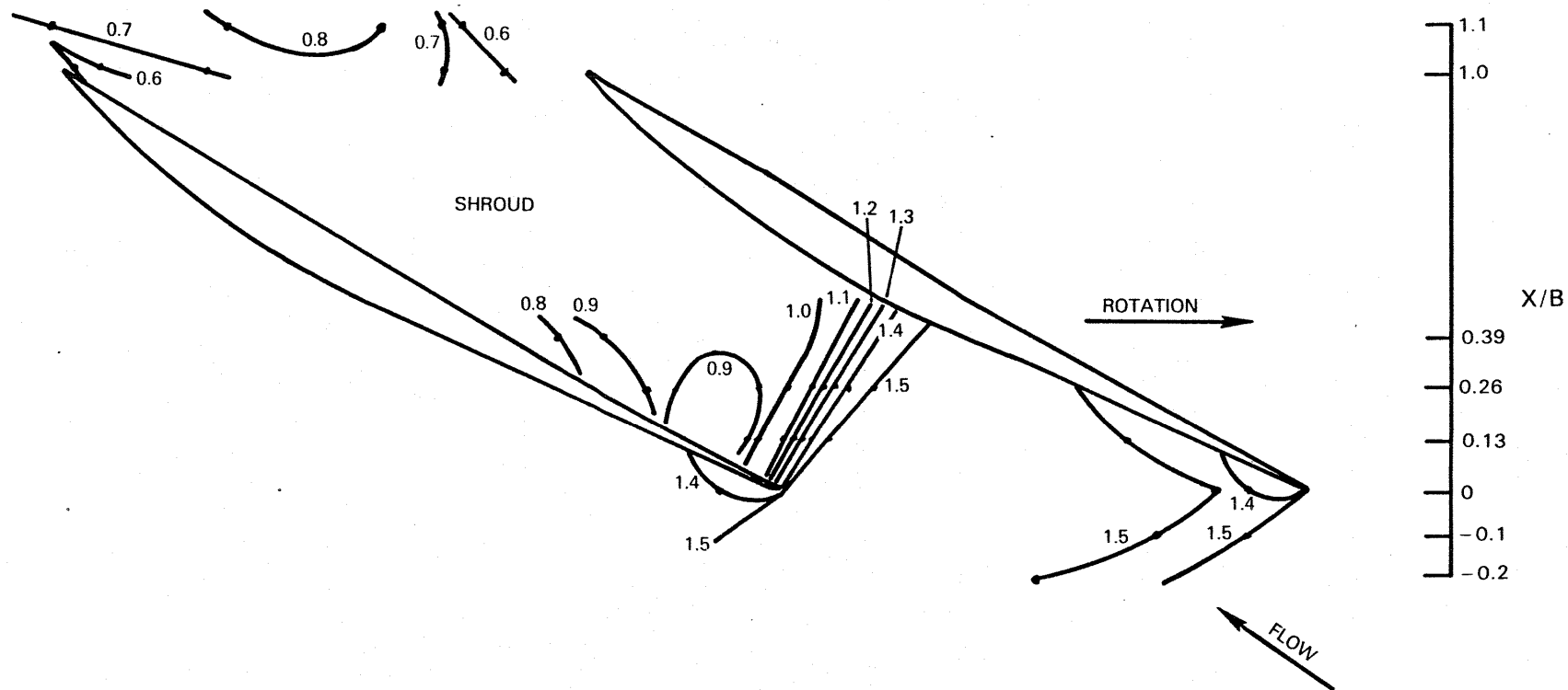
Figure 31 Mach Number Contours at 69 Percent Span, 100 Percent Design Speed, Peak Efficiency - Passage No. 1
