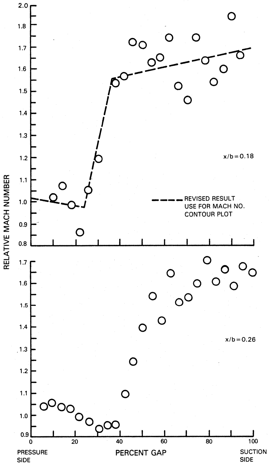
Mach Number Profiles at 95 Percent Span, 100 Percent Design Speed, Peak Efficiency - Passage No. 1
