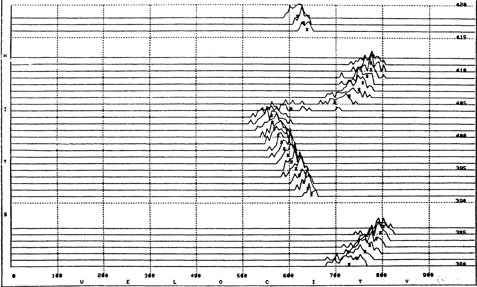
Figure 11 Sample of "Carpet Plot" Type Velocity Histogram X Indicates Mean of Each Location
