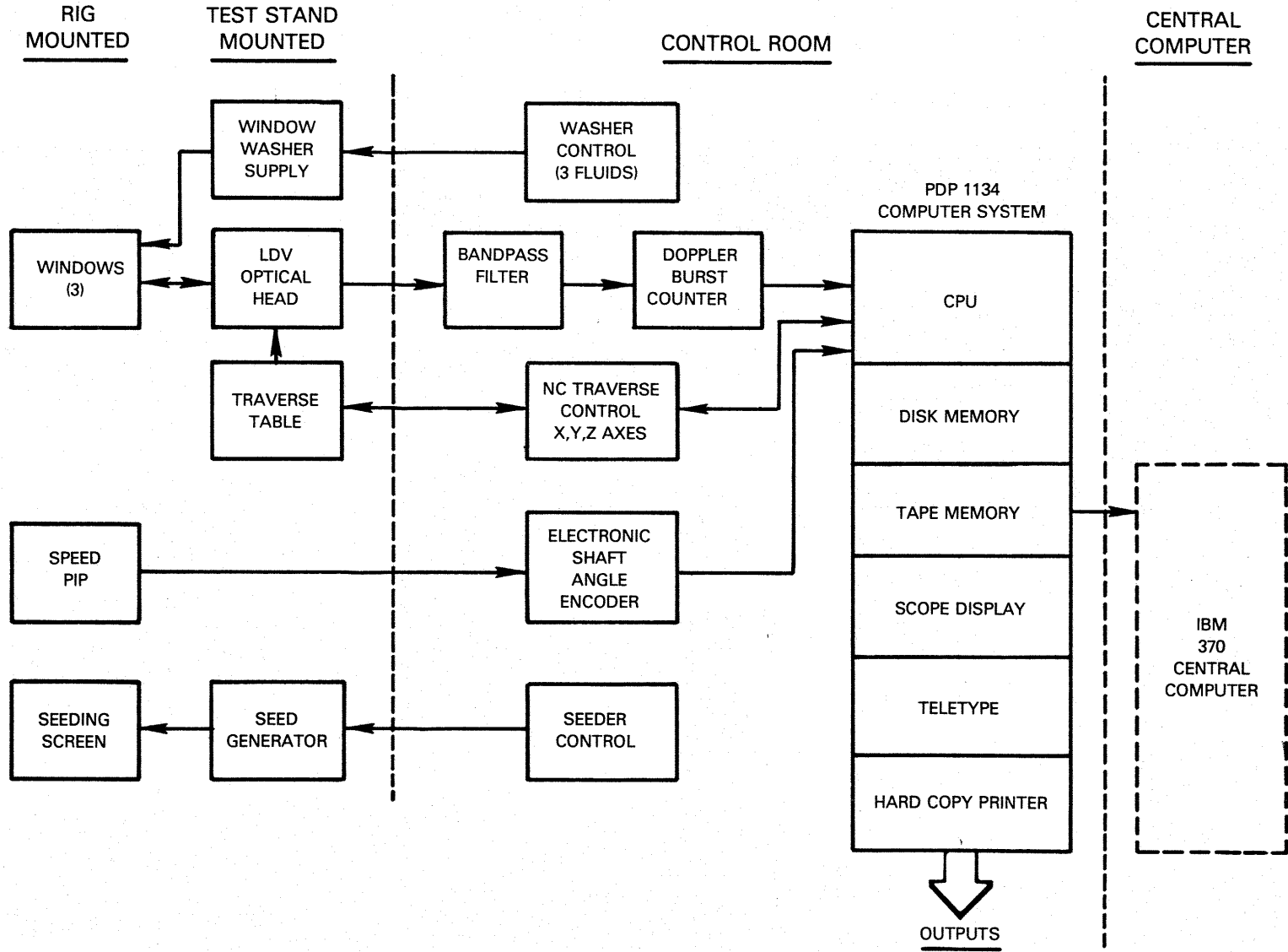
Figure 8 Computer-Controlled Data Acquisition System - Schematic Diagram
