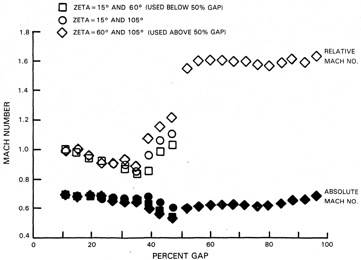
Figure 17 Aerodynamic Results at 85 Percent Span, 100 Percent Design Speed, Near Surge, x/b = 0.26 , Passage No. 1 - Results Have Been Affected by Angle Biasing
