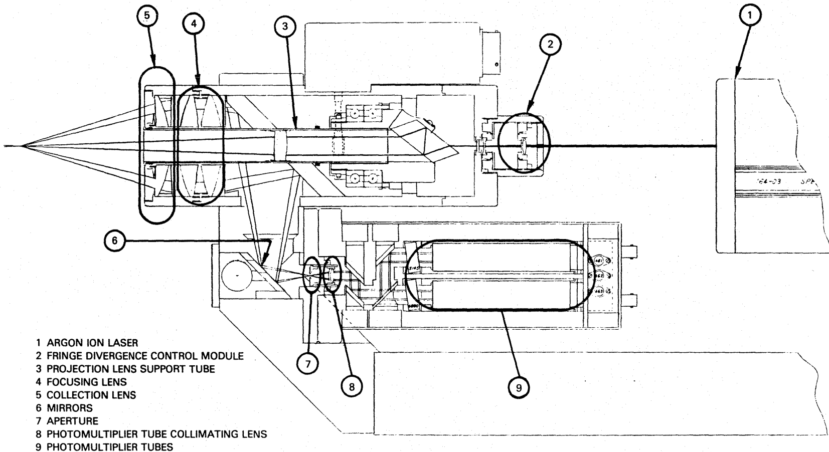
Figure 5 Optical Layout of Laser Doppler Velocimeter
