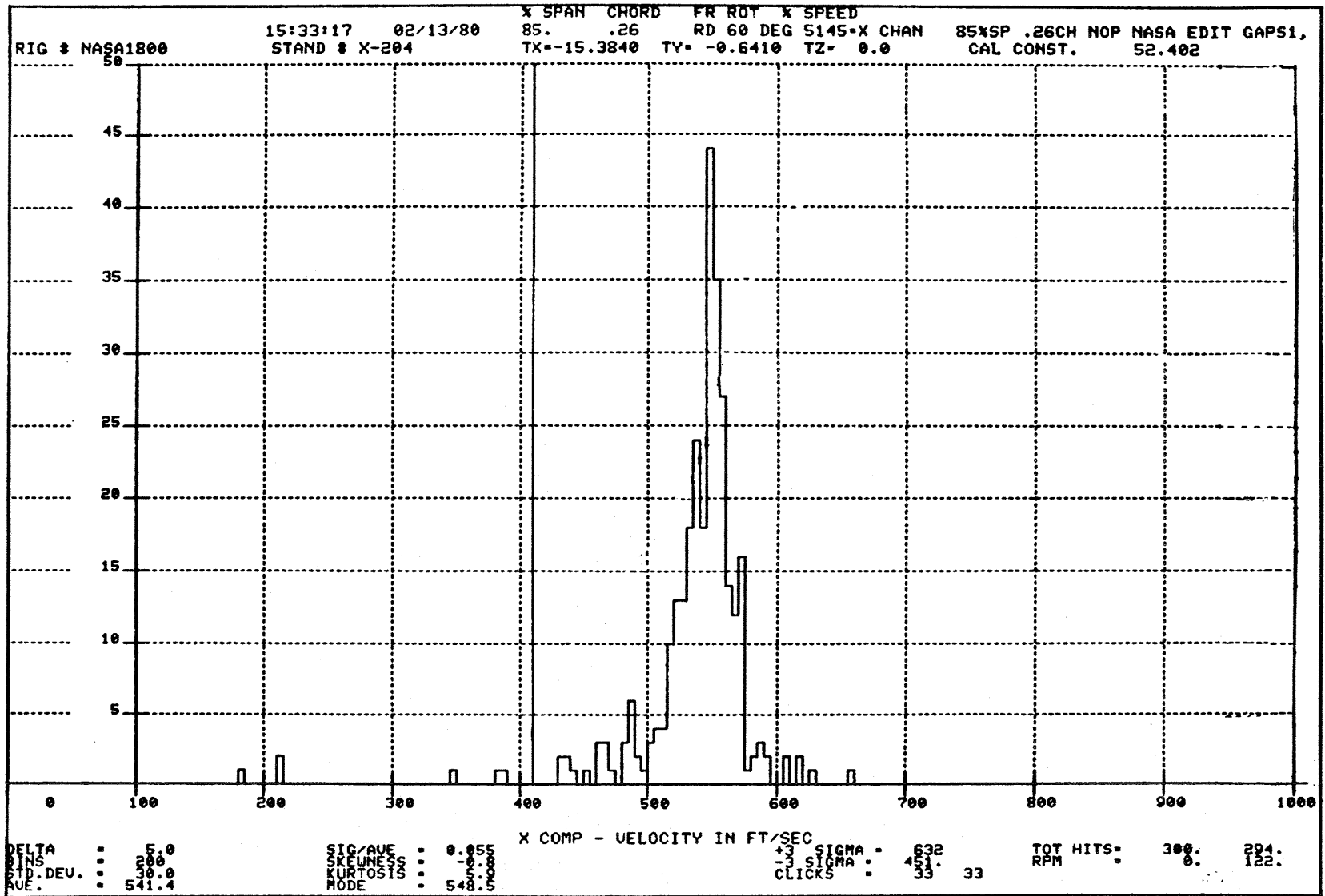
Figure 12 Velocity Histogram
