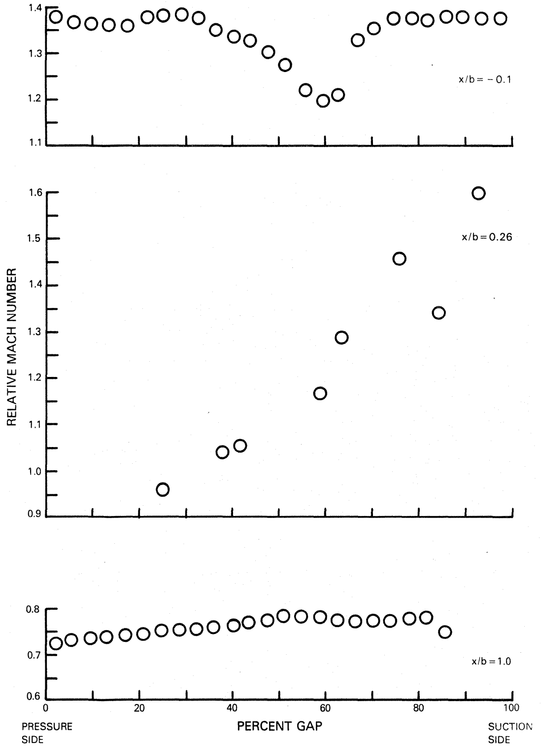
Figure 33 Mach Number Profiles at 45 Percent Span, 100 Percent Design Speed, Peak Efficiency - Passage No. 1
