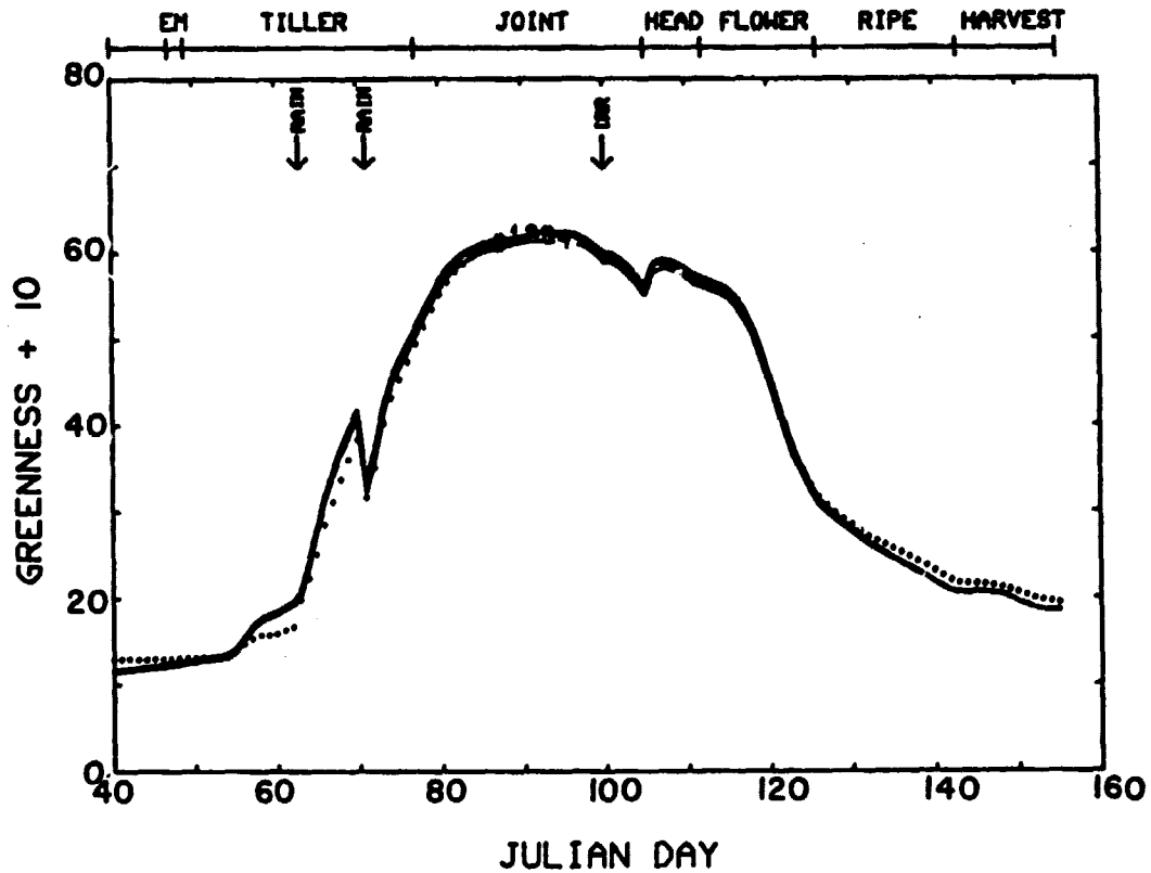
Figure 4. Adjusted greenness values for five levels of path radiance calculated using equation (8) for a dry atmosphere. The "no atmosphere" reference is shown by the dotted line.
