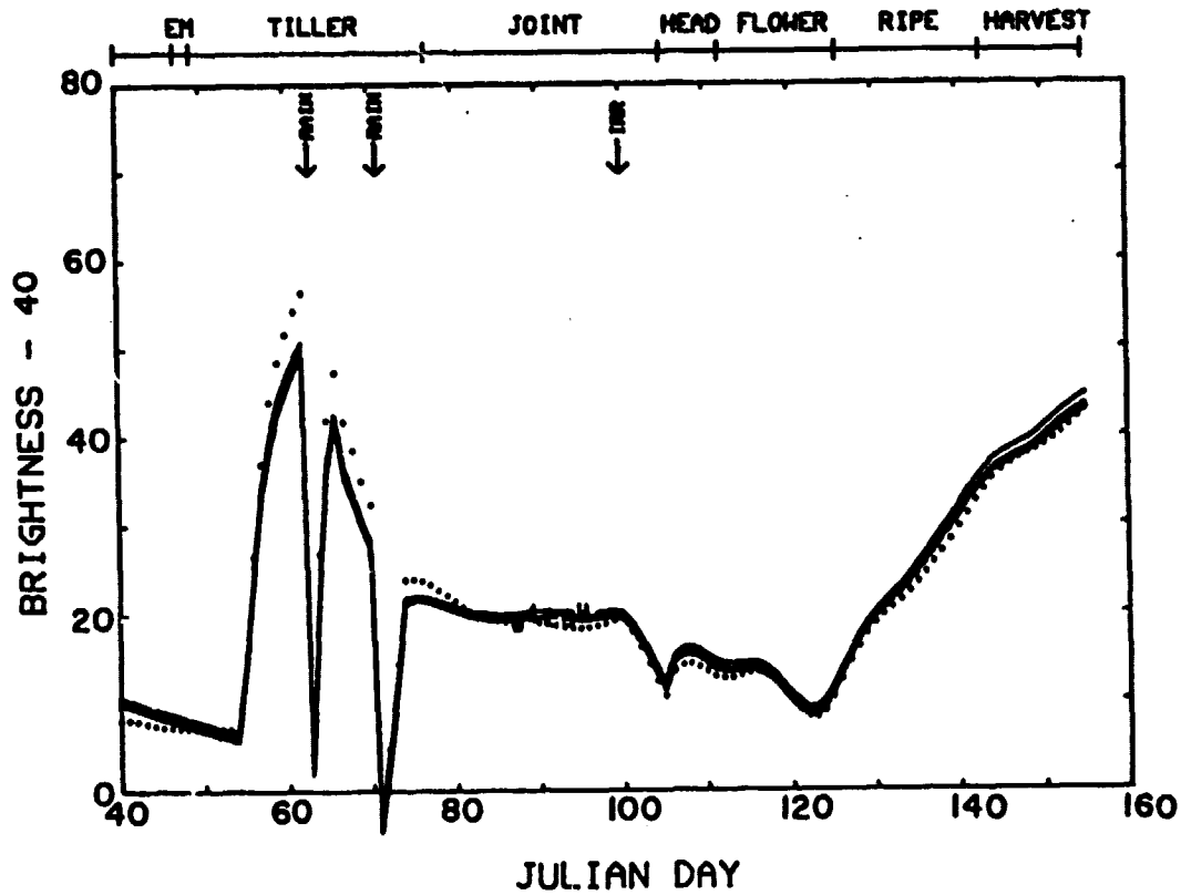
Figure 2. Adjusted brightness values for four levels of path radiance calculated using equation (7) for a dry atmosphere. The "no atmosphere" reference is shown by the dotted line.
