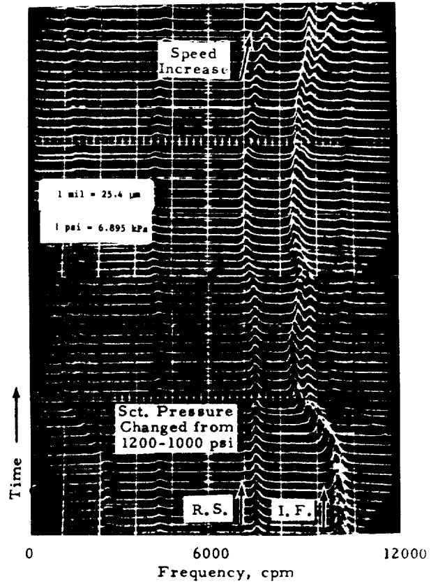
Figure 14. - Variation of instability frequency with suction pressure.
