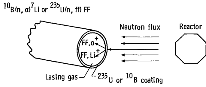
(a) Wall coating technique.
