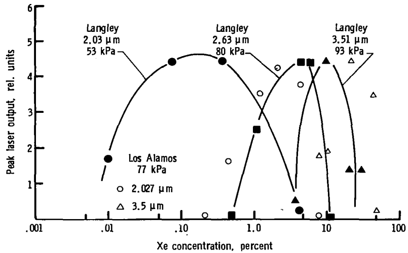
Figure 13.- 3 He-Xe laser output versus Xe concentration.
