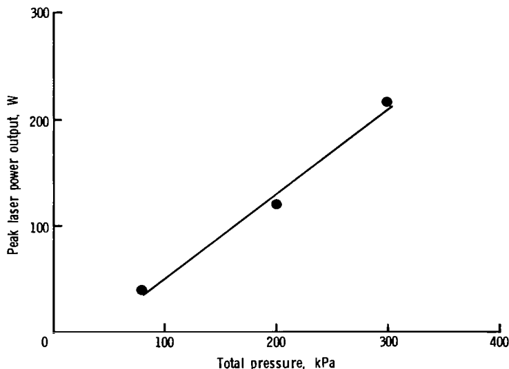
Figure 11.- ^3\text{He-Xe} laser output at 2.63\ \mu\text{m} versus total pressure.
