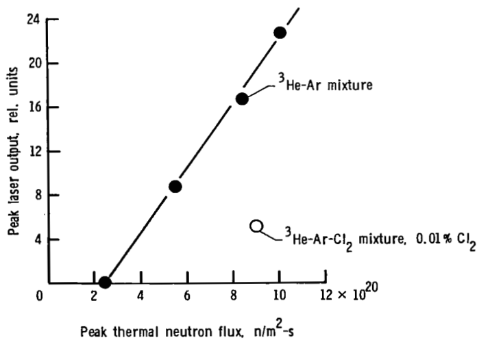
Figure 9.- 3 He-Ar laser output versus thermal neutron flux. 1 percent Ar; p = 80 \text{ kPa} .
