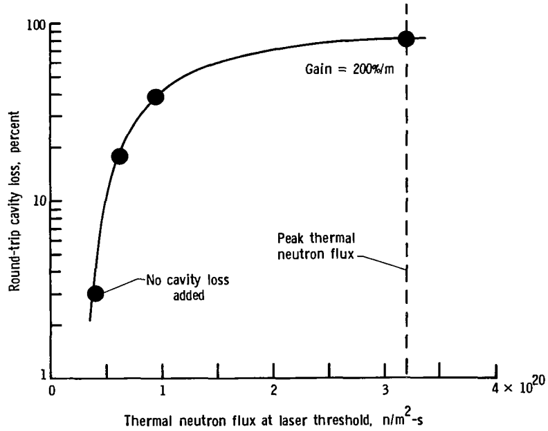
Figure 14.- Gain of 3 He-Xe laser at 2.03 μm. Gain length = 0.40 m; 0.5 percent Xe; p = 100 kPa.
