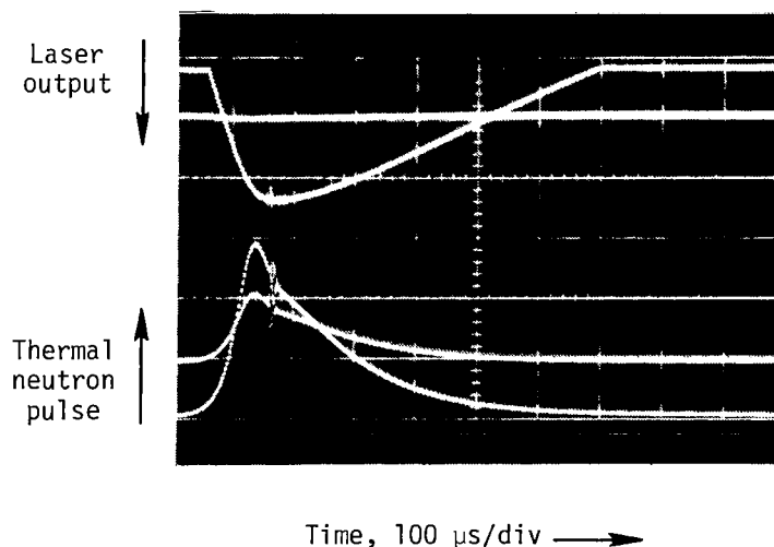
Figure 10.- Oscilloscope photograph of ^3\text{He} -Xe laser output at 2.03 \mu\text{m} .
