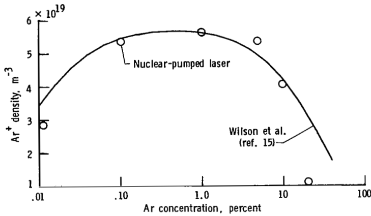
Figure 8.- 3 He-Ar laser output at 1.79 μm versus Ar concentration. p = 53 \text{ kPa} ; \phi = 6 \times 10^{20} \text{ n/m}^2\text{-s} .
