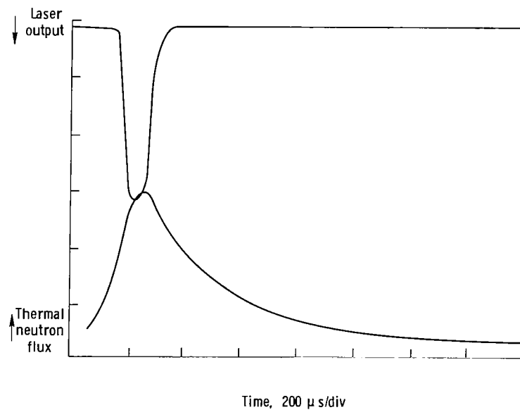
Figure 17.- Oscilloscope recording of ^3\text{He} -CO laser output.
