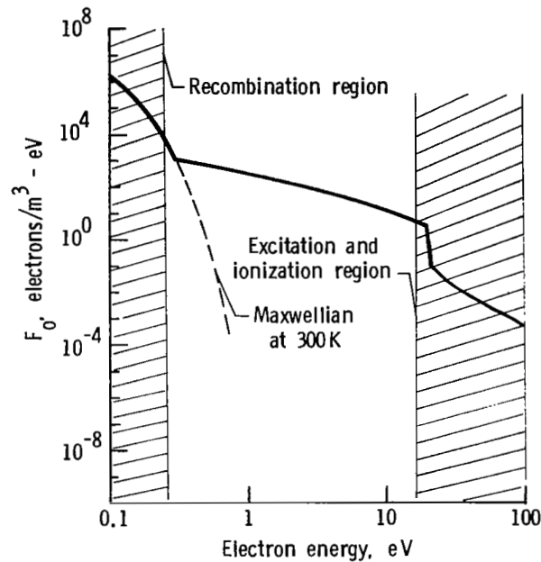
Figure 2.- Calculated electron energy distribution function F_0 in a nuclear-induced He plasma. p = 13.3 kPa; T = 300 K; \phi = 10^{20} \text{n/m}^2\text{-s} .
