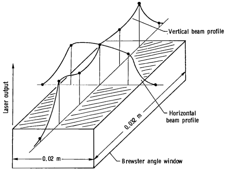
Figure 24.- Beam profile of multiple-pass box laser ( ^3\text{He-Ar} ). 1 percent Ar; p = 300 kPa; 5 passes; \phi = 2.7 \times 10^{20} n/m 2 -s.
