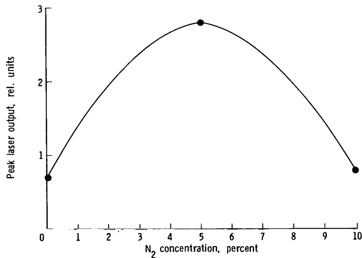
Figure 19.- ^3\text{He} -CO laser output versus N 2 concentration. 5 percent CO; p = 80 \text{ kPa} .
