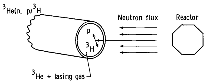
(b) Volumetric pumping technique.
